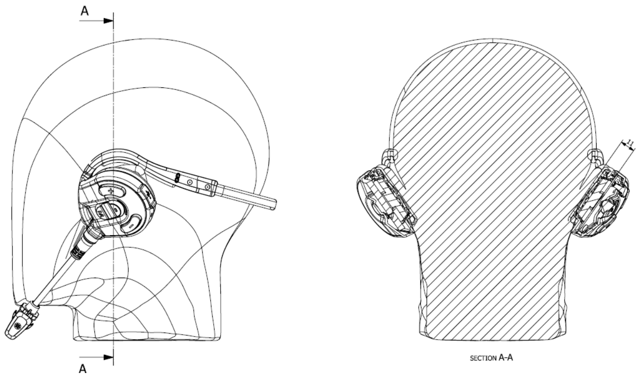
Figure E-1 Antenna Location
