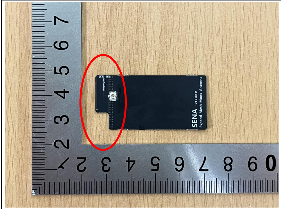
MESH Antenna 2 (M/N: Expand-Mono)
