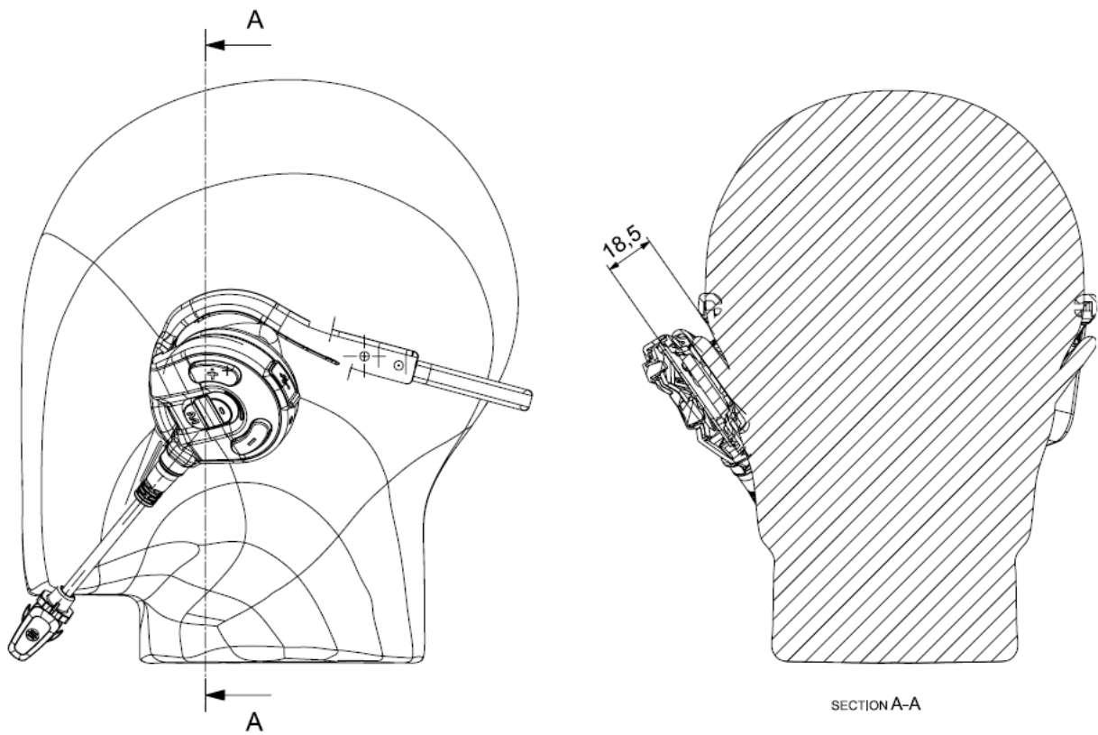
Figure E-1 Antenna Location
