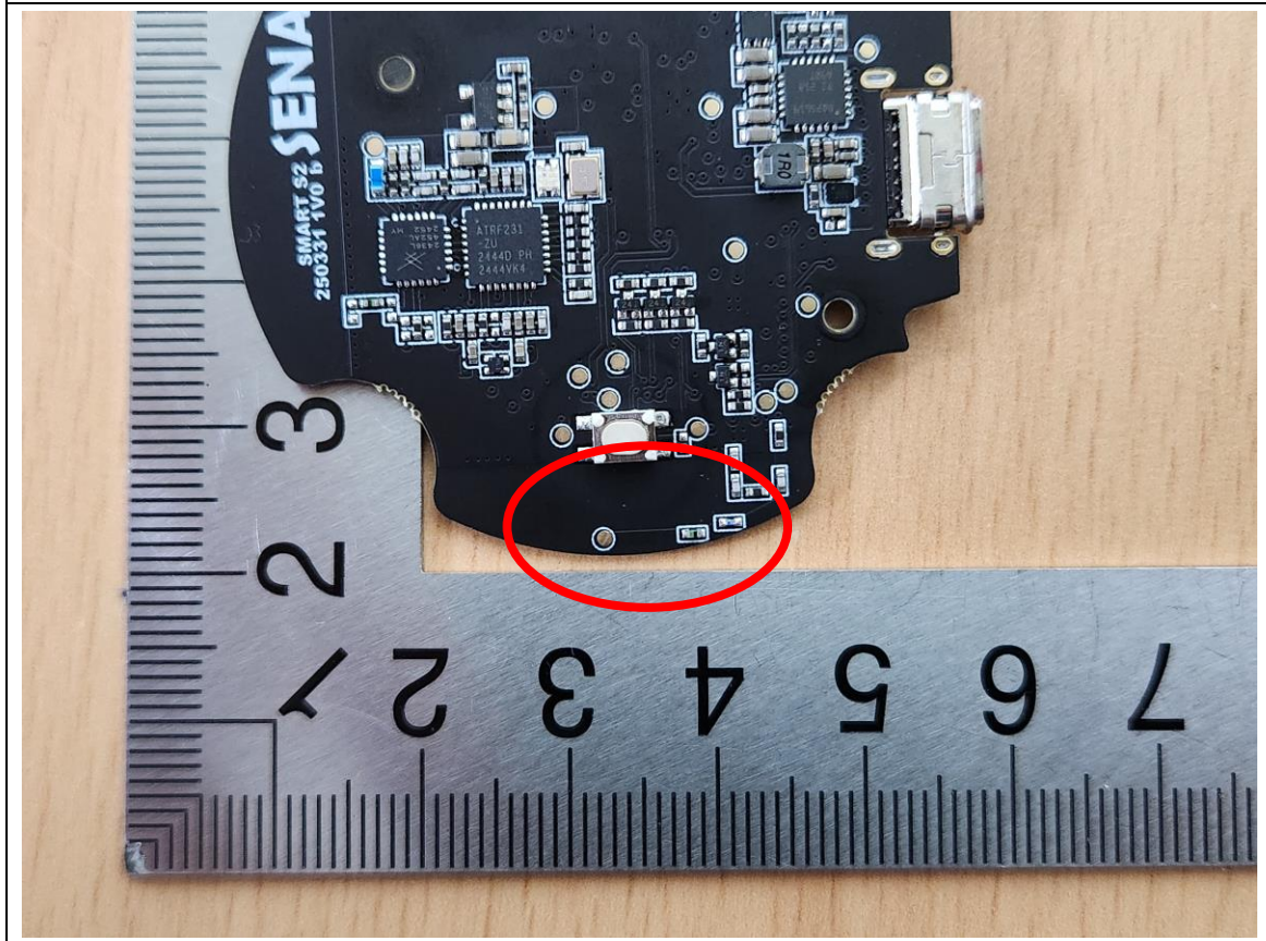
BT Antenna (M/N: LATITUDU S2 Bluetooth)
