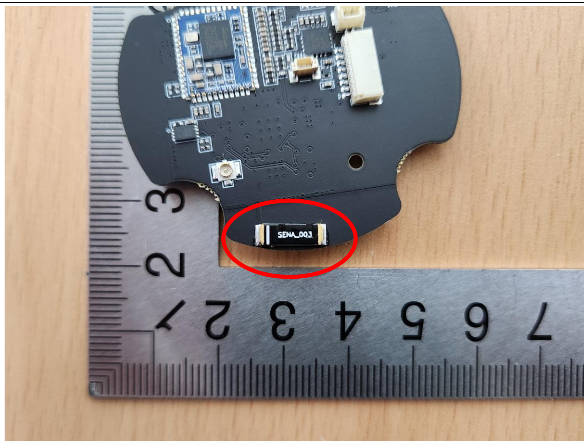
MESH Antenna 1 (M/N: SENA_003)
