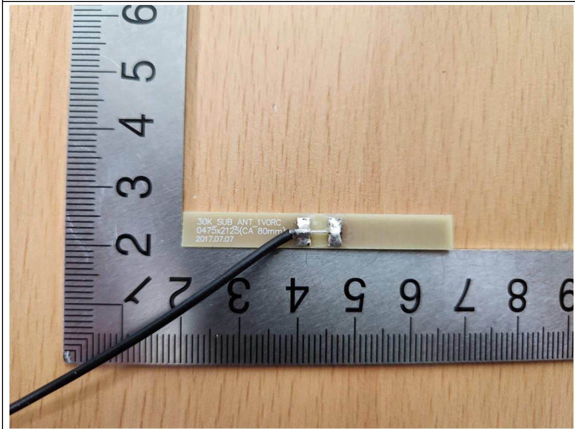
MESH Antenna 1
