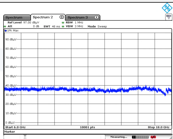
Vertical // Peak for 6 GHz to 18 GHz
