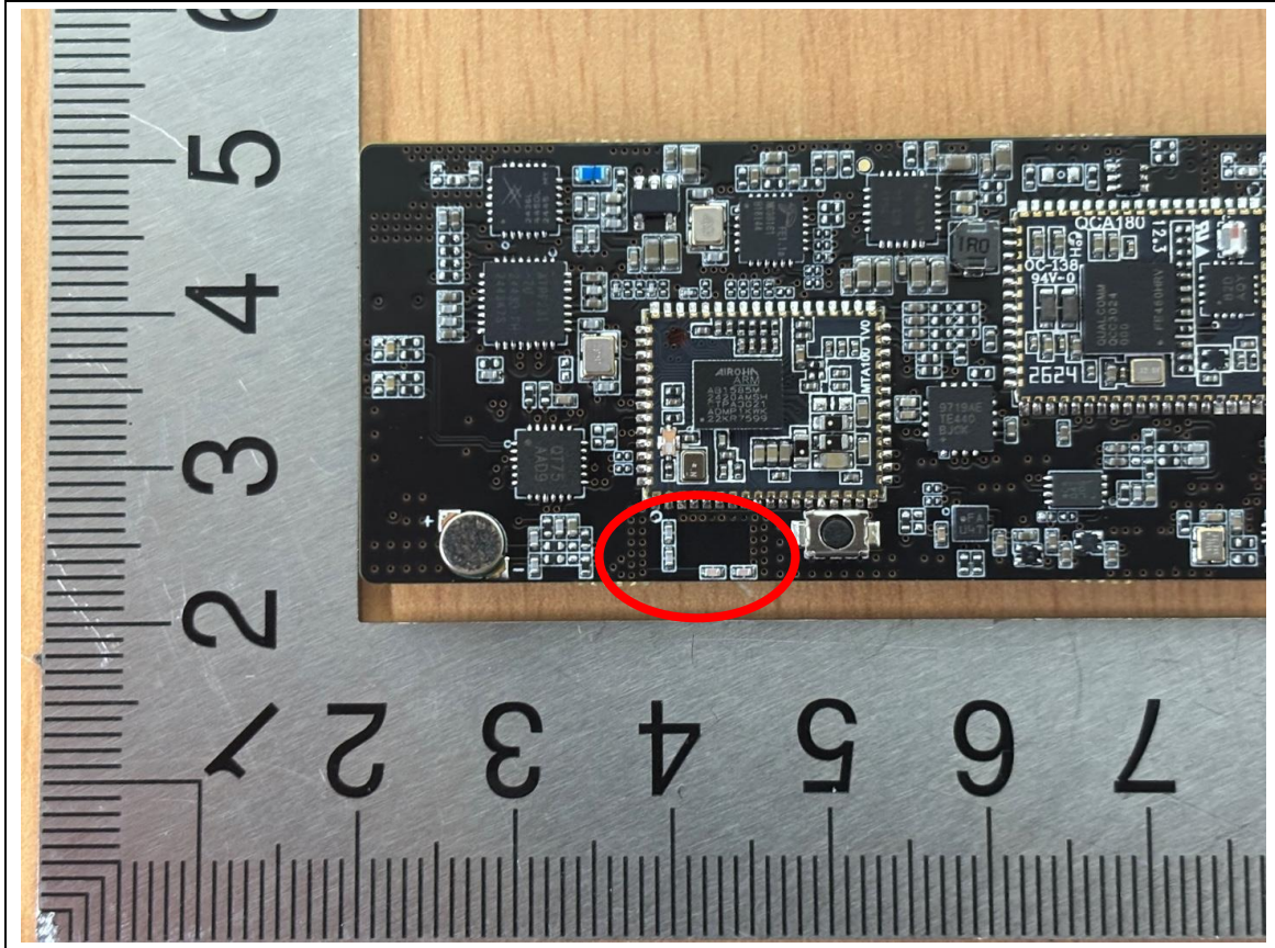
BT Antenna(BT2)
