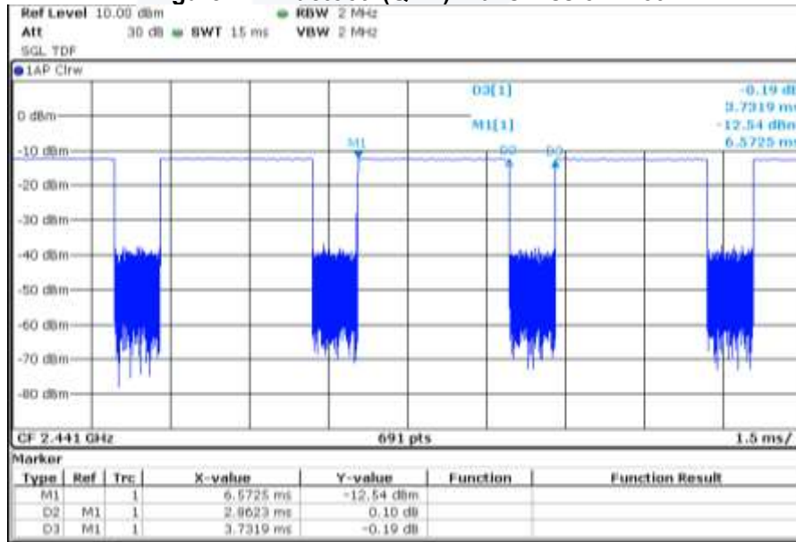
Figure 7-2 Bluetooth(QCC) Transmission Plot
