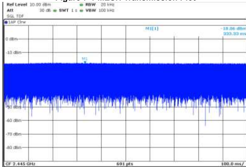
Figure 7-1 MESH Transmission Plot
