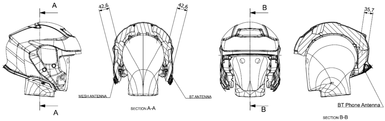
Figure E-1 Antenna Location
