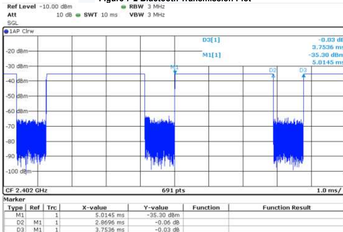
Figure 7-2 Bluetooth Transmission Plot
