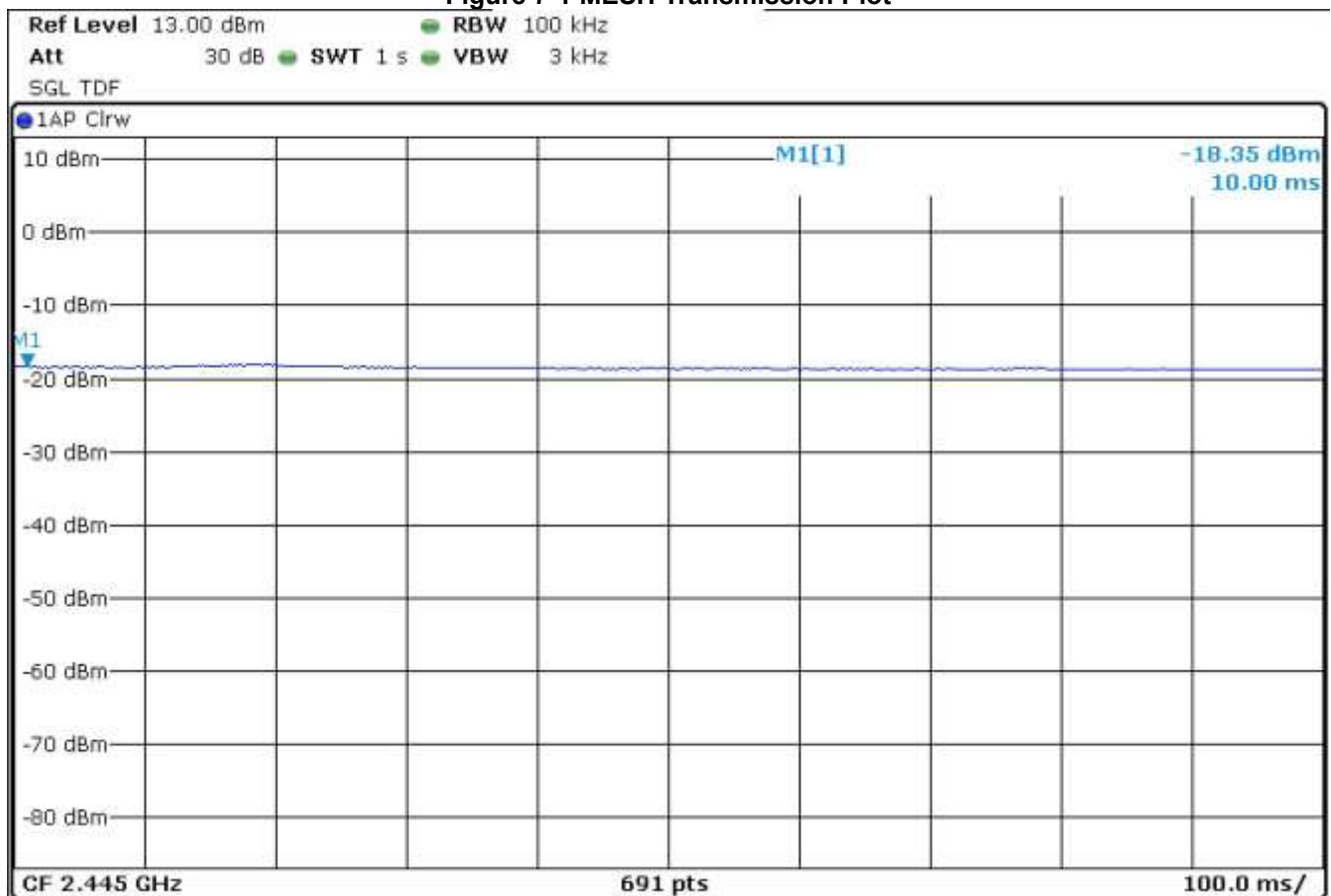
Figure 7-1 MESH Transmission Plot
