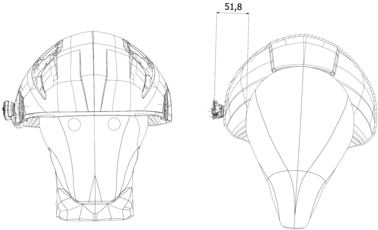
Figure E-1 Antenna Location
