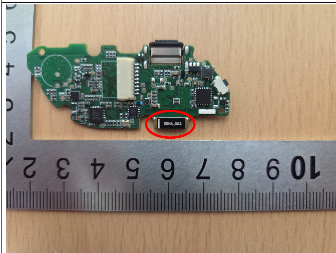
MESH Antenna
