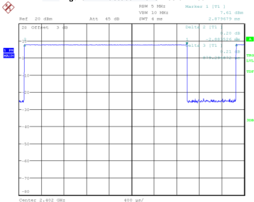
Figure 7-2 Bluetooth Transmission Plot
