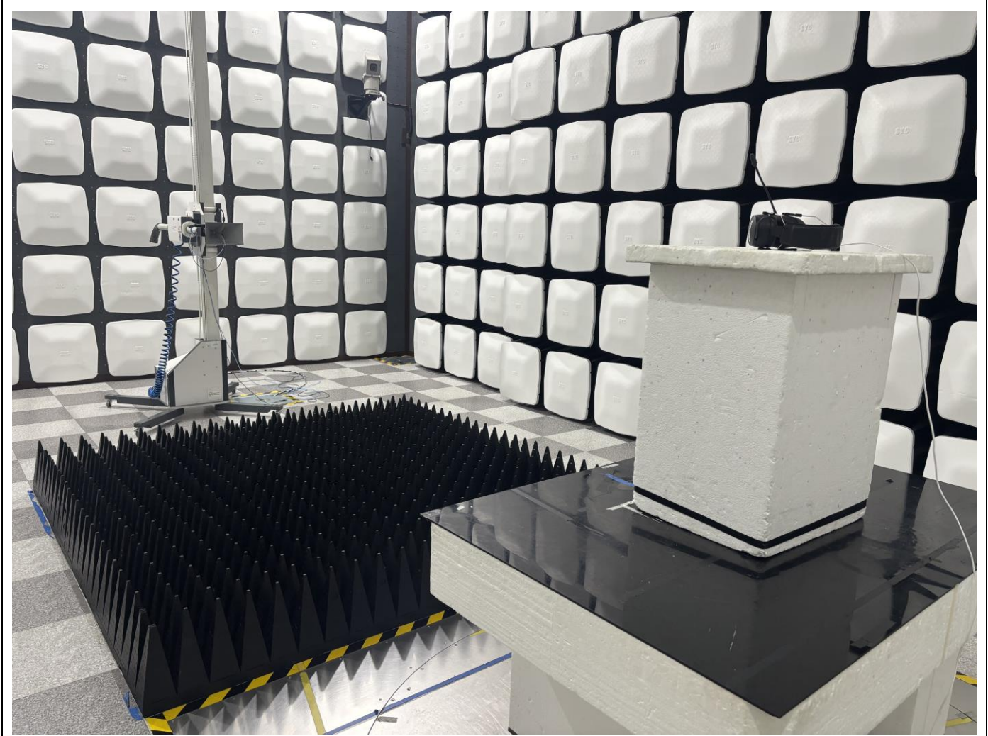
Above 1 GHz
