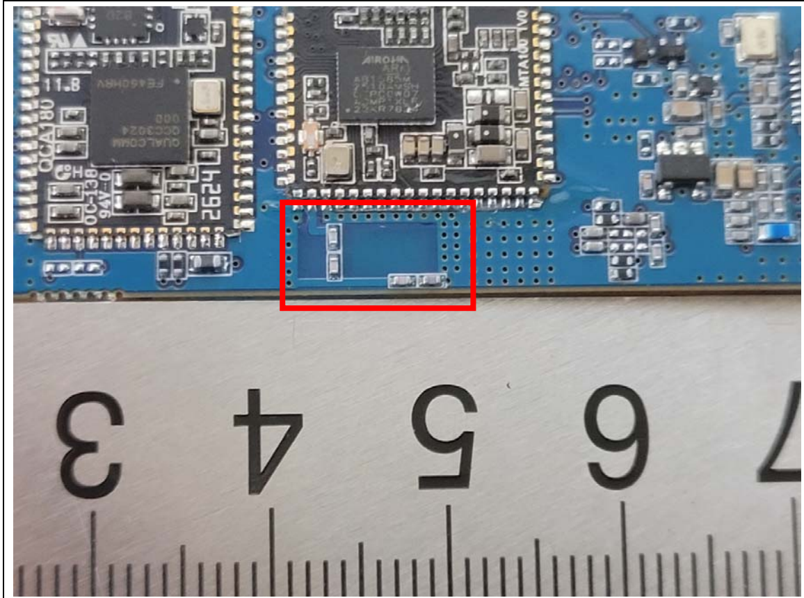
BT Antenna(BT2)
