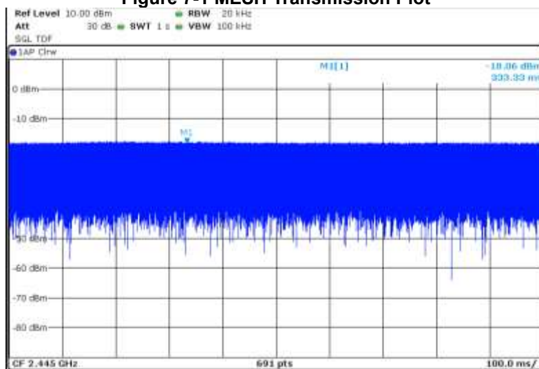
Figure 7-1 MESH Transmission Plot
