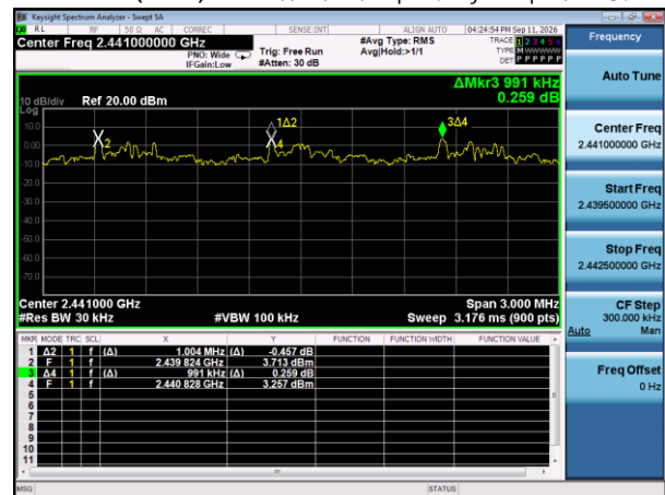
8DPSK(BT2) – Carrier Frequency Separation
