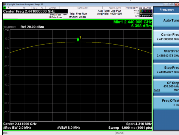
GFSK Mid Channel – Peak Output Power
