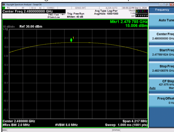
GFSK High Channel – Peak Output Power
