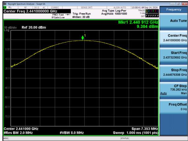
Pi/4 DQPSK Mid Channel – Peak Output Power
