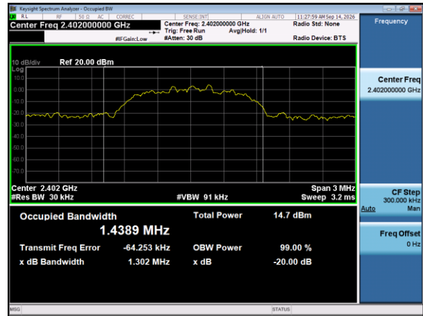
8DPSK Low Channel – 20 dB Bandwidth & Occupied Bandwidth
