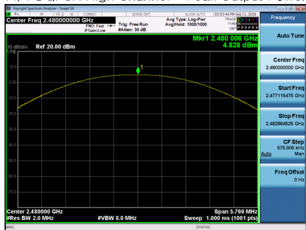
Pi/4 DQPSK High Channel – Peak Output Power
