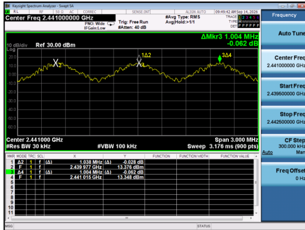
GFSK(BT1) – Carrier Frequency Separation
