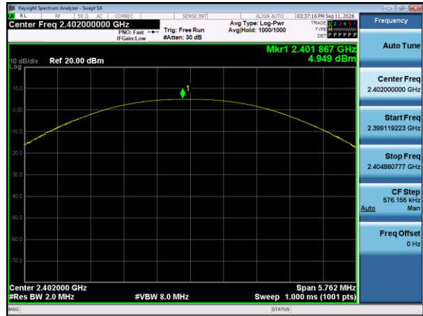
Pi/4 DQPSK Low Channel – Peak Output Power
