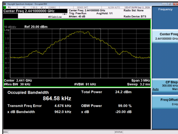
GFSK Mid Channel – 20 dB Bandwidth & Occupied Bandwidth
