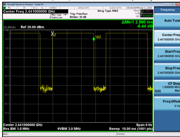
GFSK(BT2) – Time of Occupancy
