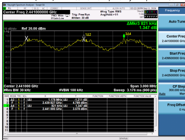
GFSK(BT2) – Carrier Frequency Separation
