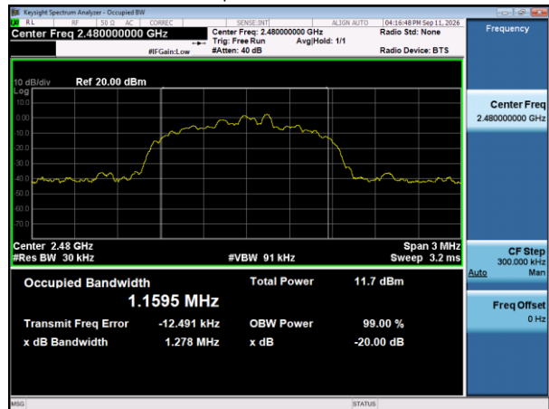
8DPSK High Channel – 20 dB Bandwidth & Occupied Bandwidth
