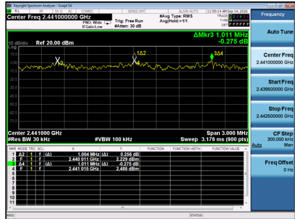
8DPSK(BT1) – Carrier Frequency Separation
