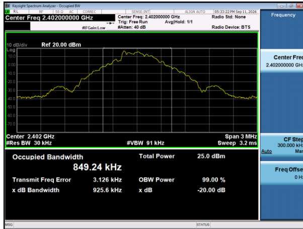
GFSK Low Channel – 20 dB Bandwidth & Occupied Bandwidth
