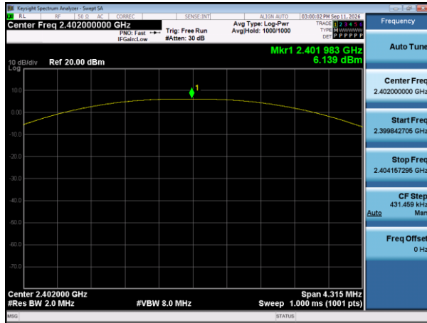
GFSK Low Channel – Peak Output Power
