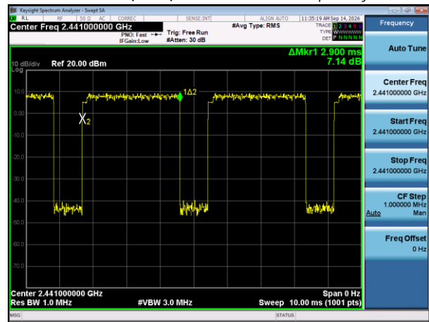
8DPSK(BT2) – Time of Occupancy
