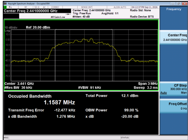
8DPSK Mid Channel – 20 dB Bandwidth & Occupied Bandwidth
