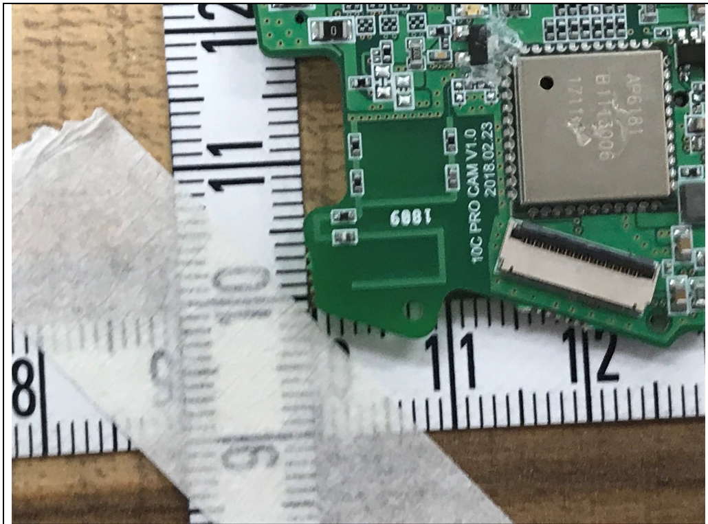
<WiFi ANTENNA>
