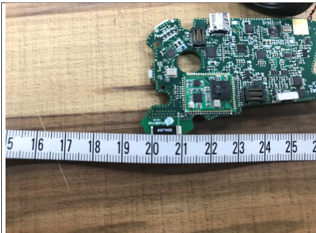
<Bluetooth ANTENNA>
