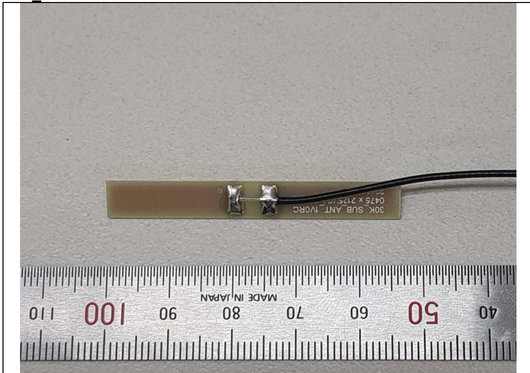
M1_Antenna Board Rear
