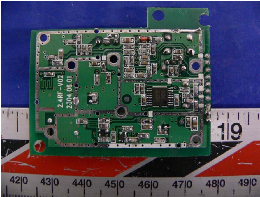
Base – Transmitter Solder View
