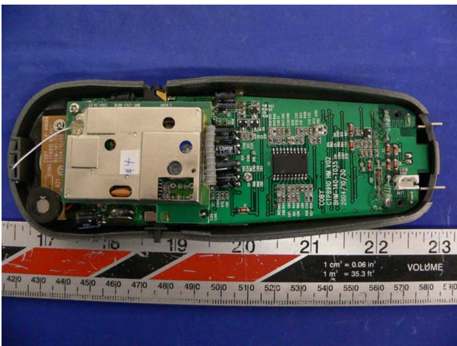
Handset – Chassis Cover Off View
