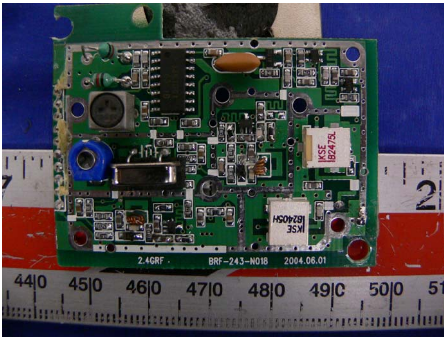
Base – Transmitter Component View
