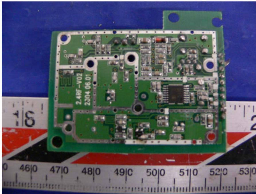
Handset – Transmitter Solder View
