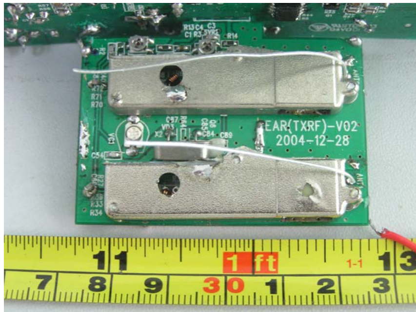
EUT- Antenna PCB Back View (2)
