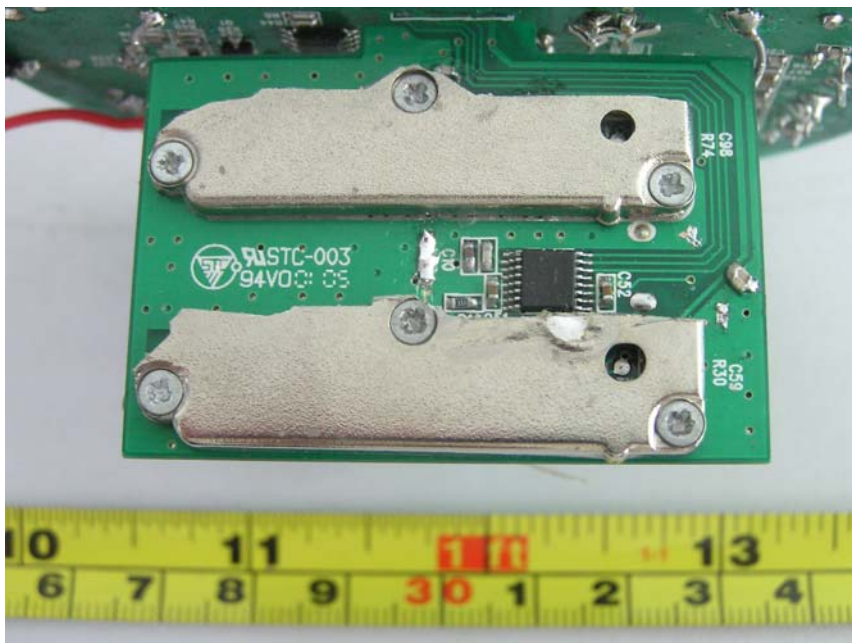
EUT- Antenna PCB Back View (1)
