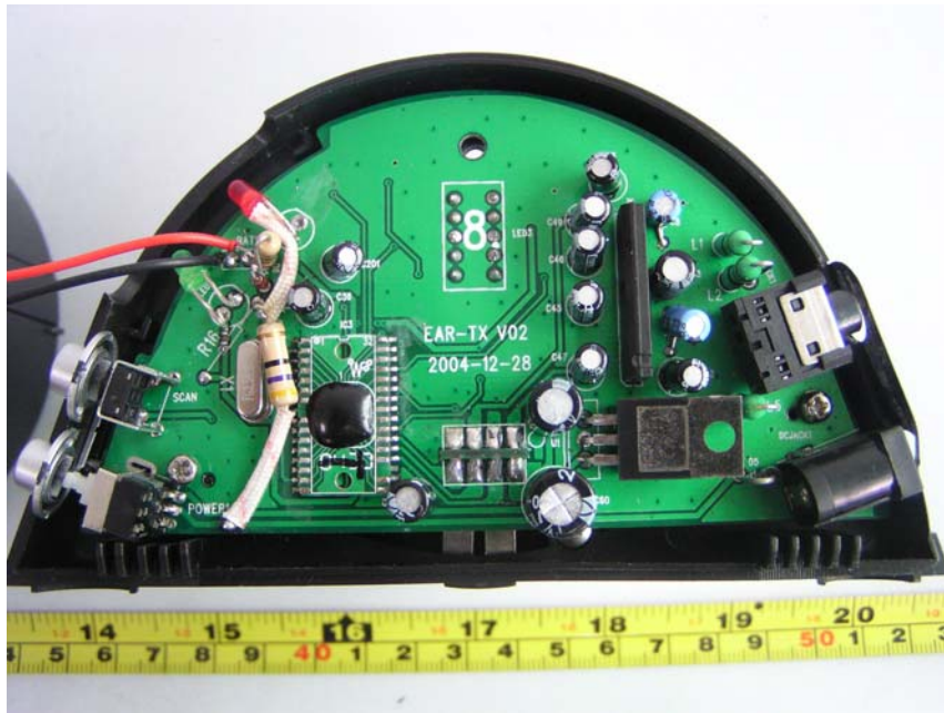
EUT- Inside View (3)
