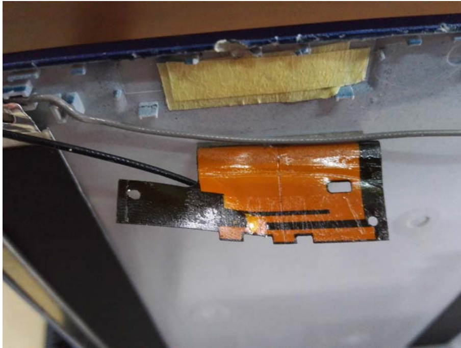
WIFI+BT Antenna(Main Antenna)
