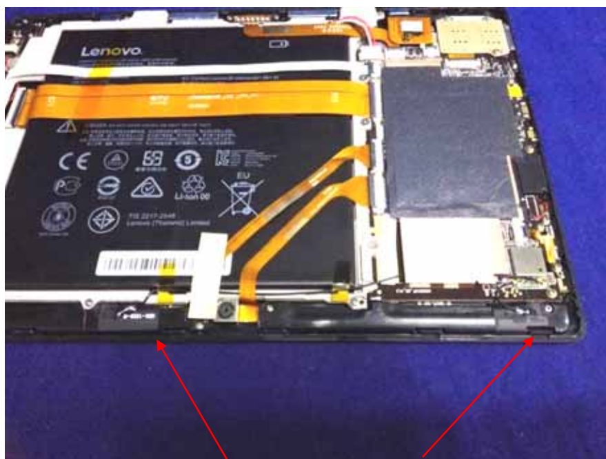
WIFI ANTENNA
