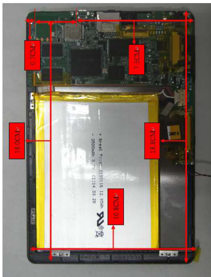
Distance of the Antenna to the EUT surface/edge
