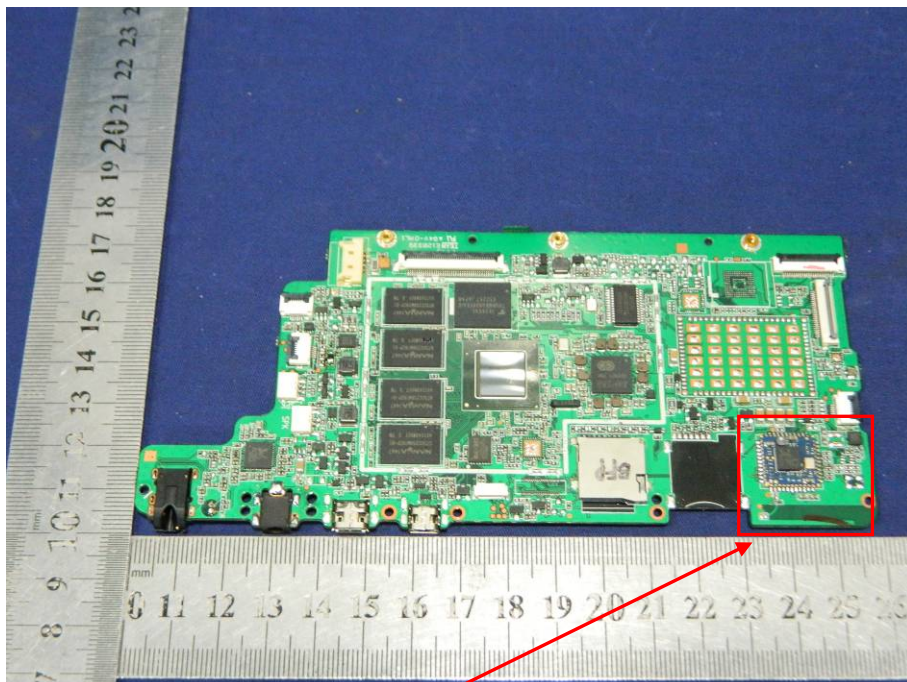
WIFI+Bluetooth Module
