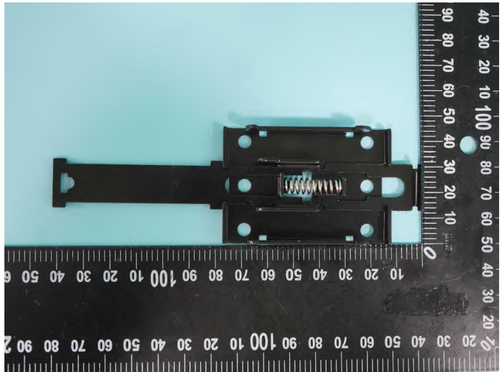
DIN-RAIL mounting bracket kit You Chang Hardware Co., Ltd / 35mm Din Rail Clip
