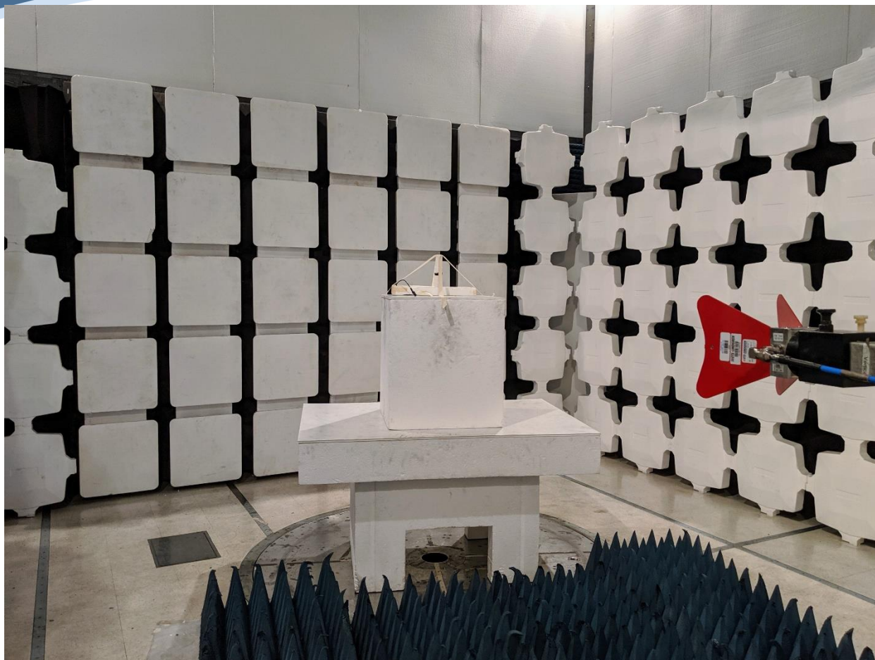
Transmitter Spurious Emissions 1-18 GHz
