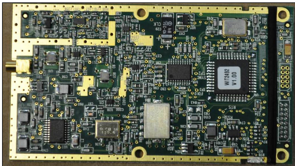
Figure 6: Internal Photo – Top of RF Module
