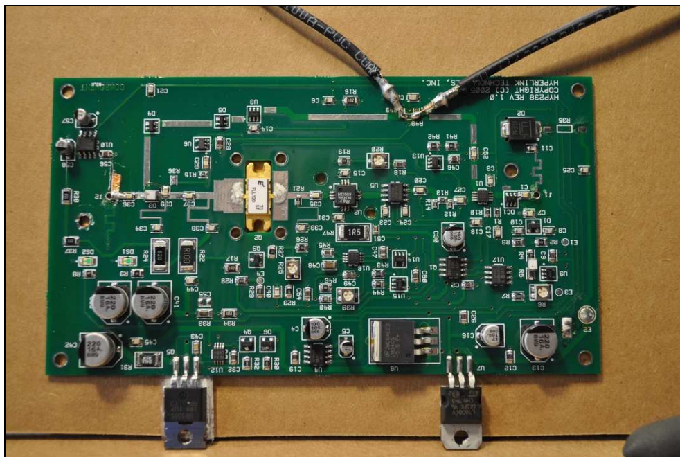
Figure 8: Internal Photo – Top of Amplifier Board
