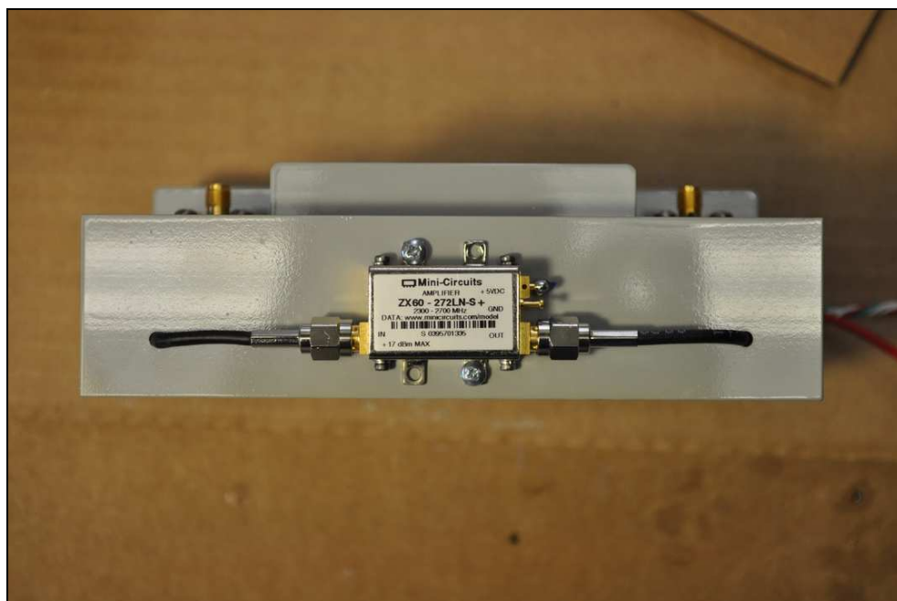
Figure 3: Internal Photo – Side View of RF Amplifier
