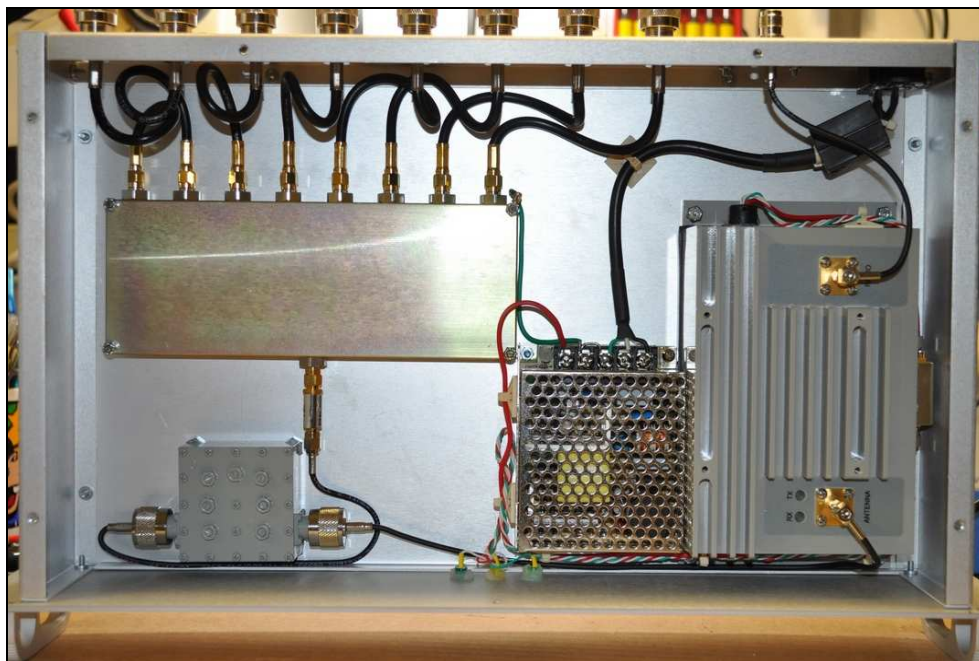
Figure 1: Internal Photo – DAS2400 Interior View
