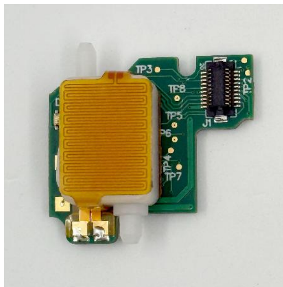
Alcohol Sensor PCBA, with sensor. Front view with slight angle to show PCBA.
