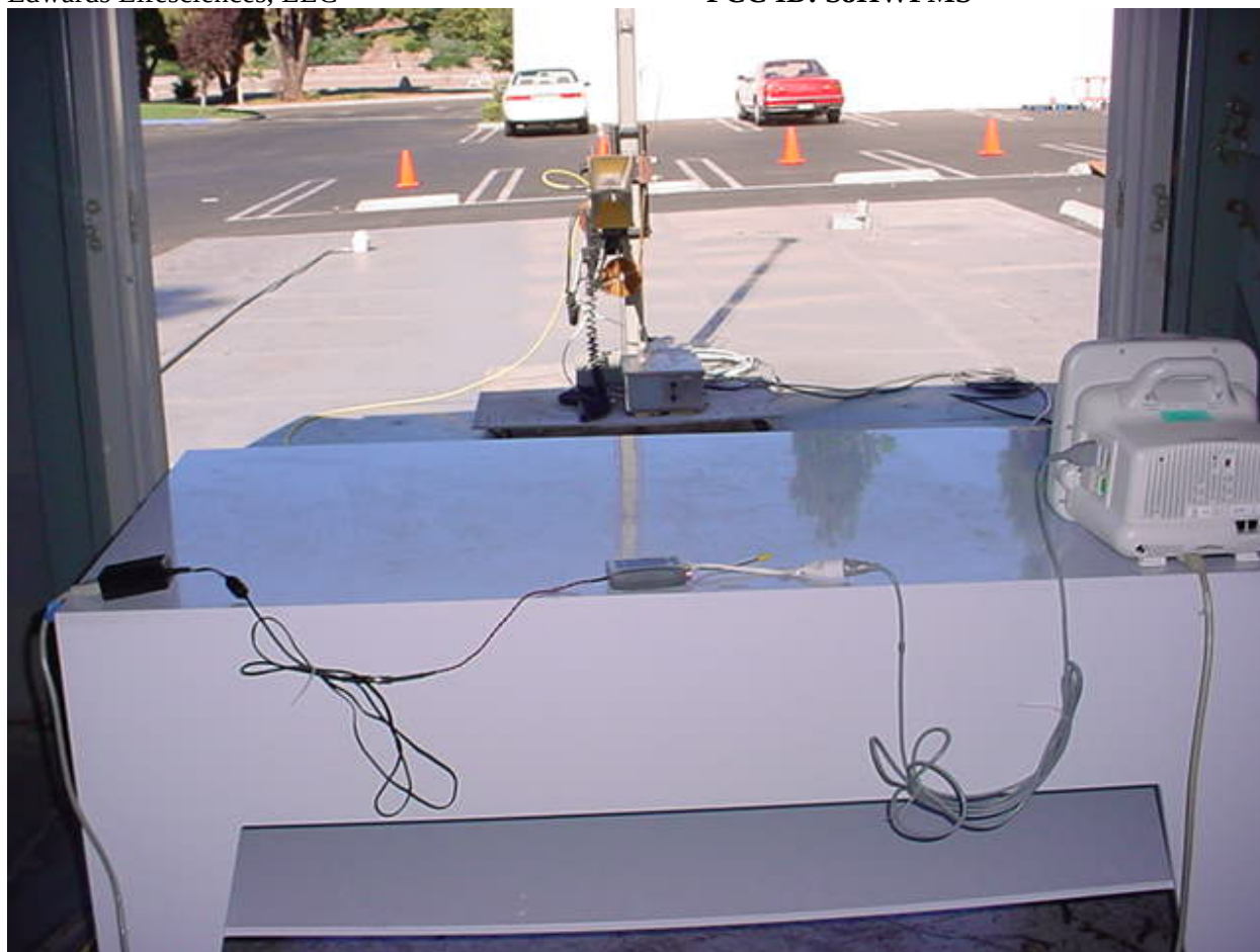
M Unit, Field Strength emission measurements (95.1115(a)(2) & (b)(2))
