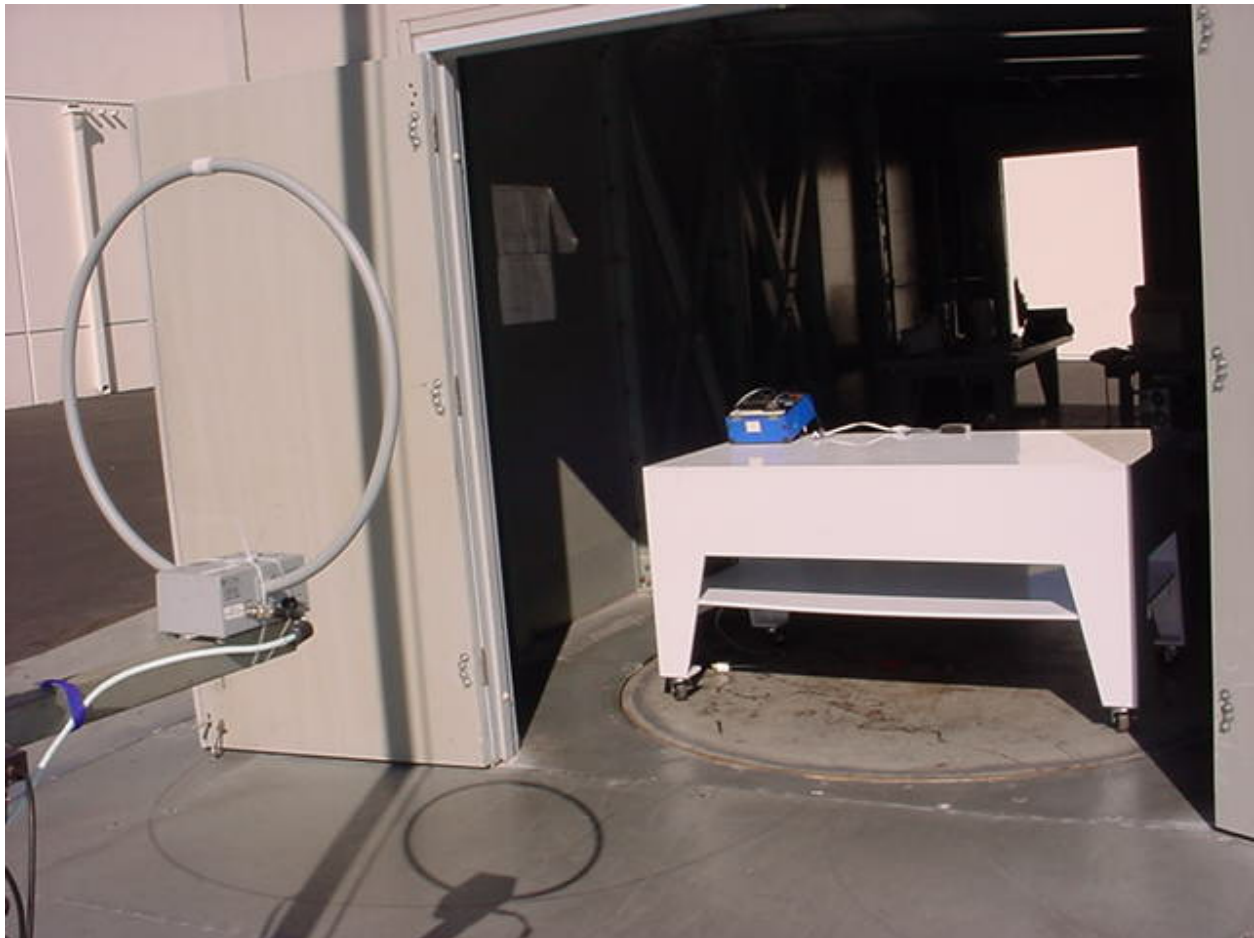
X Unit, RFID Field Strength emission measurements (15.209)
