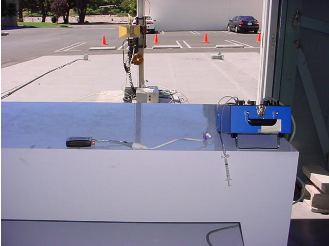
X Unit, Field Strength emission measurements (15.109/209/95.1115(a)(2) & (b)(2))
