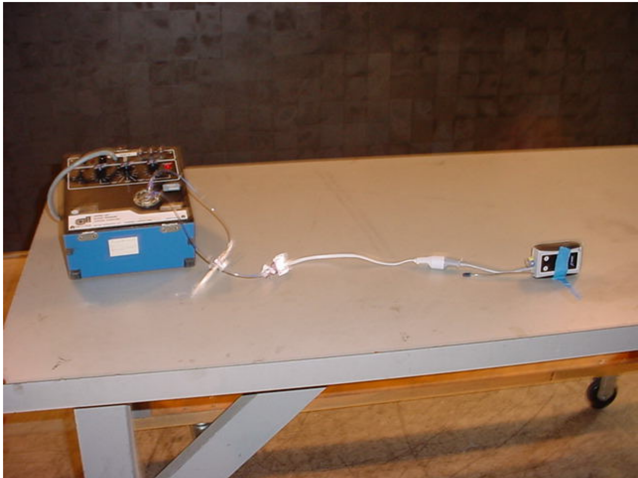
X Unit, System Setup
