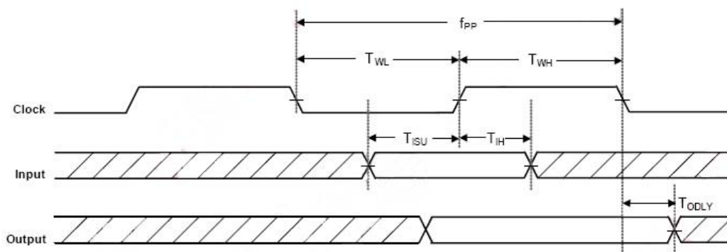
Figure 39: SDIO Protocol Timing Diagram—Normal Mode
