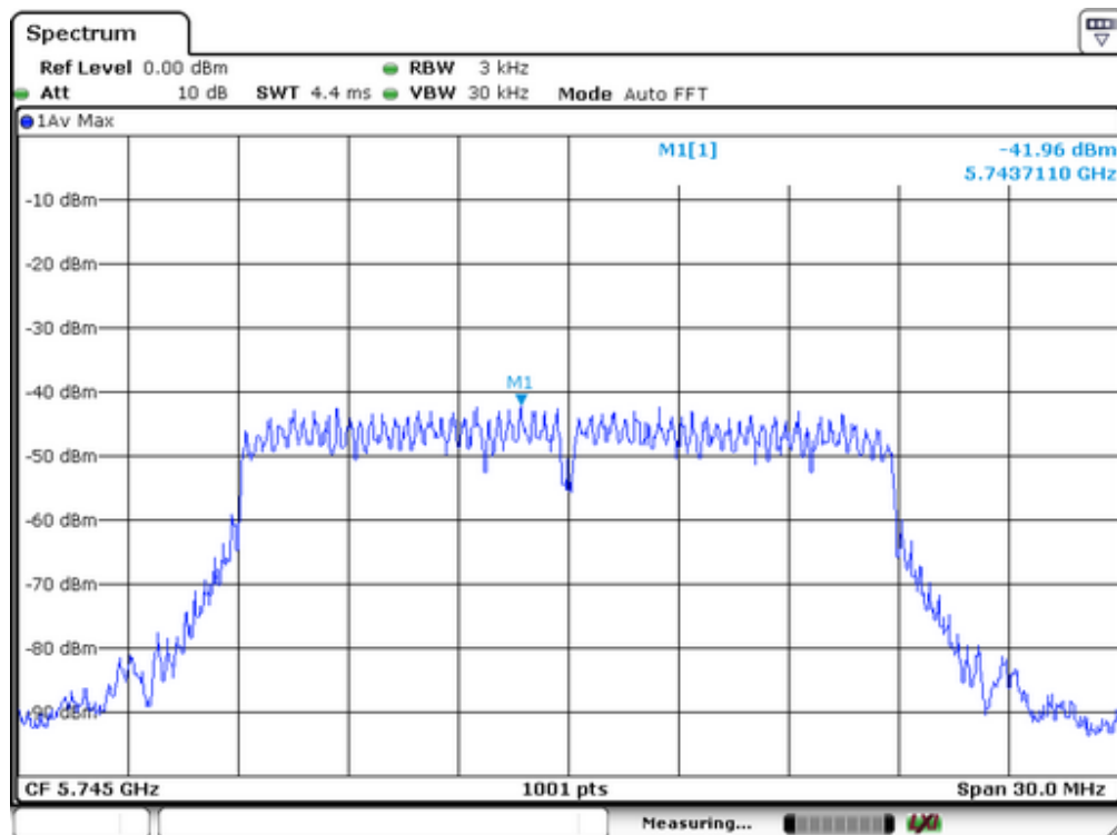
Power Density Plot on Configuration IEEE 802.11ac(HT20) at 5745 MHz
