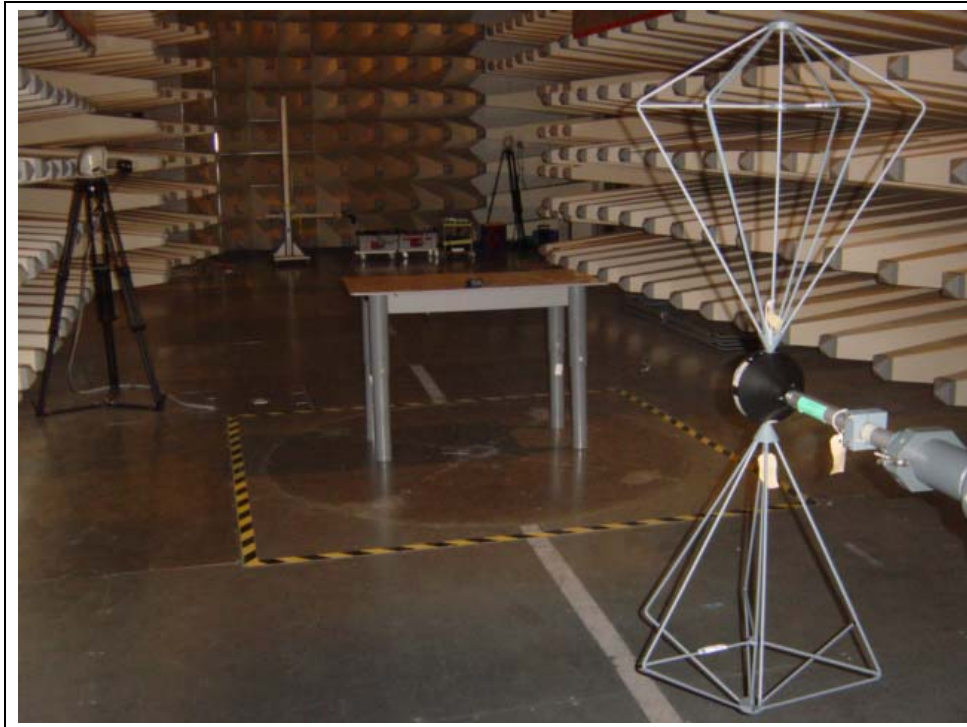
Test Setup of Radiated Spurious Emission (Receiver)
