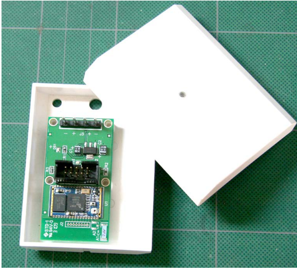
SLN05, PCB 1 mounted in enclosure
