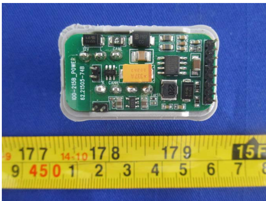
EUT – Sub Board View
