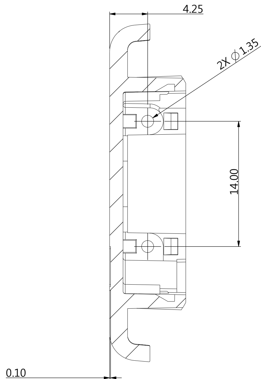
SECTION B-B
