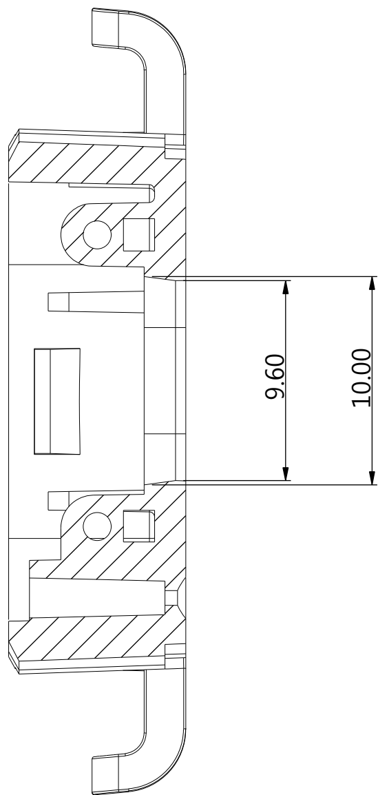
SECTION C-C
