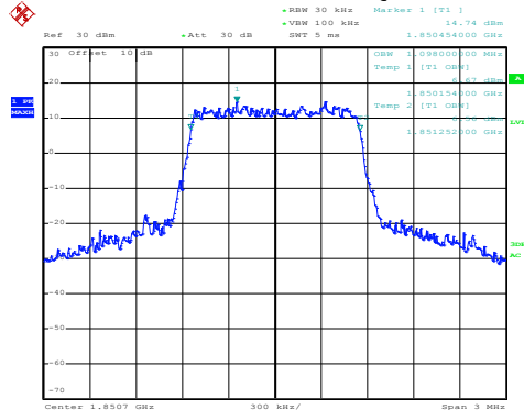
Modulation: 16QAM
