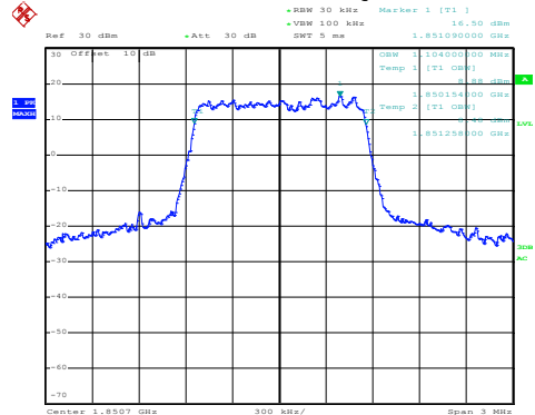
Modulation: QPSK
