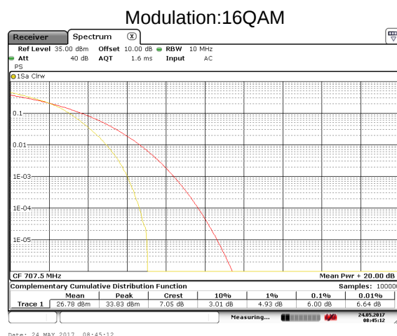
LTE Band 12 Middle channel
