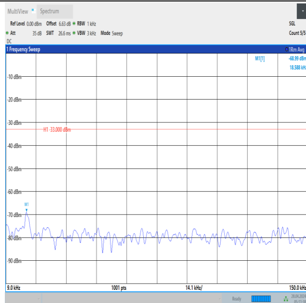
Band12_1.4MHz_QPSK_23095_1RB#5_0.009~0.15_0.009~0.15
