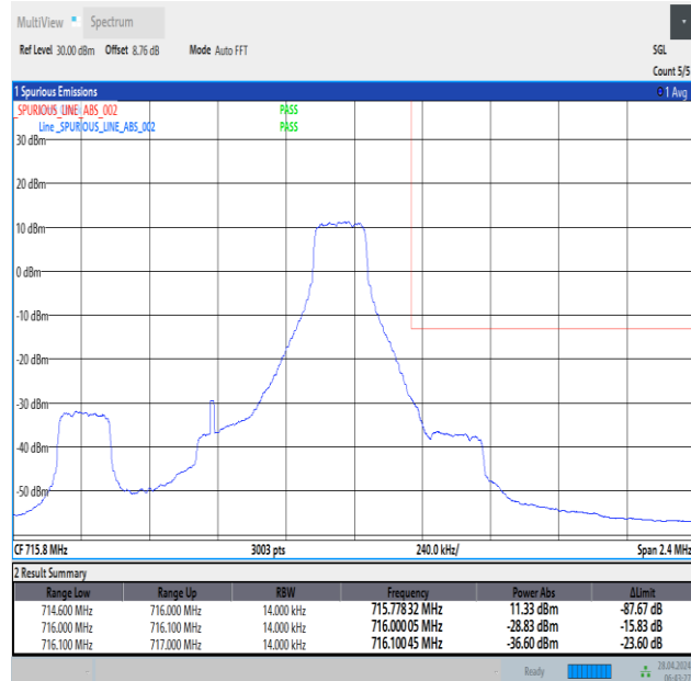
Band12_1.4MHz_QPSK_23173_1RB#5
