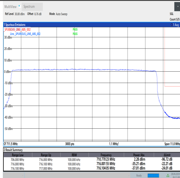
Band12_10MHz_QPSK_23130_50RB#0
