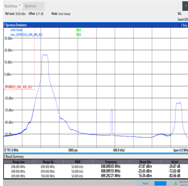
Band12_5MHz_QPSK_23035_1RB#0
