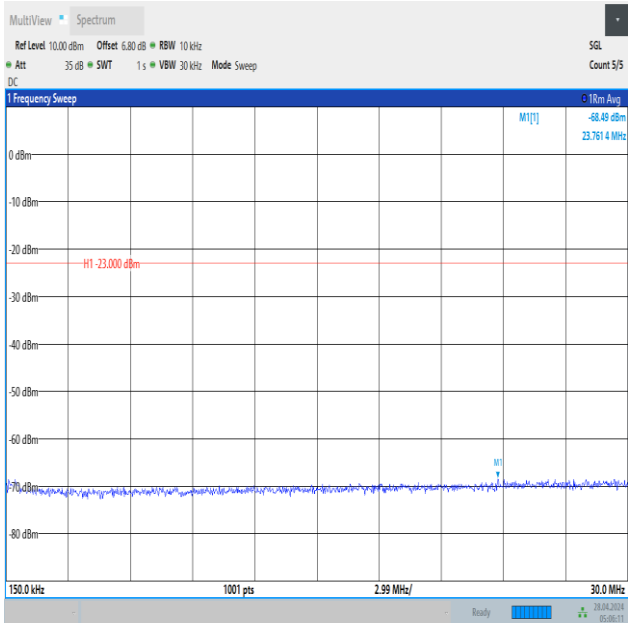
Band12_1.4MHz_16QAM_23017_1RB#0_0.15~30_0.15~30
