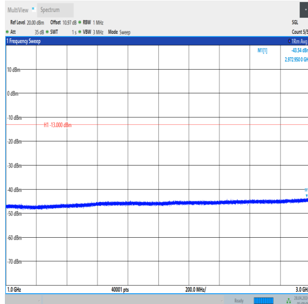
Band12_1.4MHz_16QAM_23017_1RB#5_1000~3000_1000~3000
