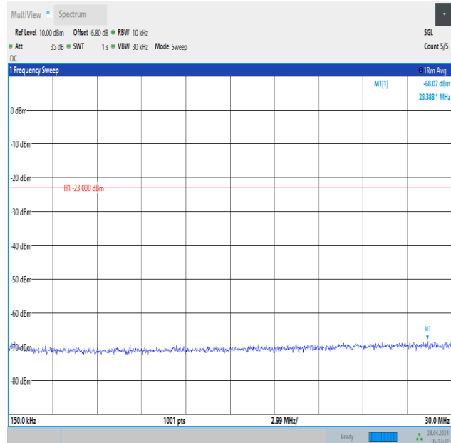
Band12_1.4MHz_16QAM_23095_1RB#5_0.15~30_0.15~30
