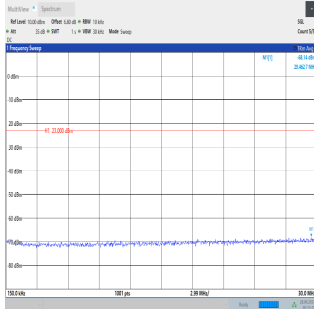
Band12_1.4MHz_QPSK_23095_6RB#0_0.15~30_0.15~30
