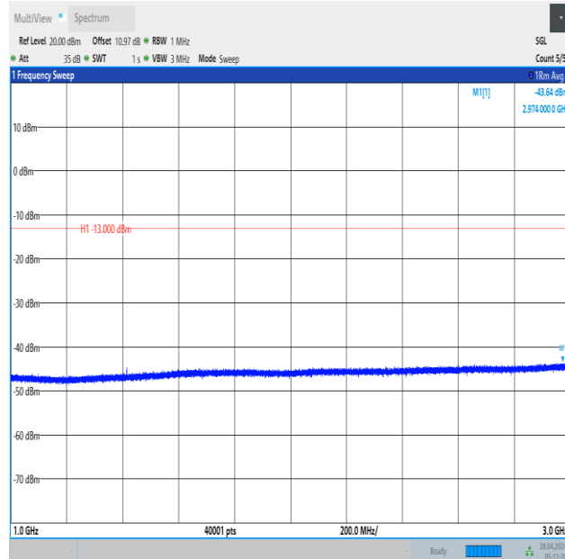
Band12_1.4MHz_16QAM_23095_1RB#0_1000~3000_1000~3000
