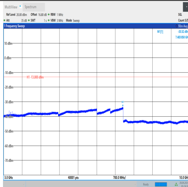
Band12_1.4MHz_16QAM_23095_6RB#0_3000~10000_3000~10000
