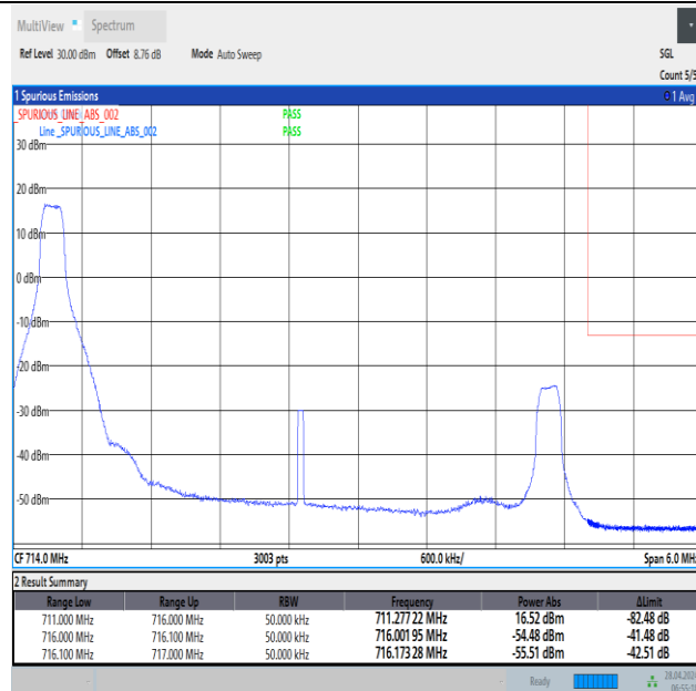
Band12_5MHz_QPSK_23155_1RB#0
