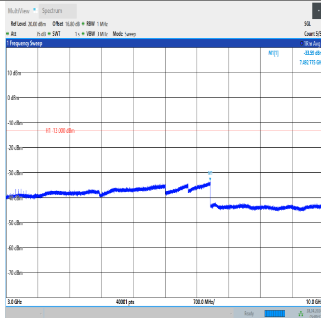
Band12_1.4MHz_16QAM_23017_6RB#0_3000~10000_3000~10000
