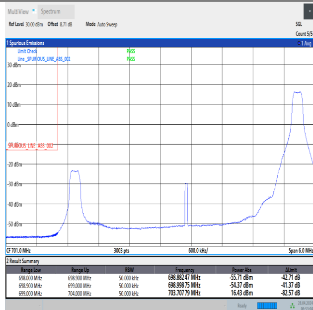
Band12_5MHz_QPSK_23035_1RB#24
