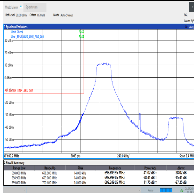
Band12_1.4MHz_QPSK_23017_1RB#0
