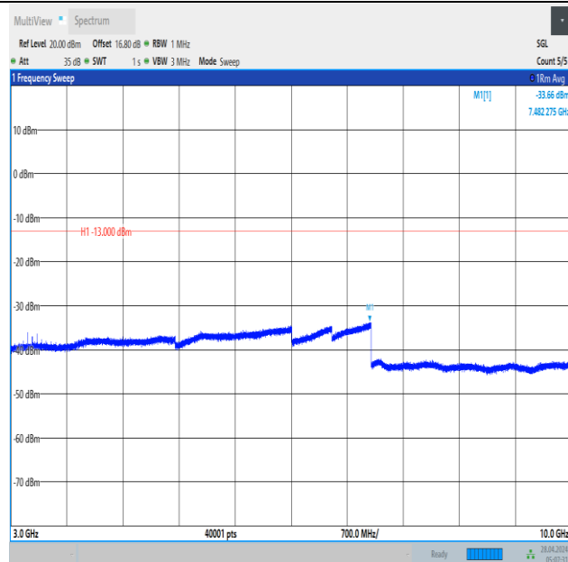
Band12_1.4MHz_QPSK_23017_1RB#5_3000~10000_3000~10000
