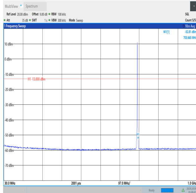
Band12_1.4MHz_QPSK_23017_6RB#0_30~1000_30~1000
