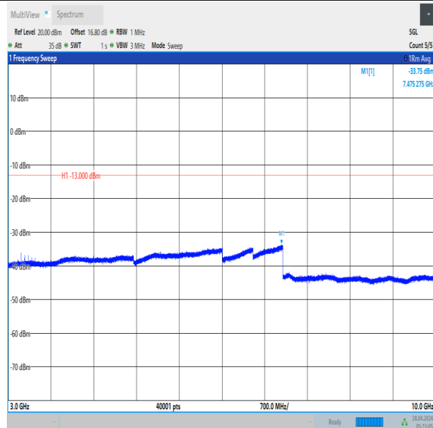
Band12_1.4MHz_16QAM_23095_1RB#5_3000~10000_3000~10000
