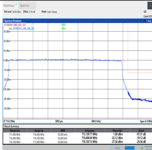
Band12_5MHz_16QAM_23155_25RB#0
