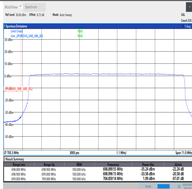
Band12_10MHz_QPSK_23060_50RB#0
