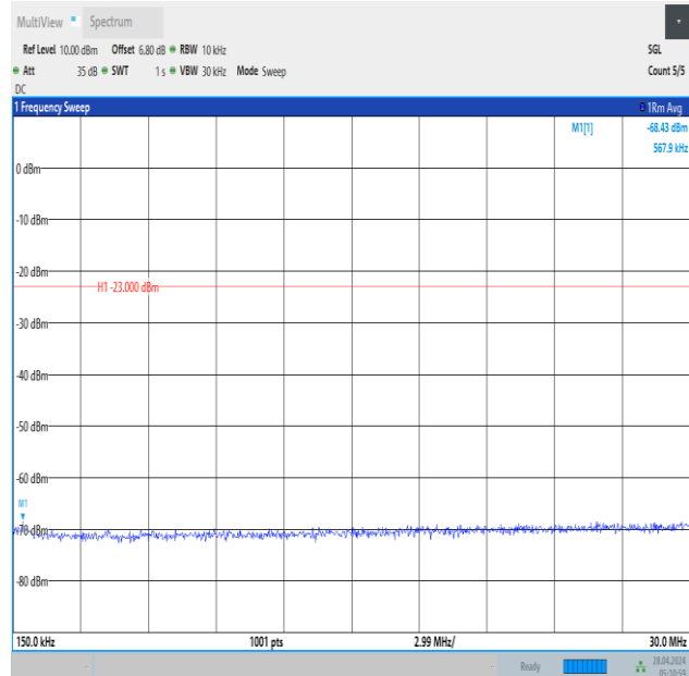
Band12_1.4MHz_16QAM_23095_1RB#0_0.15~30_0.15~30
