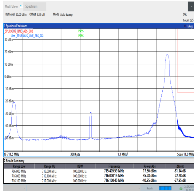
Band12_10MHz_16QAM_23130_1RB#49
