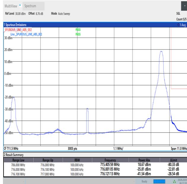
Band12_10MHz_QPSK_23130_1RB#49
