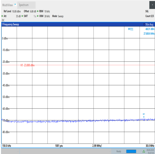
Band12_1.4MHz_16QAM_23017_1RB#5_0.15~30_0.15~30
