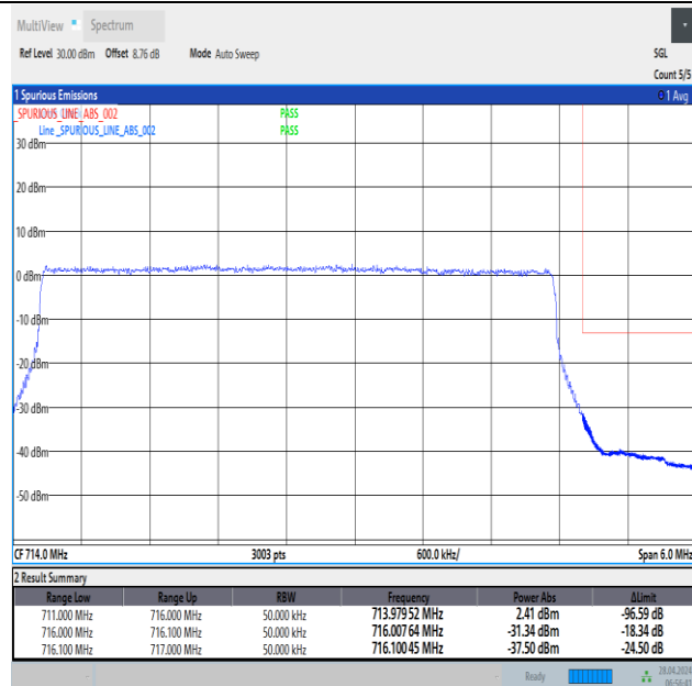
Band12_5MHz_QPSK_23155_25RB#0
