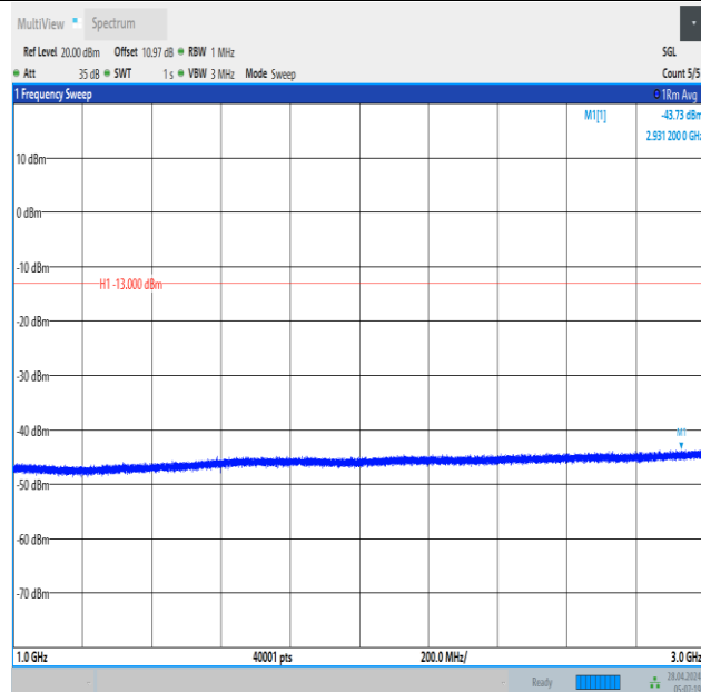
Band12_1.4MHz_QPSK_23017_1RB#5_1000~3000_1000~3000
