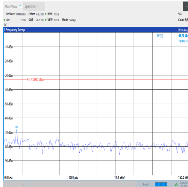
Band12_1.4MHz_16QAM_23095_1RB#0_0.009~0.15_0.009~0.15
