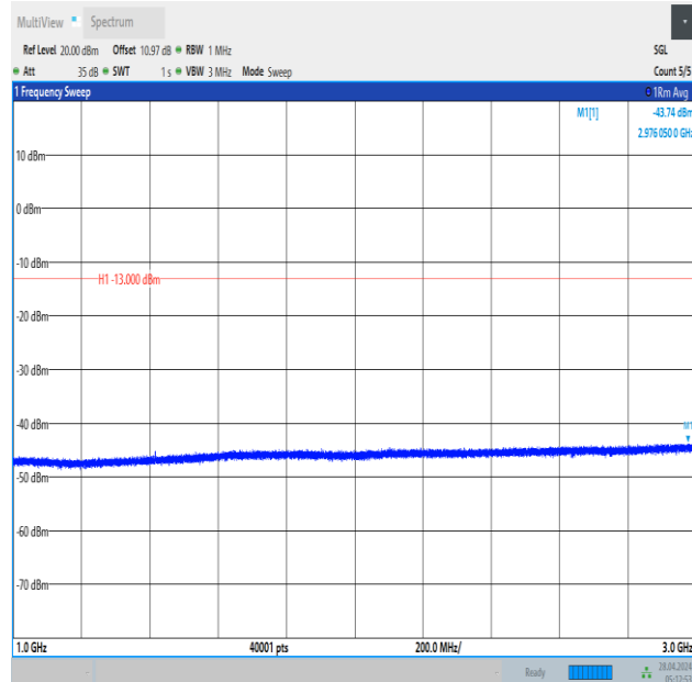
Band12_1.4MHz_16QAM_23095_1RB#5_1000~3000_1000~3000
