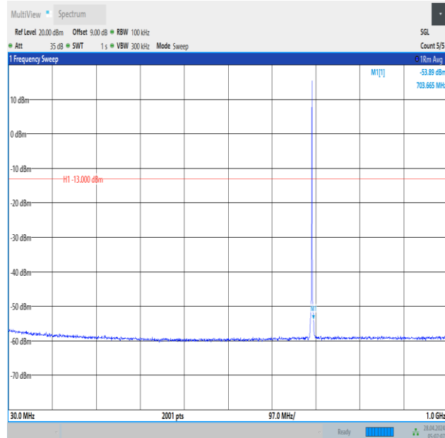
Band12_1.4MHz_QPSK_23017_1RB#5_30~1000_30~1000
