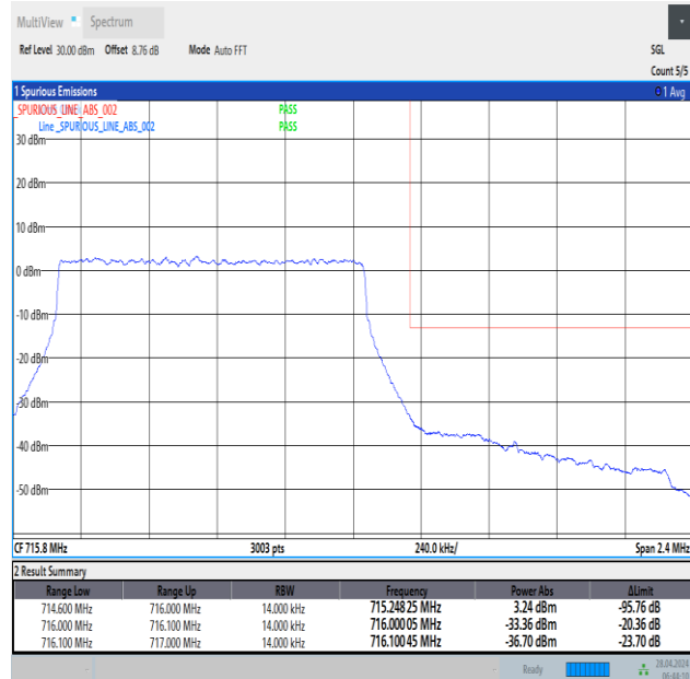
Band12_1.4MHz_QPSK_23173_6RB#0
