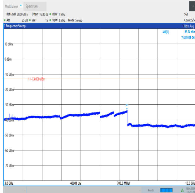
Band12_1.4MHz_QPSK_23095_1RB#5_3000~10000_3000~10000
