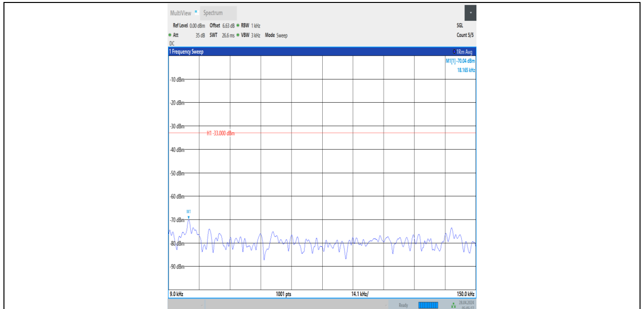
Band12_1.4MHz_QPSK_23017_1RB#0_0.009~0.15_0.009~0.15
