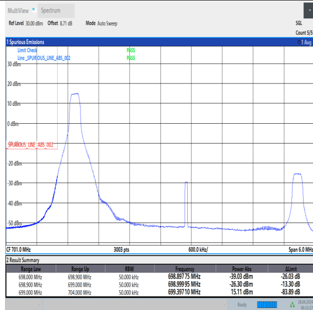
Band12_5MHz_16QAM_23035_1RB#0
