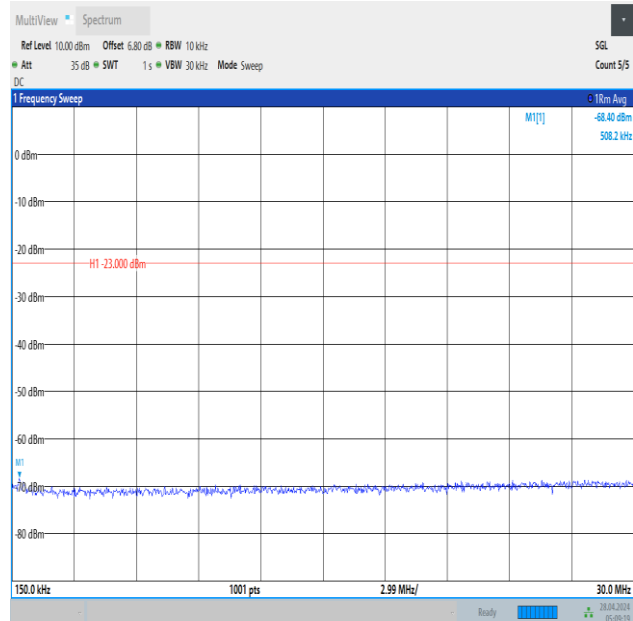
Band12_1.4MHz_16QAM_23017_6RB#0_0.15~30_0.15~30
