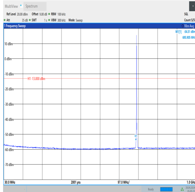
Band12_1.4MHz_QPSK_23017_1RB#0_30~1000_30~1000
