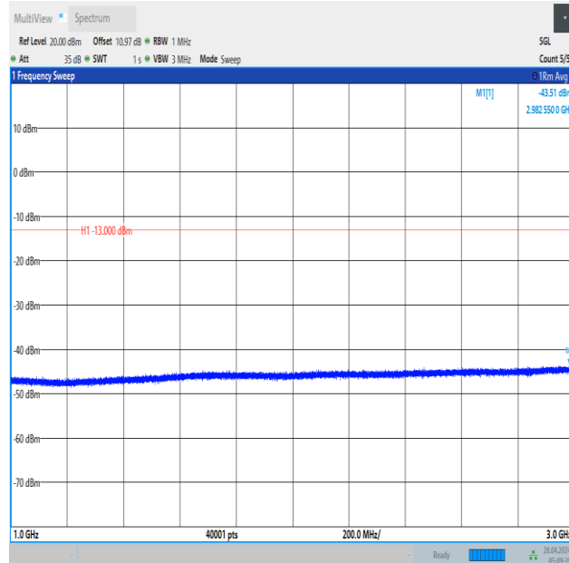
Band12_1.4MHz_16QAM_23017_6RB#0_1000~3000_1000~3000
