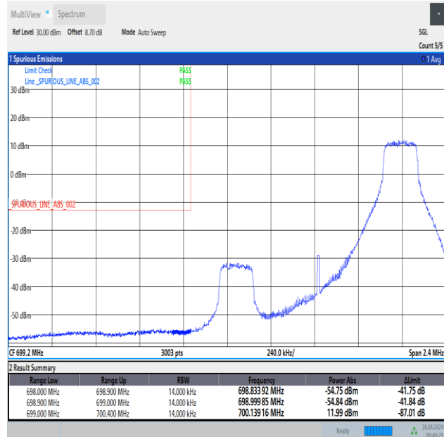
Band12_1.4MHz_QPSK_23017_1RB#5
