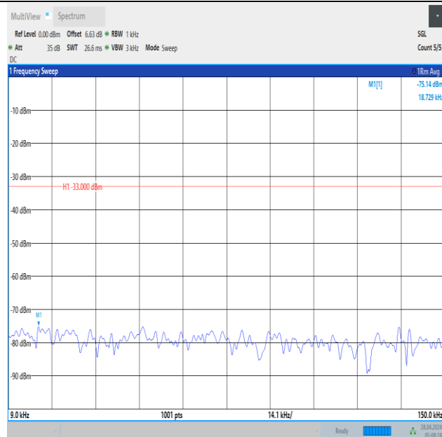
Band12_1.4MHz_QPSK_23017_6RB#0_0.009~0.15_0.009~0.15
