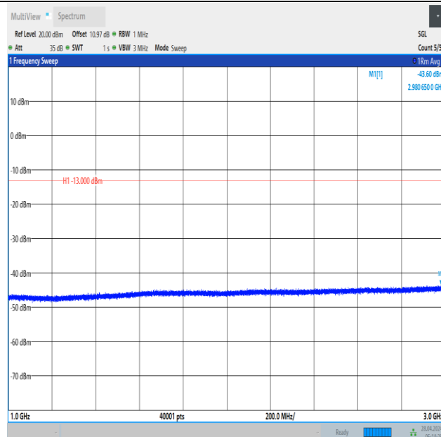
Band12_1.4MHz_16QAM_23095_6RB#0_1000~3000_1000~3000
