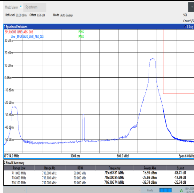
Band12_5MHz_16QAM_23155_1RB#24
