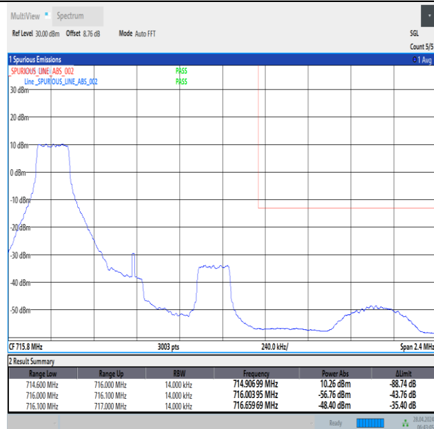
Band12_1.4MHz_16QAM_23173_1RB#0
