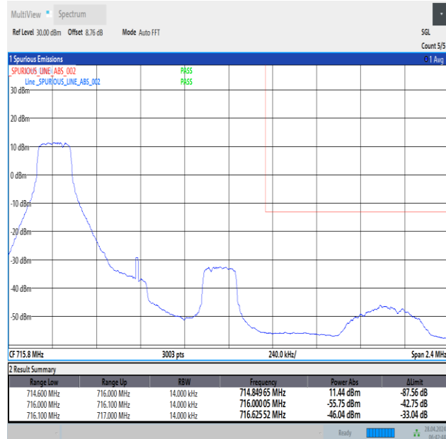
Band12_1.4MHz_QPSK_23173_1RB#0
