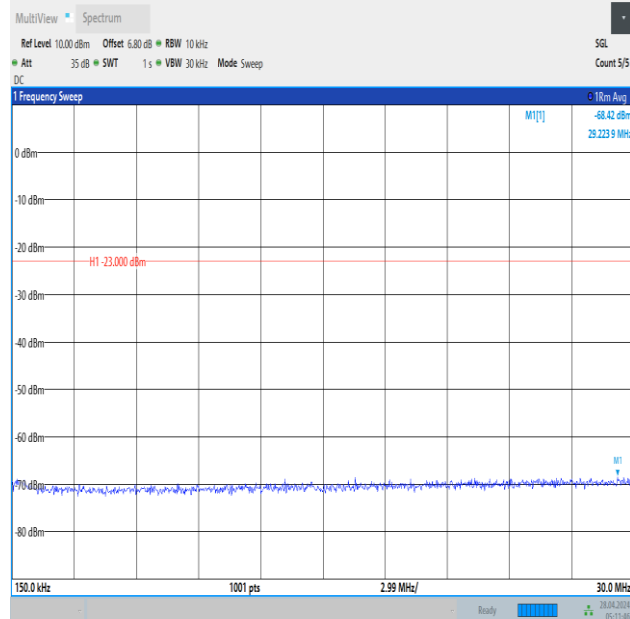
Band12_1.4MHz_QPSK_23095_1RB#5_0.15~30_0.15~30
