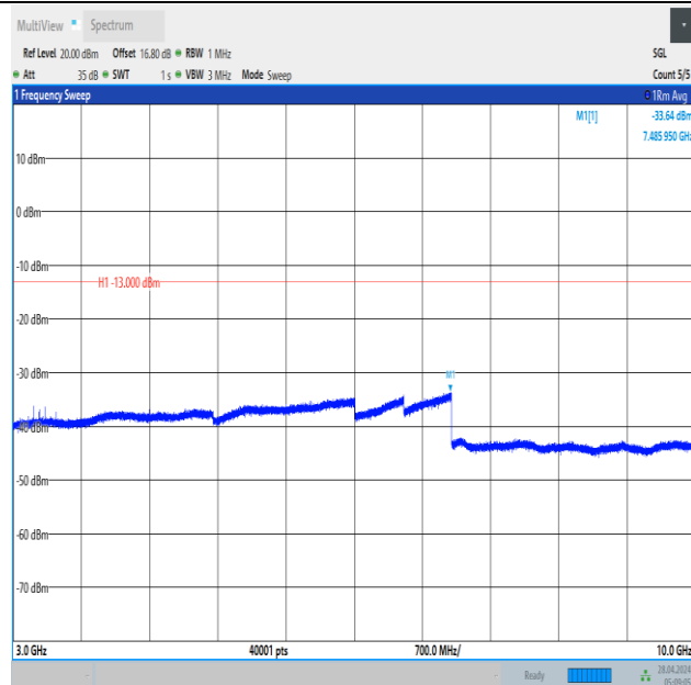
Band12_1.4MHz_QPSK_23017_6RB#0_3000~10000_3000~10000
