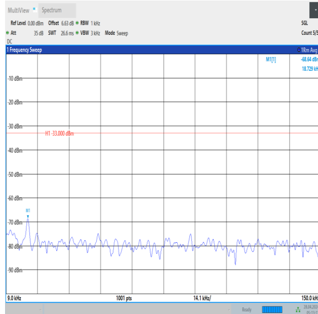
Band12_1.4MHz_QPSK_23095_6RB#0_0.009~0.15_0.009~0.15
