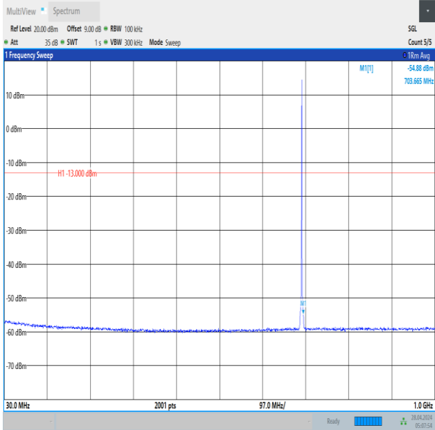
Band12_1.4MHz_16QAM_23017_1RB#5_30~1000_30~1000
