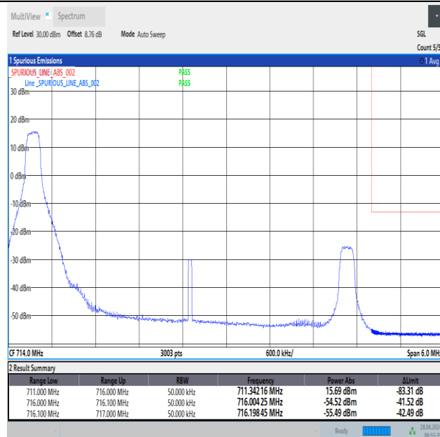
Band12_5MHz_16QAM_23155_1RB#0
