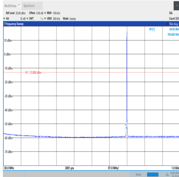
Band12_1.4MHz_QPSK_23095_1RB#0_30~1000_30~1000
