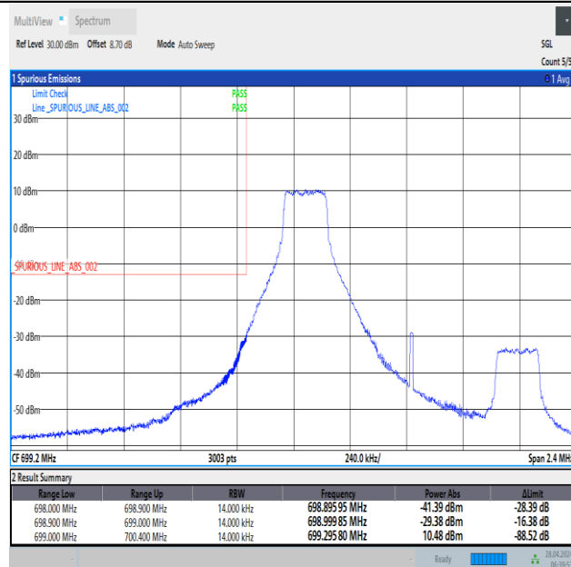
Band12_1.4MHz_16QAM_23017_1RB#0
