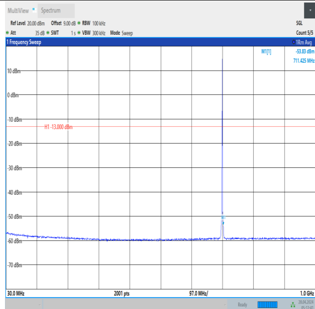
Band12_1.4MHz_16QAM_23095_1RB#5_30~1000_30~1000
