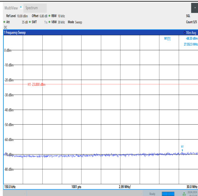
Band12_1.4MHz_16QAM_23173_1RB#5_0.15~30_0.15~30
