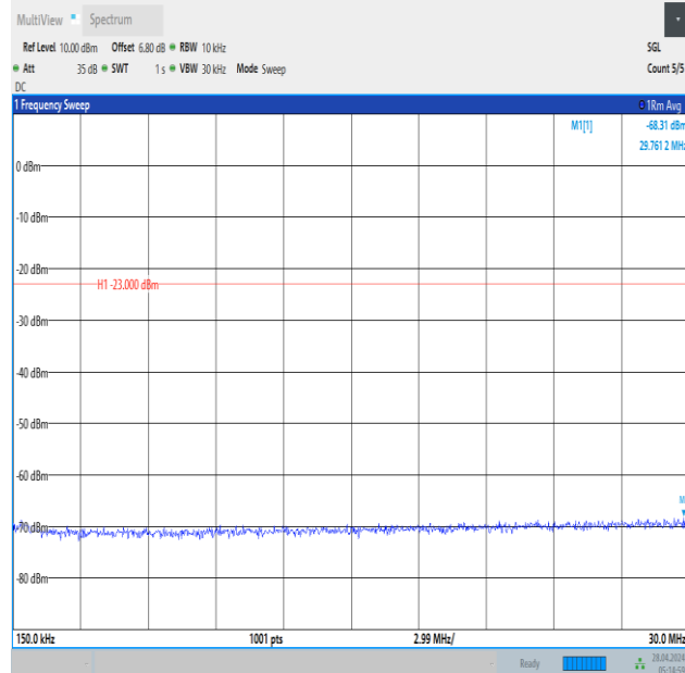
Band12_1.4MHz_QPSK_23173_1RB#0_0.15~30_0.15~30
