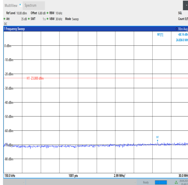
Band12_5MHz_QPSK_23095_25RB#0_0.15~30_0.15~30
