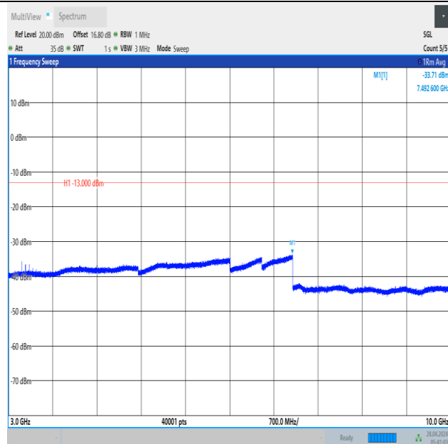
Band12_5MHz_QPSK_23095_25RB#0_3000~10000_3000~10000
