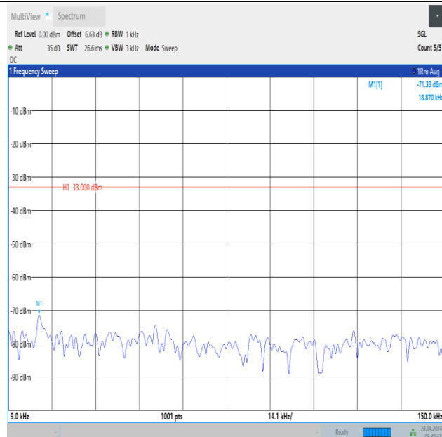
Band12_5MHz_QPSK_23155_1RB#0_0.009~0.15_0.009~0.15
