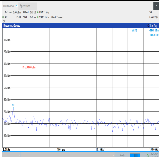
Band12_5MHz_QPSK_23035_1RB#0_0.009~0.15_0.009~0.15
