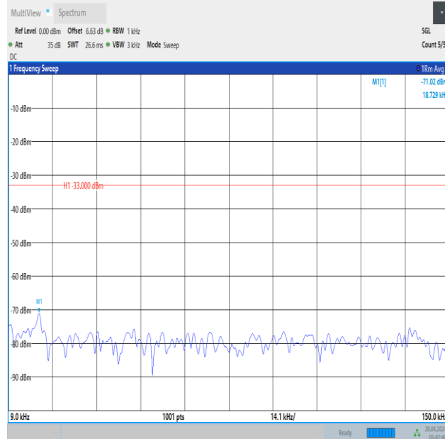
Band12_5MHz_16QAM_23155_1RB#0_0.009~0.15_0.009~0.15
