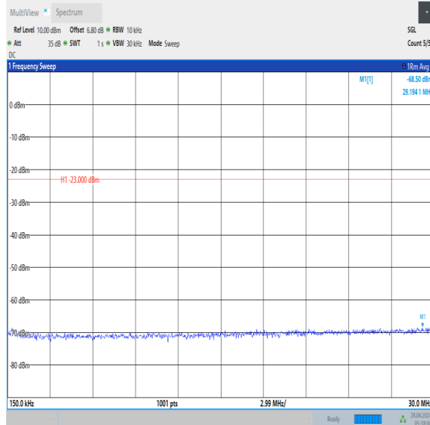
Band12_1.4MHz_QPSK_23173_6RB#0_0.15~30_0.15~30
