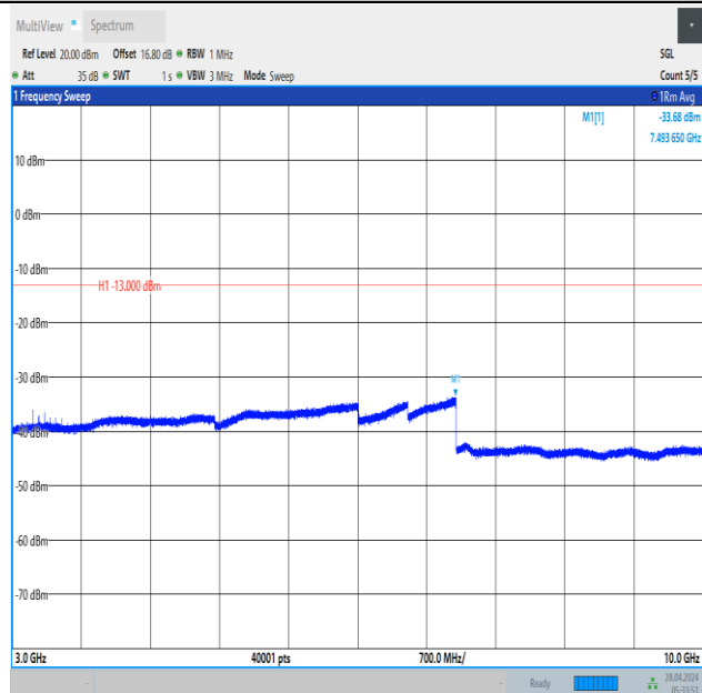
Band12_5MHz_16QAM_23035_1RB#0_3000~10000_3000~10000
