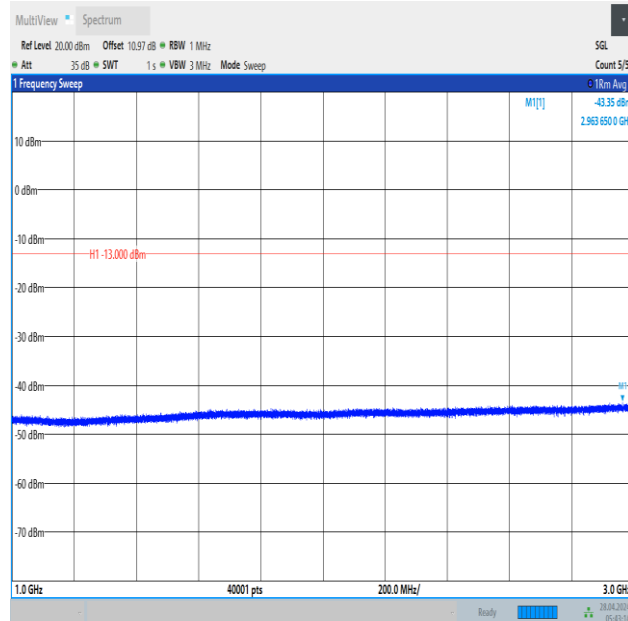
Band12_5MHz_16QAM_23155_1RB#0_1000~3000_1000~3000
