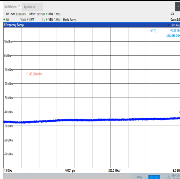
Band12_5MHz_16QAM_23035_25RB#0_1000~3000_1000~3000
