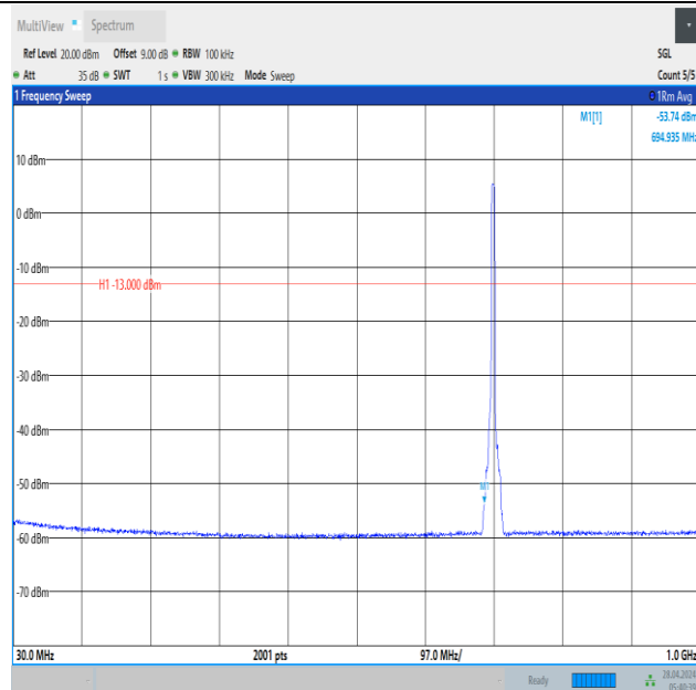
Band12_5MHz_QPSK_23095_25RB#0_30~1000_30~1000
