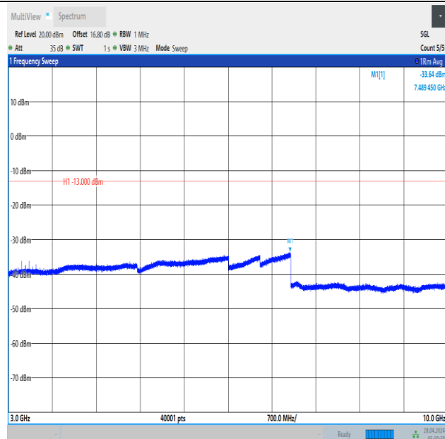
Band12_5MHz_QPSK_23095_1RB#24_3000~10000_3000~10000
