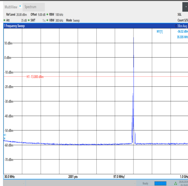
Band12_5MHz_QPSK_23095_1RB#24_30~1000_30~1000
