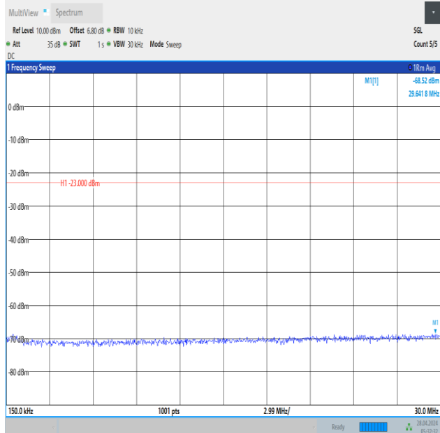
Band12_5MHz_QPSK_23035_1RB#0_0.15~30_0.15~30
