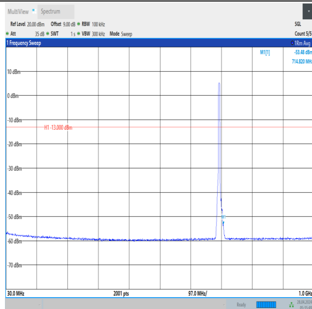
Band12_5MHz_QPSK_23035_25RB#0_30~1000_30~1000
