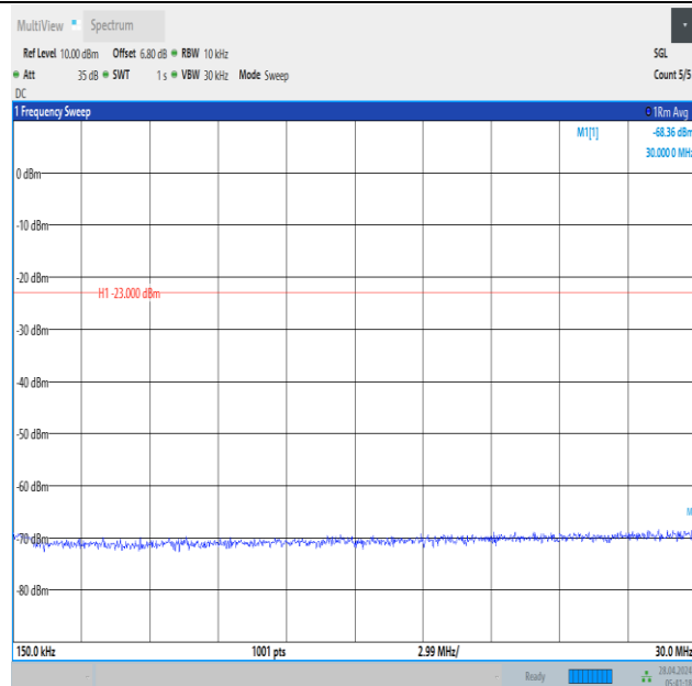
Band12_5MHz_16QAM_23095_25RB#0_0.15~30_0.15~30
