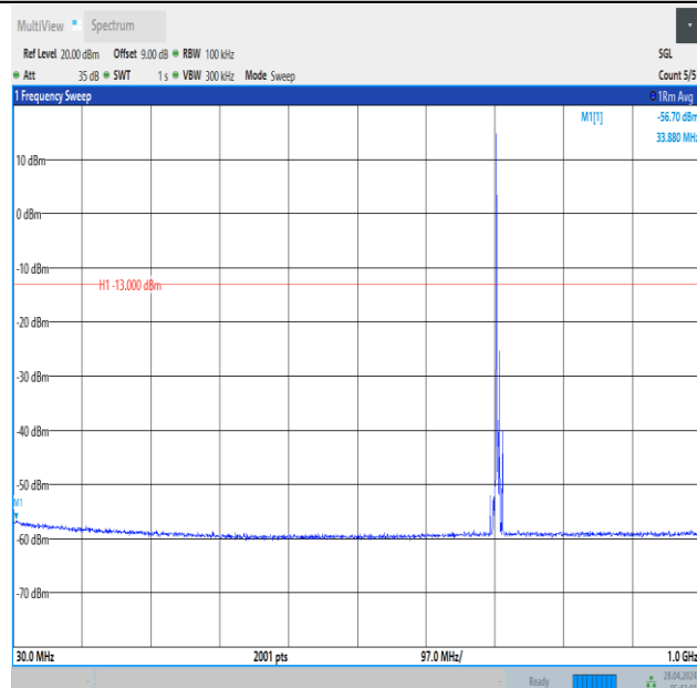
Band12_5MHz_16QAM_23155_1RB#0_30~1000_30~1000
