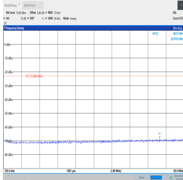
Band12_5MHz_QPSK_23155_1RB#0_0.15~30_0.15~30
