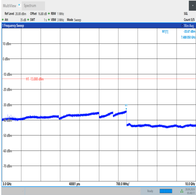
Band12_5MHz_16QAM_23095_1RB#24_3000~10000_3000~10000
