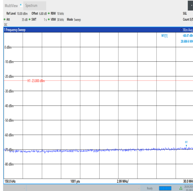
Band12_5MHz_QPSK_23095_1RB#24_0.15~30_0.15~30
