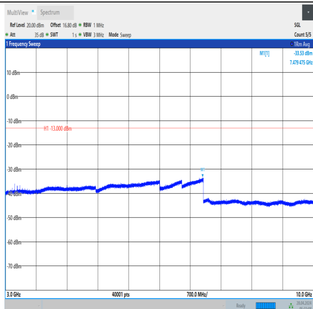
Band12_5MHz_QPSK_23035_1RB#0_3000~10000_3000~10000
