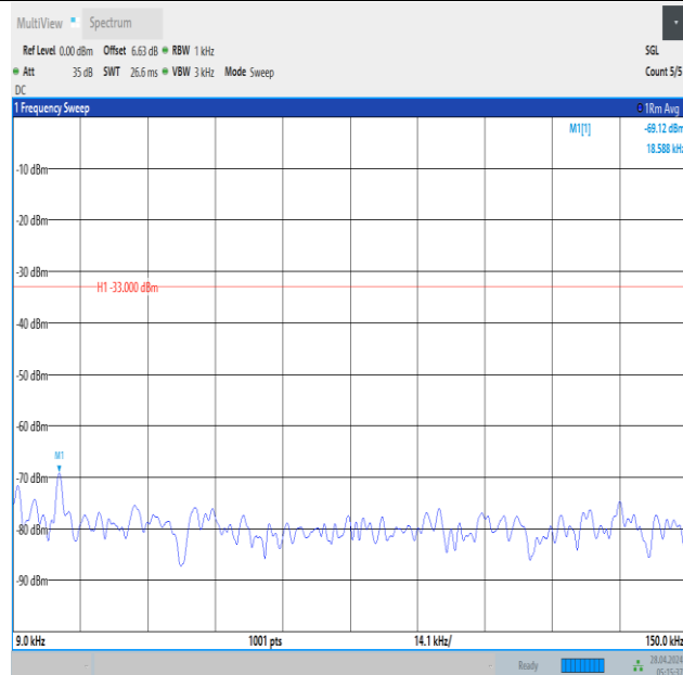
Band12_1.4MHz_16QAM_23173_1RB#0_0.009~0.15_0.009~0.15
