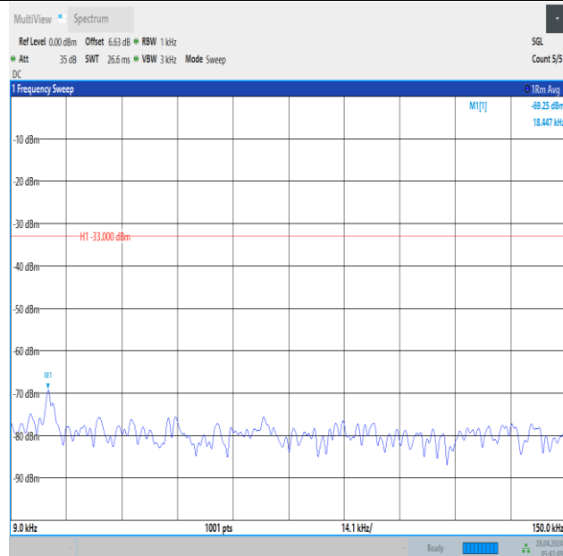
Band12_5MHz_16QAM_23095_25RB#0_0.009~0.15_0.009~0.15
