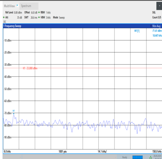
Band12_1.4MHz_QPSK_23173_1RB#5_0.009~0.15_0.009~0.15
