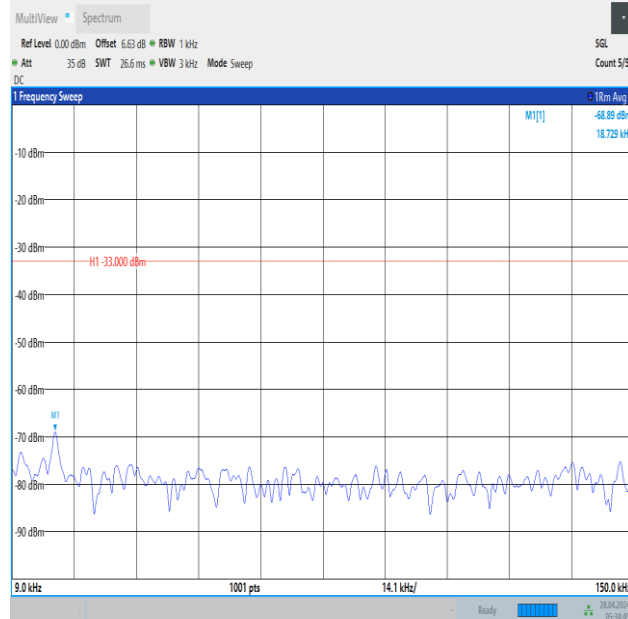
Band12_5MHz_16QAM_23035_1RB#24_0.009~0.15_0.009~0.15
