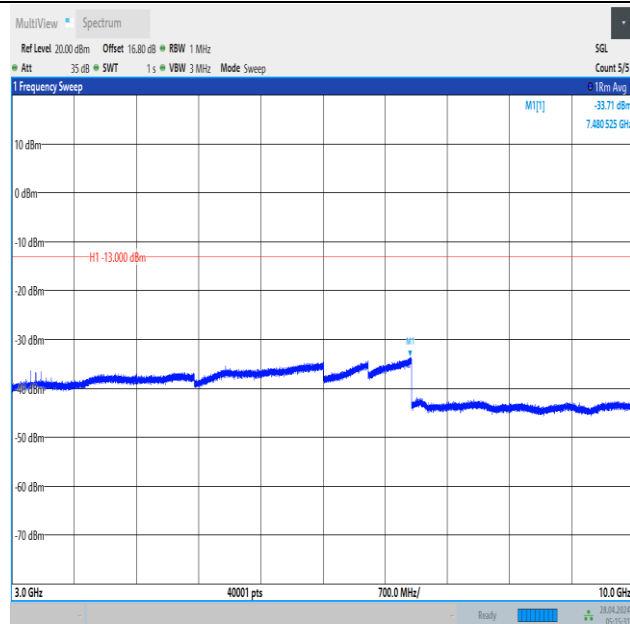
Band12_1.4MHz_QPSK_23173_1RB#0_3000~10000_3000~10000
