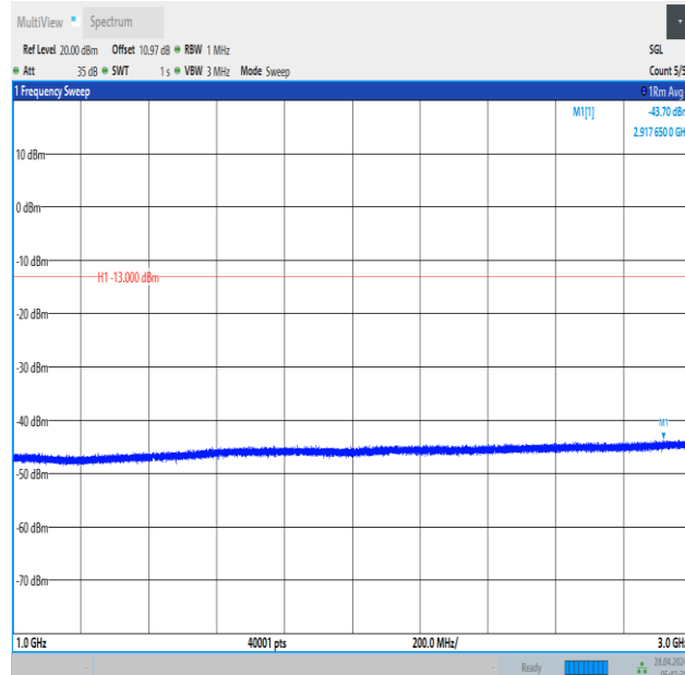
Band12_5MHz_16QAM_23095_25RB#0_1000~3000_1000~3000
