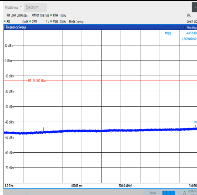
Band12_5MHz_16QAM_23035_1RB#24_1000~3000_1000~3000
