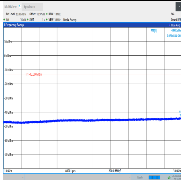
Band12_5MHz_QPSK_23095_1RB#24_1000~3000_1000~3000
