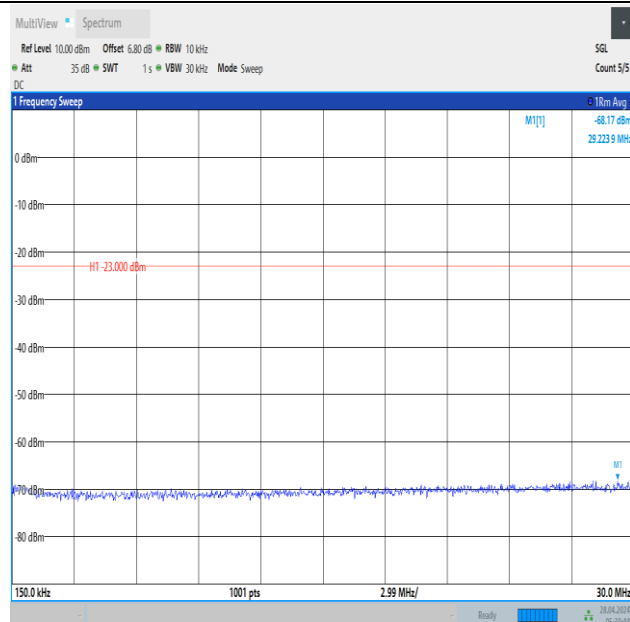
Band12_5MHz_16QAM_23095_1RB#24_0.15~30_0.15~30
