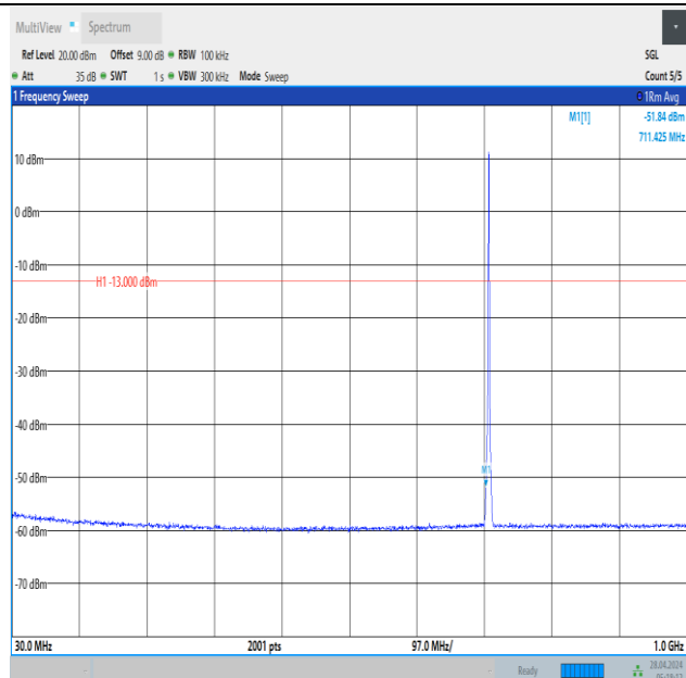
Band12_1.4MHz_QPSK_23173_6RB#0_30~1000_30~1000
