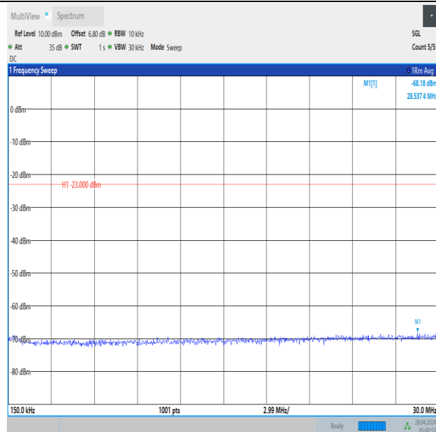
Band12_5MHz_16QAM_23155_1RB#0_0.15~30_0.15~30
