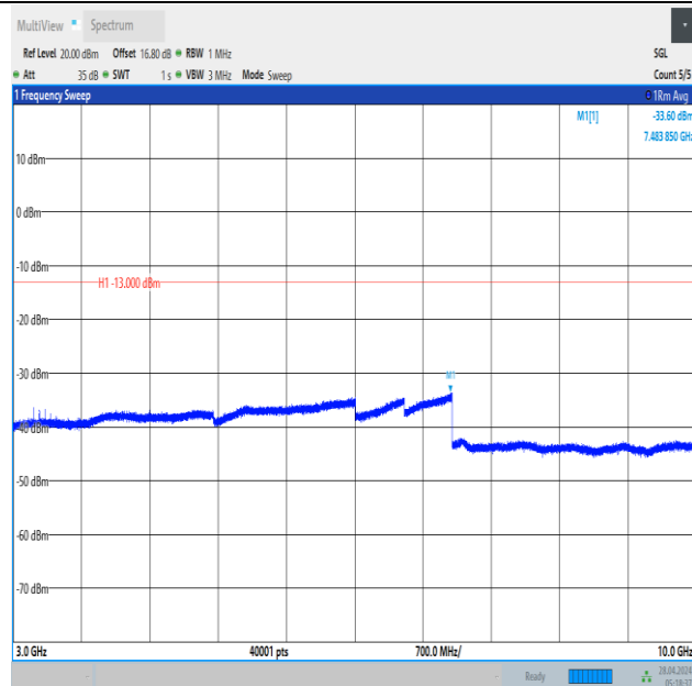
Band12_1.4MHz_QPSK_23173_6RB#0_3000~10000_3000~10000
