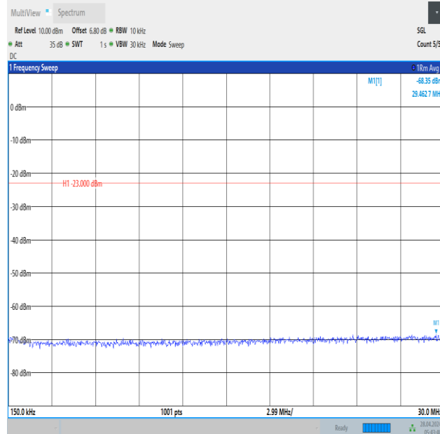
Band12_5MHz_QPSK_23155_1RB#24_0.15~30_0.15~30
