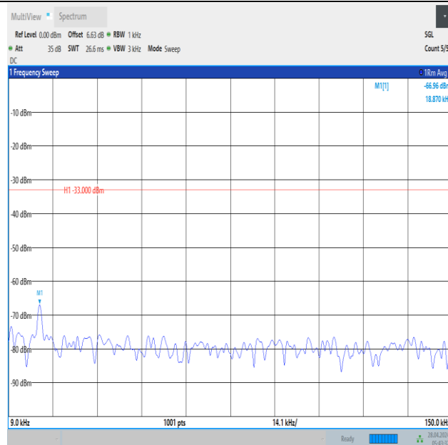
Band12_5MHz_QPSK_23155_1RB#24_0.009~0.15_0.009~0.15
