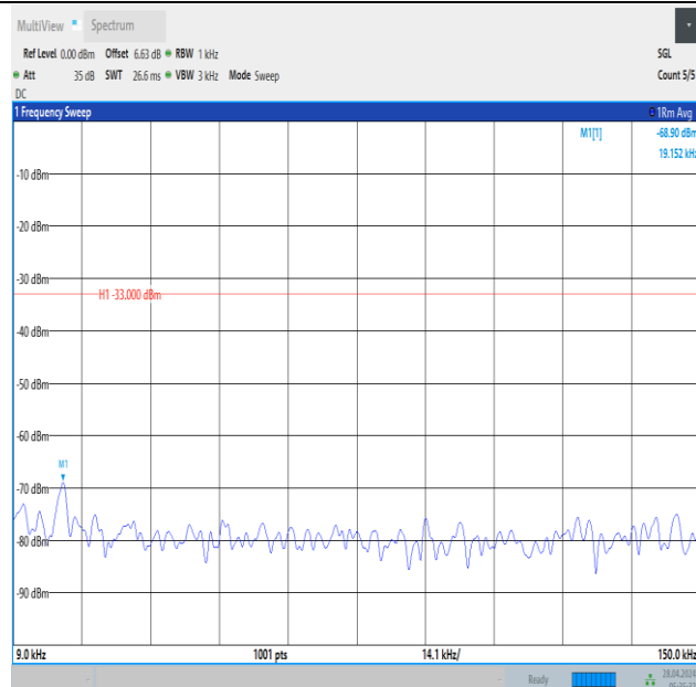
Band12_5MHz_QPSK_23035_25RB#0_0.009~0.15_0.009~0.15
