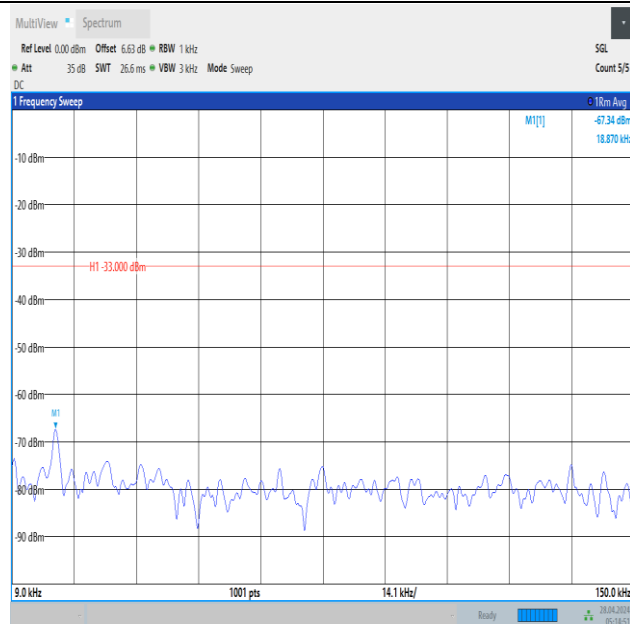
Band12_1.4MHz_QPSK_23173_1RB#0_0.009~0.15_0.009~0.15
