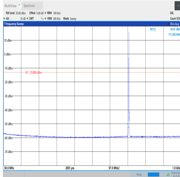
Band12_1.4MHz_QPSK_23173_1RB#0_30~1000_30~1000
