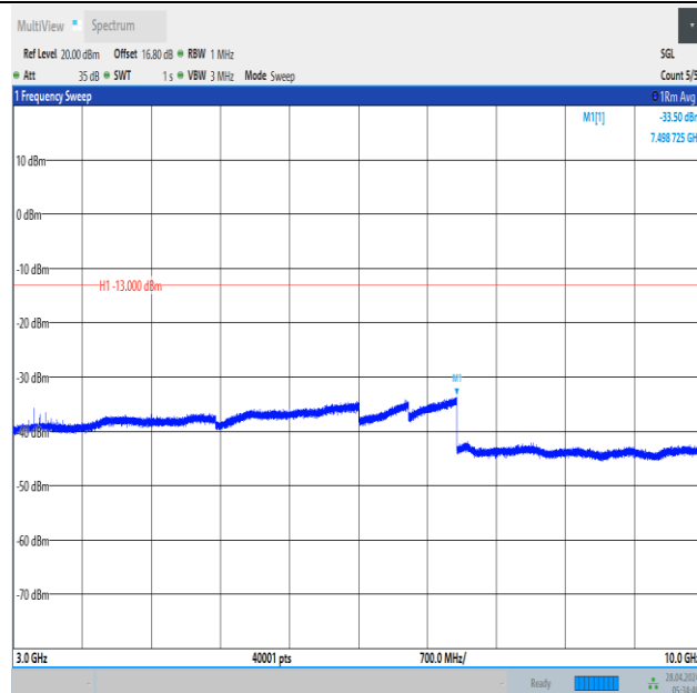
Band12_5MHz_QPSK_23035_1RB#24_3000~10000_3000~10000
