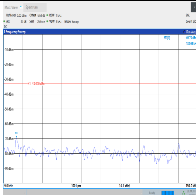
Band12_1.4MHz_QPSK_23173_6RB#0_0.009~0.15_0.009~0.15
