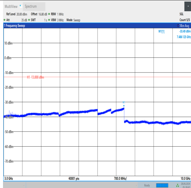
Band12_5MHz_16QAM_23095_1RB#0_3000~10000_3000~10000
