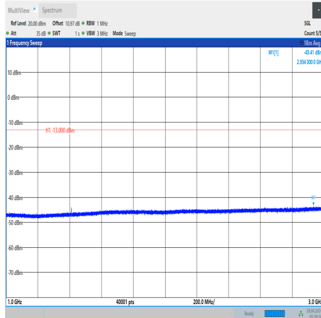
Band12_5MHz_16QAM_23095_1RB#0_1000~3000_1000~3000
