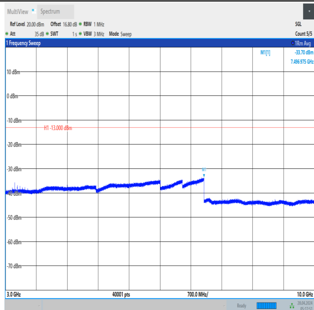
Band12_1.4MHz_16QAM_23173_1RB#5_3000~10000_3000~10000
