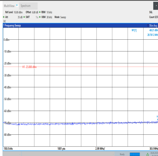
Band12_5MHz_16QAM_23095_1RB#0_0.15~30_0.15~30
