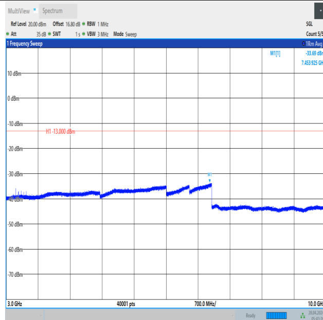
Band12_5MHz_16QAM_23155_1RB#0_3000~10000_3000~10000
