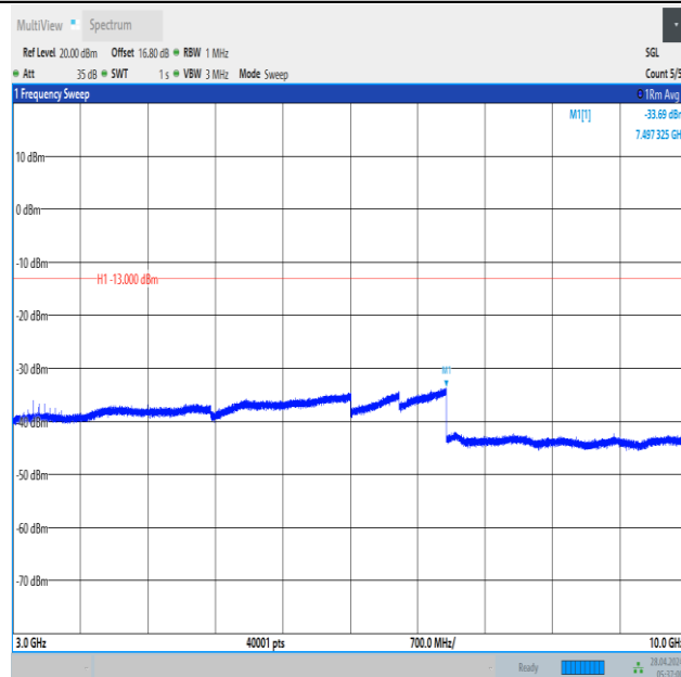
Band12_5MHz_16QAM_23035_25RB#0_3000~10000_3000~10000
