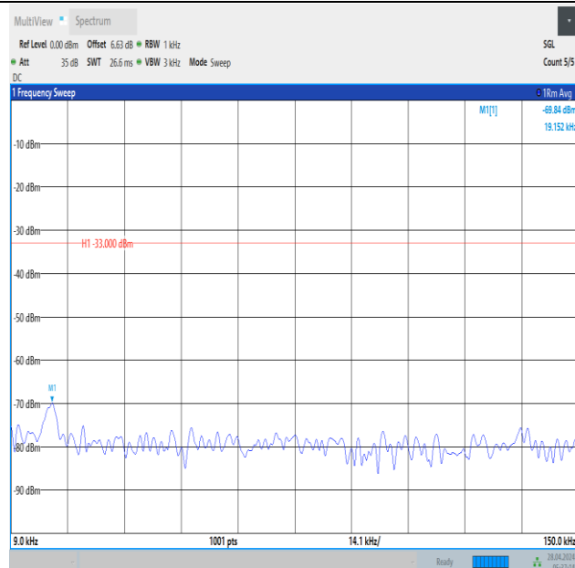
Band12_5MHz_QPSK_23095_1RB#0_0.009~0.15_0.009~0.15
