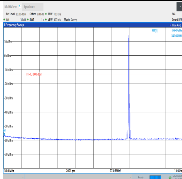
Band12_5MHz_16QAM_23095_1RB#0_30~1000_30~1000
