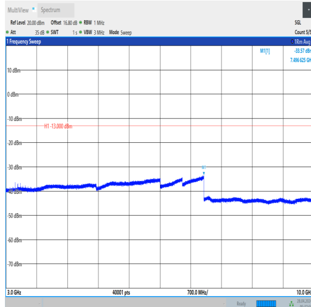
Band12_5MHz_QPSK_23095_1RB#0_3000~10000_3000~10000
