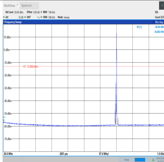
Band12_5MHz_16QAM_23095_1RB#24_30~1000_30~1000
