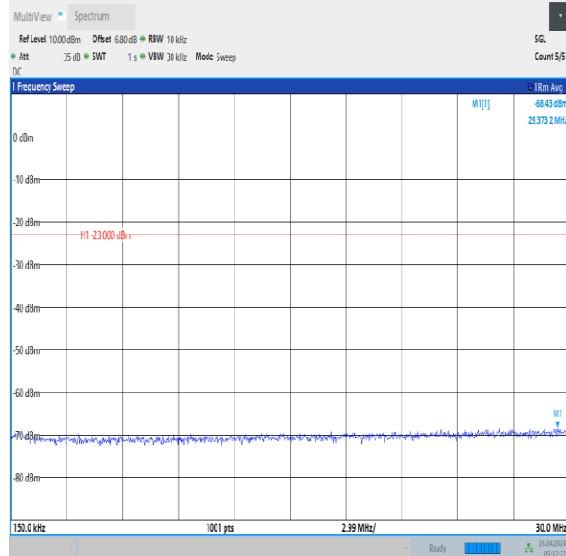
Band12_5MHz_QPSK_23095_1RB#0_0.15~30_0.15~30
