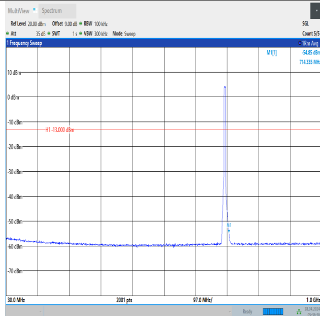
Band12_5MHz_16QAM_23035_25RB#0_30~1000_30~1000
