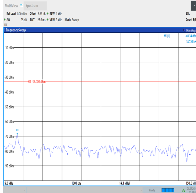
Band12_5MHz_16QAM_23095_1RB#0_0.009~0.15_0.009~0.15
