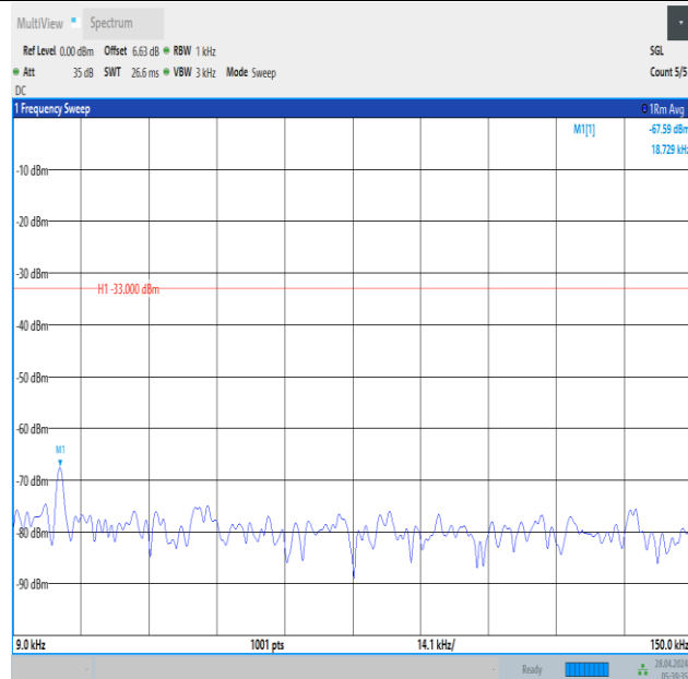
Band12_5MHz_16QAM_23095_1RB#24_0.009~0.15_0.009~0.15
