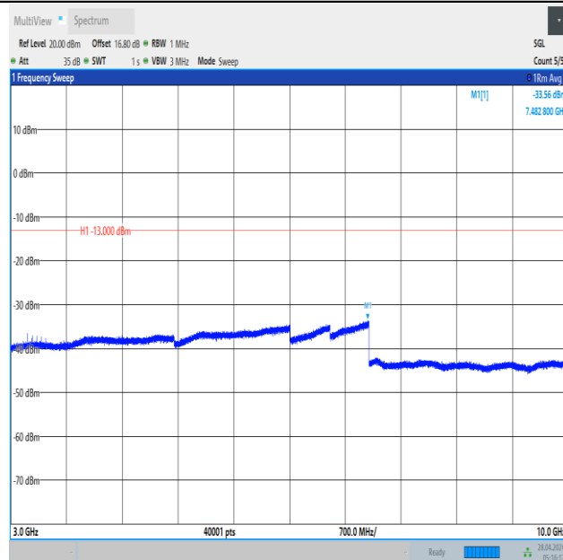
Band12_1.4MHz_16QAM_23173_1RB#0_3000~10000_3000~10000
