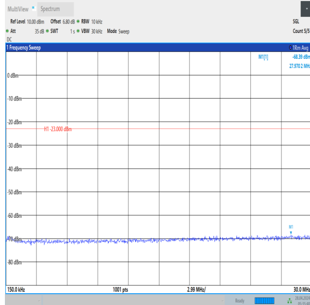
Band12_5MHz_QPSK_23035_25RB#0_0.15~30_0.15~30
