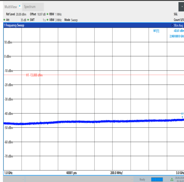
Band12_5MHz_QPSK_23035_25RB#0_1000~3000_1000~3000
