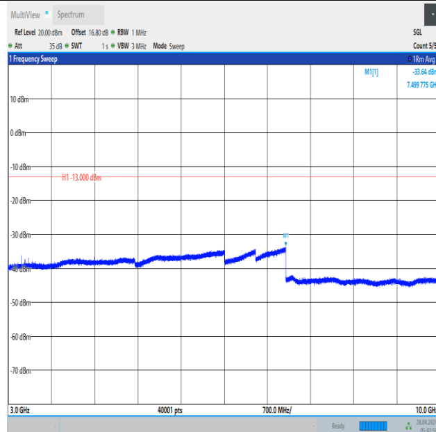
Band12_5MHz_16QAM_23095_25RB#0_3000~10000_3000~10000
