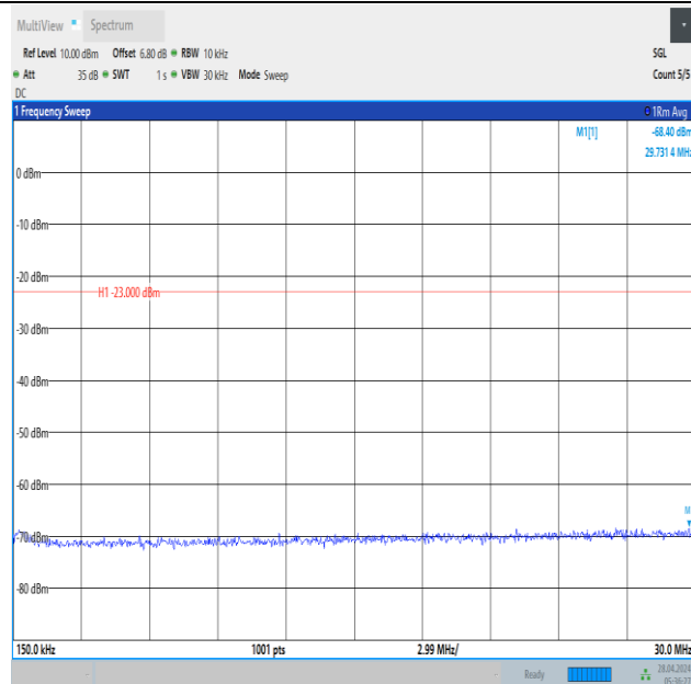
Band12_5MHz_16QAM_23035_25RB#0_0.15~30_0.15~30
