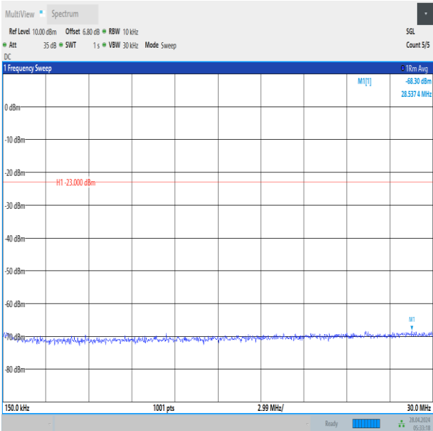
Band12_5MHz_16QAM_23035_1RB#0_0.15~30_0.15~30
