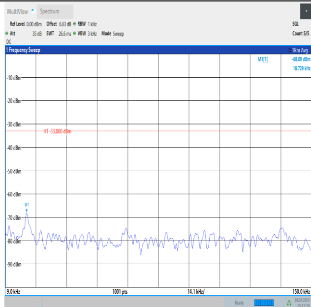
Band12_1.4MHz_16QAM_23173_1RB#5_0.009~0.15_0.009~0.15
