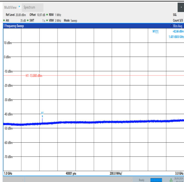
Band12_1.4MHz_16QAM_23173_1RB#5_1000~3000_1000~3000
