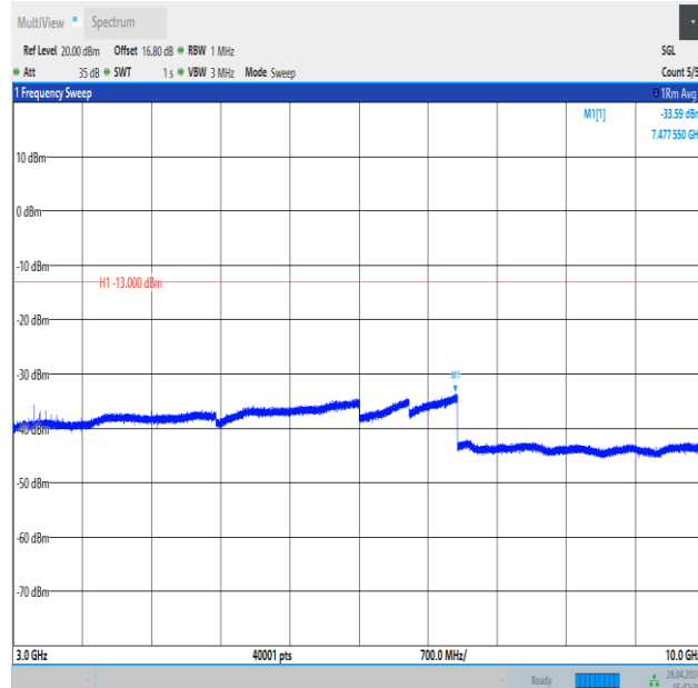
Band12_5MHz_QPSK_23155_1RB#0_3000~10000_3000~10000
