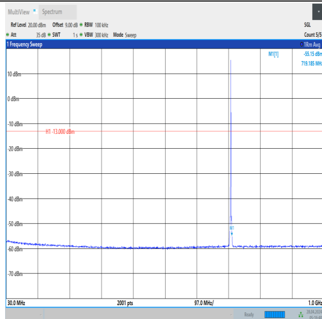
Band12_1.4MHz_QPSK_23173_1RB#5_30~1000_30~1000
