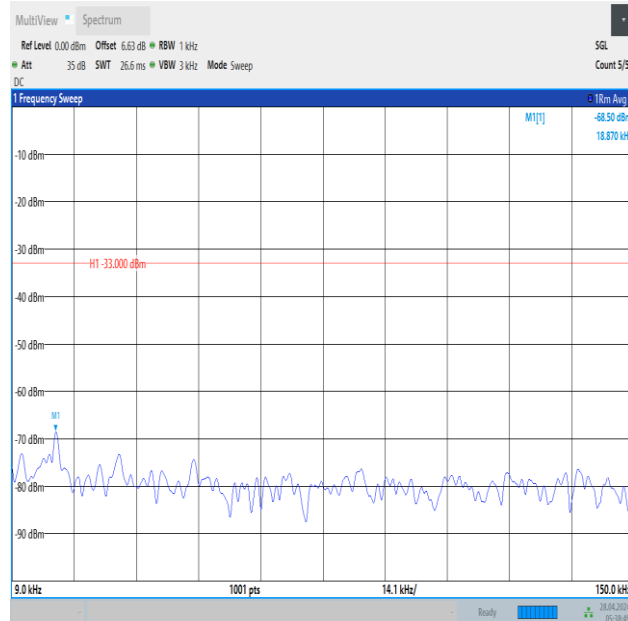
Band12_5MHz_QPSK_23095_1RB#24_0.009~0.15_0.009~0.15
