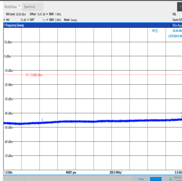
Band12_1.4MHz_16QAM_23173_1RB#0_1000~3000_1000~3000
