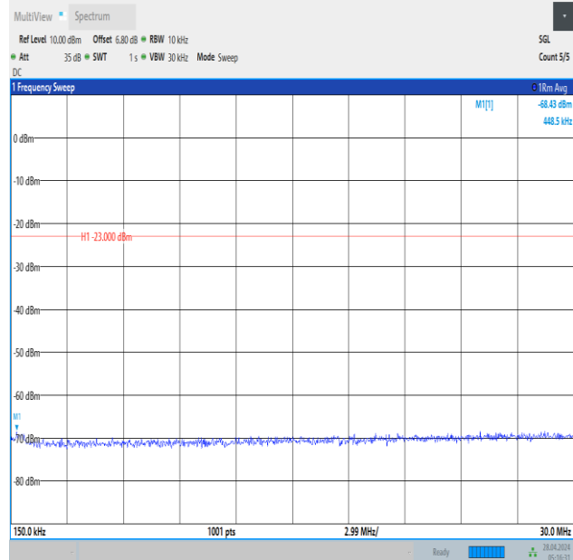
Band12_1.4MHz_QPSK_23173_1RB#5_0.15~30_0.15~30
