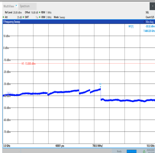
Band12_1.4MHz_QPSK_23173_1RB#5_3000~10000_3000~10000
