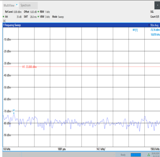
Band12_5MHz_16QAM_23035_1RB#0_0.009~0.15_0.009~0.15
