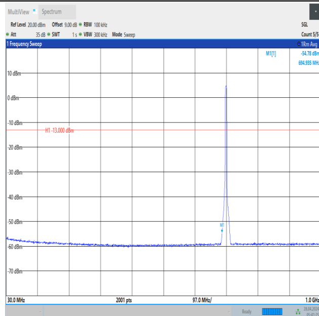
Band12_5MHz_16QAM_23095_25RB#0_30~1000_30~1000
