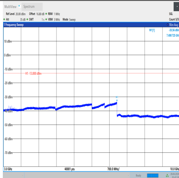
Band12_10MHz_QPSK_23060_1RB#0_3000~10000_3000~10000
