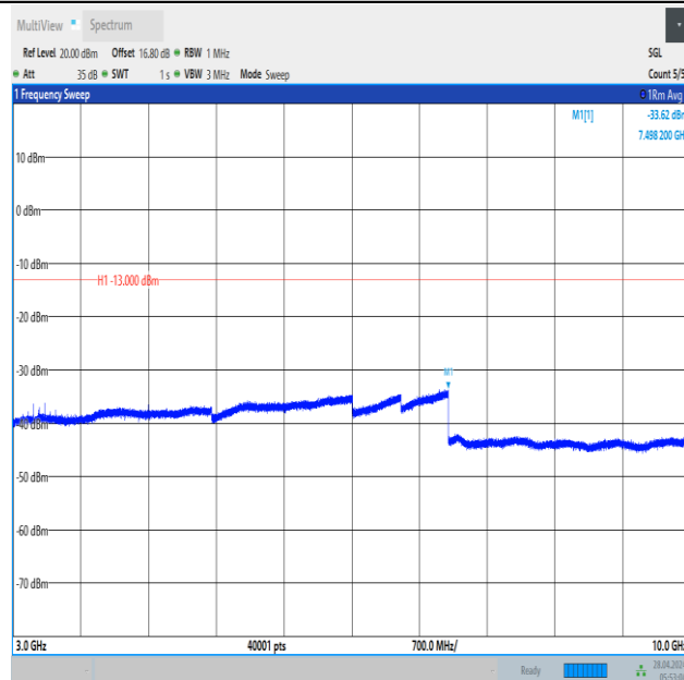
Band12_10MHz_16QAM_23095_1RB#49_3000~10000_3000~10000
