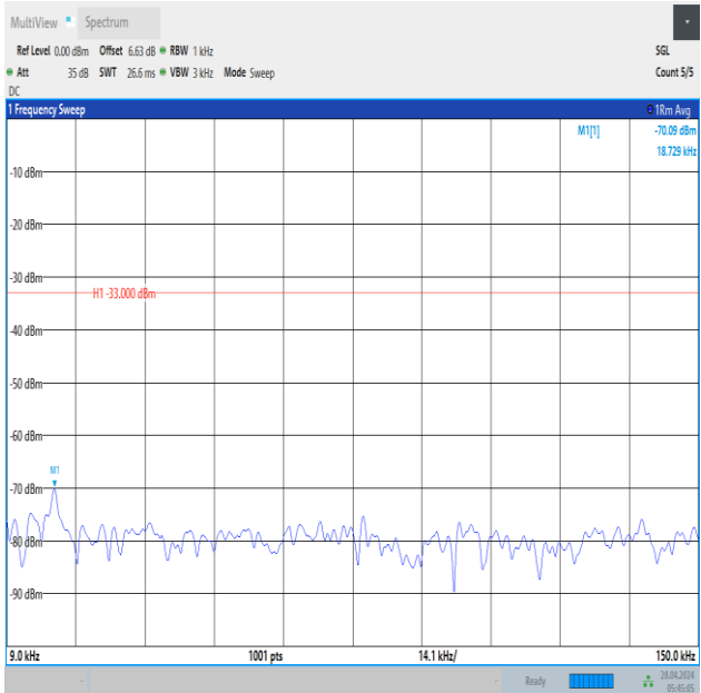
Band12_5MHz_QPSK_23155_25RB#0_0.009~0.15_0.009~0.15
