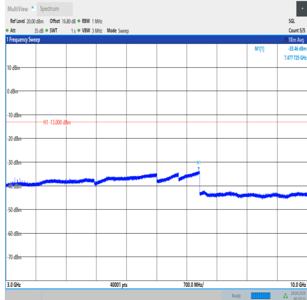
Band12_3MHz_QPSK_23025_1RB#0_3000~10000_3000~10000
