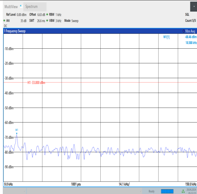
Band12_10MHz_16QAM_23095_1RB#49_0.009~0.15_0.009~0.15
