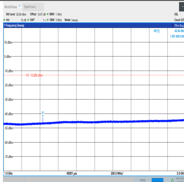
Band12_5MHz_16QAM_23155_1RB#24_1000~3000_1000~3000
