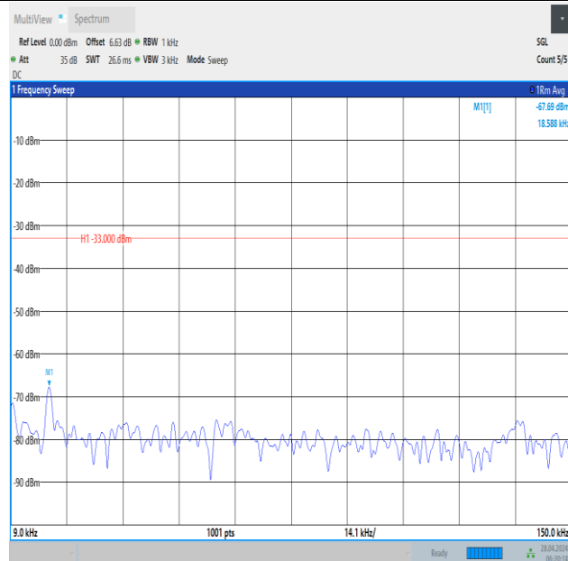
Band12_3MHz_QPSK_23025_1RB#0_0.009~0.15_0.009~0.15
