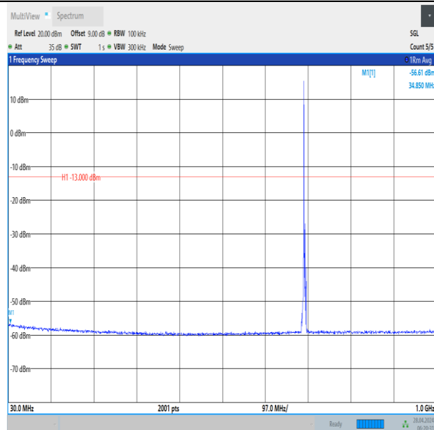
Band12_3MHz_QPSK_23025_1RB#0_30~1000_30~1000
