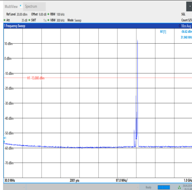
Band12_10MHz_16QAM_23130_1RB#49_30~1000_30~1000
