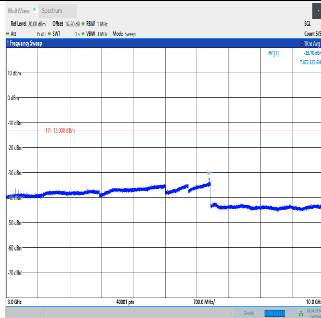
Band12_10MHz_16QAM_23060_1RB#49_3000~10000_3000~10000
