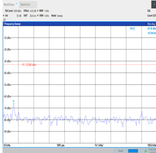
Band12_10MHz_16QAM_23060_1RB#0_0.009~0.15_0.009~0.15
