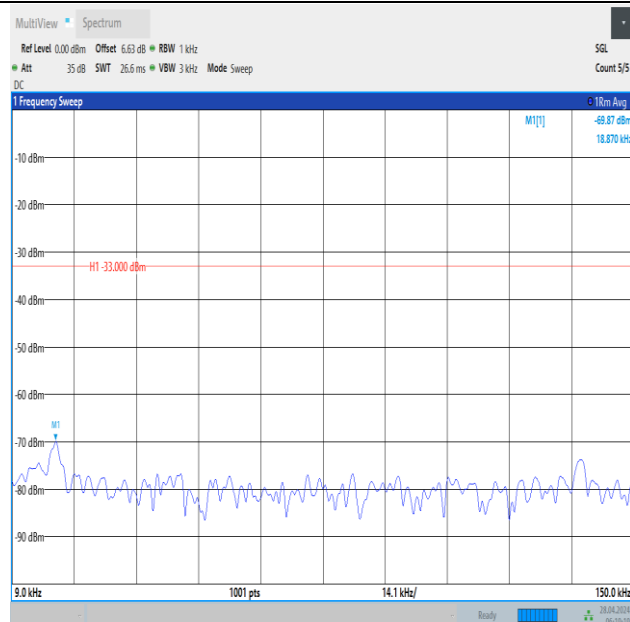
Band12_10MHz_QPSK_23130_50RB#0_0.009~0.15_0.009~0.15
