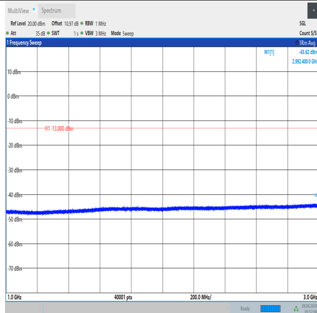
Band12_10MHz_QPSK_23095_1RB#49_1000~3000_1000~3000
