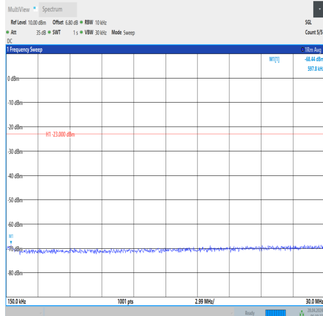
Band12_10MHz_QPSK_23130_50RB#0_0.15~30_0.15~30
