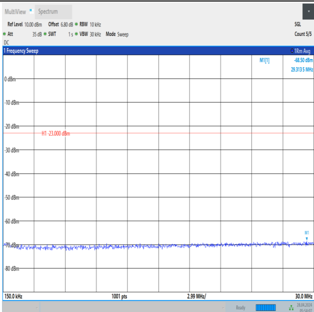
Band12_10MHz_16QAM_23130_1RB#0_0.15~30_0.15~30
