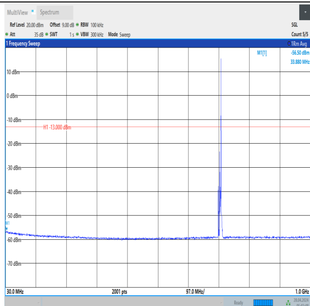
Band12_5MHz_QPSK_23155_1RB#24_30~1000_30~1000
