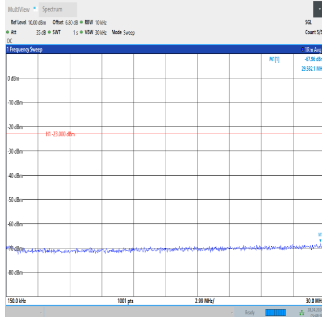
Band12_10MHz_QPSK_23060_1RB#49_0.15~30_0.15~30
