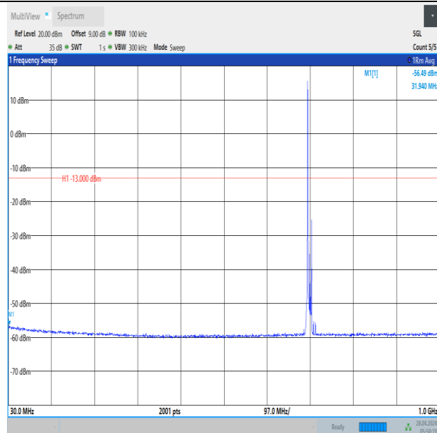
Band12_10MHz_QPSK_23095_1RB#0_30~1000_30~1000
