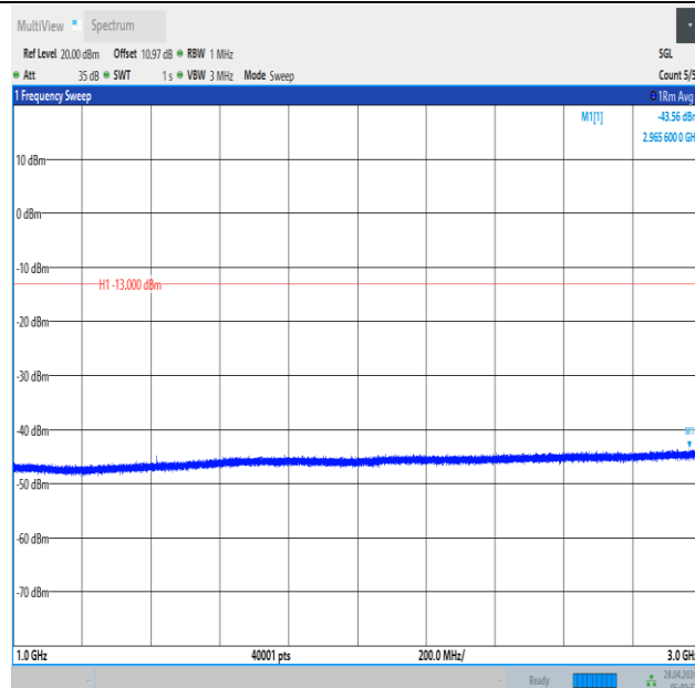
Band12_10MHz_16QAM_23060_1RB#49_1000~3000_1000~3000
