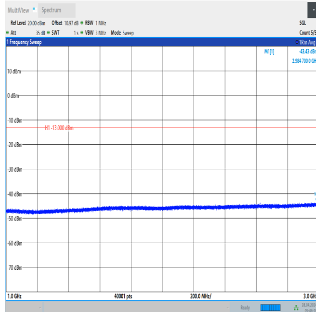
Band12_5MHz_16QAM_23155_25RB#0_1000~3000_1000~3000
