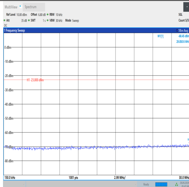
Band12_10MHz_16QAM_23060_1RB#0_0.15~30_0.15~30
