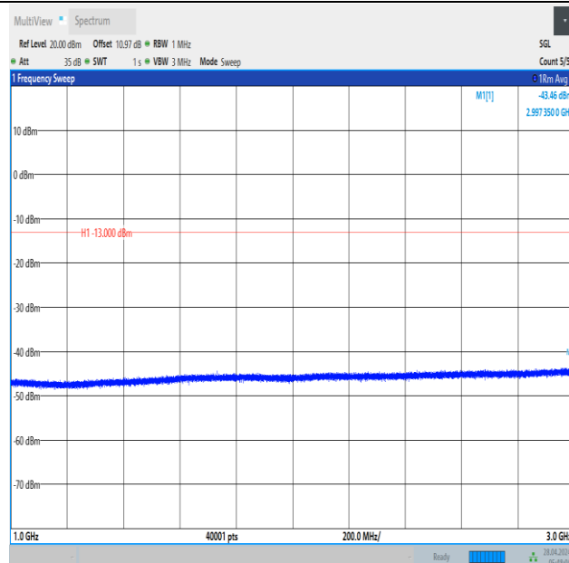
Band12_10MHz_16QAM_23060_1RB#0_1000~3000_1000~3000
