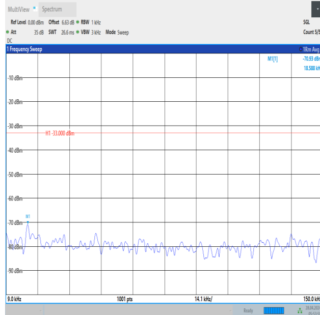
Band12_10MHz_16QAM_23130_1RB#0_0.009~0.15_0.009~0.15
