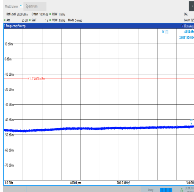
Band12_3MHz_QPSK_23025_1RB#0_1000~3000_1000~3000
