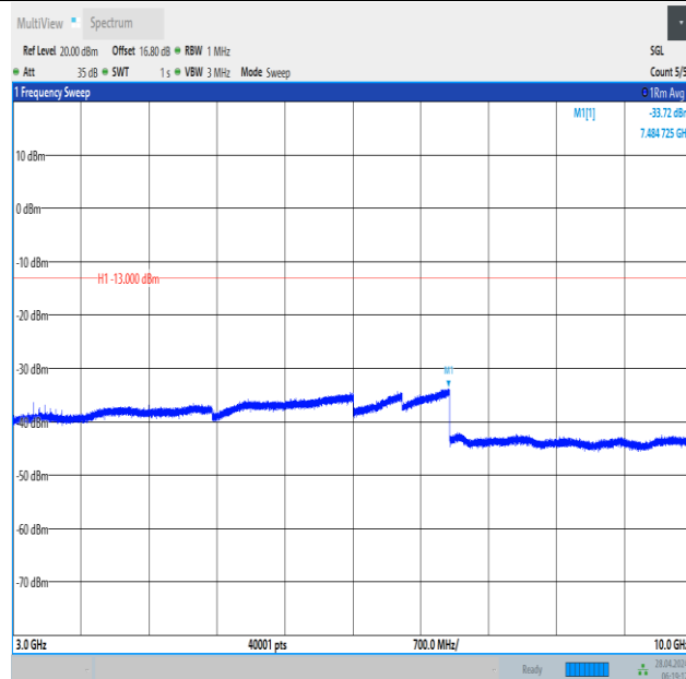
Band12_10MHz_QPSK_23095_50RB#0_3000~10000_3000~10000
