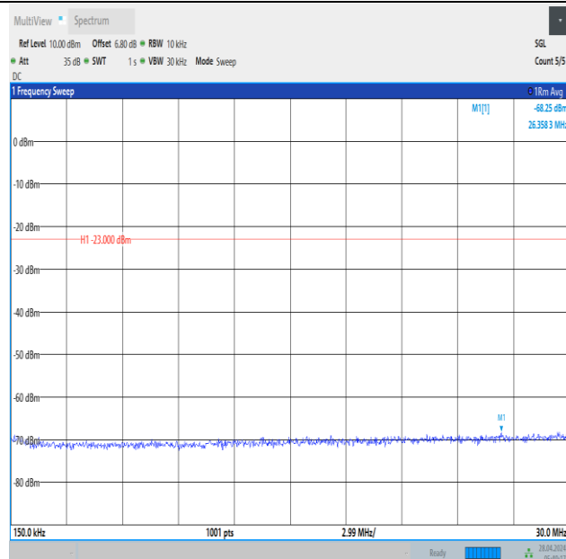
Band12_10MHz_16QAM_23060_1RB#49_0.15~30_0.15~30
