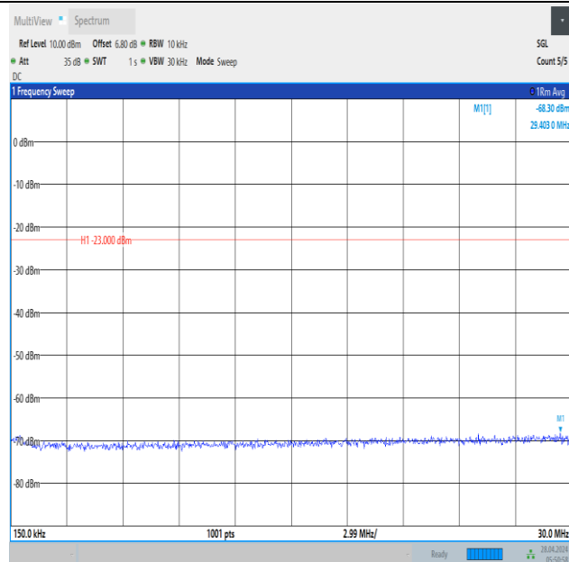
Band12_10MHz_16QAM_23095_1RB#0_0.15~30_0.15~30
