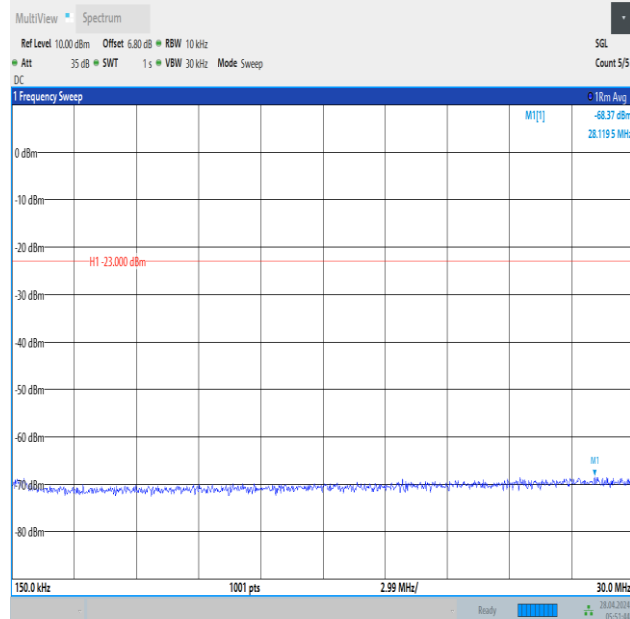
Band12_10MHz_QPSK_23095_1RB#49_0.15~30_0.15~30
