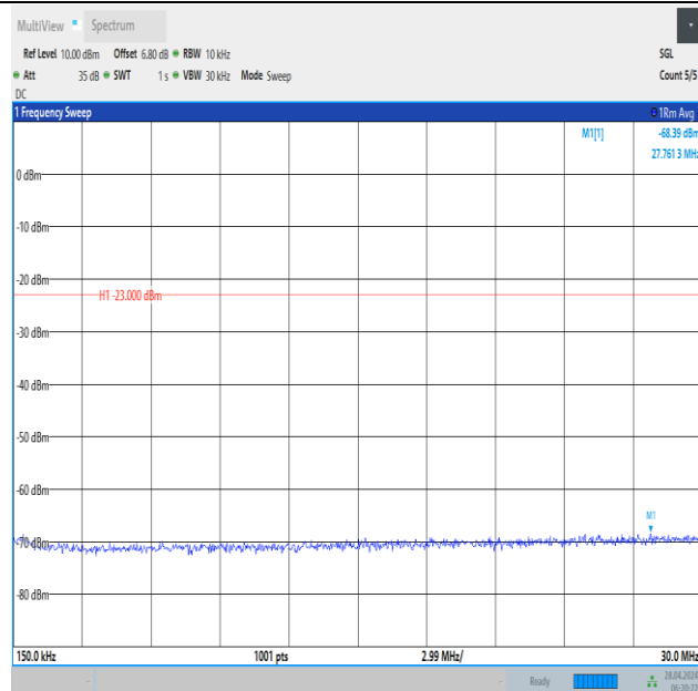
Band12_3MHz_QPSK_23025_1RB#0_0.15~30_0.15~30
