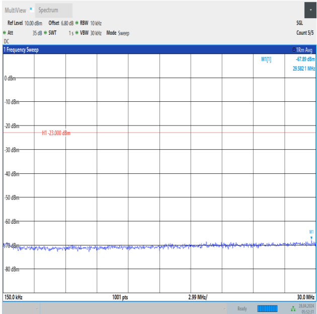
Band12_10MHz_16QAM_23095_1RB#49_0.15~30_0.15~30
