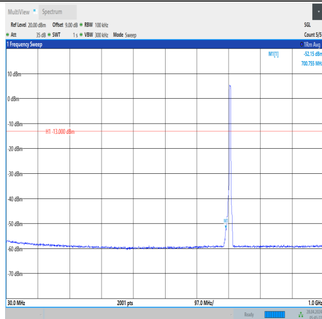
Band12_5MHz_QPSK_23155_25RB#0_30~1000_30~1000
