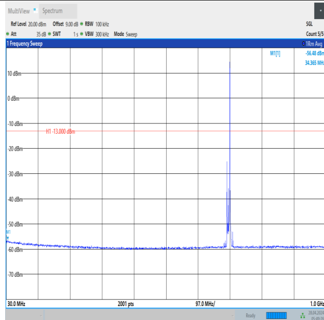
Band12_10MHz_16QAM_23060_1RB#49_30~1000_30~1000
