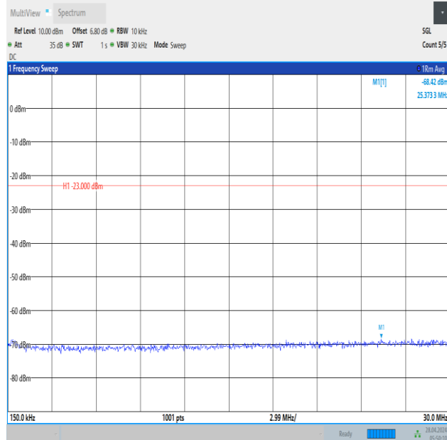
Band12_10MHz_QPSK_23095_1RB#0_0.15~30_0.15~30
