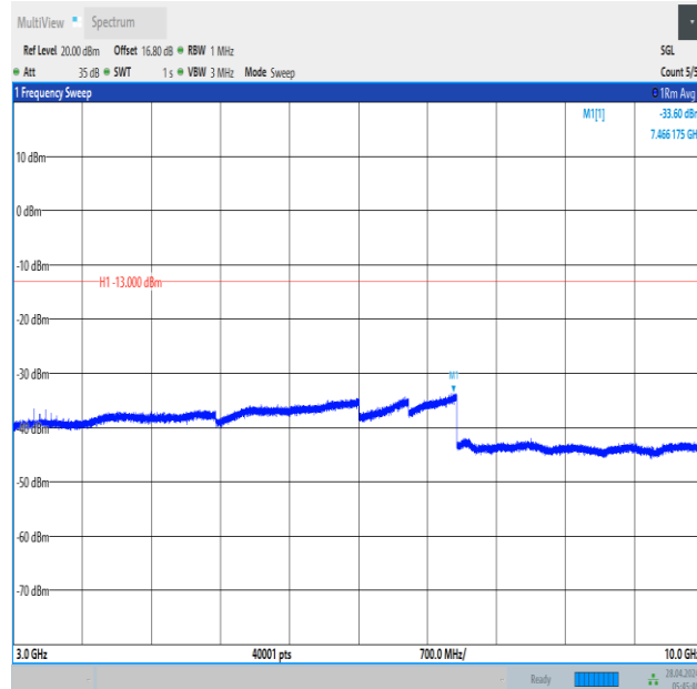
Band12_5MHz_QPSK_23155_25RB#0_3000~10000_3000~10000
