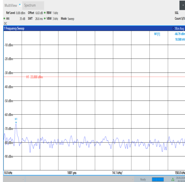
Band12_10MHz_16QAM_23095_1RB#0_0.009~0.15_0.009~0.15
