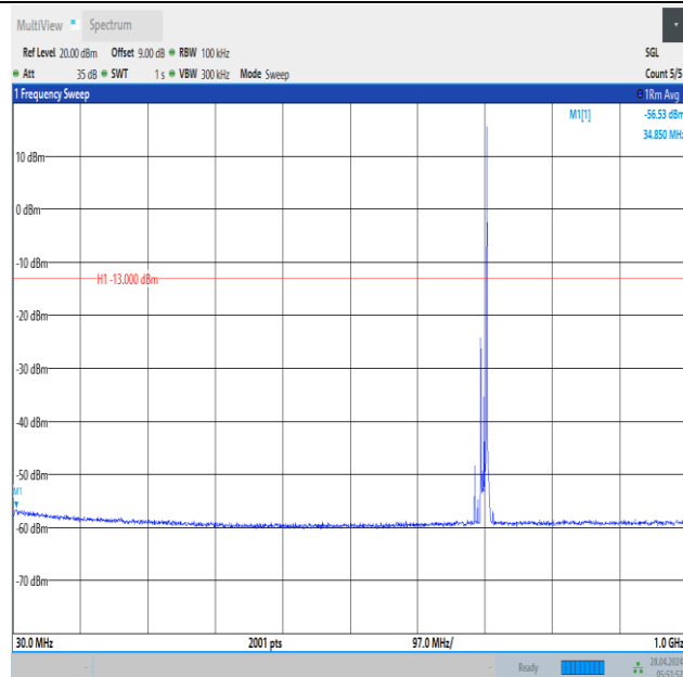
Band12_10MHz_QPSK_23095_1RB#49_30~1000_30~1000
