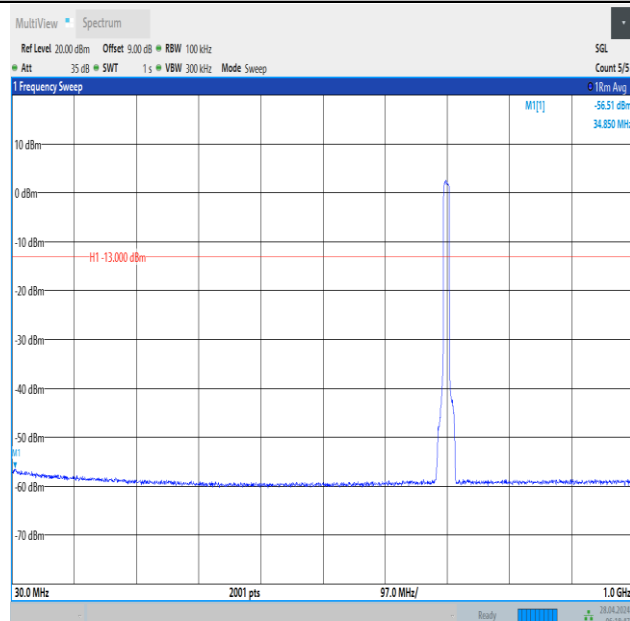
Band12_10MHz_QPSK_23095_50RB#0_30~1000_30~1000
