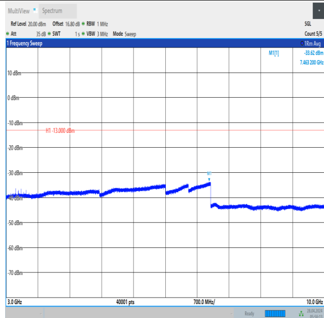
Band12_10MHz_16QAM_23130_1RB#49_3000~10000_3000~10000
