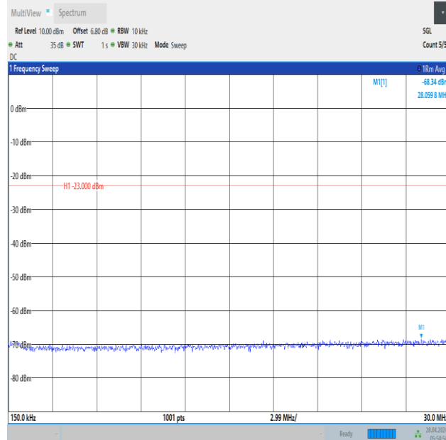
Band12_10MHz_QPSK_23130_1RB#49_0.15~30_0.15~30
