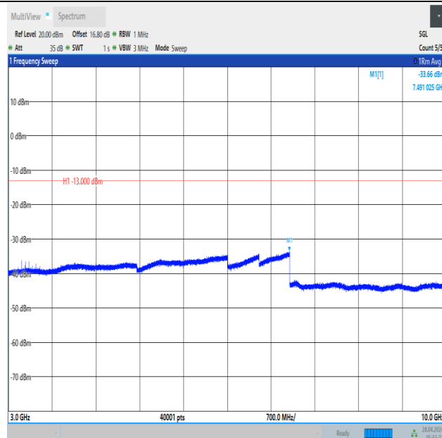
Band12_10MHz_QPSK_23130_1RB#49_3000~10000_3000~10000
