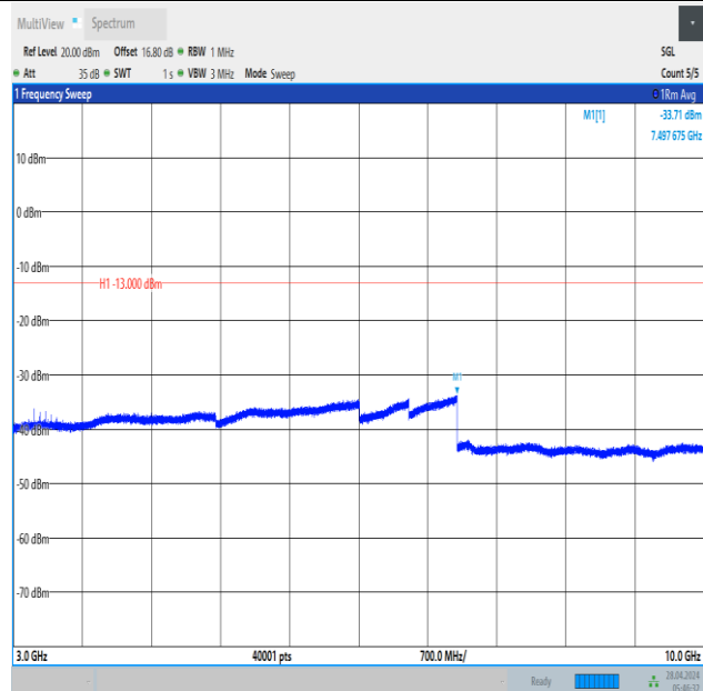
Band12_5MHz_16QAM_23155_25RB#0_3000~10000_3000~10000
