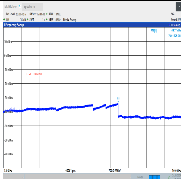
Band12_10MHz_QPSK_23130_50RB#0_3000~10000_3000~10000
