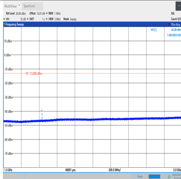
Band12_10MHz_QPSK_23130_1RB#49_1000~3000_1000~3000
