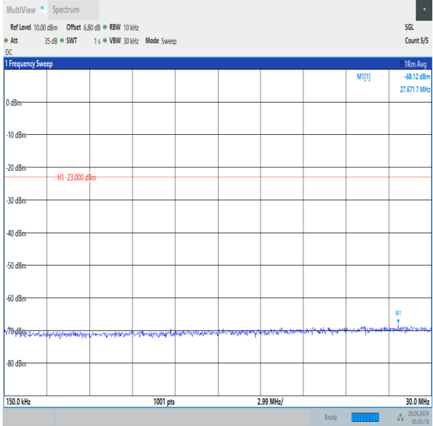
Band12_5MHz_QPSK_23155_25RB#0_0.15~30_0.15~30
