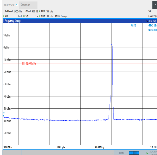
Band12_10MHz_QPSK_23130_50RB#0_30~1000_30~1000
