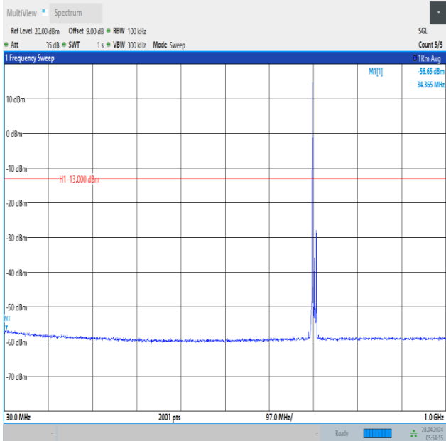
Band12_10MHz_16QAM_23130_1RB#0_30~1000_30~1000
