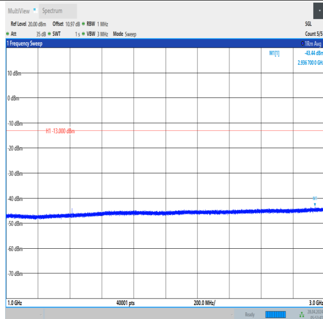
Band12_10MHz_QPSK_23130_1RB#0_1000~3000_1000~3000
