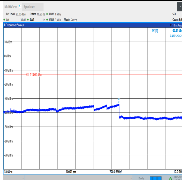
Band12_10MHz_16QAM_23060_1RB#0_3000~10000_3000~10000
