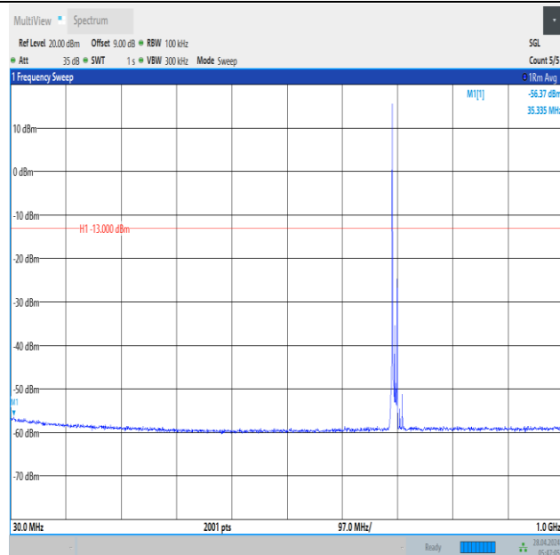
Band12_10MHz_QPSK_23060_1RB#0_30~1000_30~1000
