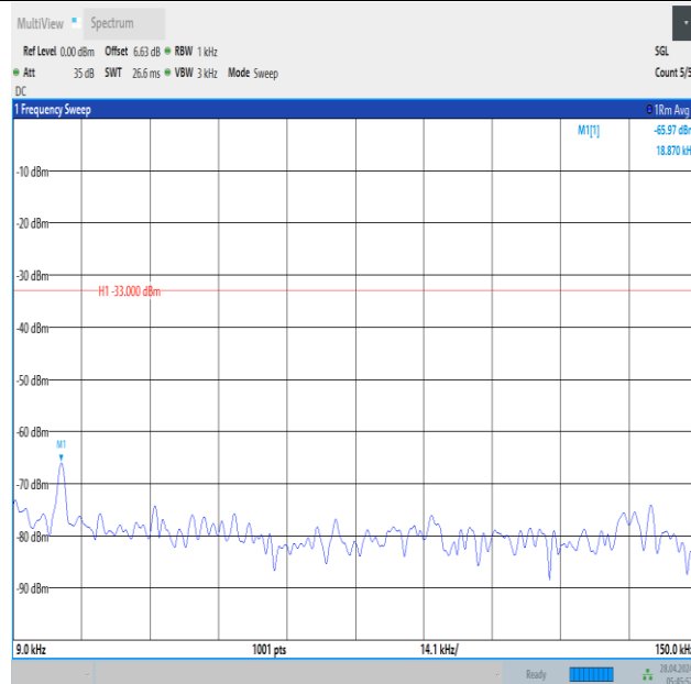
Band12_5MHz_16QAM_23155_25RB#0_0.009~0.15_0.009~0.15
