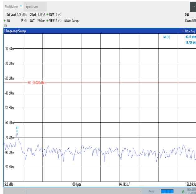
Band12_10MHz_16QAM_23060_1RB#49_0.009~0.15_0.009~0.15
