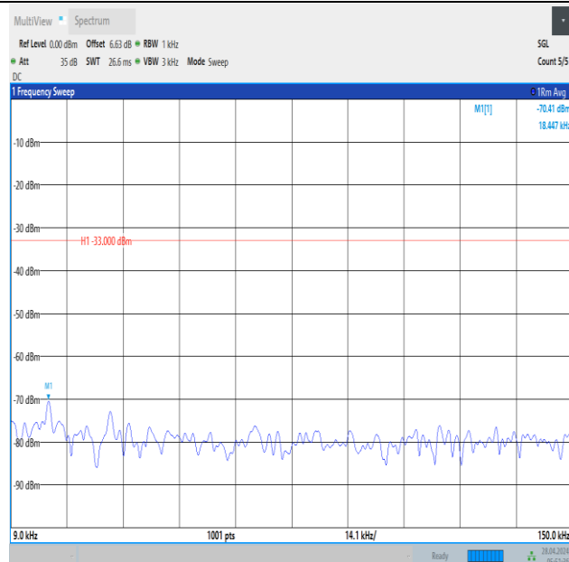
Band12_10MHz_QPSK_23095_1RB#49_0.009~0.15_0.009~0.15
