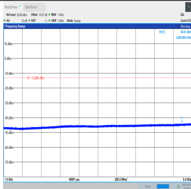
Band12_10MHz_QPSK_23060_1RB#49_1000~3000_1000~3000
