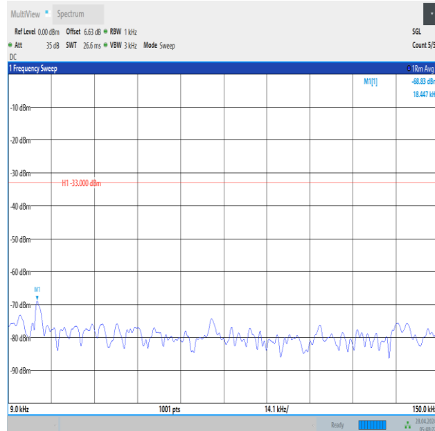
Band12_10MHz_QPSK_23060_1RB#49_0.009~0.15_0.009~0.15
