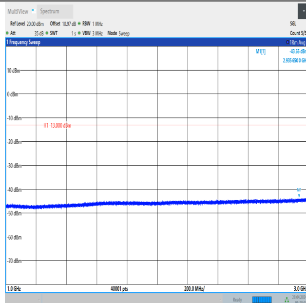
Band12_10MHz_QPSK_23095_50RB#0_1000~3000_1000~3000
