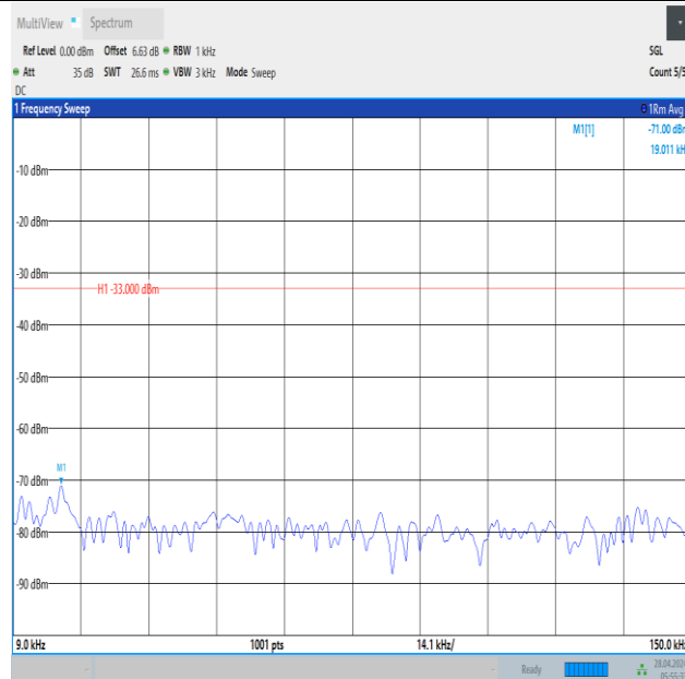
Band12_10MHz_16QAM_23130_1RB#49_0.009~0.15_0.009~0.15
