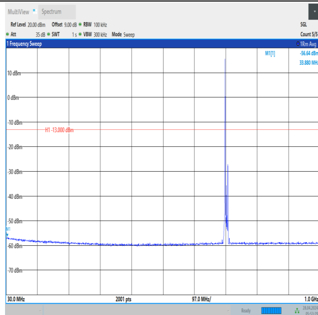
Band12_10MHz_QPSK_23130_1RB#0_30~1000_30~1000
