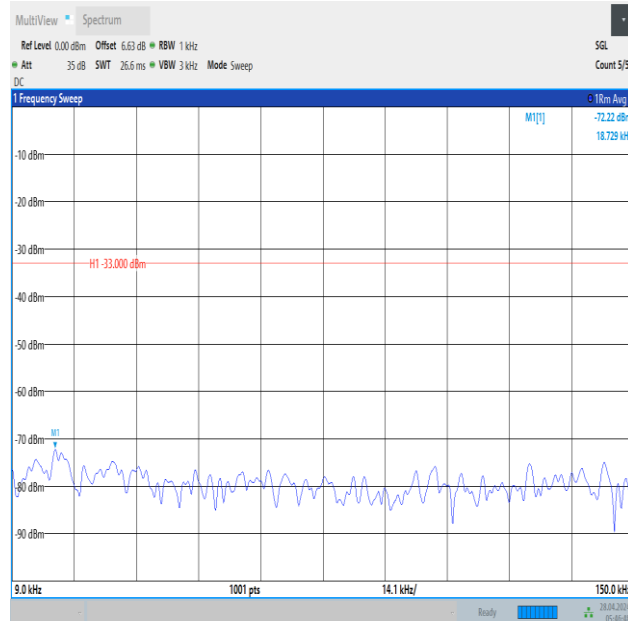
Band12_10MHz_QPSK_23060_1RB#0_0.009~0.15_0.009~0.15
