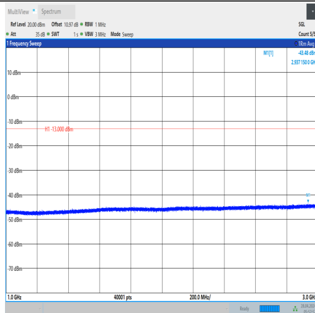
Band12_10MHz_16QAM_23095_1RB#49_1000~3000_1000~3000
