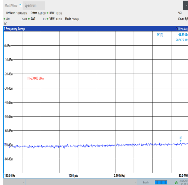
Band12_10MHz_QPSK_23130_1RB#0_0.15~30_0.15~30
