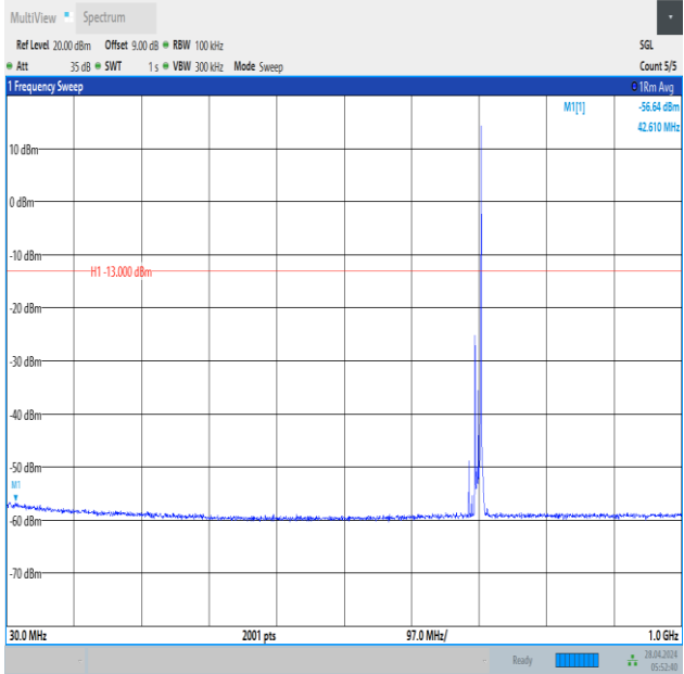
Band12_10MHz_16QAM_23095_1RB#49_30~1000_30~1000
