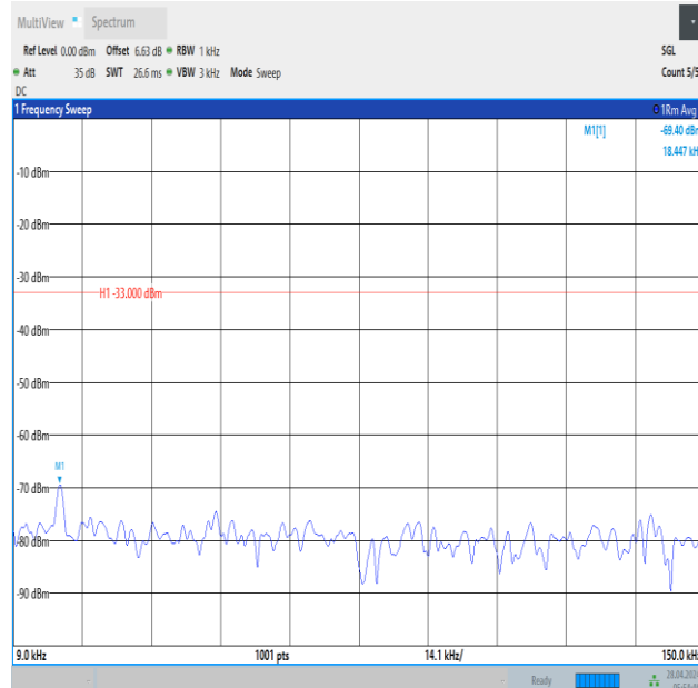
Band12_10MHz_QPSK_23130_1RB#49_0.009~0.15_0.009~0.15
