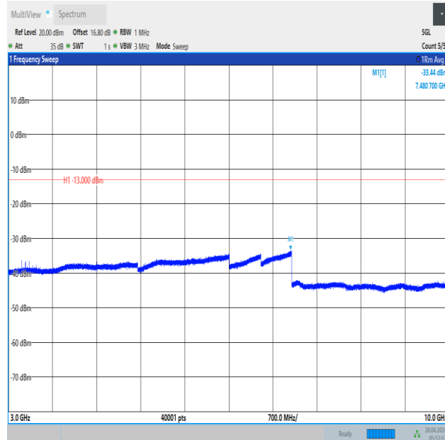
Band12_10MHz_QPSK_23130_1RB#0_3000~10000_3000~10000
