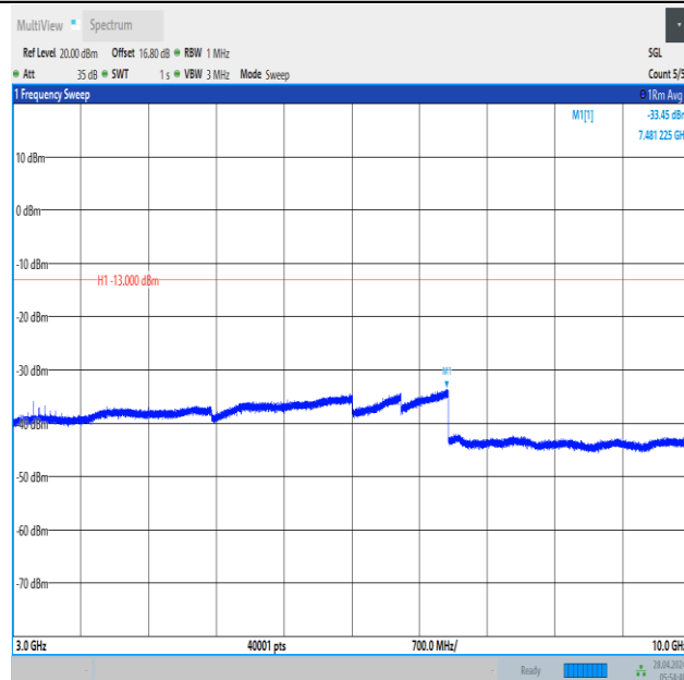
Band12_10MHz_16QAM_23130_1RB#0_3000~10000_3000~10000
