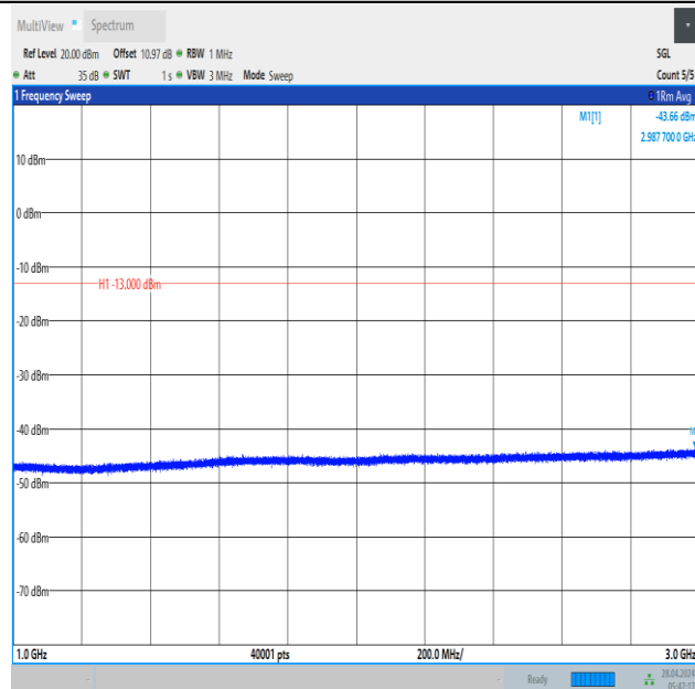
Band12_10MHz_QPSK_23060_1RB#0_1000~3000_1000~3000
