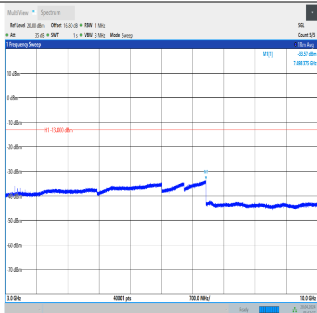
Band12_10MHz_QPSK_23095_1RB#49_3000~10000_3000~10000
