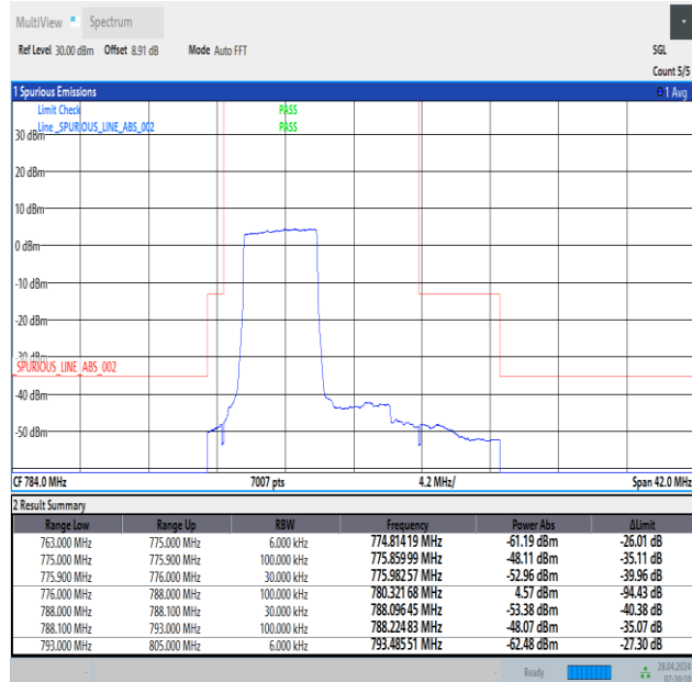
Band13_5MHz_QPSK_23205_25RB#0
