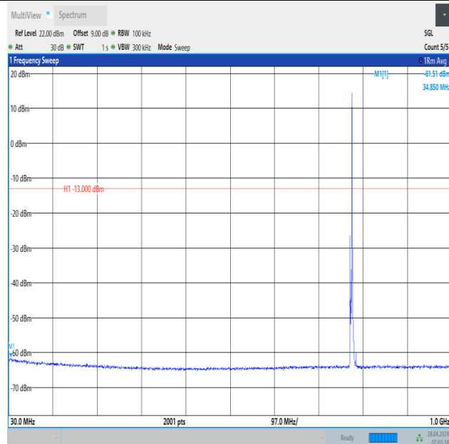
Band13_5MHz_16QAM_23205_1RB#24_30~1000_30~1000
