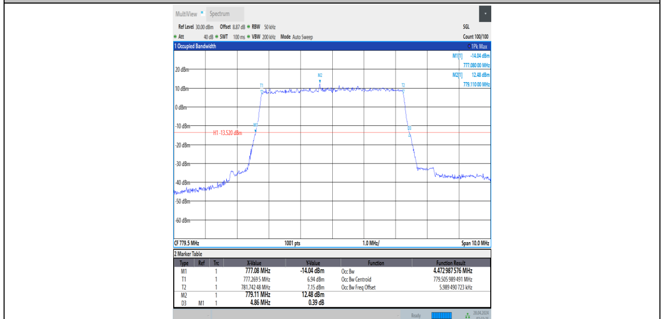
Band13-5MHz-16QAM-23205-25RB#0-PASS
