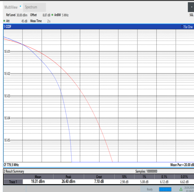
Band13-5MHz-16QAM-23205-25RB#0-PASS
