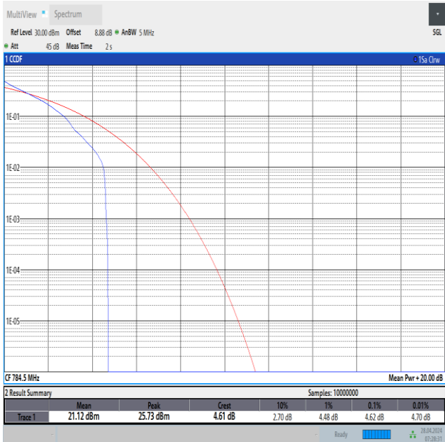
Band13-5MHz-QPSK-23255-1RB#0-PASS
