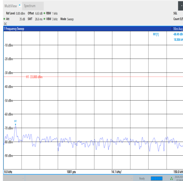
Band13_5MHz_QPSK_23205_25RB#0_0.009~0.15_0.009~0.15
