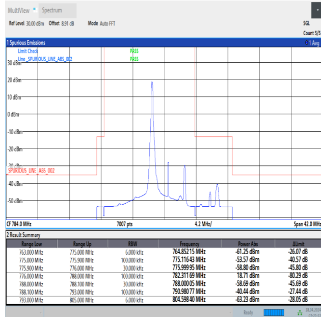
Band13_5MHz_QPSK_23255_1RB#0
