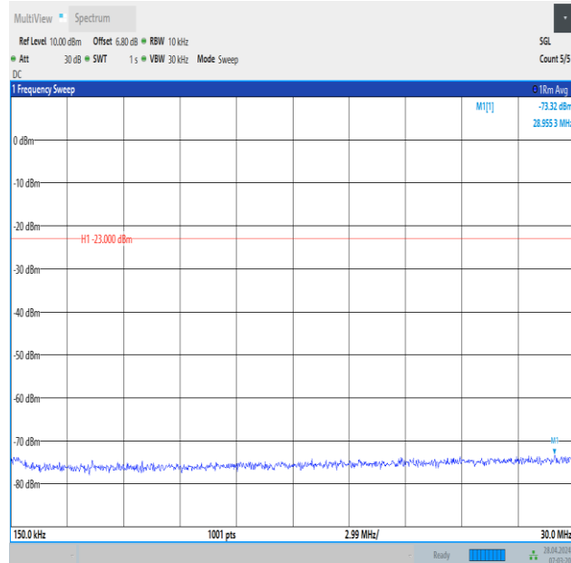
Band13_5MHz_16QAM_23205_1RB#24_0.15~30_0.15~30
