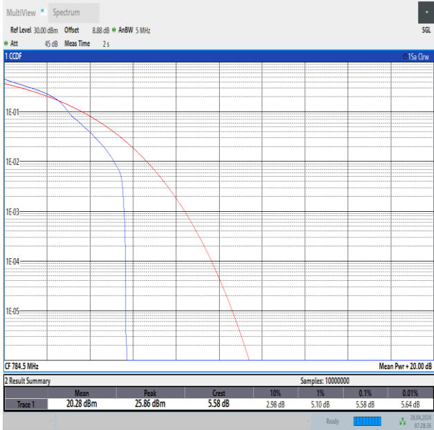
Band13-5MHz-16QAM-23255-1RB#0-PASS
