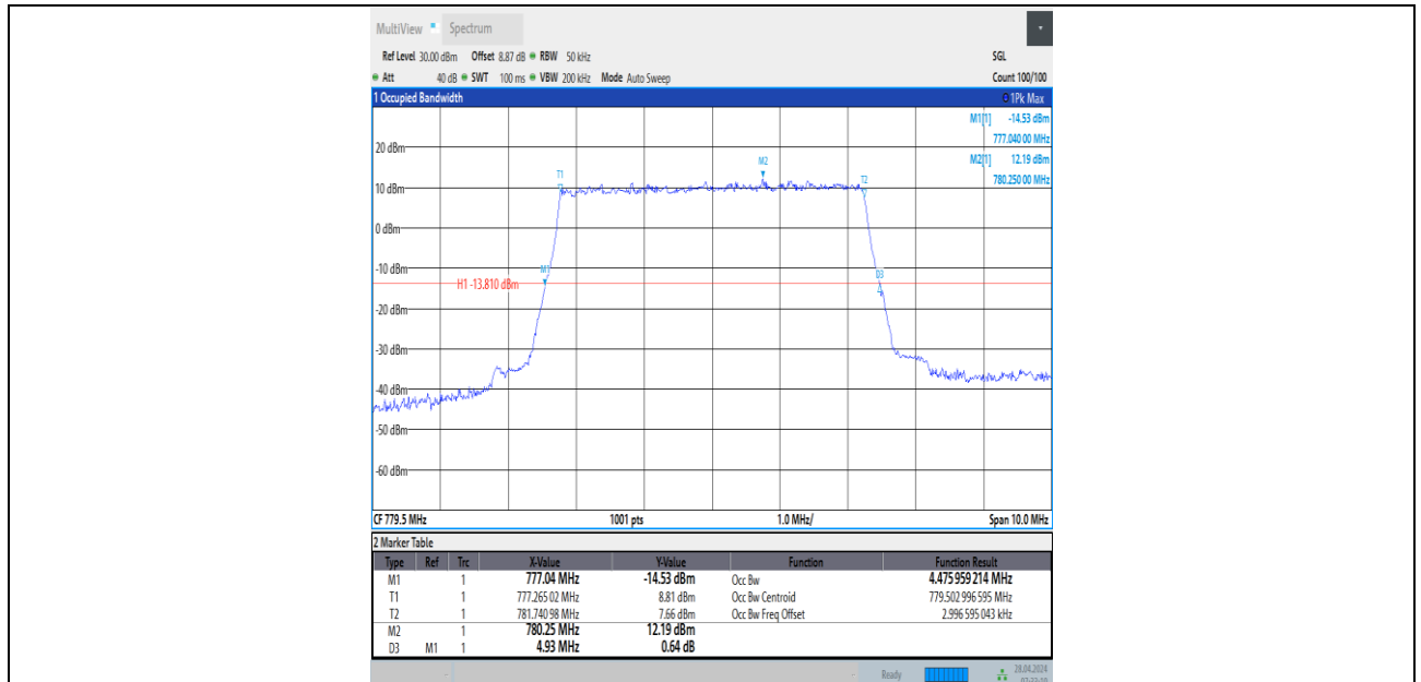
Band13-5MHz-QPSK-23205-25RB#0-PASS
