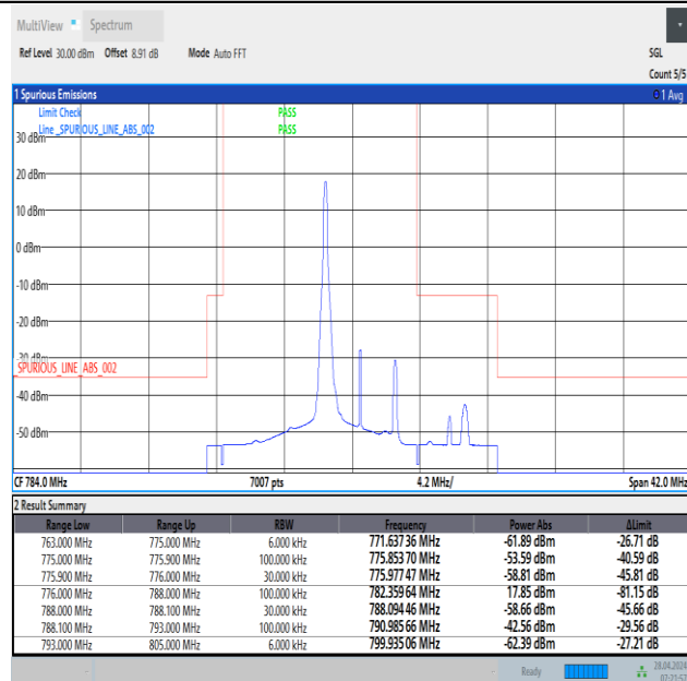
Band13_5MHz_16QAM_23255_1RB#0
