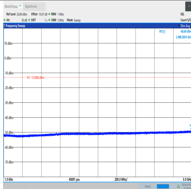
Band13_5MHz_QPSK_23205_25RB#0_1000~3000_1000~3000
