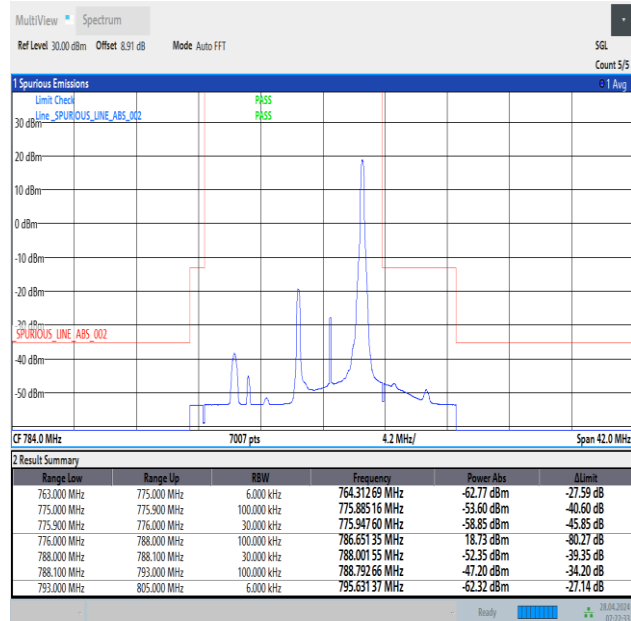
Band13_5MHz_QPSK_23255_1RB#24
