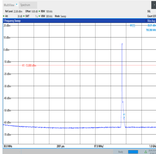
Band13_5MHz_QPSK_23205_25RB#0_30~1000_30~1000
