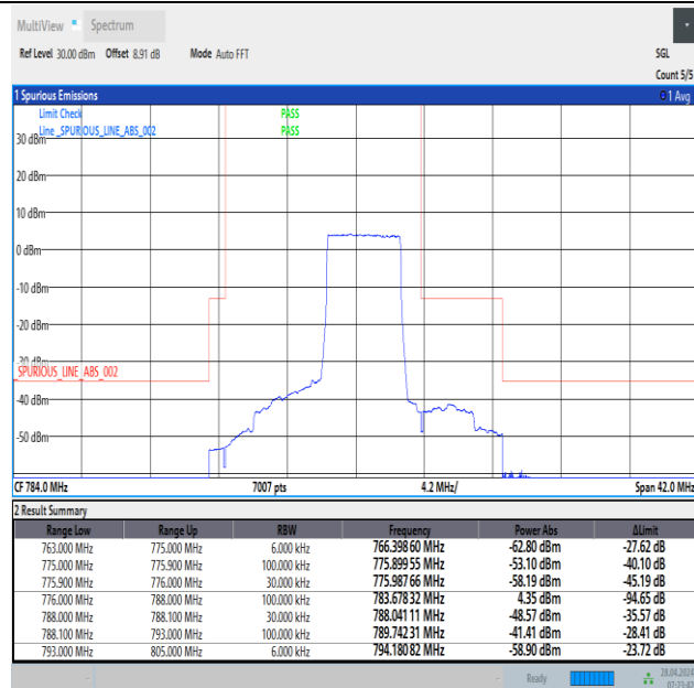
Band13_5MHz_QPSK_23255_25RB#0
