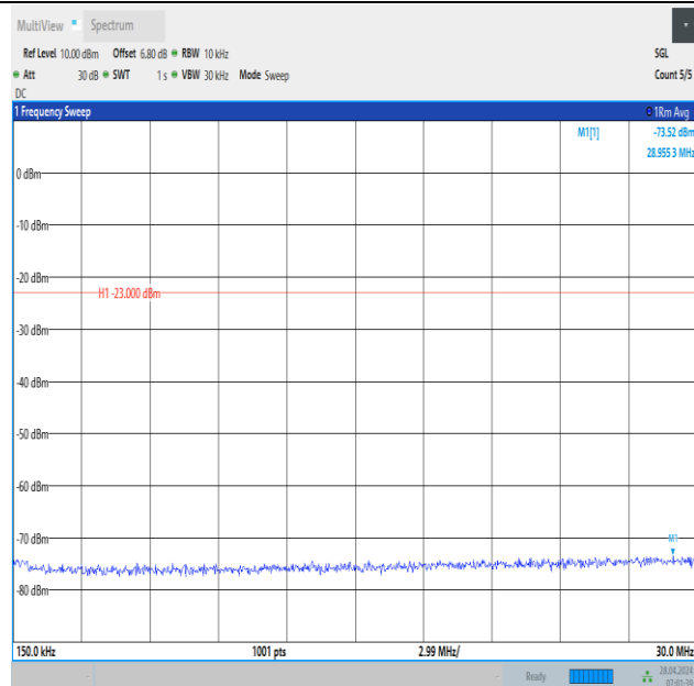
Band13_5MHz_16QAM_23205_1RB#0_0.15~30_0.15~30
