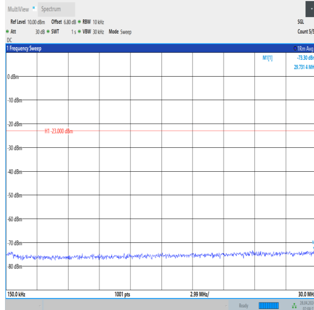
Band13_5MHz_QPSK_23205_25RB#0_0.15~30_0.15~30
