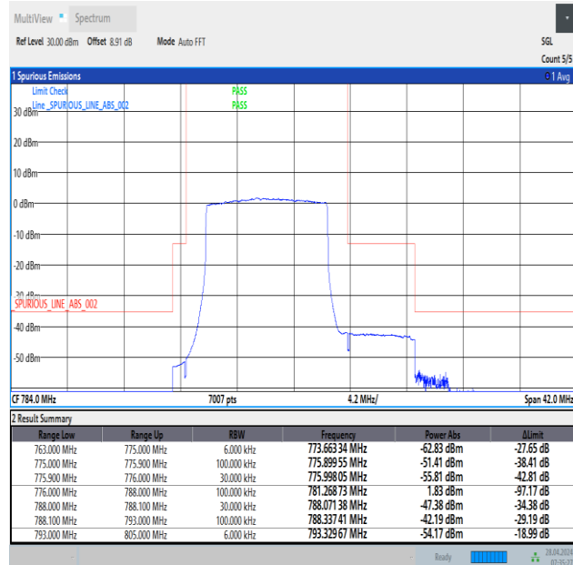
Band13_10MHz_QPSK_23230_50RB#0
