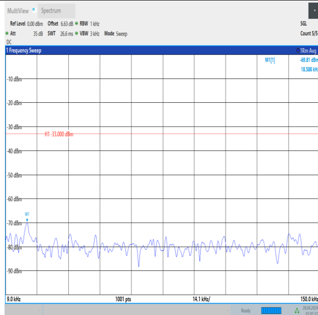
Band13_5MHz_16QAM_23205_1RB#0_0.009~0.15_0.009~0.15
