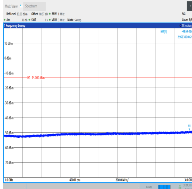
Band13_5MHz_16QAM_23205_25RB#0_1000~3000_1000~3000
