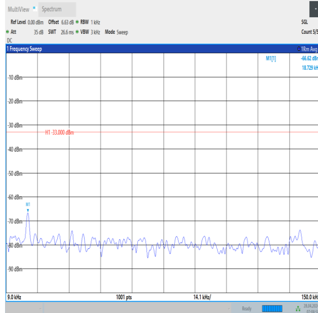
Band13_5MHz_16QAM_23205_25RB#0_0.009~0.15_0.009~0.15
