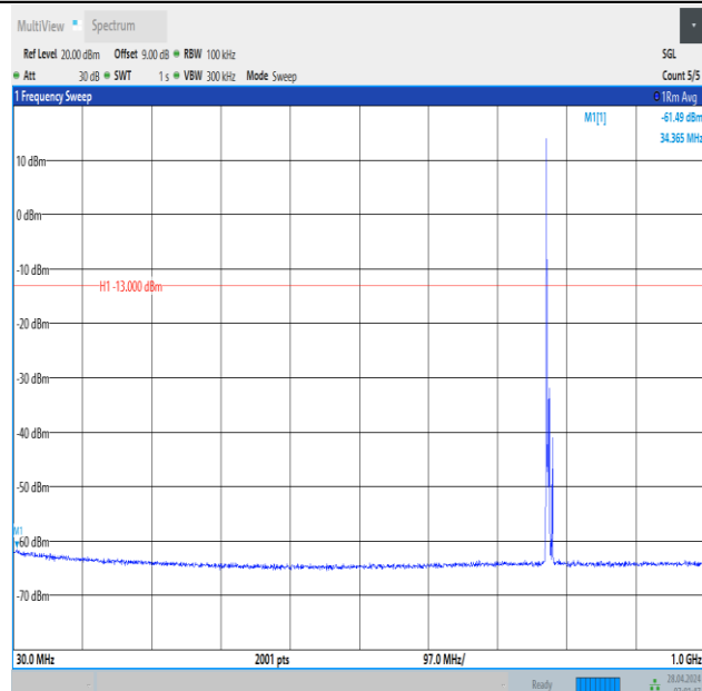
Band13_5MHz_16QAM_23205_1RB#0_30~1000_30~1000
