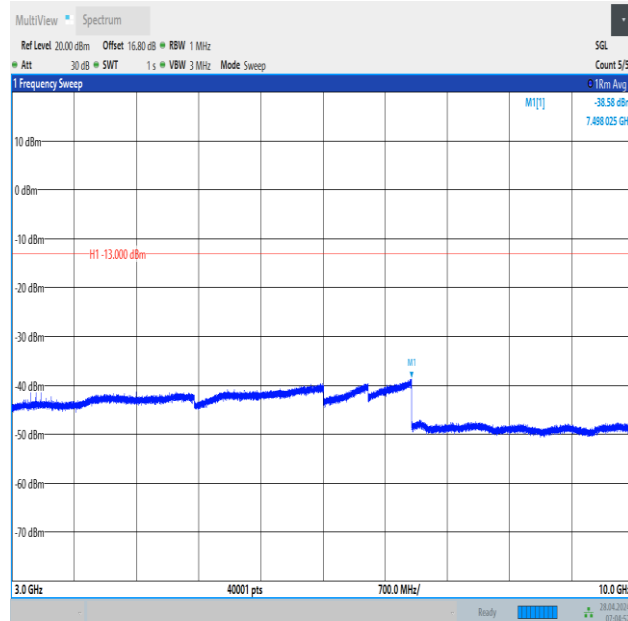
Band13_5MHz_QPSK_23205_25RB#0_3000~10000_3000~10000
