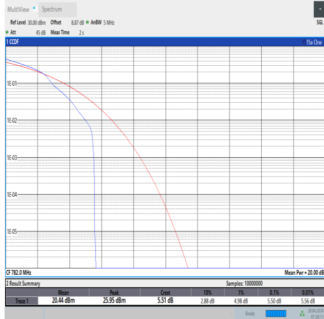
Band13-5MHz-16QAM-23230-1RB#0-PASS
