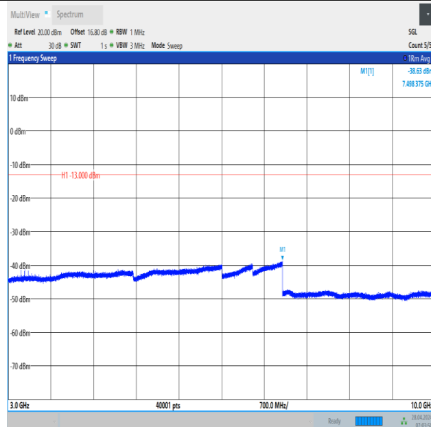
Band13_5MHz_16QAM_23205_1RB#24_3000~10000_3000~10000
