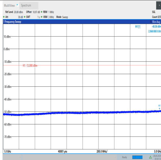
Band13_5MHz_QPSK_23205_1RB#0_1000~3000_1000~3000
