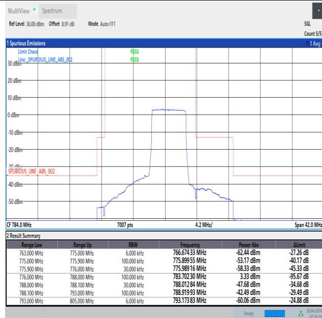
Band13_5MHz_16QAM_23255_25RB#0
