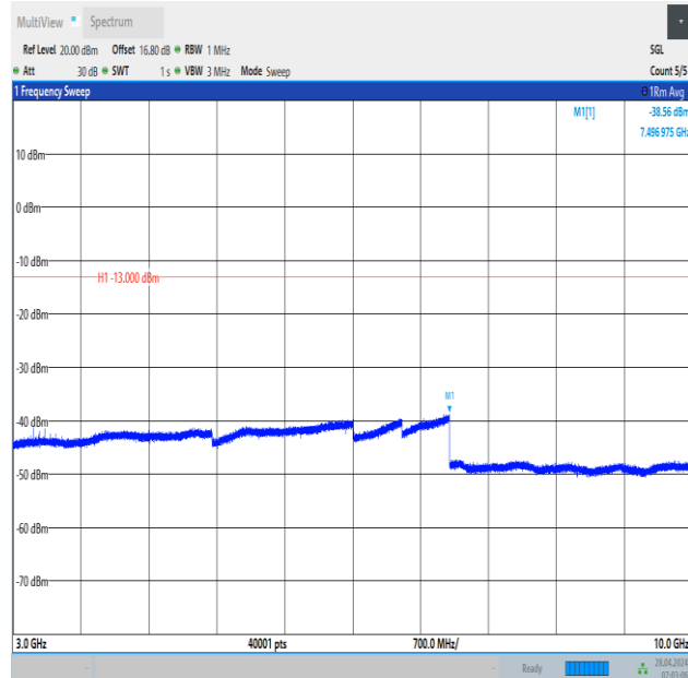
Band13_5MHz_QPSK_23205_1RB#24_3000~10000_3000~10000
