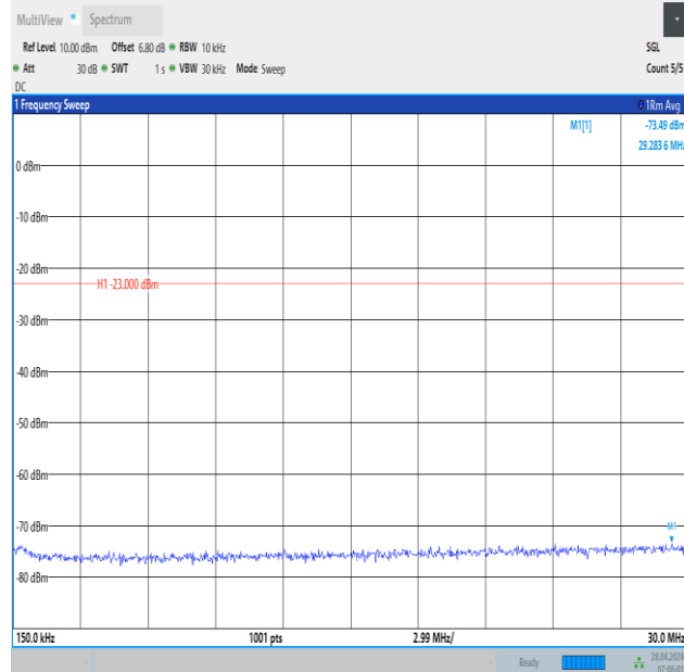
Band13_5MHz_QPSK_23230_1RB#0_0.15~30_0.15~30
