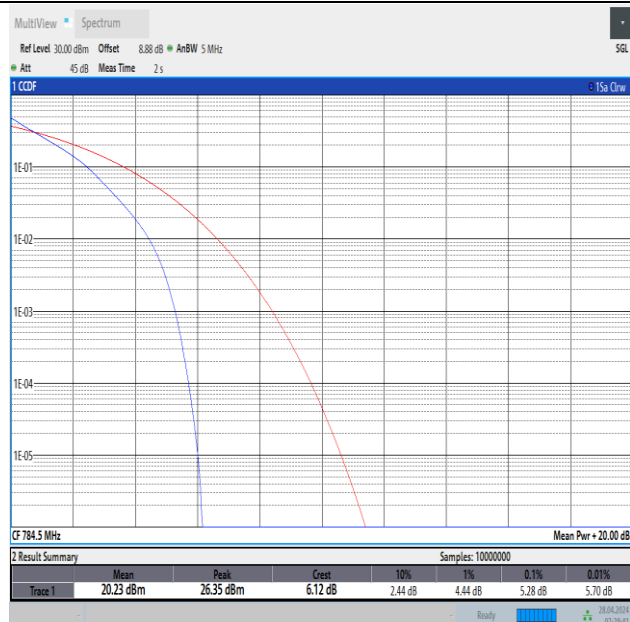
Band13-5MHz-QPSK-23255-25RB#0-PASS
