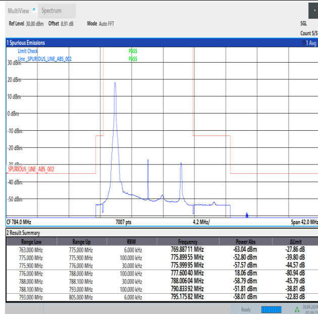
Band13_10MHz_QPSK_23230_1RB#0
