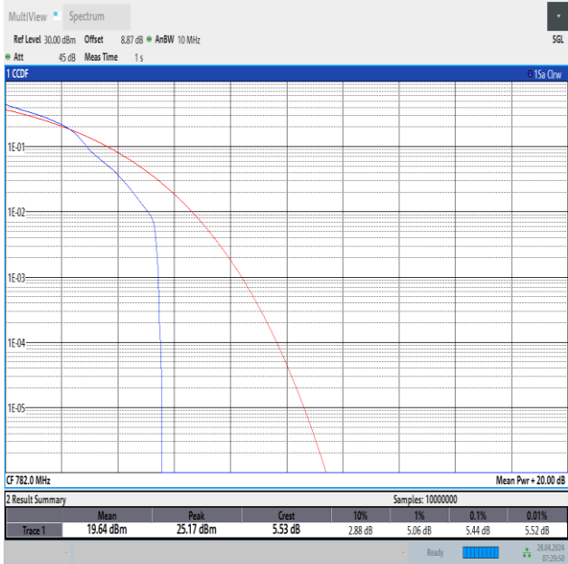
Band13-10MHz-16QAM-23230-1RB#0-PASS
