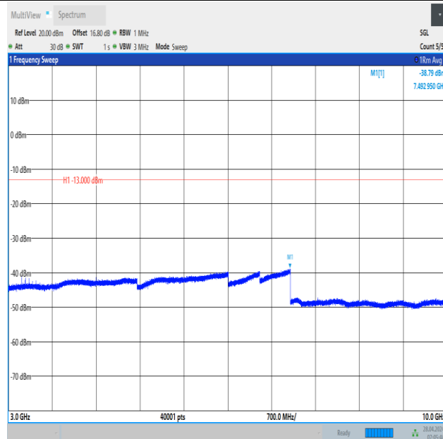
Band13_5MHz_16QAM_23205_25RB#0_3000~10000_3000~10000
