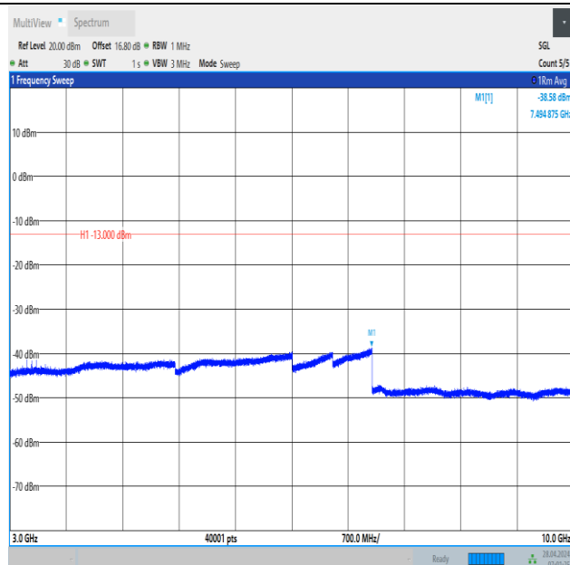
Band13_5MHz_QPSK_23205_1RB#0_3000~10000_3000~10000
