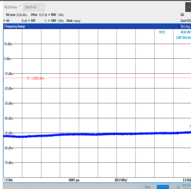
Band13_5MHz_16QAM_23205_1RB#0_1000~3000_1000~3000
