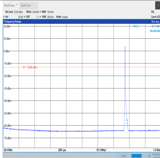
Band13_5MHz_16QAM_23205_25RB#0_30~1000_30~1000
