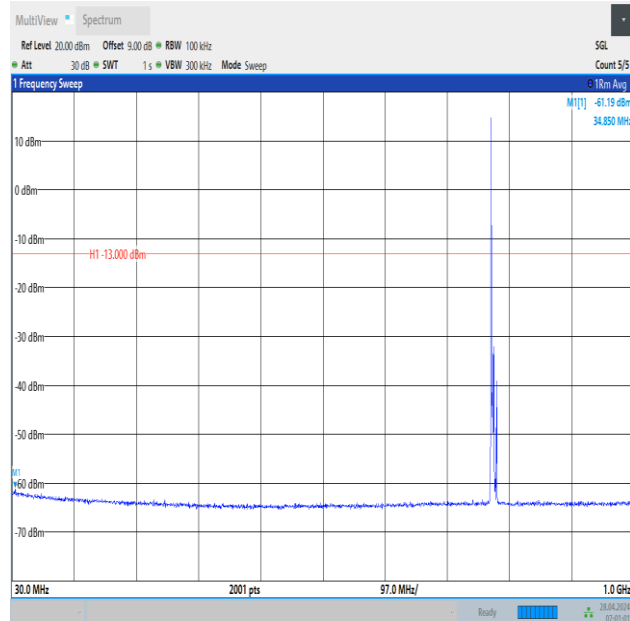
Band13_5MHz_QPSK_23205_1RB#0_30~1000_30~1000
