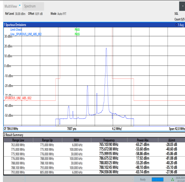
Band13_5MHz_16QAM_23255_1RB#24
