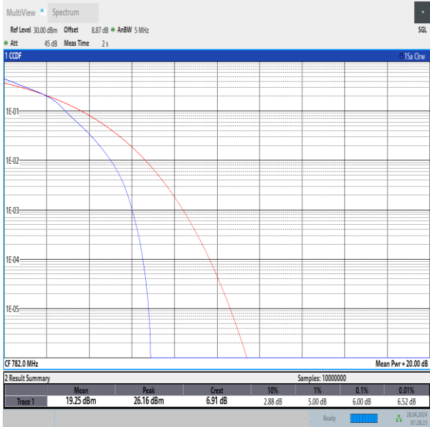
Band13-5MHz-16QAM-23230-25RB#0-PASS
