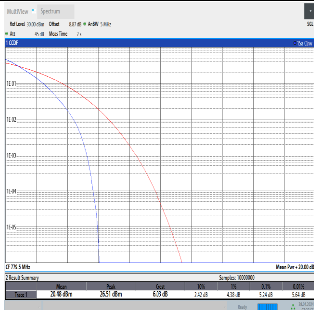
Band13-5MHz-QPSK-23205-25RB#0-PASS
