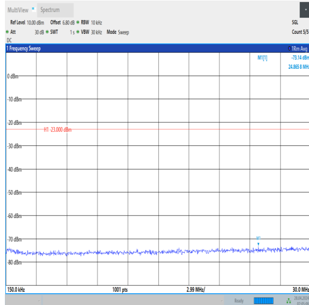
Band13_5MHz_16QAM_23205_25RB#0_0.15~30_0.15~30
