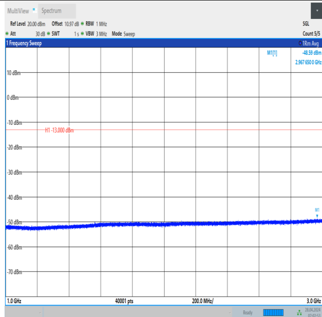
Band13_5MHz_QPSK_23205_1RB#24_1000~3000_1000~3000
