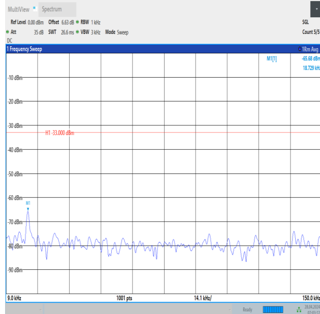
Band13_5MHz_16QAM_23205_1RB#24_0.009~0.15_0.009~0.15
