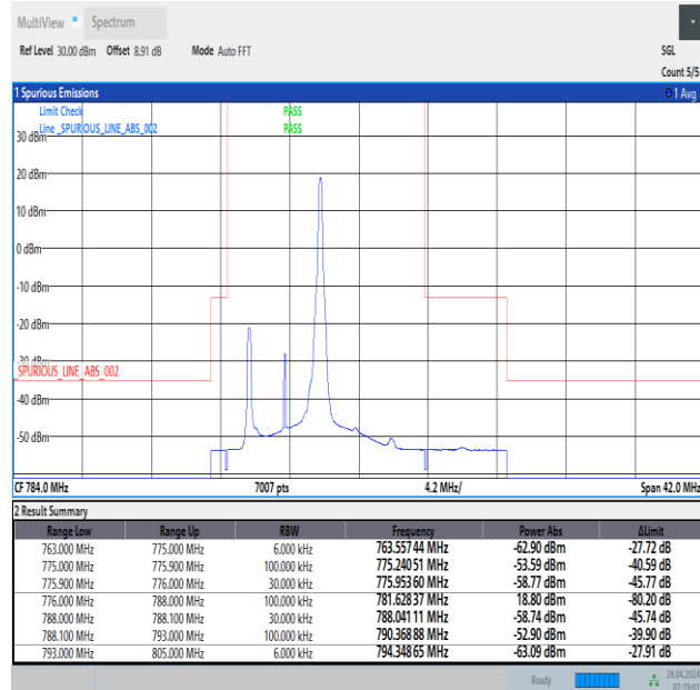
Band13_5MHz_QPSK_23205_1RB#24
