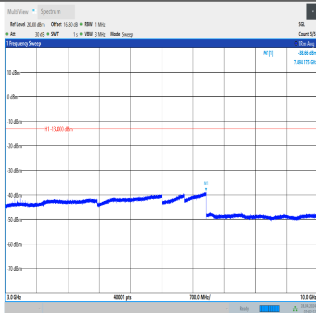
Band13_5MHz_16QAM_23205_1RB#0_3000~10000_3000~10000
