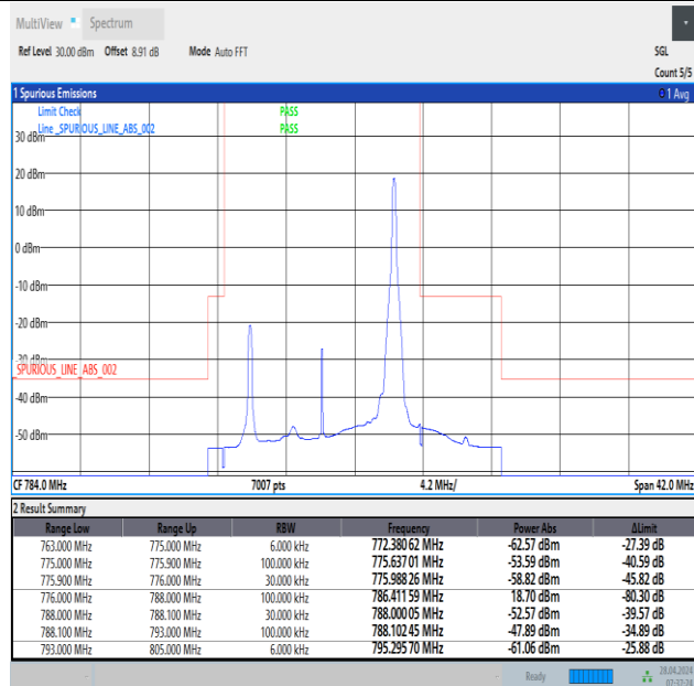
Band13_10MHz_QPSK_23230_1RB#49
