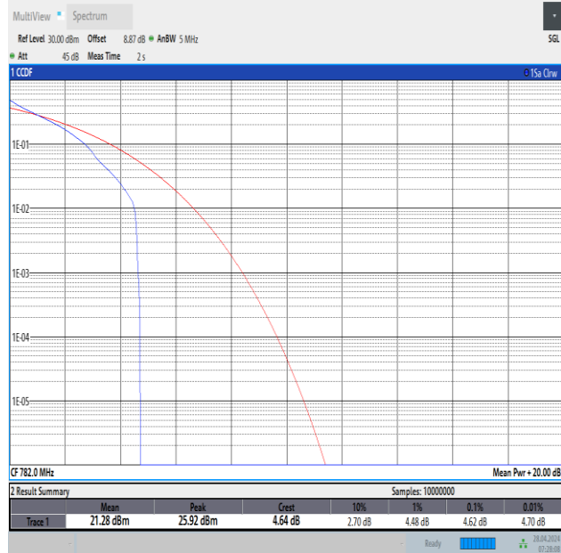
Band13-5MHz-QPSK-23230-1RB#0-PASS
