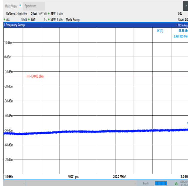
Band13_5MHz_16QAM_23205_1RB#24_1000~3000_1000~3000
