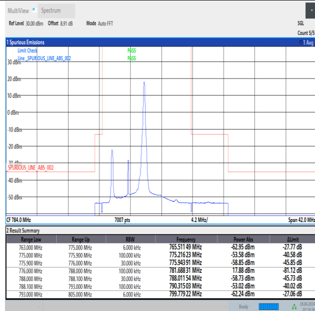
Band13_5MHz_16QAM_23205_1RB#24
