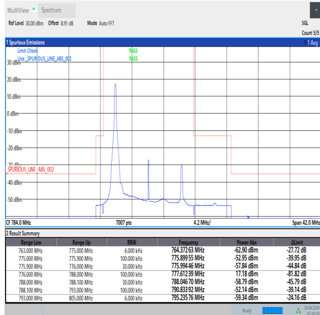
Band13_10MHz_16QAM_23230_1RB#0
