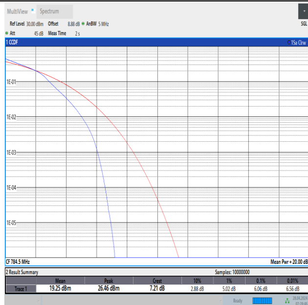
Band13-5MHz-16QAM-23255-25RB#0-PASS
