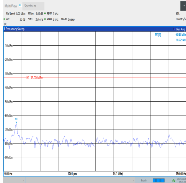
Band13_5MHz_QPSK_23230_1RB#0_0.009~0.15_0.009~0.15
