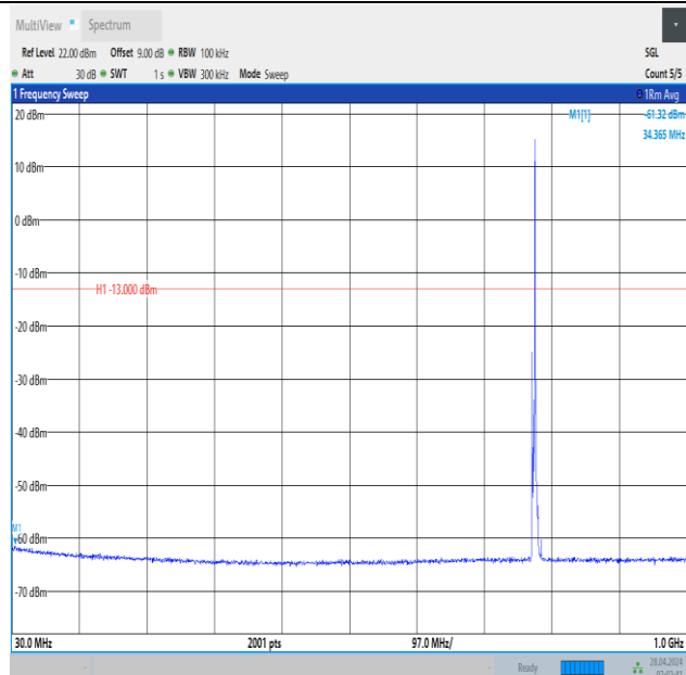
Band13_5MHz_QPSK_23205_1RB#24_30~1000_30~1000
