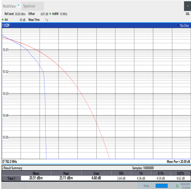
Band13-10MHz-QPSK-23230-1RB#0-PASS
