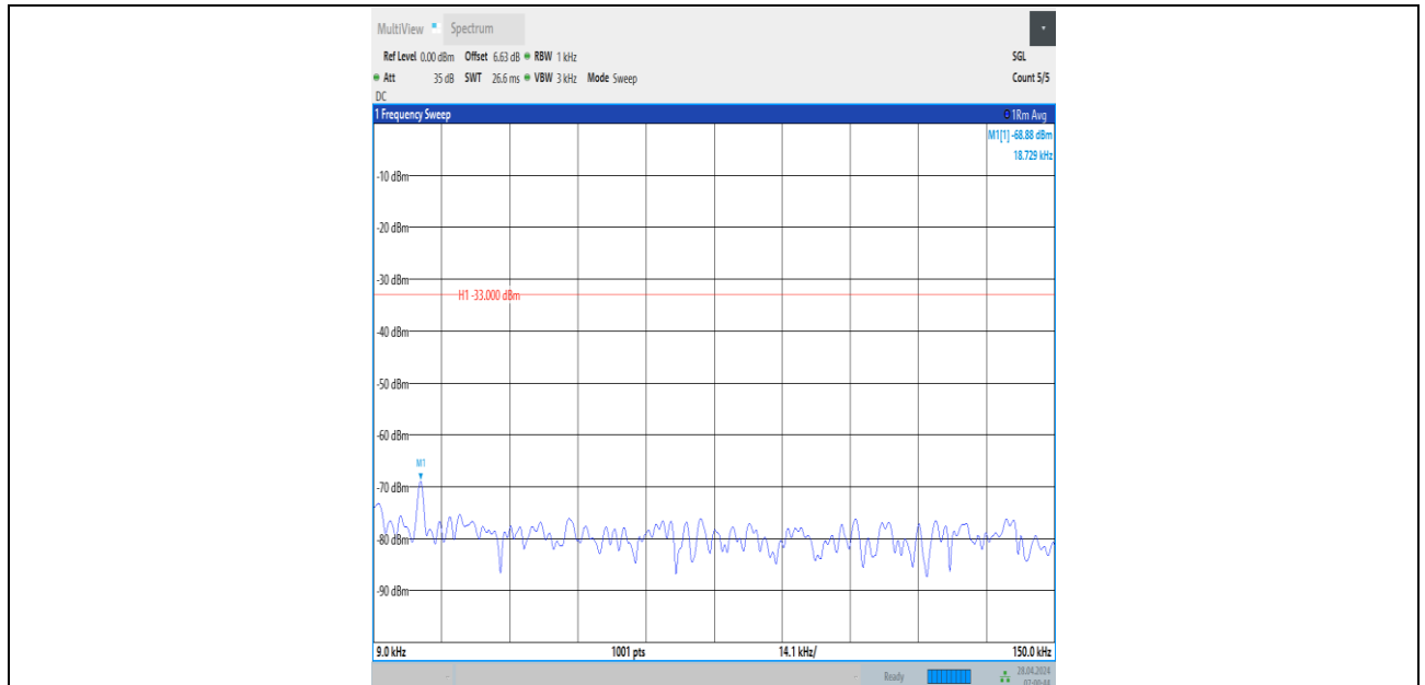
Band13_5MHz_QPSK_23205_1RB#0_0.009~0.15_0.009~0.15
