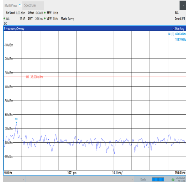
Band13_10MHz_QPSK_23230_1RB#0_0.009~0.15_0.009~0.15
