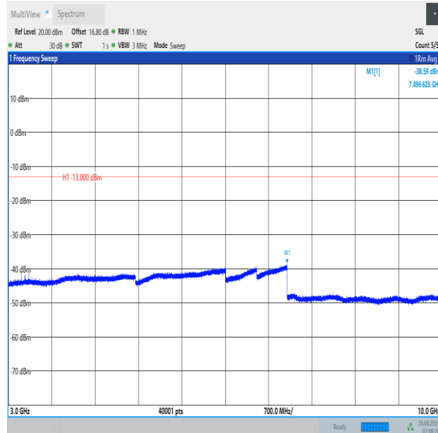
Band13_5MHz_QPSK_23230_1RB#24_3000~10000_3000~10000
