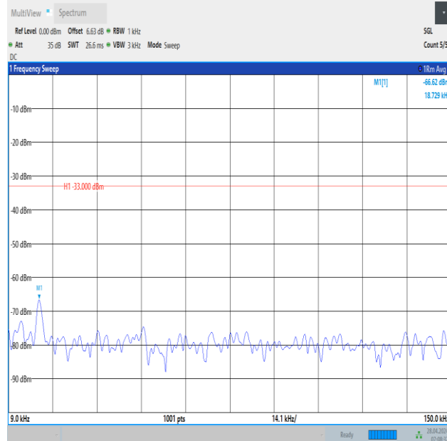
Band13_5MHz_16QAM_23230_1RB#24_0.009~0.15_0.009~0.15
