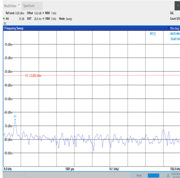
Band13_10MHz_QPSK_23230_50RB#0_0.009~0.15_0.009~0.15
