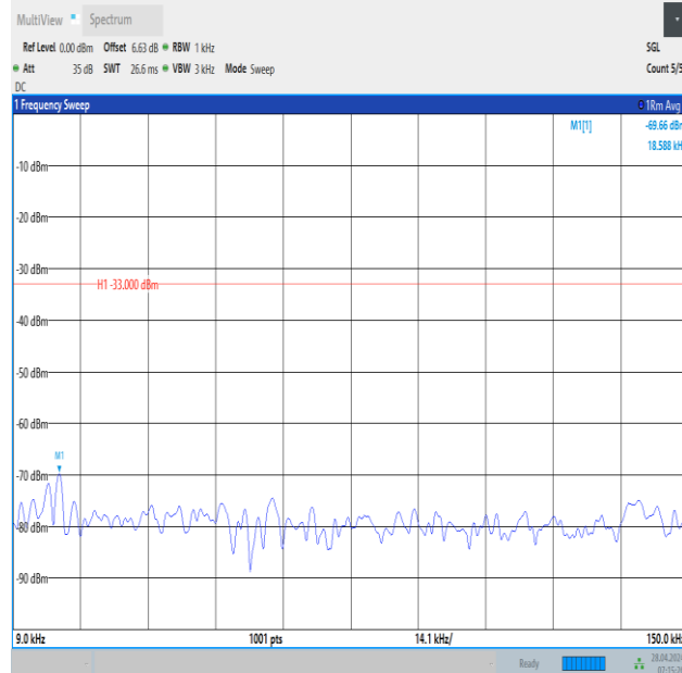
Band13_5MHz_16QAM_23255_25RB#0_0.009~0.15_0.009~0.15
