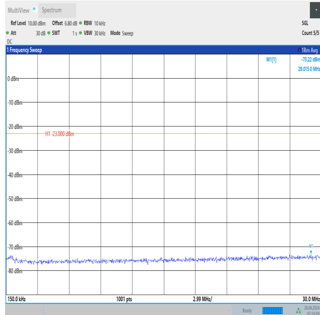
Band13_5MHz_16QAM_23255_1RB#24_0.15~30_0.15~30
