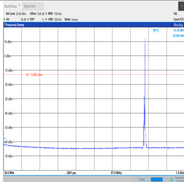
Band13_5MHz_16QAM_23255_1RB#24_30~1000_30~1000
