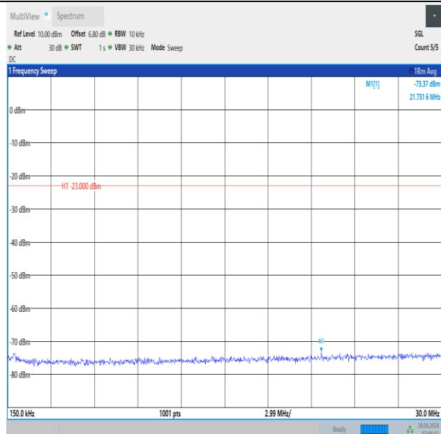
Band13_5MHz_16QAM_23230_1RB#24_0.15~30_0.15~30
