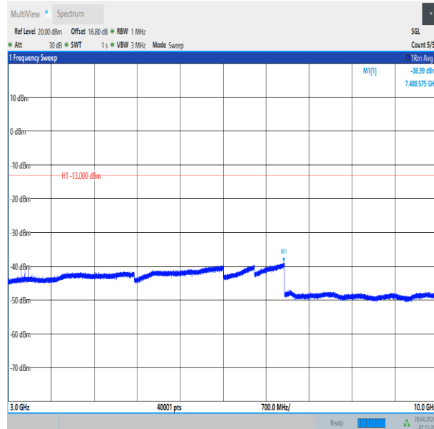
Band13_5MHz_QPSK_23255_25RB#0_3000~10000_3000~10000
