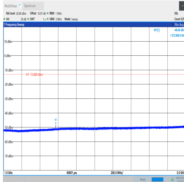
Band13_10MHz_QPSK_23230_1RB#49_1000~3000_1000~3000
