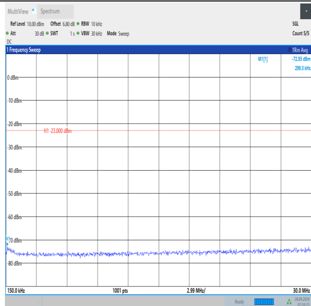
Band13_5MHz_16QAM_23230_25RB#0_0.15~30_0.15~30
