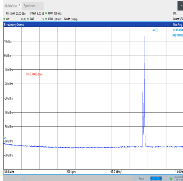
Band13_10MHz_16QAM_23230_1RB#49_30~1000_30~1000
