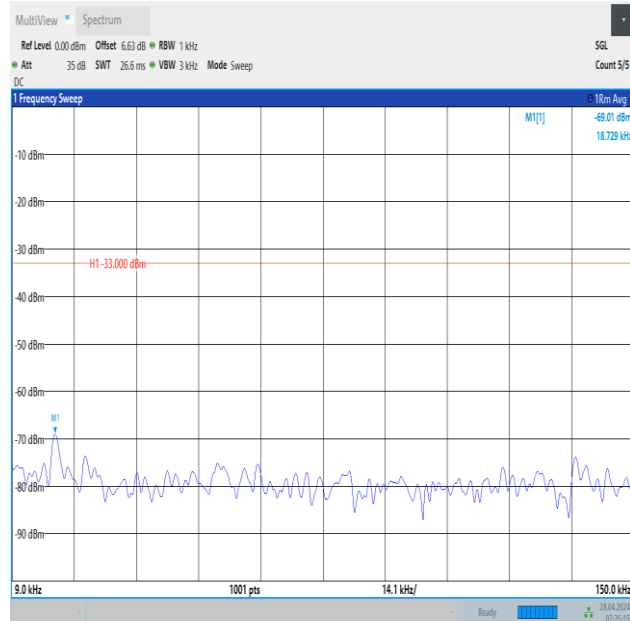
Band13_10MHz_16QAM_23230_1RB#0_0.009~0.15_0.009~0.15
