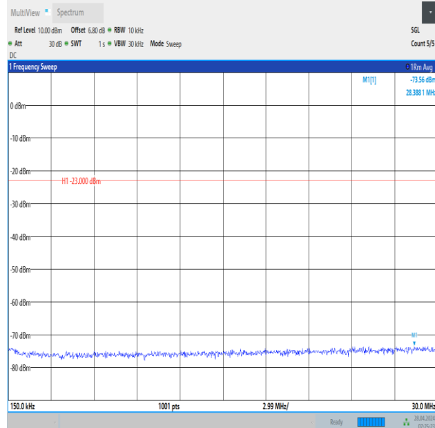
Band13_10MHz_16QAM_23230_1RB#0_0.15~30_0.15~30
