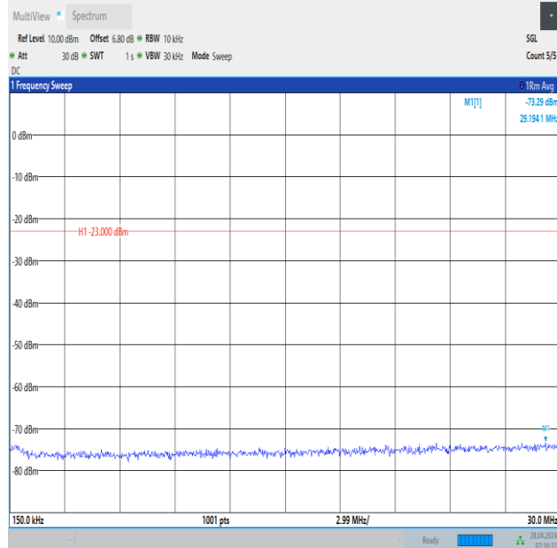
Band13_10MHz_QPSK_23230_50RB#0_0.15~30_0.15~30
