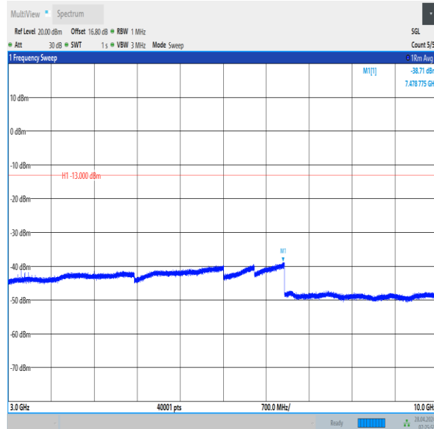
Band13_10MHz_16QAM_23230_1RB#0_3000~10000_3000~10000
