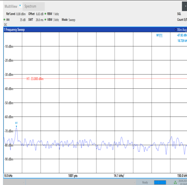
Band13_10MHz_QPSK_23230_1RB#49_0.009~0.15_0.009~0.15
