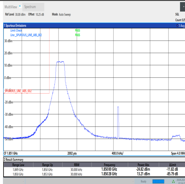
Band2_3MHz_16QAM_18615_1RB#0
