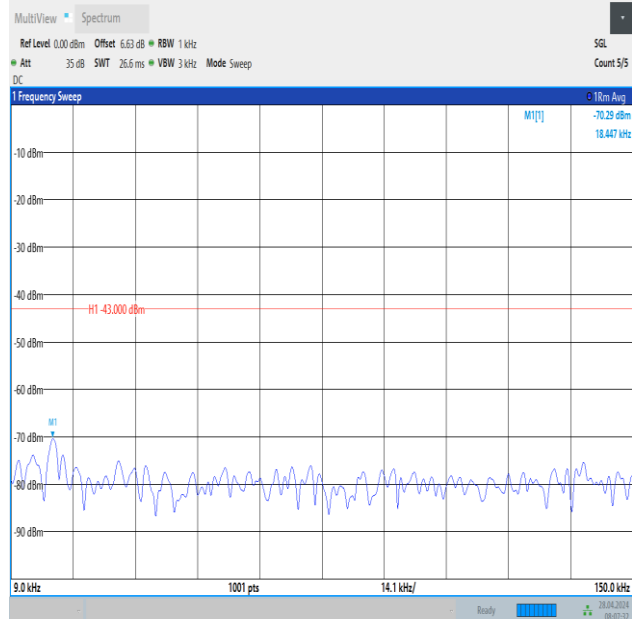
Band2_20MHz_16QAM_18900_1RB#99_0.009~0.15_0.009~0.15
