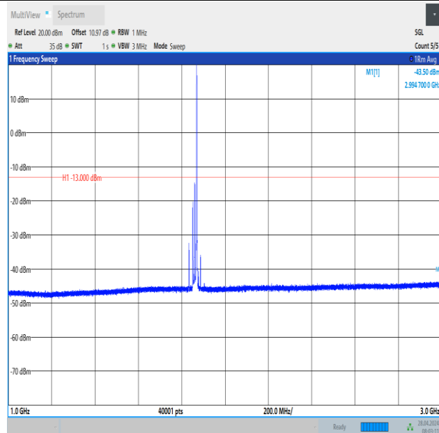
Band2_20MHz_QPSK_18700_1RB#99_1000~3000_1000~3000
