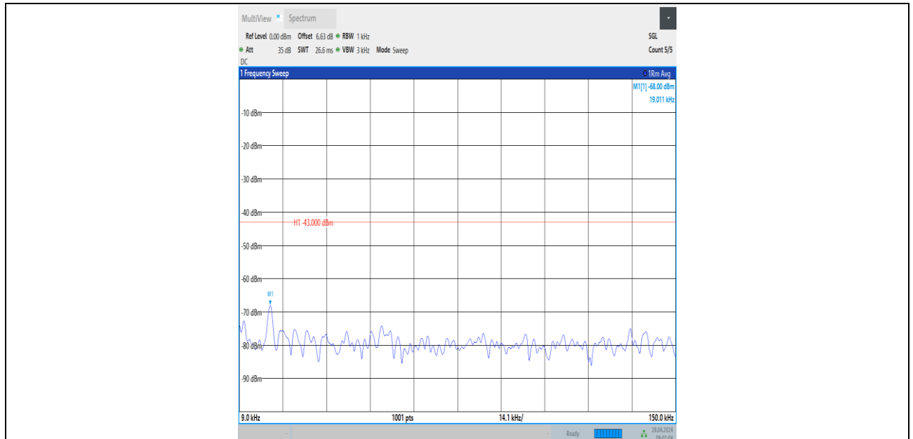
Band2_20MHz_QPSK_18700_1RB#0_0.009~0.15_0.009~0.15
