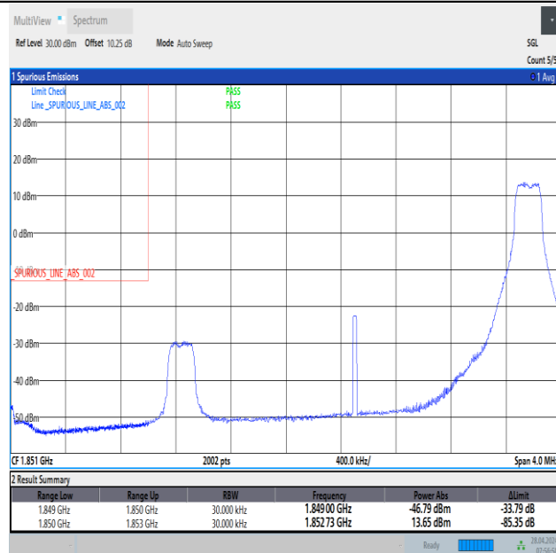
Band2_3MHz_16QAM_18615_1RB#14
