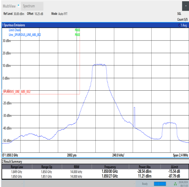
Band2_1.4MHz_QPSK_18607_1RB#0
