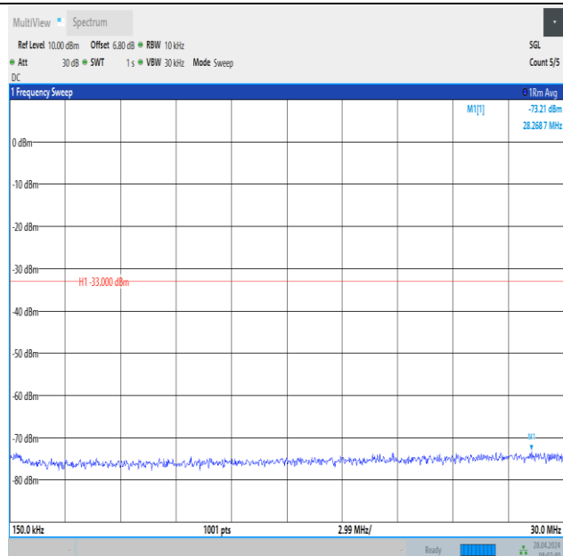
Band2_20MHz_16QAM_18900_1RB#99_0.15~30_0.15~30
