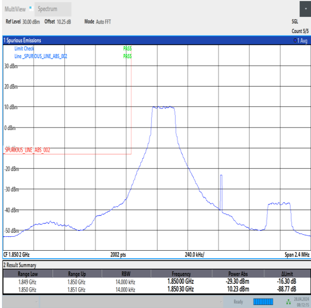
Band2_1.4MHz_16QAM_18607_1RB#0
