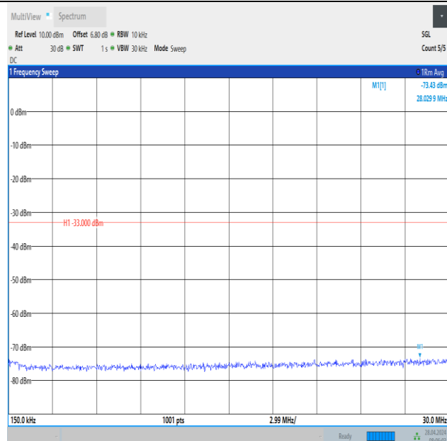
Band2_20MHz_16QAM_18900_1RB#0_0.15~30_0.15~30
