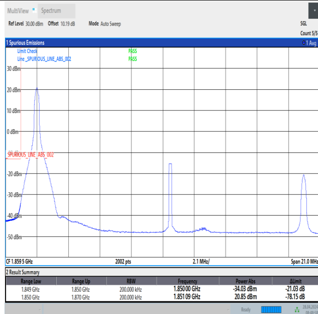
Band2_20MHz_16QAM_18700_1RB#0
