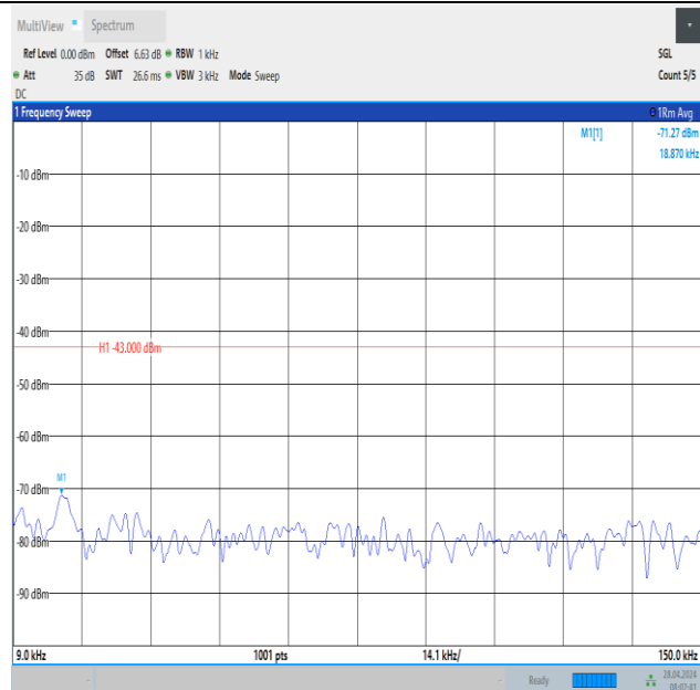
Band2_20MHz_QPSK_18700_1RB#99_0.009~0.15_0.009~0.15
