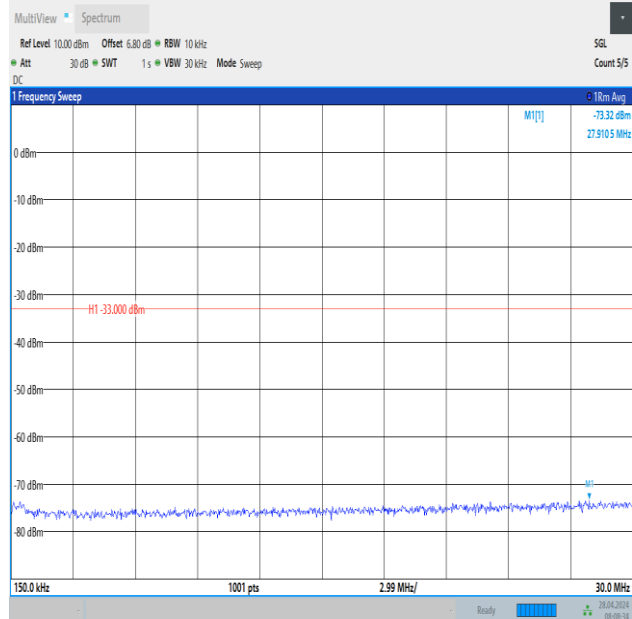
Band2_20MHz_QPSK_19100_1RB#0_0.15~30_0.15~30
