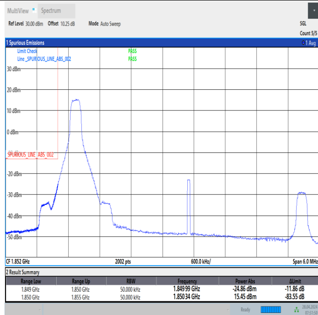
Band2_5MHz_16QAM_18625_1RB#0
