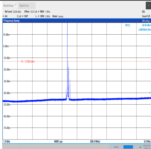
Band2_20MHz_QPSK_18900_1RB#0_1000~3000_1000~3000
