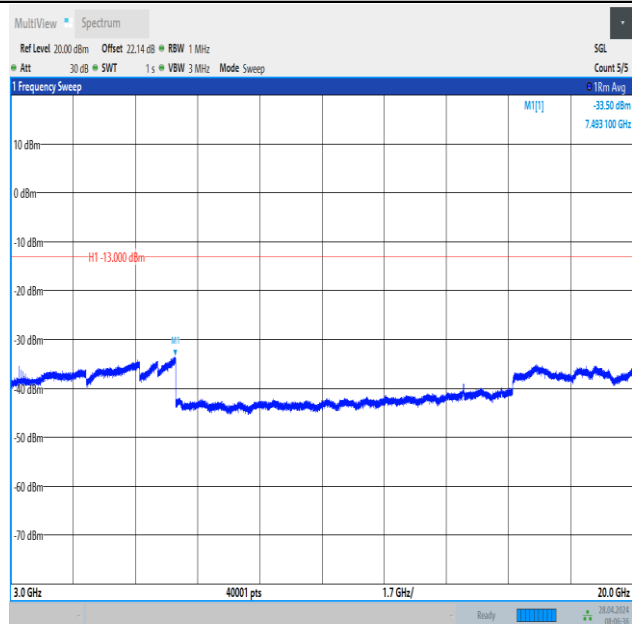
Band2_20MHz_16QAM_18900_1RB#0_3000~20000_3000~20000
