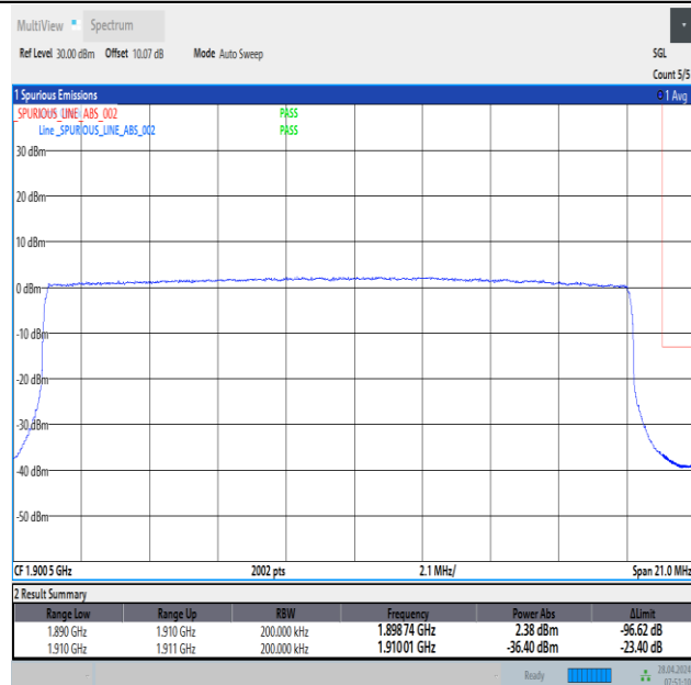
Band2_20MHz_QPSK_19100_100RB#0
