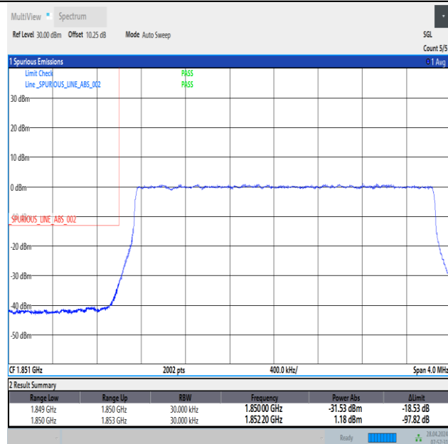
Band2_3MHz_16QAM_18615_15RB#0
