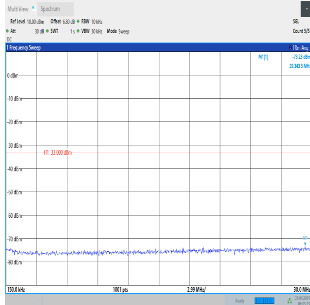
Band2_20MHz_QPSK_18900_1RB#0_0.15~30_0.15~30
