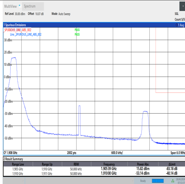
Band2_5MHz_16QAM_19175_1RB#0
