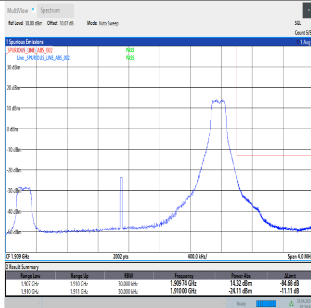
Band2_3MHz_16QAM_19185_1RB#14
