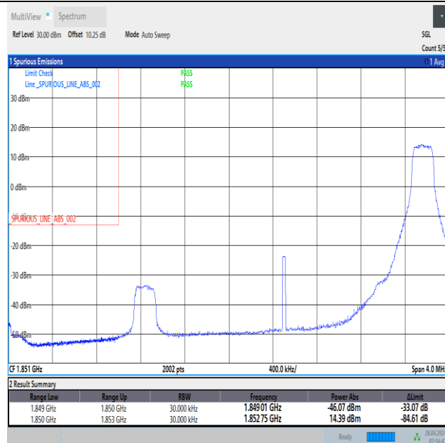
Band2_3MHz_QPSK_18615_1RB#14
