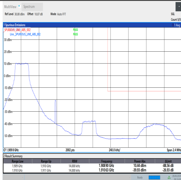
Band2_1.4MHz_16QAM_19193_1RB#0
