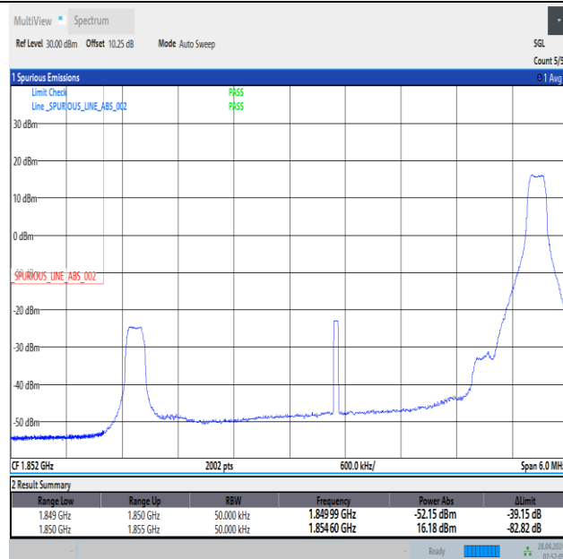
Band2_5MHz_QPSK_18625_1RB#24
