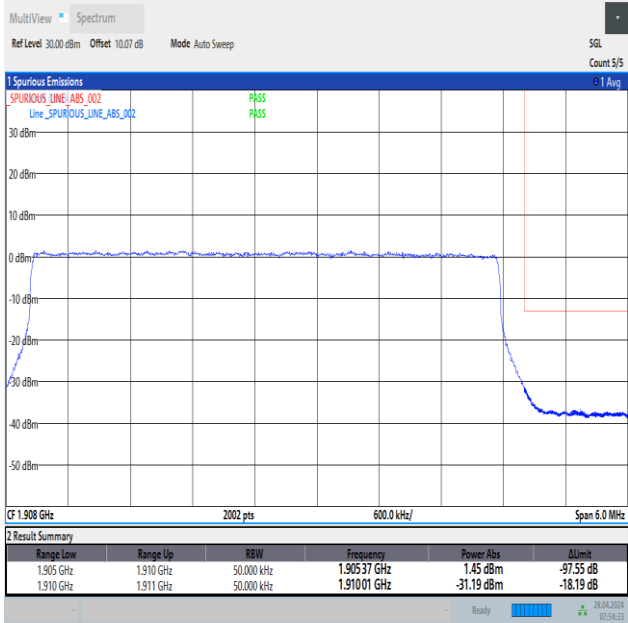
Band2_5MHz_16QAM_19175_25RB#0
