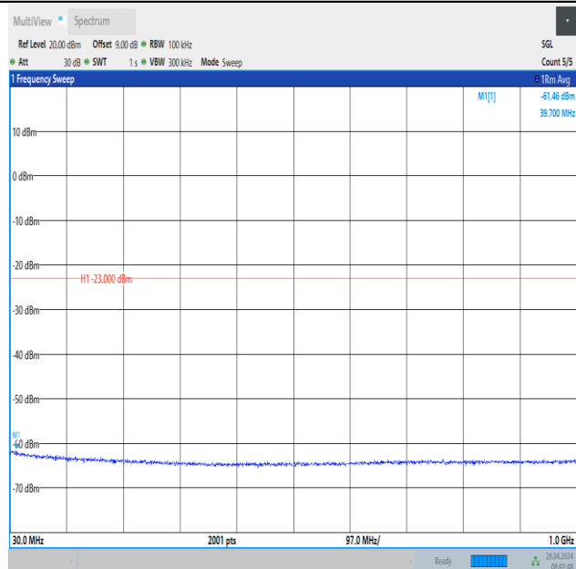
Band2_20MHz_16QAM_18900_1RB#99_30~1000_30~1000
