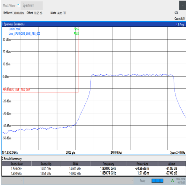
Band2_1.4MHz_16QAM_18607_6RB#0
