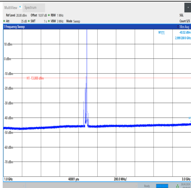
Band2_20MHz_16QAM_18900_1RB#99_1000~3000_1000~3000
