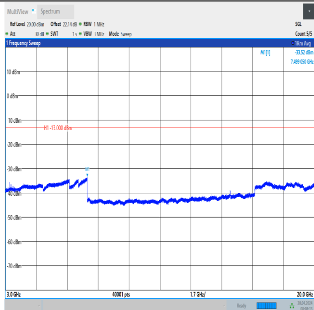
Band2_20MHz_16QAM_18900_1RB#99_3000~20000_3000~20000
