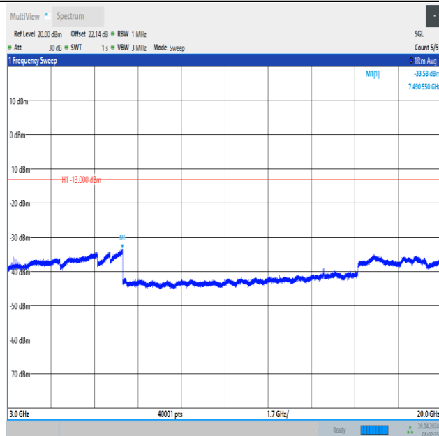
Band2_20MHz_16QAM_18700_1RB#0_3000~20000_3000~20000
