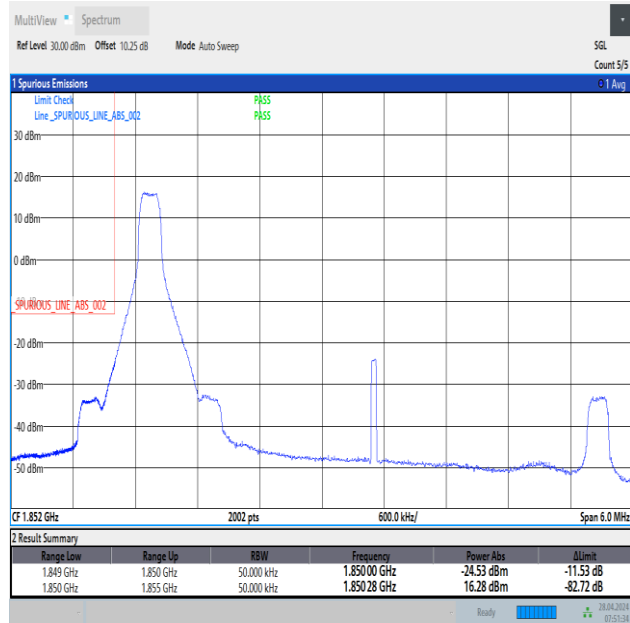
Band2_5MHz_QPSK_18625_1RB#0
