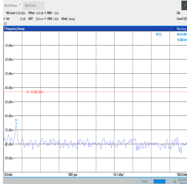
Band2_20MHz_16QAM_18700_1RB#99_0.009~0.15_0.009~0.15
