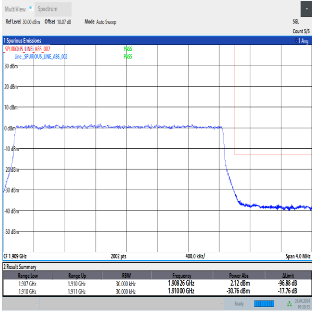
Band2_3MHz_16QAM_19185_15RB#0
