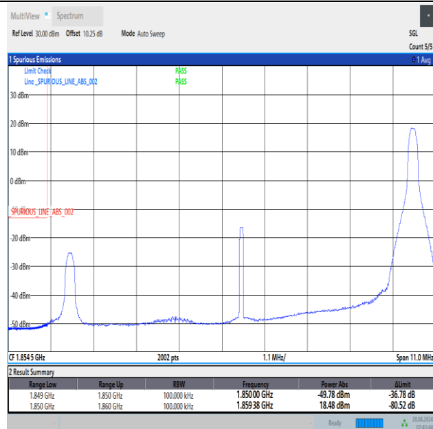
Band2_10MHz_16QAM_18650_1RB#49
