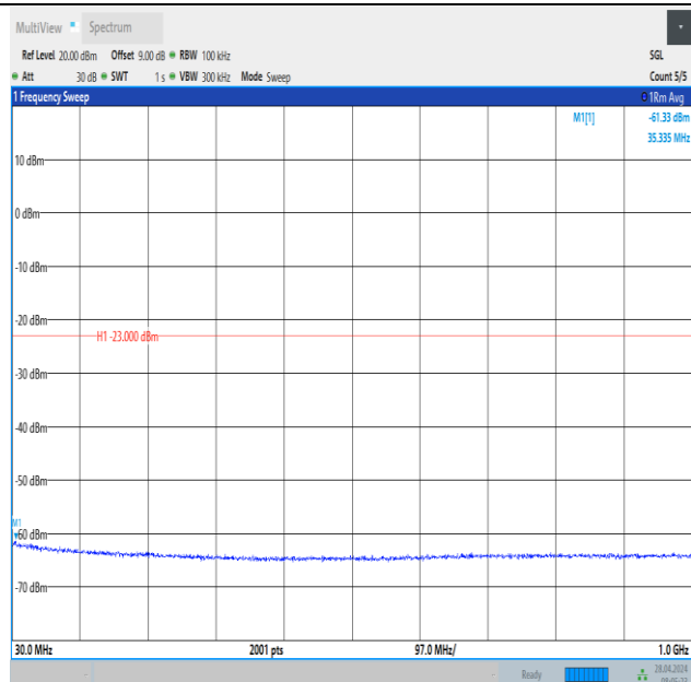
Band2_20MHz_QPSK_18900_1RB#0_30~1000_30~1000
