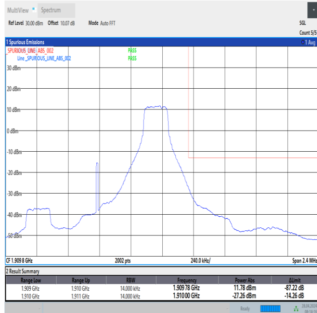
Band2_1.4MHz_QPSK_19193_1RB#5
