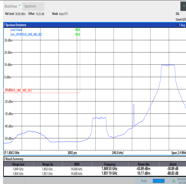
Band2_1.4MHz_16QAM_18607_1RB#5
