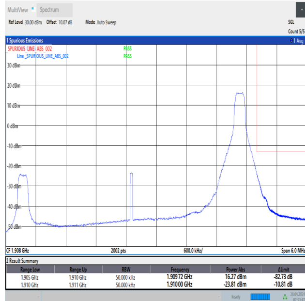
Band2_5MHz_QPSK_19175_1RB#24
