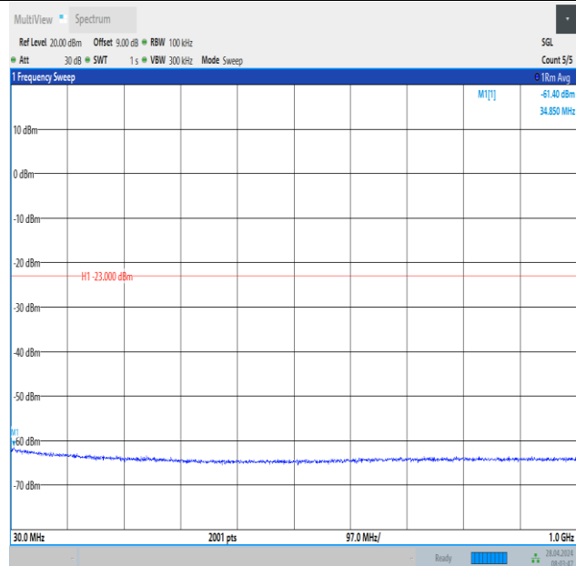
Band2_20MHz_16QAM_18700_1RB#99_30~1000_30~1000
