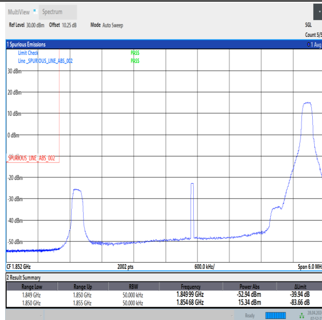
Band2_5MHz_16QAM_18625_1RB#24
