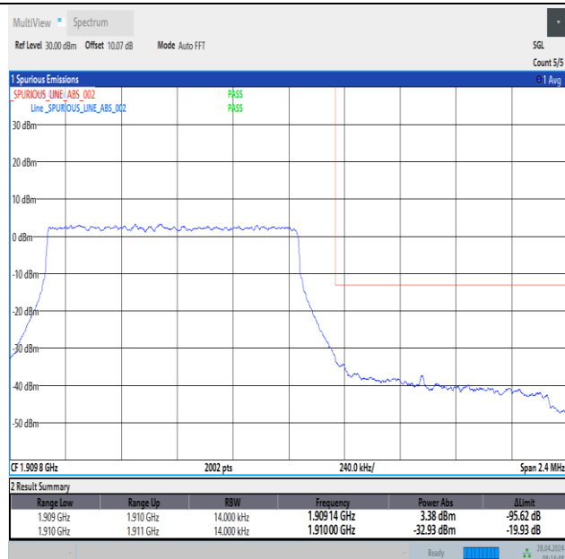
Band2_1.4MHz_QPSK_19193_6RB#0
