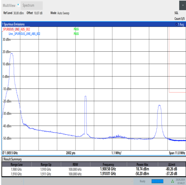
Band2_10MHz_16QAM_19150_1RB#0
