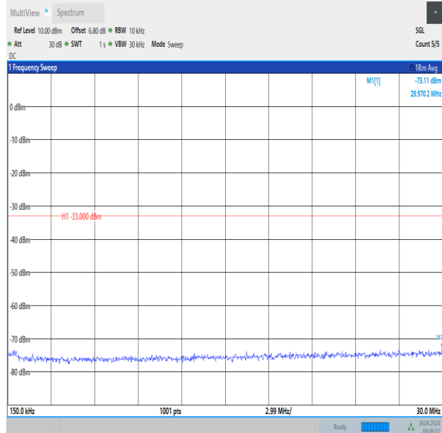
Band2_20MHz_QPSK_18900_1RB#99_0.15~30_0.15~30
