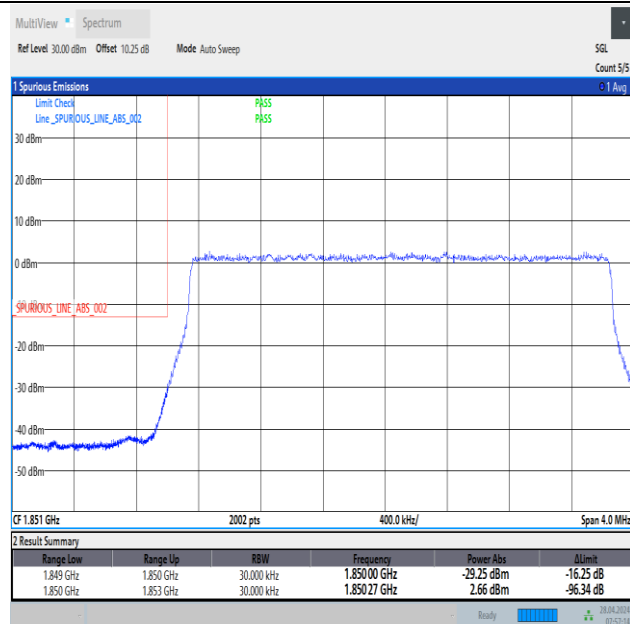
Band2_3MHz_QPSK_18615_15RB#0
