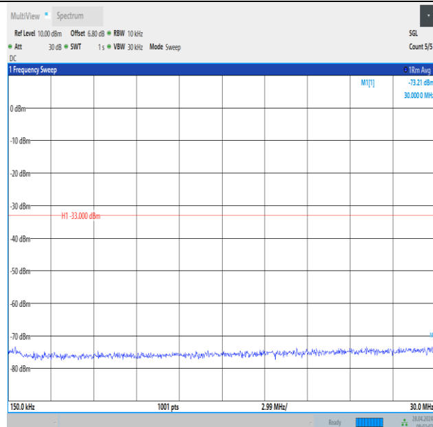
Band2_20MHz_16QAM_18700_1RB#0_0.15~30_0.15~30
