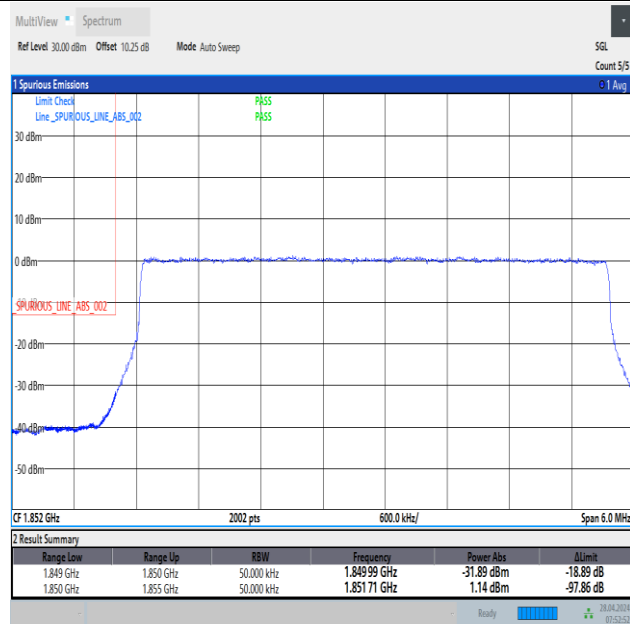
Band2_5MHz_16QAM_18625_25RB#0
