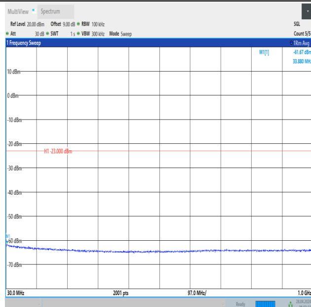
Band2_20MHz_16QAM_18700_1RB#0_30~1000_30~1000
