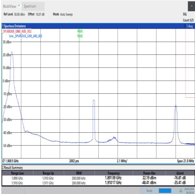
Band2_20MHz_QPSK_19100_1RB#0
