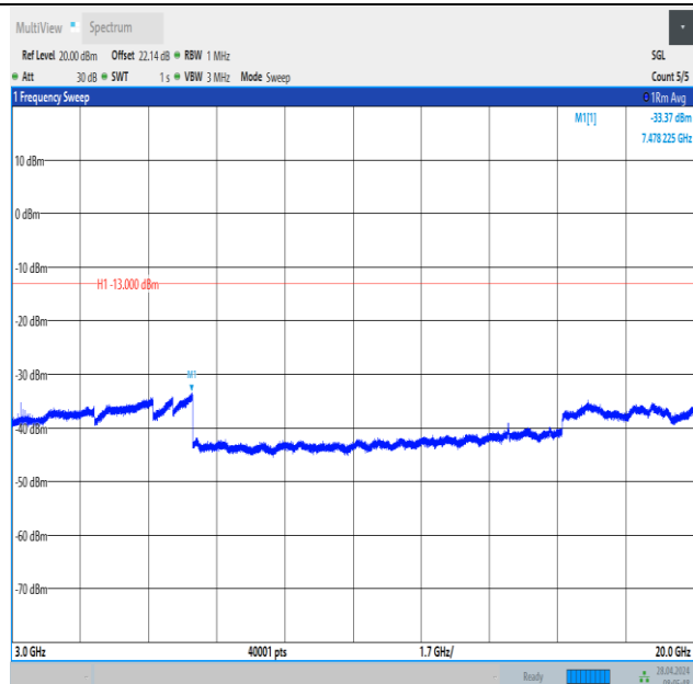
Band2_20MHz_QPSK_18900_1RB#0_3000~20000_3000~20000
