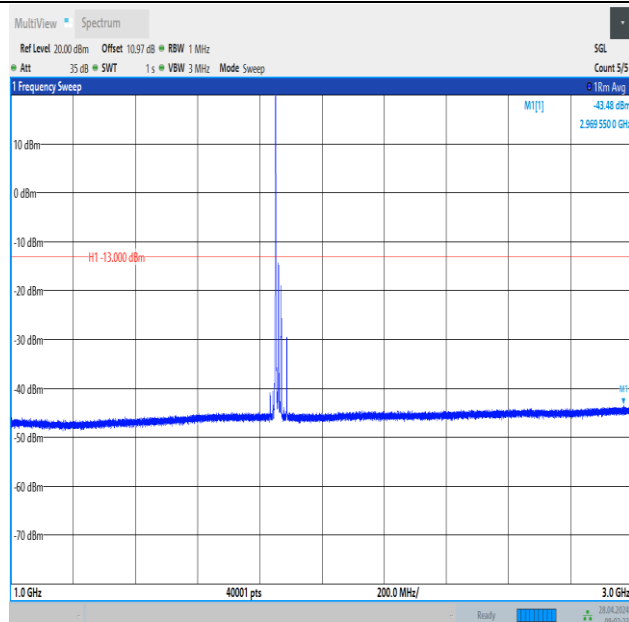
Band2_20MHz_16QAM_18700_1RB#0_1000~3000_1000~3000
