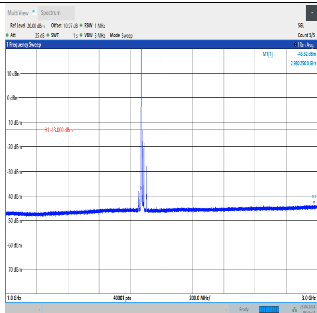
Band2_20MHz_16QAM_18900_1RB#0_1000~3000_1000~3000
