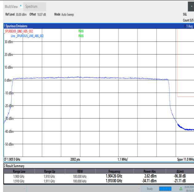
Band2_10MHz_QPSK_19150_50RB#0
