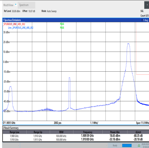
Band2_10MHz_16QAM_19150_1RB#49
