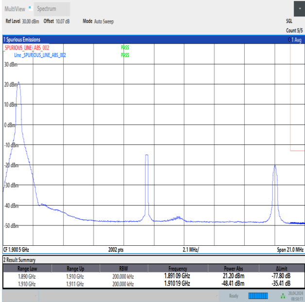
Band2_20MHz_16QAM_19100_1RB#0
