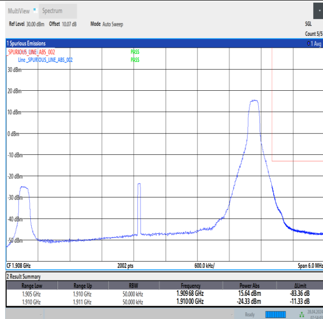
Band2_5MHz_16QAM_19175_1RB#24
