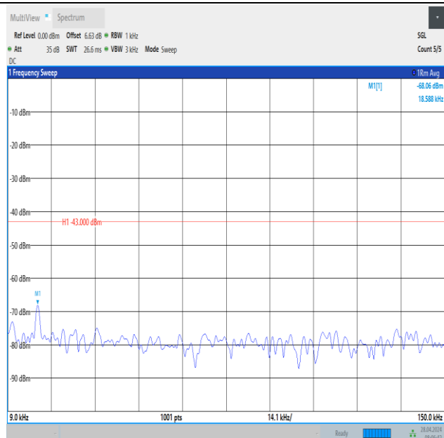
Band2_20MHz_QPSK_18900_1RB#99_0.009~0.15_0.009~0.15
