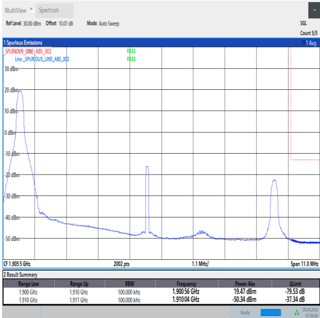
Band2_10MHz_QPSK_19150_1RB#0
