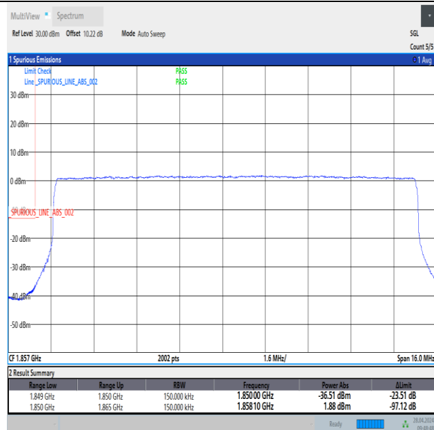
Band2_15MHz_QPSK_18675_75RB#0
