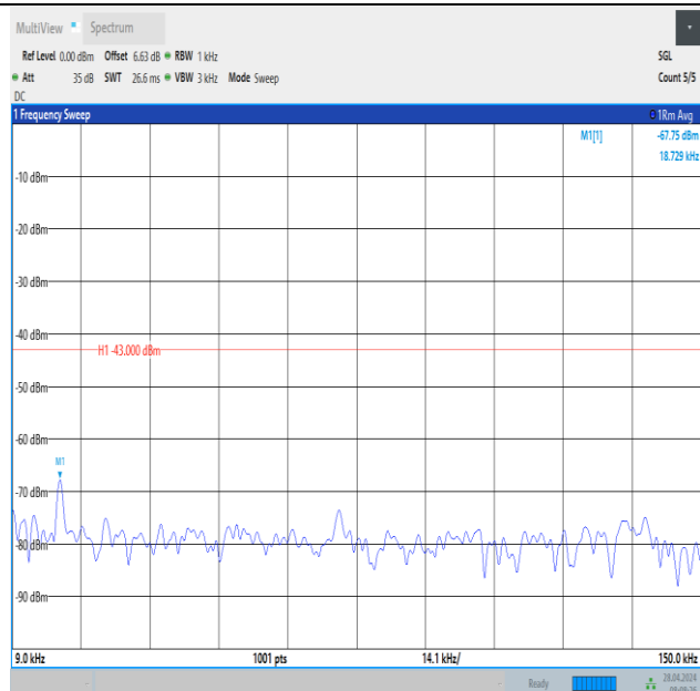
Band2_20MHz_QPSK_19100_1RB#0_0.009~0.15_0.009~0.15
