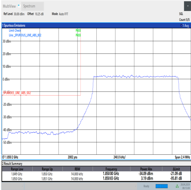
Band2_1.4MHz_QPSK_18607_6RB#0
