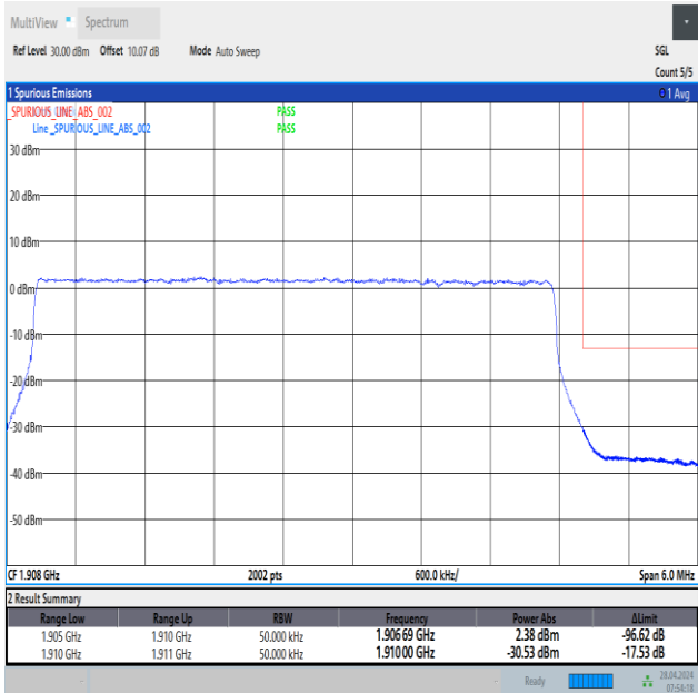
Band2_5MHz_QPSK_19175_25RB#0
