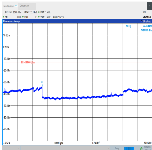
Band2_20MHz_QPSK_18900_1RB#99_3000~20000_3000~20000
