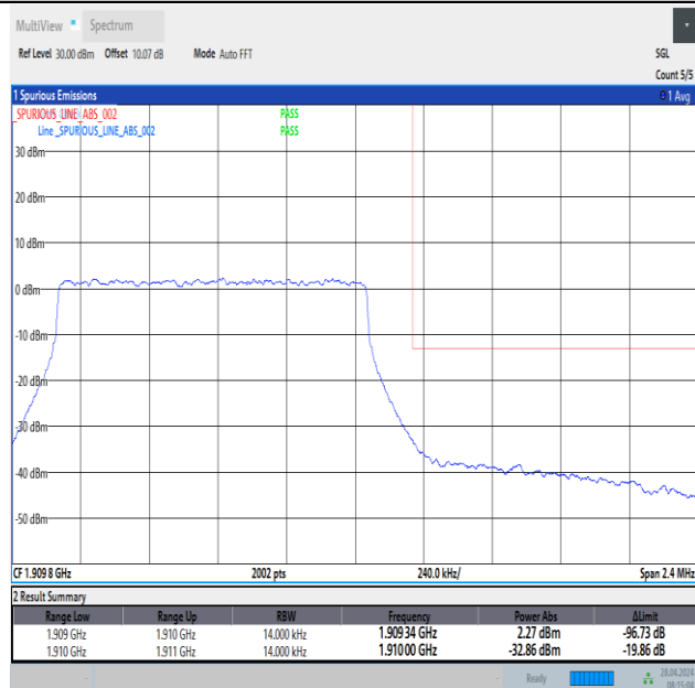
Band2_1.4MHz_16QAM_19193_6RB#0
