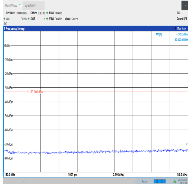
Band2_20MHz_QPSK_18700_1RB#99_0.15~30_0.15~30
