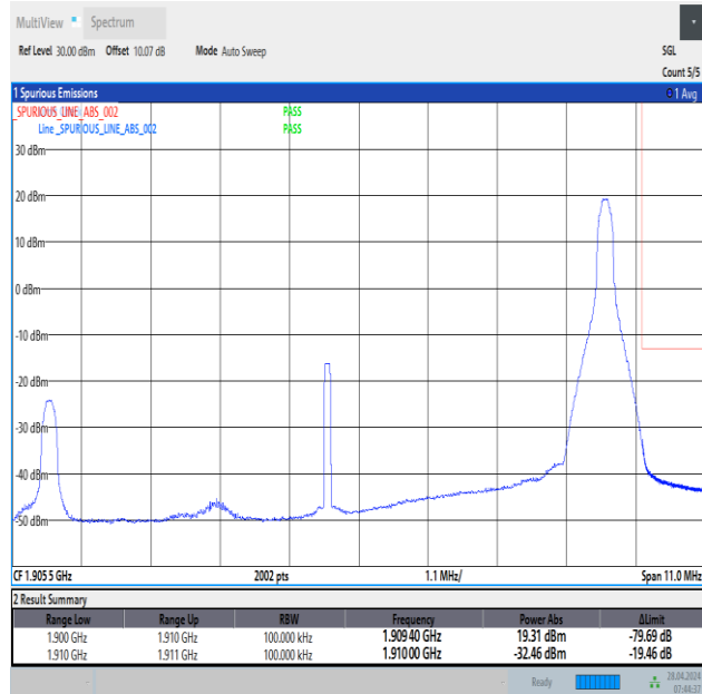
Band2_10MHz_QPSK_19150_1RB#49
