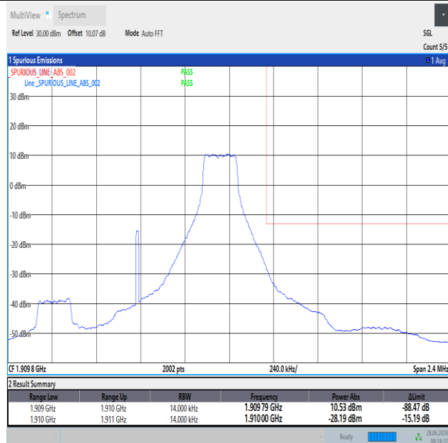
Band2_1.4MHz_16QAM_19193_1RB#5
