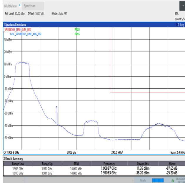
Band2_1.4MHz_QPSK_19193_1RB#0
