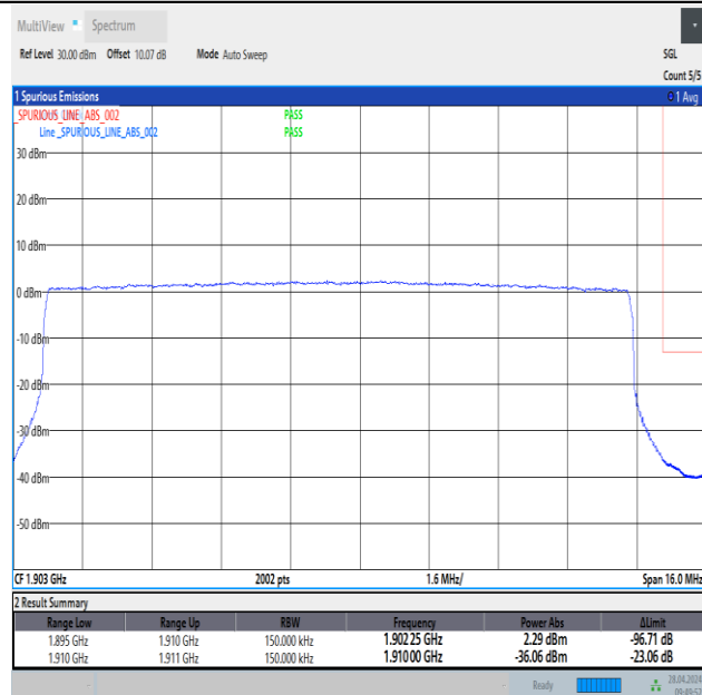
Band2_15MHz_QPSK_19125_75RB#0
