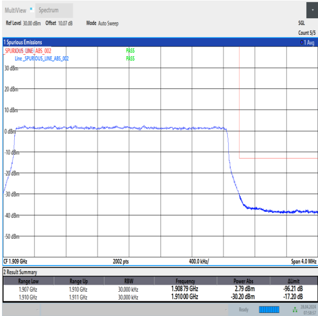
Band2_3MHz_QPSK_19185_15RB#0
