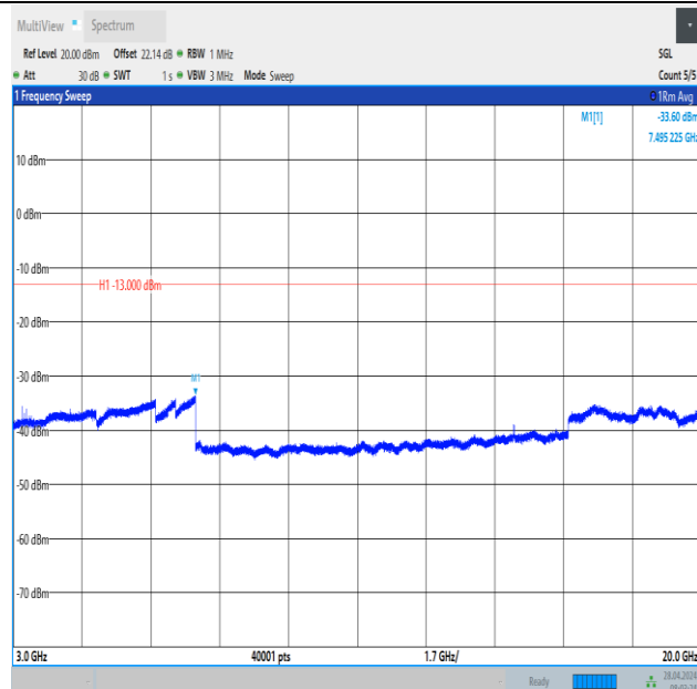
Band2_20MHz_QPSK_18700_1RB#99_3000~20000_3000~20000
