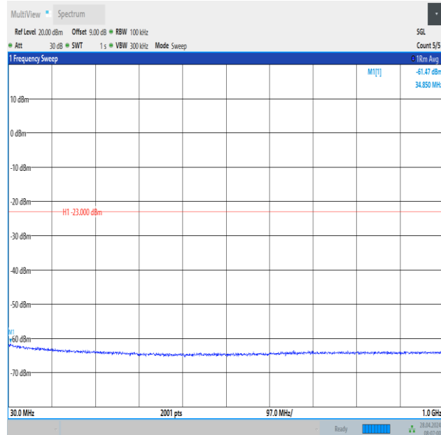
Band2_20MHz_QPSK_18900_1RB#99_30~1000_30~1000
