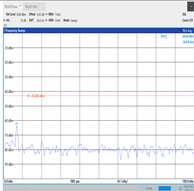
Band2_20MHz_16QAM_18900_1RB#0_0.009~0.15_0.009~0.15
