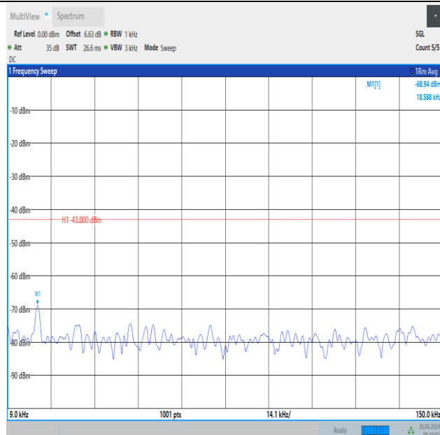
Band2_20MHz_QPSK_19100_1RB#99_0.009~0.15_0.009~0.15
