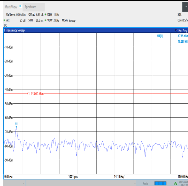
Band2_15MHz_QPSK_19125_75RB#0_0.009~0.15_0.009~0.15
