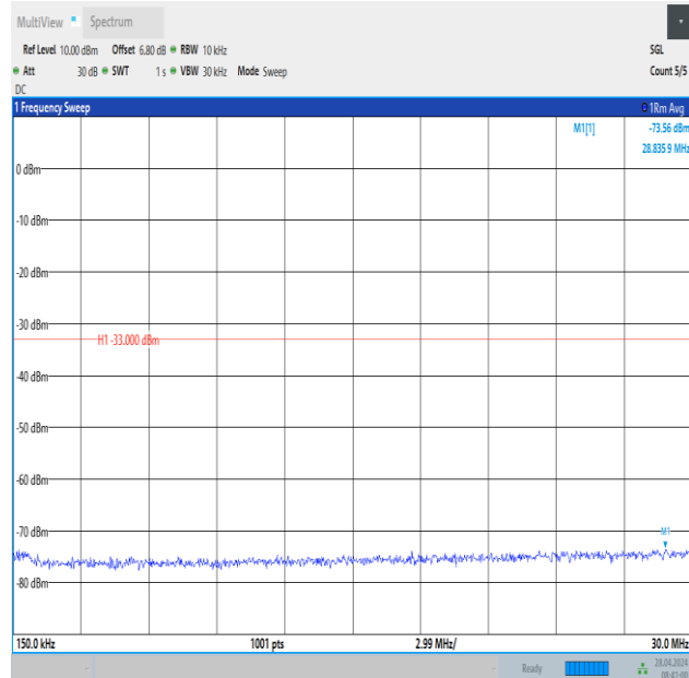
Band2_20MHz_QPSK_19100_100RB#0_0.15~30_0.15~30
