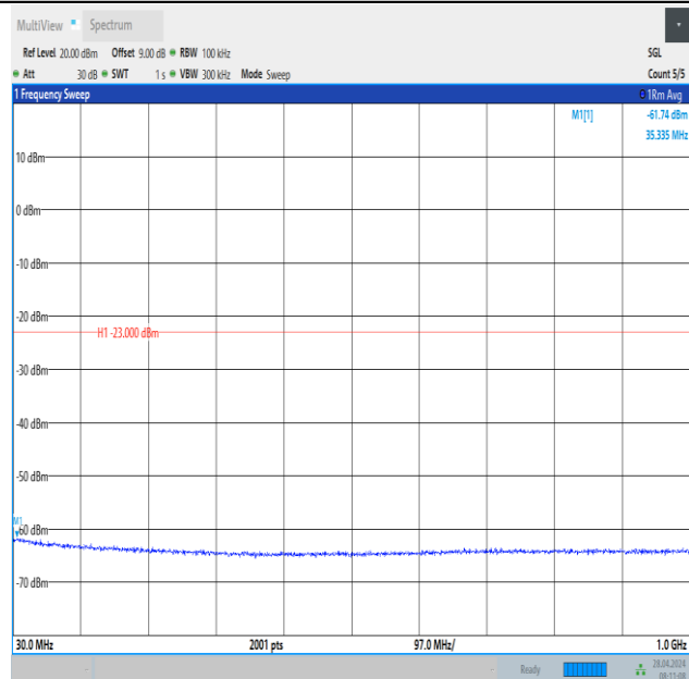
Band2_20MHz_16QAM_19100_1RB#99_30~1000_30~1000
