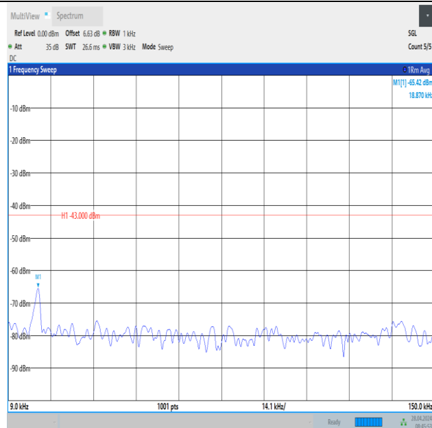
Band2_15MHz_QPSK_18675_75RB#0_0.009~0.15_0.009~0.15
