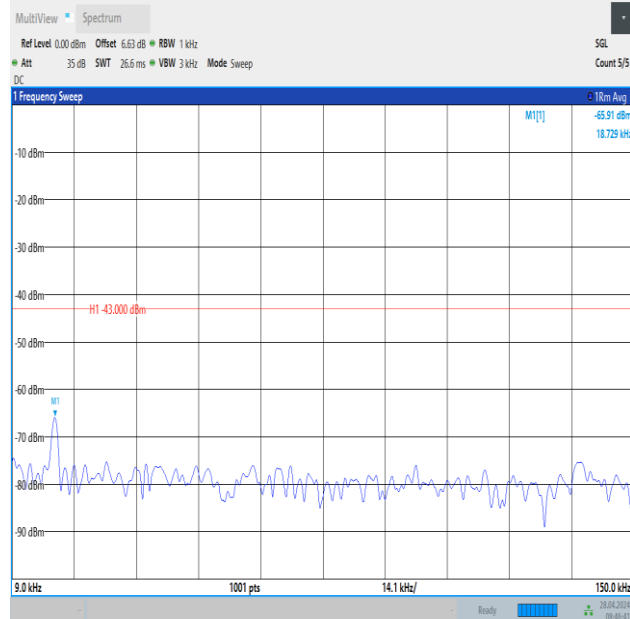
Band2_15MHz_QPSK_18900_75RB#0_0.009~0.15_0.009~0.15
