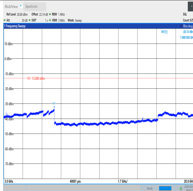
Band2_15MHz_QPSK_18900_75RB#0_3000~20000_3000~20000
