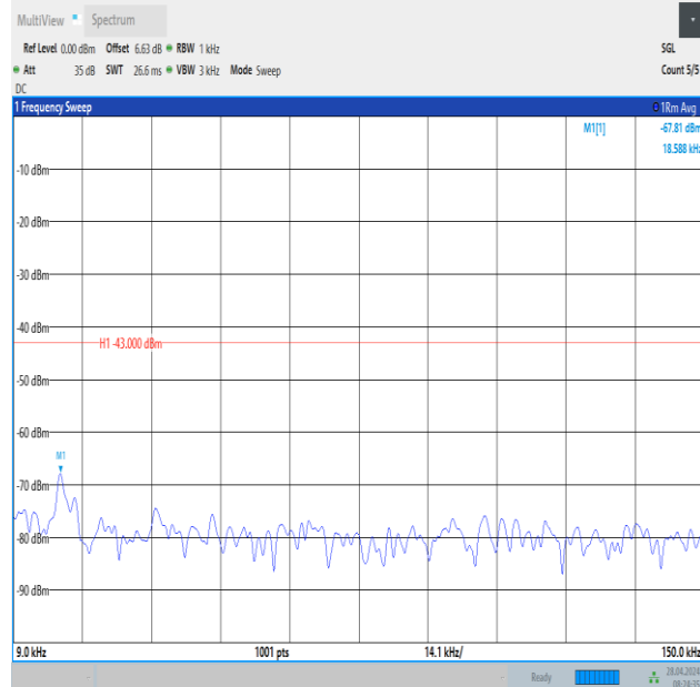
Band2_10MHz_QPSK_18900_50RB#0_0.009~0.15_0.009~0.15
