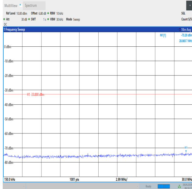
Band2_20MHz_QPSK_19100_1RB#99_0.15~30_0.15~30
