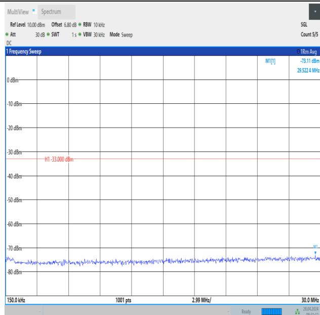
Band2_10MHz_QPSK_18900_1RB#49_0.15~30_0.15~30
