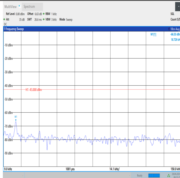
Band2_10MHz_QPSK_19150_50RB#0_0.009~0.15_0.009~0.15
