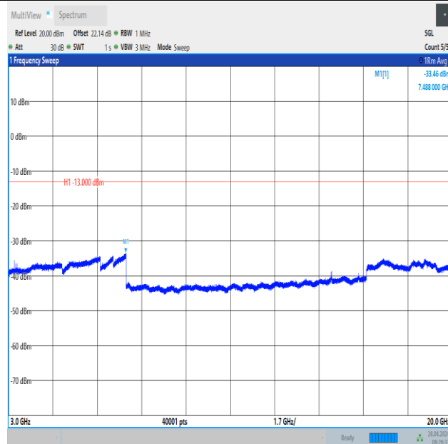
Band2_10MHz_QPSK_18650_1RB#49_3000~20000_3000~20000
