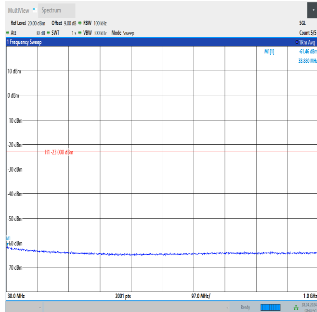
Band2_15MHz_QPSK_19125_75RB#0_30~1000_30~1000
