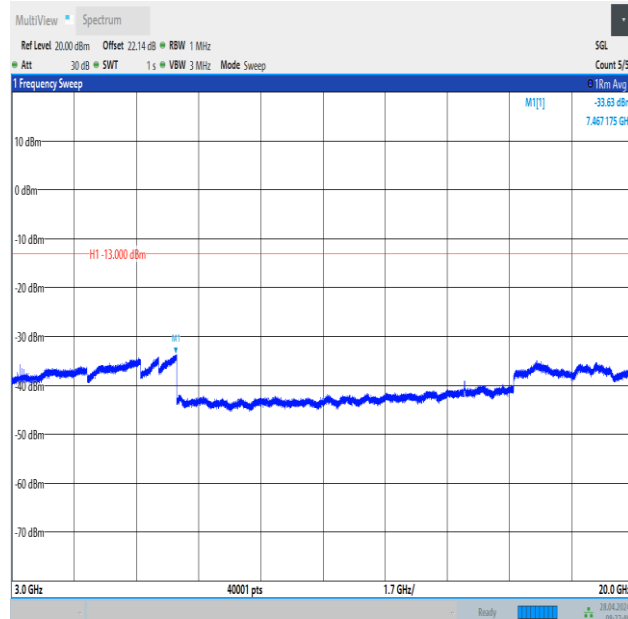
Band2_10MHz_16QAM_18650_1RB#0_3000~20000_3000~20000
