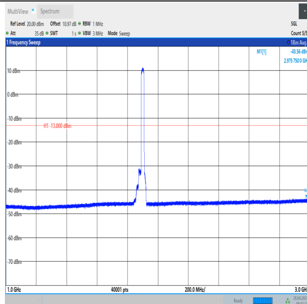
Band2_20MHz_QPSK_19100_100RB#0_1000~3000_1000~3000
