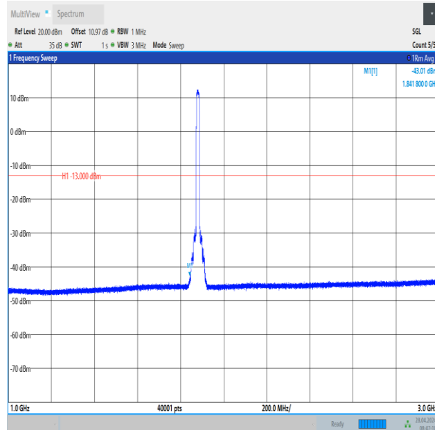
Band2_15MHz_QPSK_18900_75RB#0_1000~3000_1000~3000
