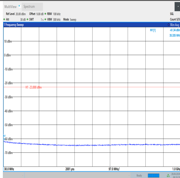
Band2_20MHz_QPSK_19100_1RB#99_30~1000_30~1000
