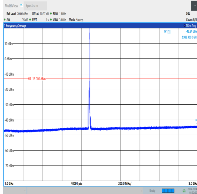
Band2_10MHz_16QAM_18900_1RB#49_1000~3000_1000~3000
