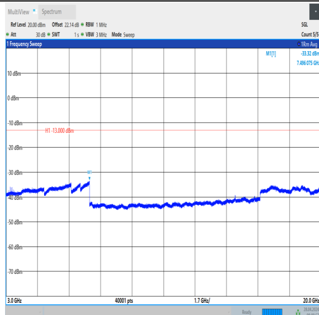
Band2_20MHz_16QAM_19100_1RB#0_3000~20000_3000~20000
