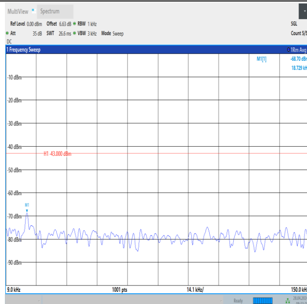
Band2_10MHz_16QAM_19150_1RB#0_0.009~0.15_0.009~0.15
