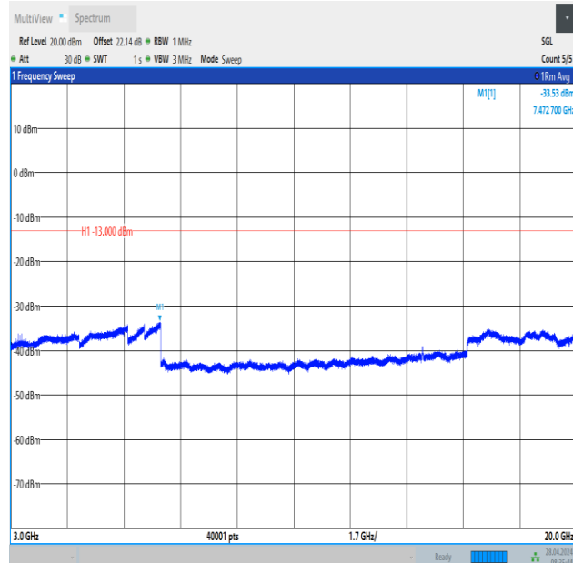
Band2_10MHz_16QAM_19150_1RB#49_3000~20000_3000~20000
