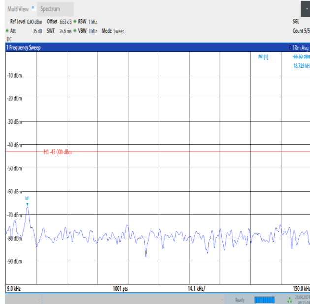
Band2_10MHz_QPSK_18900_1RB#49_0.009~0.15_0.009~0.15
