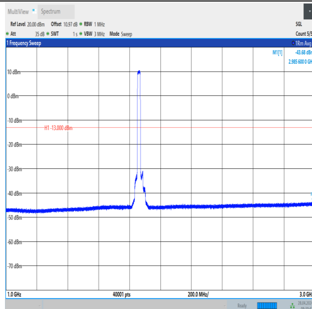
Band2_20MHz_QPSK_18700_100RB#0_1000~3000_1000~3000
