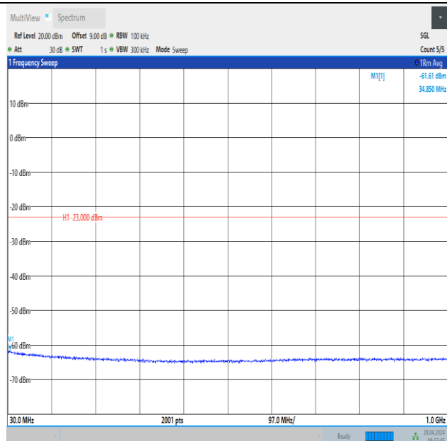
Band2_10MHz_16QAM_19150_1RB#0_30~1000_30~1000
