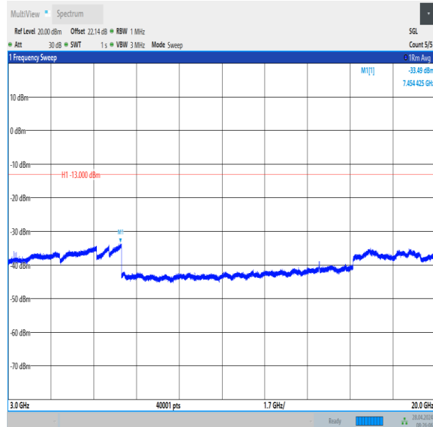
Band2_10MHz_QPSK_19150_50RB#0_3000~20000_3000~20000
