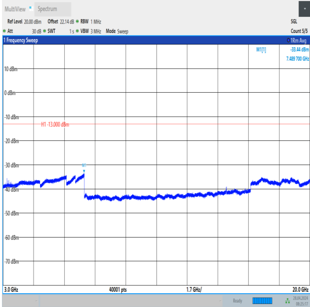
Band2_10MHz_QPSK_18900_50RB#0_3000~20000_3000~20000
