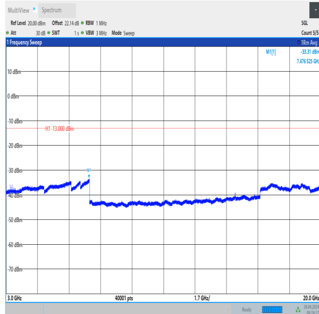
Band2_10MHz_QPSK_18650_50RB#0_3000~20000_3000~20000
