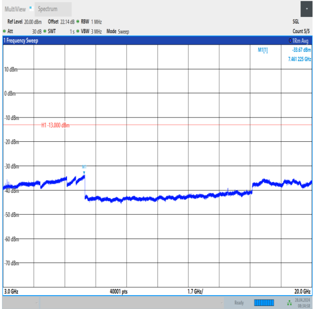
Band2_10MHz_QPSK_19150_1RB#49_3000~20000_3000~20000
