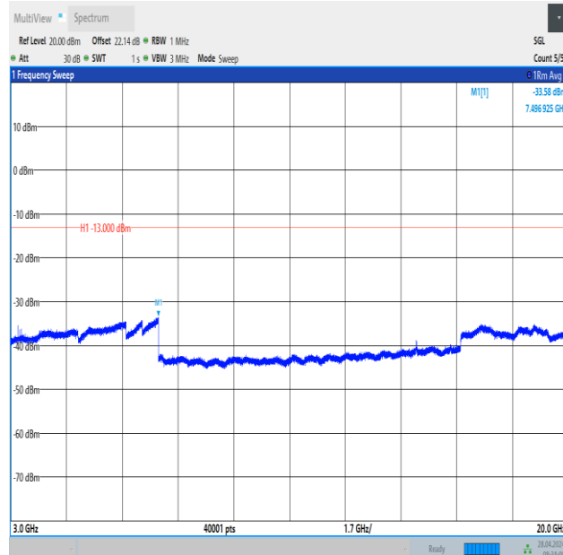
Band2_10MHz_16QAM_19150_1RB#0_3000~20000_3000~20000
