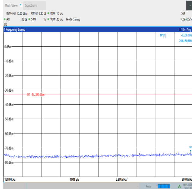
Band2_15MHz_QPSK_19125_75RB#0_0.15~30_0.15~30
