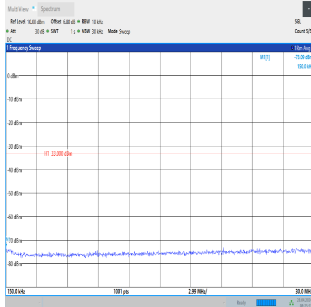
Band2_10MHz_QPSK_19150_50RB#0_0.15~30_0.15~30
