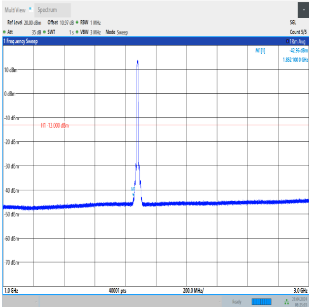
Band2_10MHz_QPSK_18900_50RB#0_1000~3000_1000~3000
