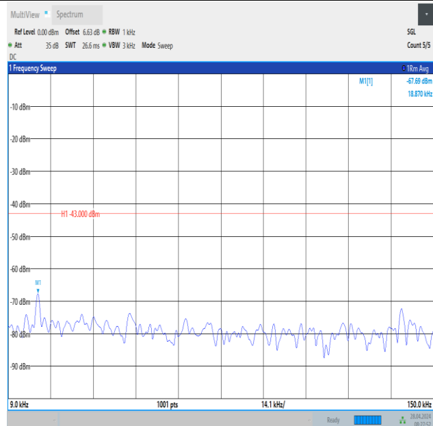
Band2_10MHz_QPSK_18650_1RB#49_0.009~0.15_0.009~0.15
