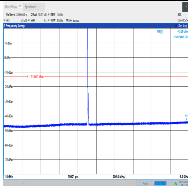
Band2_5MHz_16QAM_19175_1RB#0_1000~3000_1000~3000
