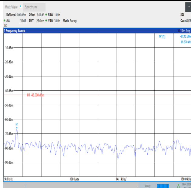
Band2_3MHz_16QAM_18900_1RB#14_0.009~0.15_0.009~0.15
