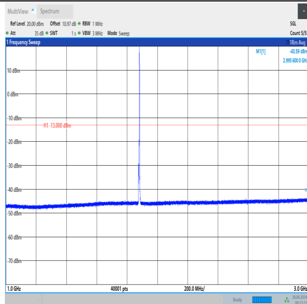
Band2_3MHz_16QAM_18900_1RB#14_1000~3000_1000~3000
