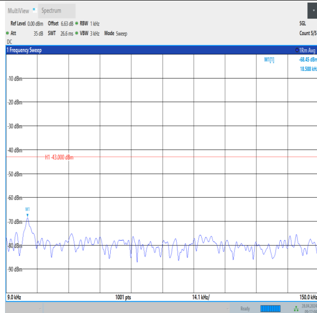
Band2_3MHz_QPSK_18615_1RB#14_0.009~0.15_0.009~0.15
