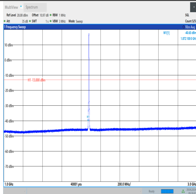
Band2_3MHz_16QAM_18900_15RB#0_1000~3000_1000~3000
