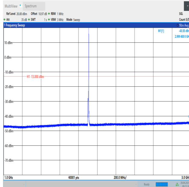
Band2_5MHz_QPSK_19175_1RB#24_1000~3000_1000~3000
