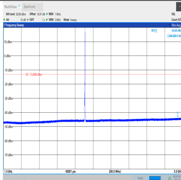
Band2_3MHz_QPSK_19185_1RB#14_1000~3000_1000~3000
