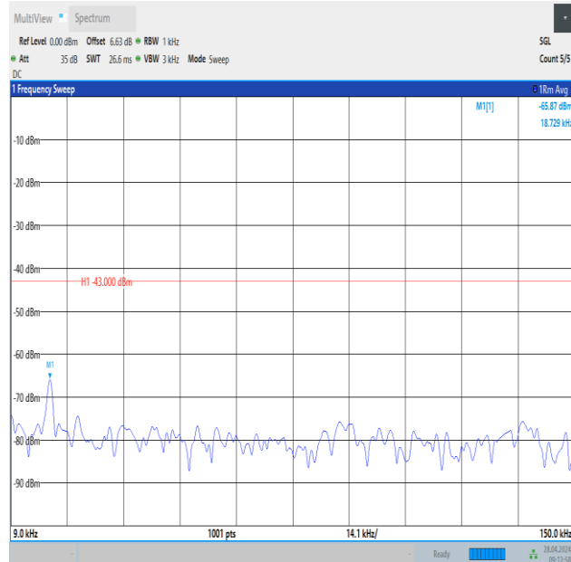
Band2_5MHz_16QAM_19175_1RB#24_0.009~0.15_0.009~0.15
