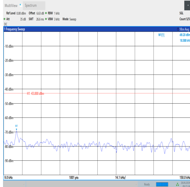
Band2_3MHz_QPSK_18900_1RB#14_0.009~0.15_0.009~0.15
