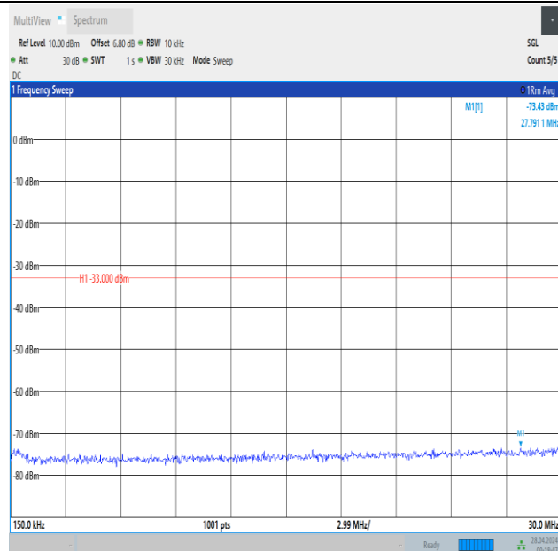
Band2_3MHz_QPSK_18615_15RB#0_0.15~30_0.15~30
