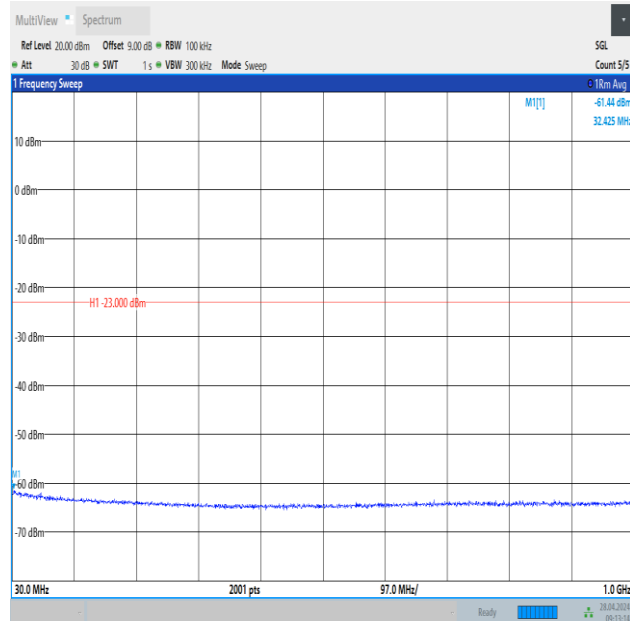
Band2_5MHz_16QAM_19175_1RB#24_30~1000_30~1000
