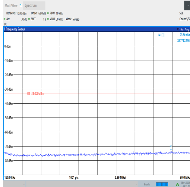
Band2_3MHz_16QAM_18900_1RB#0_0.15~30_0.15~30
