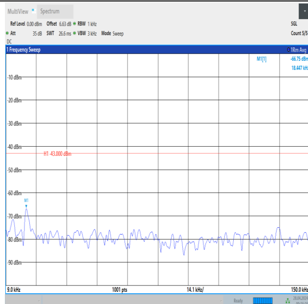
Band2_3MHz_16QAM_18615_1RB#0_0.009~0.15_0.009~0.15
