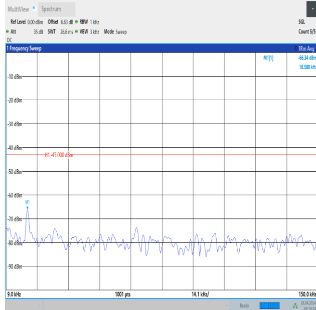
Band2_3MHz_QPSK_18615_15RB#0_0.009~0.15_0.009~0.15
