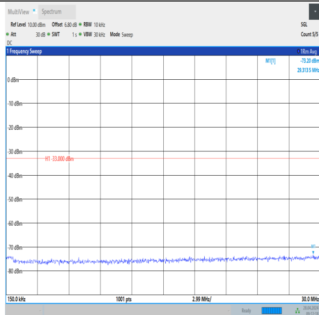
Band2_5MHz_QPSK_19175_1RB#24_0.15~30_0.15~30
