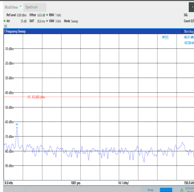
Band2_3MHz_16QAM_18900_15RB#0_0.009~0.15_0.009~0.15
