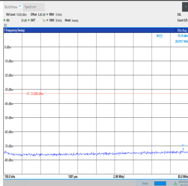
Band2_5MHz_QPSK_19175_25RB#0_0.15~30_0.15~30
