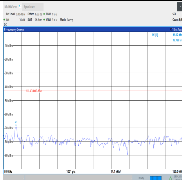
Band2_3MHz_16QAM_18615_15RB#0_0.009~0.15_0.009~0.15
