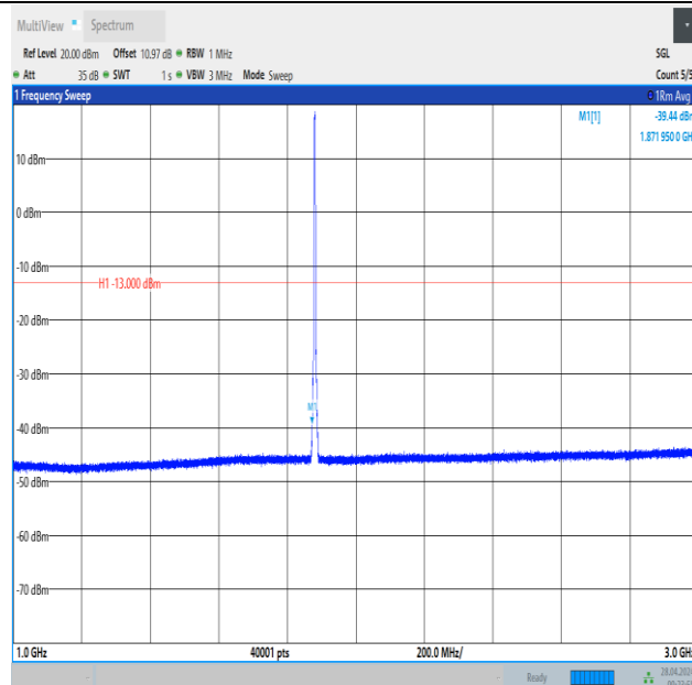
Band2_3MHz_QPSK_18900_15RB#0_1000~3000_1000~3000
