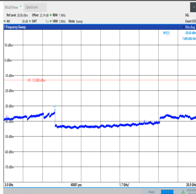
Band2_5MHz_16QAM_19175_25RB#0_3000~20000_3000~20000
