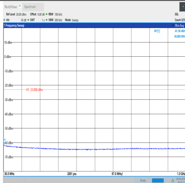
Band2_3MHz_16QAM_19185_1RB#0_30~1000_30~1000
