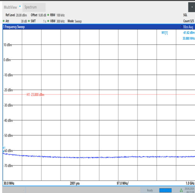
Band2_3MHz_QPSK_18615_1RB#14_30~1000_30~1000
