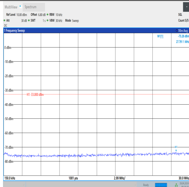
Band2_3MHz_QPSK_18900_1RB#0_0.15~30_0.15~30
