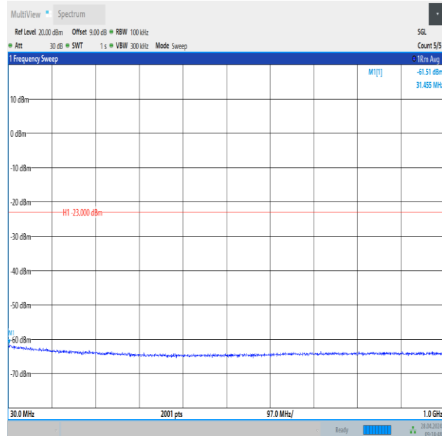
Band2_5MHz_16QAM_19175_25RB#0_30~1000_30~1000
