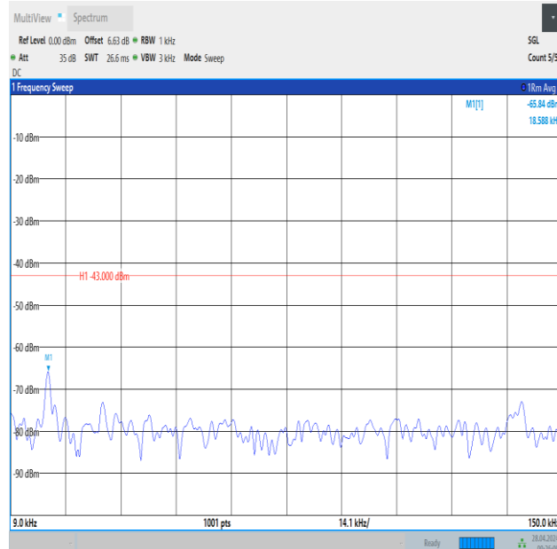
Band2_3MHz_16QAM_19185_1RB#0_0.009~0.15_0.009~0.15
