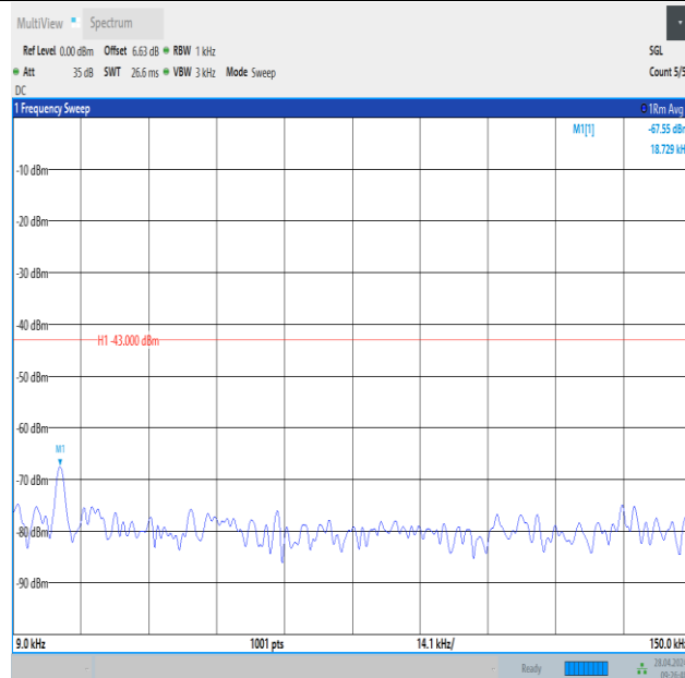
Band2_3MHz_QPSK_19185_1RB#14_0.009~0.15_0.009~0.15
