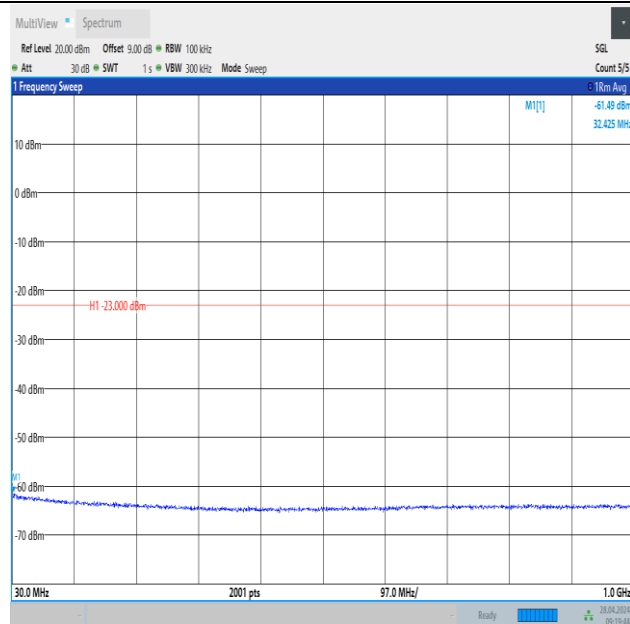
Band2_3MHz_16QAM_18615_15RB#0_30~1000_30~1000
