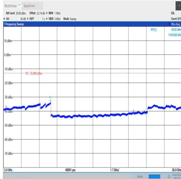
Band2_5MHz_16QAM_18900_25RB#0_3000~20000_3000~20000
