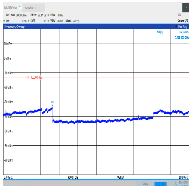
Band2_3MHz_16QAM_18615_15RB#0_3000~20000_3000~20000
