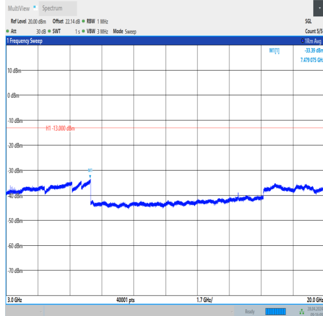
Band2_3MHz_QPSK_18615_1RB#0_3000~20000_3000~20000
