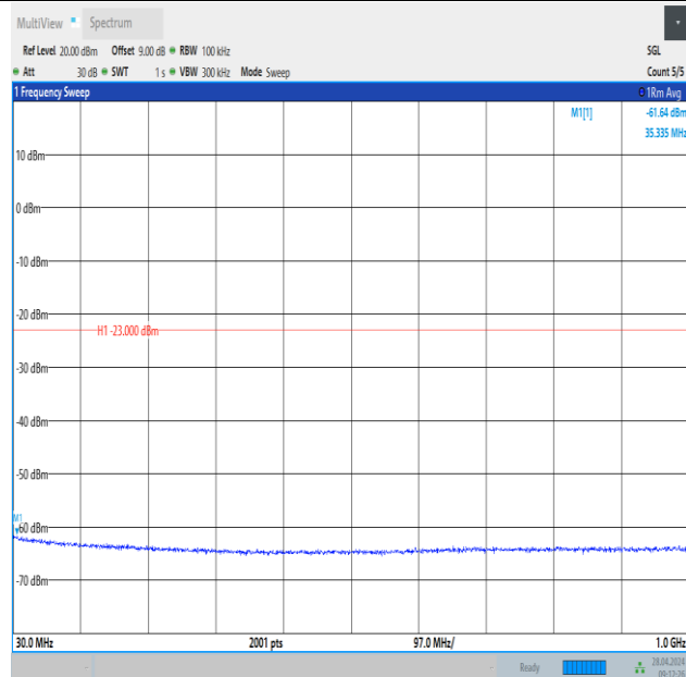
Band2_5MHz_QPSK_19175_1RB#24_30~1000_30~1000
