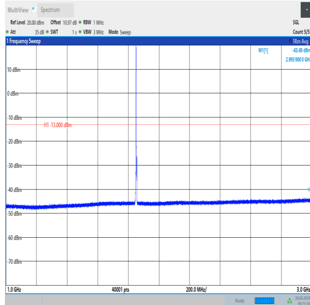
Band2_3MHz_QPSK_18615_1RB#0_1000~3000_1000~3000
