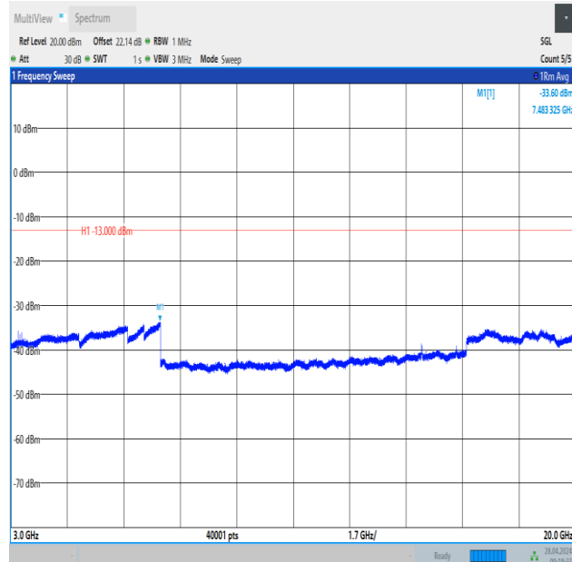
Band2_3MHz_16QAM_18615_1RB#14_3000~20000_3000~20000
