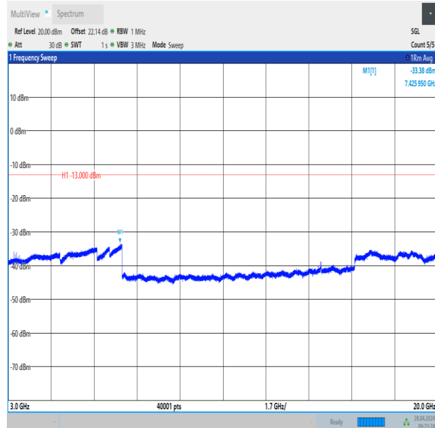
Band2_3MHz_16QAM_18900_1RB#14_3000~20000_3000~20000
