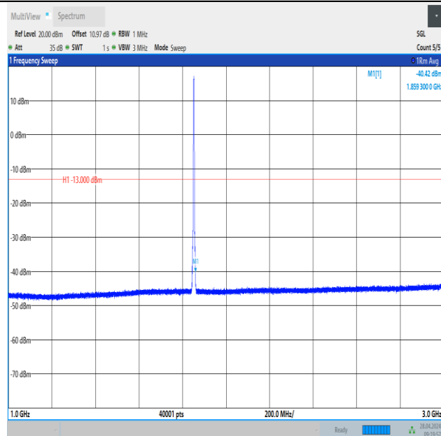
Band2_3MHz_16QAM_18615_15RB#0_1000~3000_1000~3000
