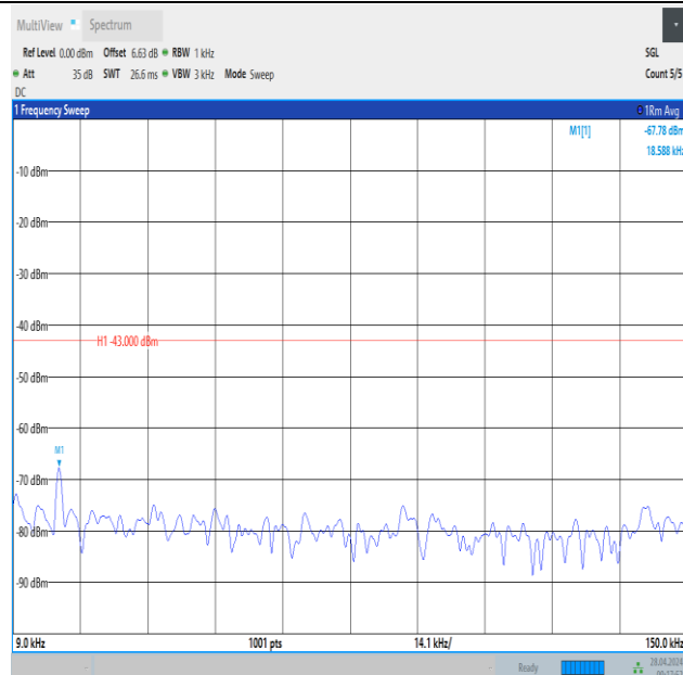
Band2_3MHz_16QAM_18615_1RB#14_0.009~0.15_0.009~0.15
