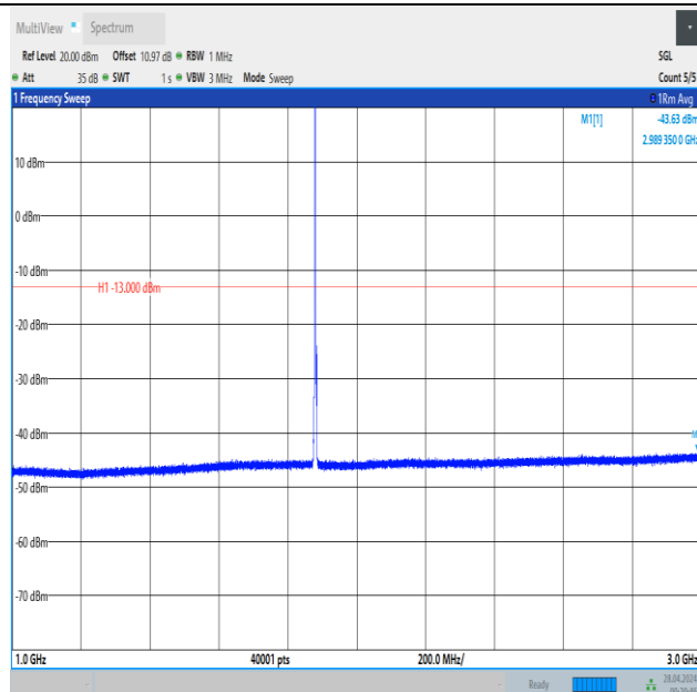
Band2_3MHz_QPSK_18900_1RB#0_1000~3000_1000~3000
