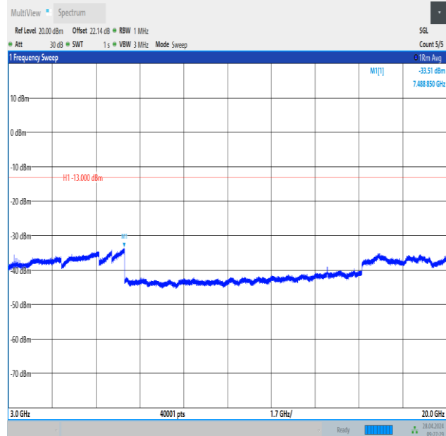
Band2_3MHz_QPSK_19185_1RB#14_3000~20000_3000~20000
