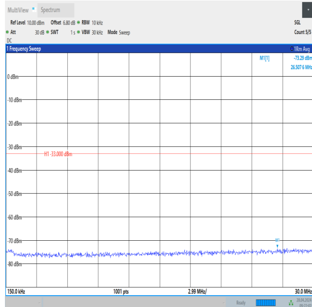
Band2_3MHz_QPSK_18900_1RB#14_0.15~30_0.15~30
