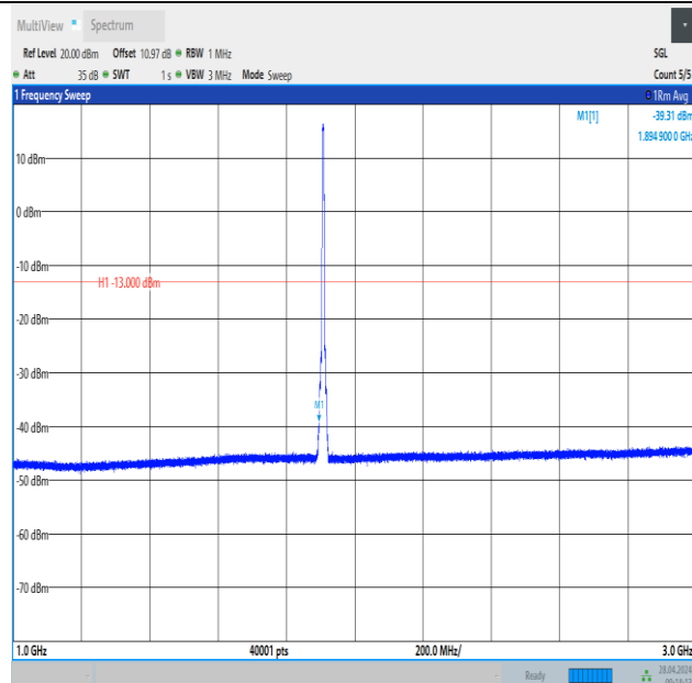
Band2_5MHz_QPSK_19175_25RB#0_1000~3000_1000~3000
