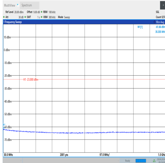
Band2_3MHz_16QAM_18615_1RB#14_30~1000_30~1000
