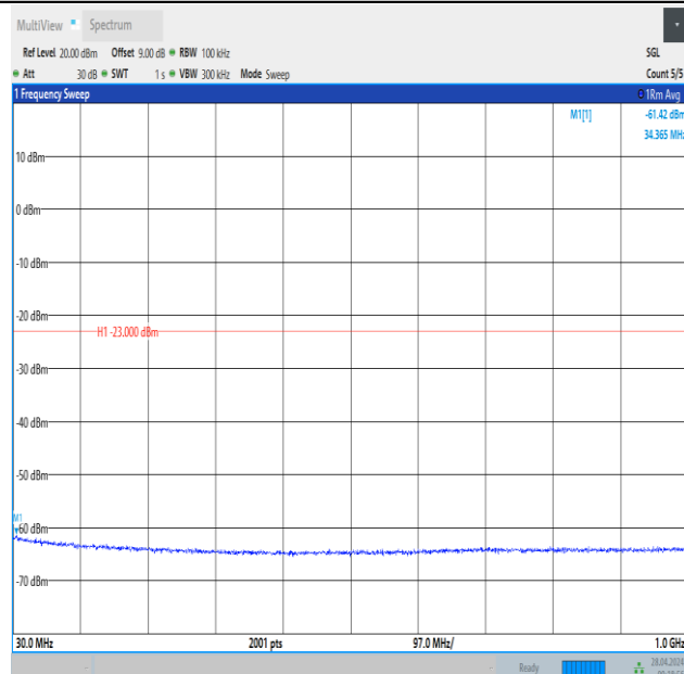
Band2_3MHz_QPSK_18615_15RB#0_30~1000_30~1000
