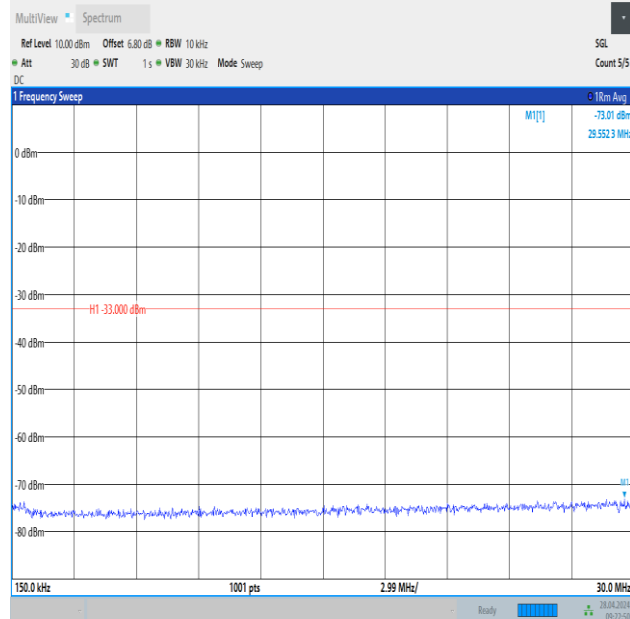
Band2_3MHz_16QAM_18900_1RB#14_0.15~30_0.15~30
