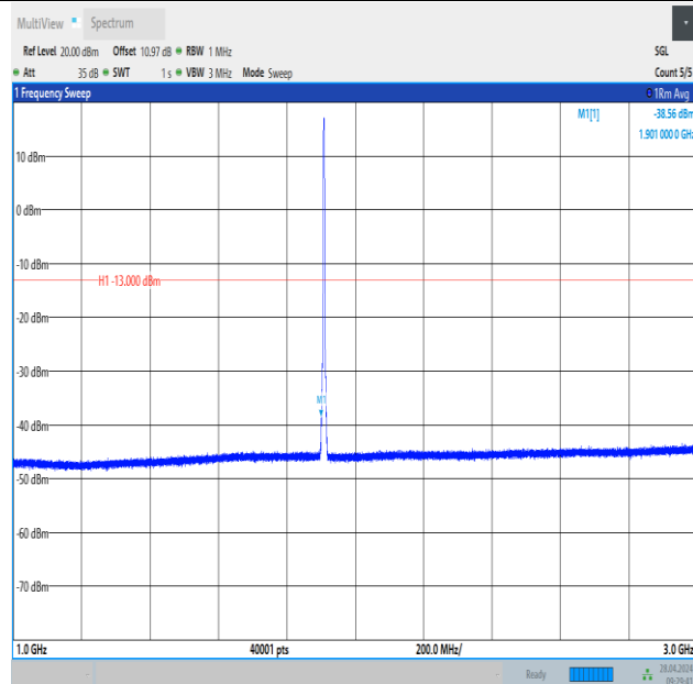
Band2_3MHz_16QAM_19185_15RB#0_1000~3000_1000~3000
