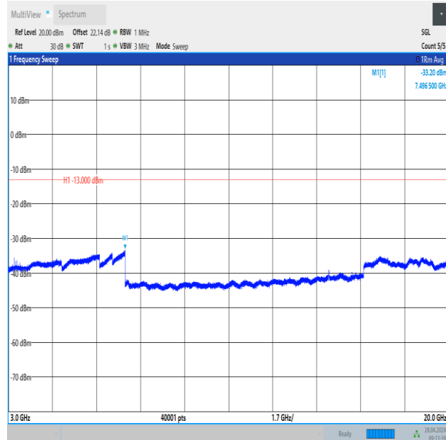
Band2_5MHz_16QAM_19175_1RB#24_3000~20000_3000~20000
