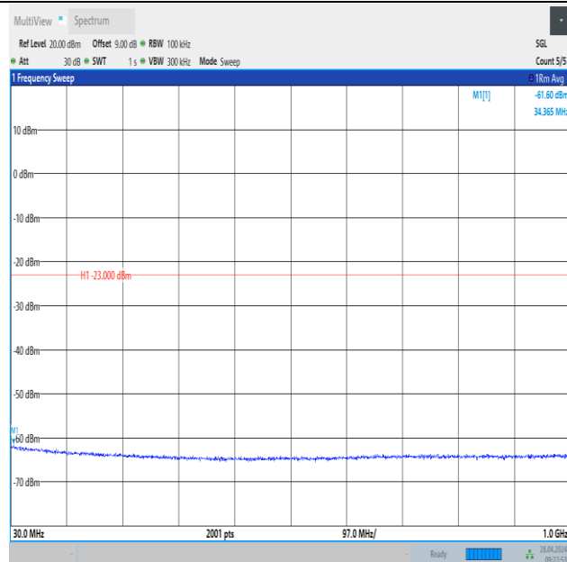
Band2_3MHz_16QAM_19185_1RB#14_30~1000_30~1000
