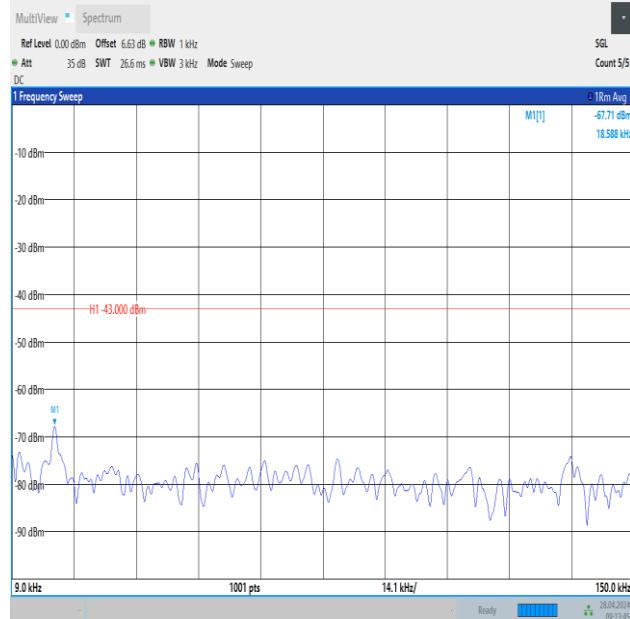
Band2_5MHz_QPSK_19175_25RB#0_0.009~0.15_0.009~0.15
