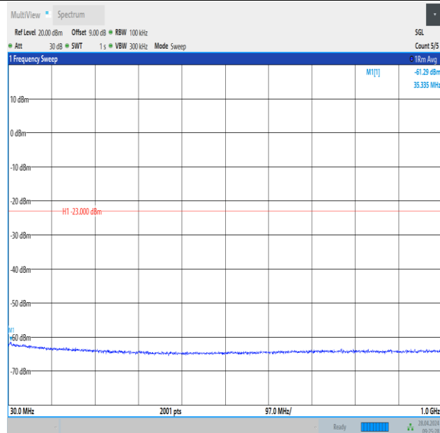
Band2_3MHz_QPSK_19185_1RB#0_30~1000_30~1000
