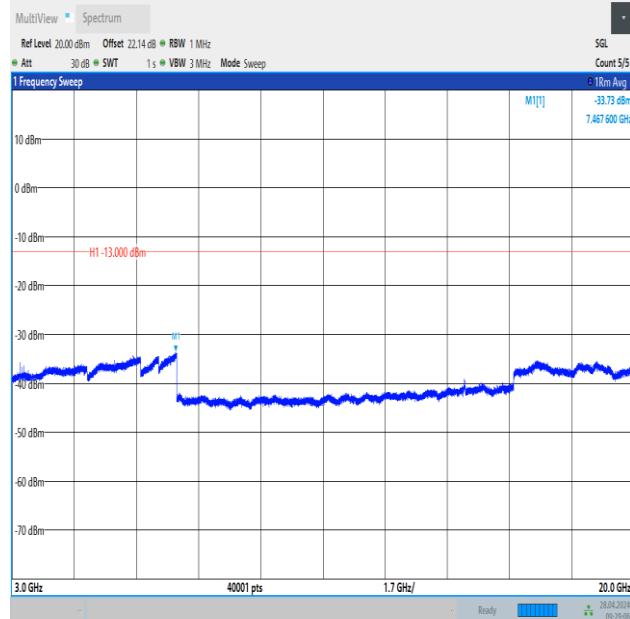
Band2_3MHz_QPSK_19185_15RB#0_3000~20000_3000~20000
