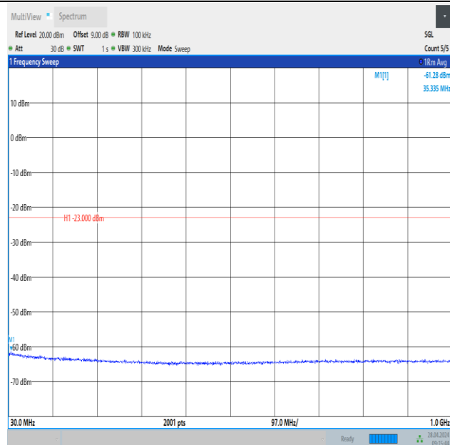
Band2_3MHz_QPSK_18615_1RB#0_30~1000_30~1000
