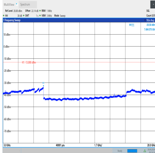
Band2_5MHz_QPSK_19175_25RB#0_3000~20000_3000~20000
