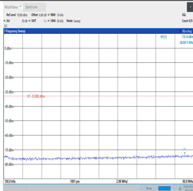
Band2_3MHz_QPSK_18615_1RB#0_0.15~30_0.15~30
