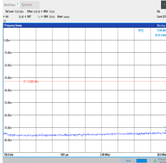
Band2_5MHz_16QAM_19175_1RB#24_0.15~30_0.15~30
