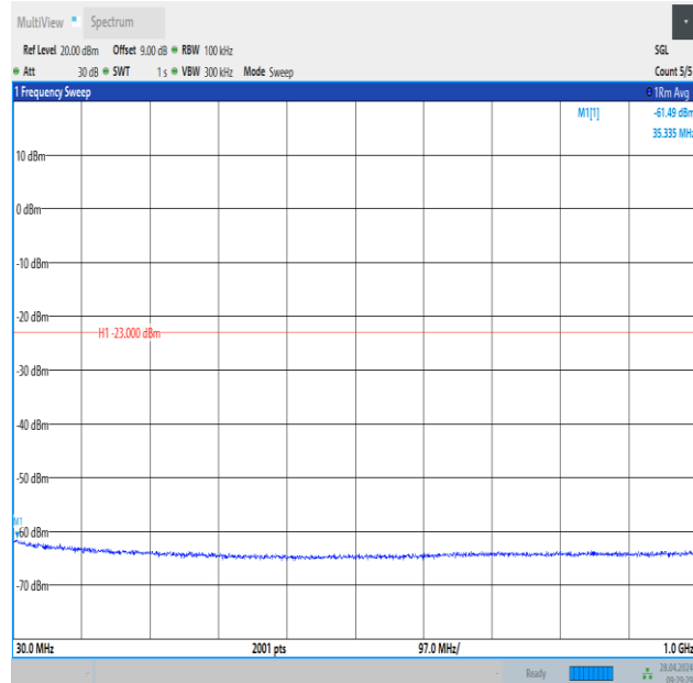
Band2_3MHz_16QAM_19185_15RB#0_30~1000_30~1000
