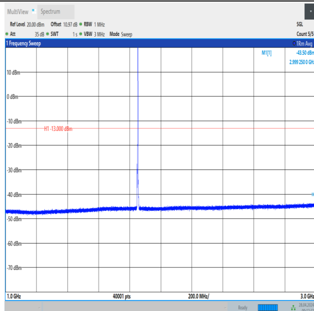
Band2_3MHz_QPSK_18615_1RB#14_1000~3000_1000~3000
