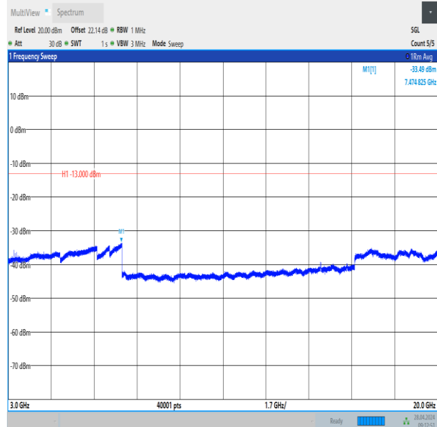
Band2_5MHz_QPSK_19175_1RB#24_3000~20000_3000~20000
