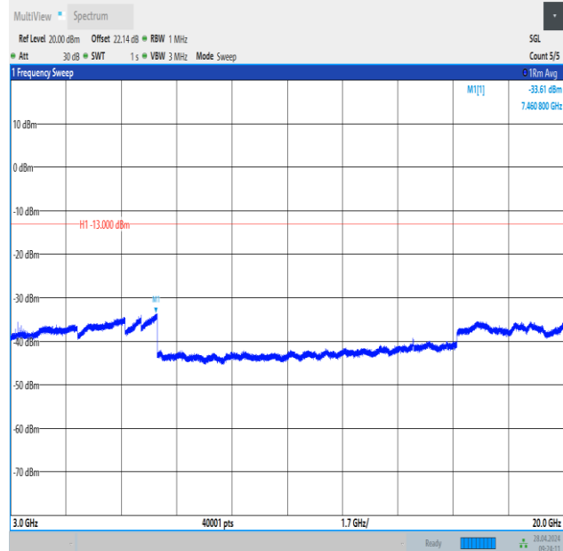
Band2_3MHz_QPSK_18900_15RB#0_3000~20000_3000~20000
