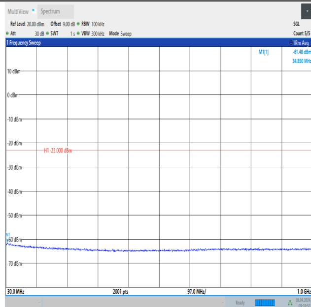
Band2_5MHz_QPSK_19175_1RB#0_30~1000_30~1000
