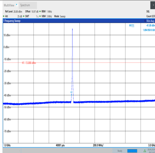
Band2_5MHz_16QAM_19175_25RB#0_1000~3000_1000~3000
