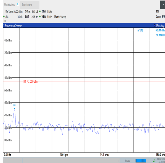
Band2_5MHz_QPSK_19175_1RB#24_0.009~0.15_0.009~0.15
