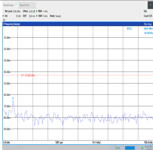
Band2_3MHz_QPSK_18900_1RB#0_0.009~0.15_0.009~0.15
