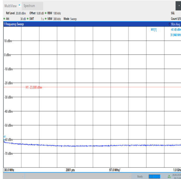
Band2_3MHz_16QAM_18900_1RB#14_30~1000_30~1000
