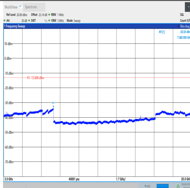
Band2_3MHz_16QAM_19185_1RB#0_3000~20000_3000~20000
