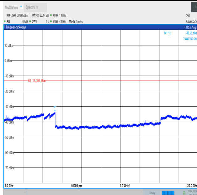
Band2_3MHz_16QAM_19185_1RB#14_3000~20000_3000~20000
