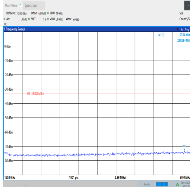
Band2_3MHz_16QAM_18615_1RB#14_0.15~30_0.15~30
