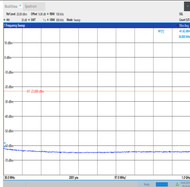
Band2_3MHz_QPSK_18900_1RB#0_30~1000_30~1000
