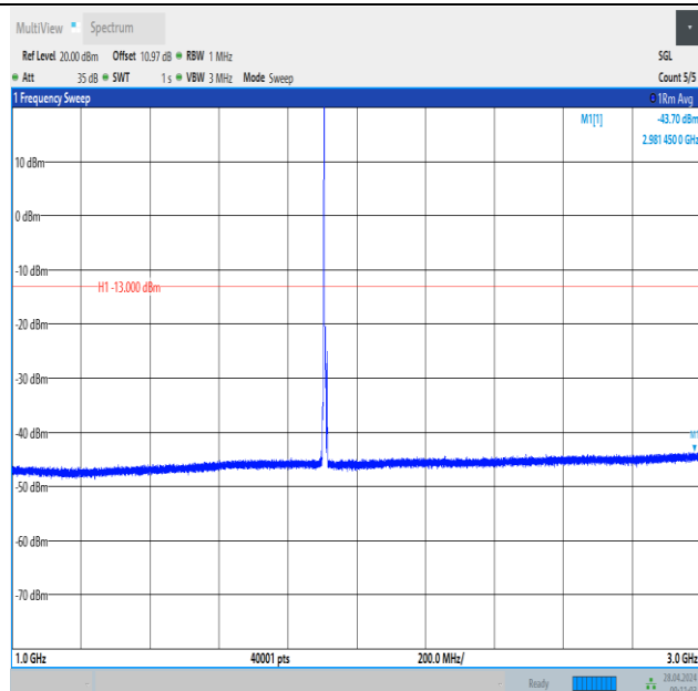
Band2_5MHz_QPSK_19175_1RB#0_1000~3000_1000~3000
