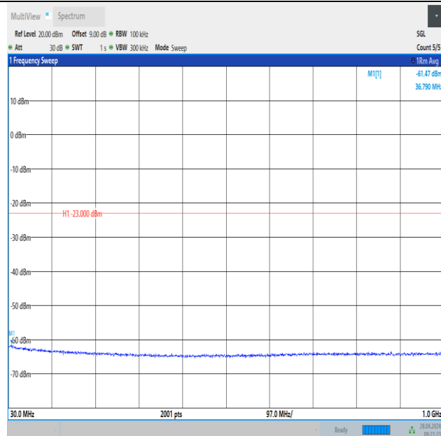
Band2_3MHz_16QAM_18900_1RB#0_30~1000_30~1000
