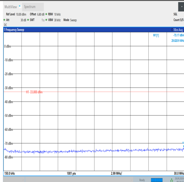
Band2_3MHz_QPSK_19185_1RB#14_0.15~30_0.15~30
