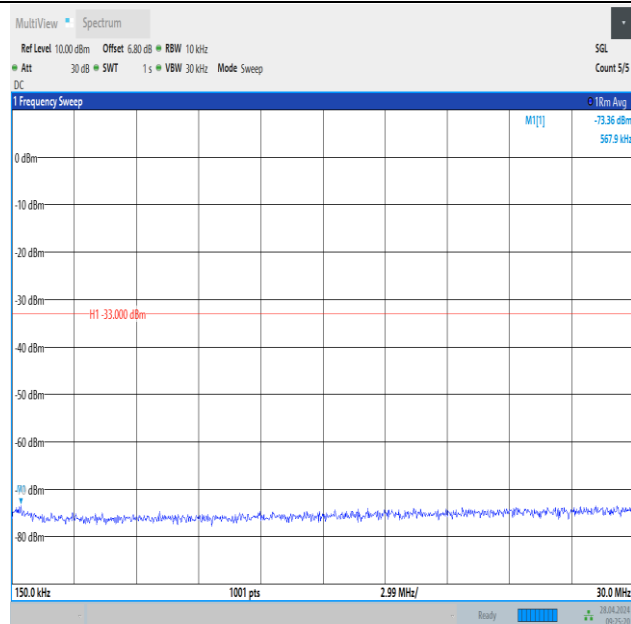
Band2_3MHz_QPSK_19185_1RB#0_0.15~30_0.15~30
