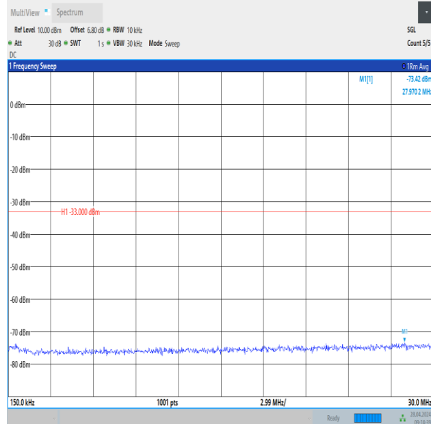
Band2_5MHz_16QAM_19175_25RB#0_0.15~30_0.15~30
