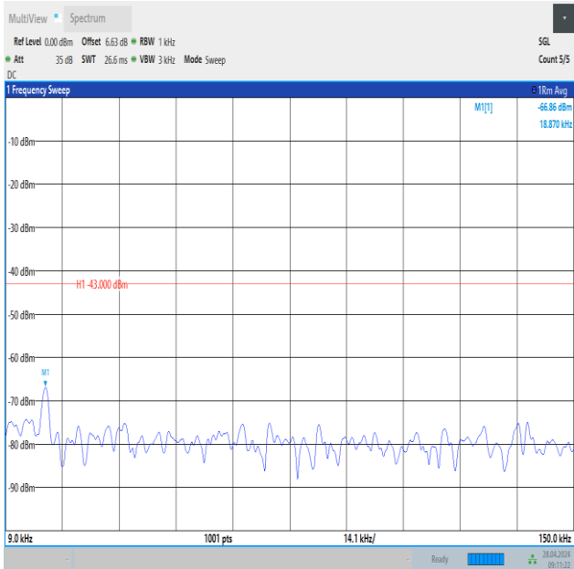
Band2_5MHz_16QAM_19175_1RB#0_0.009~0.15_0.009~0.15
