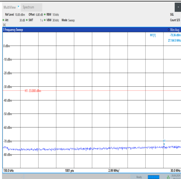
Band2_3MHz_QPSK_18615_1RB#14_0.15~30_0.15~30
