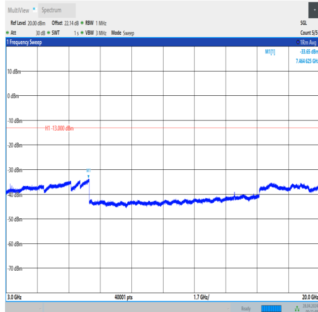
Band2_3MHz_16QAM_18900_1RB#0_3000~20000_3000~20000
