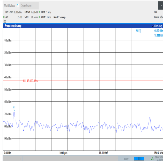
Band2_3MHz_QPSK_19185_15RB#0_0.009~0.15_0.009~0.15
