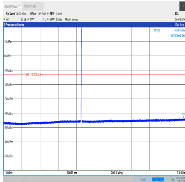
Band2_3MHz_16QAM_18615_1RB#14_1000~3000_1000~3000
