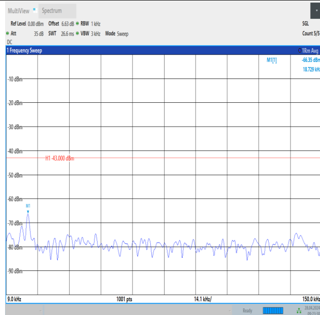
Band2_3MHz_QPSK_18900_15RB#0_0.009~0.15_0.009~0.15
