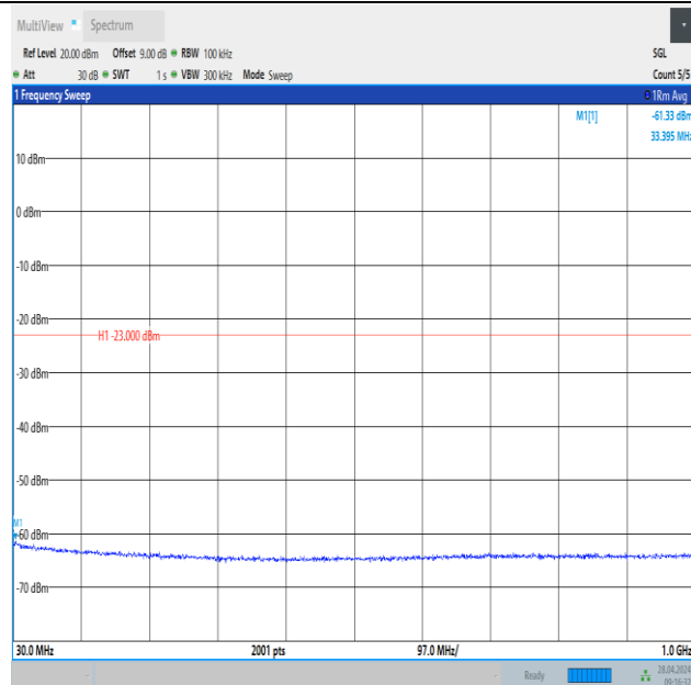
Band2_3MHz_16QAM_18615_1RB#0_30~1000_30~1000
