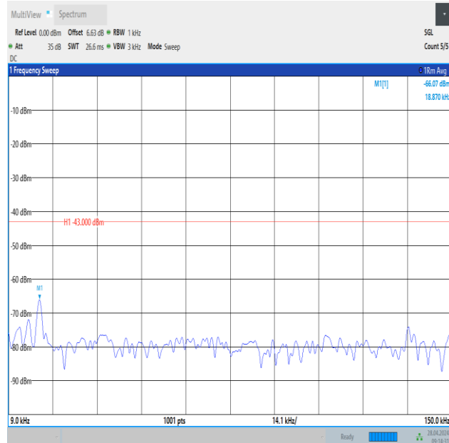
Band2_5MHz_16QAM_19175_25RB#0_0.009~0.15_0.009~0.15
