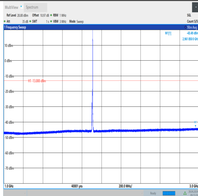
Band2_5MHz_16QAM_19175_1RB#24_1000~3000_1000~3000
