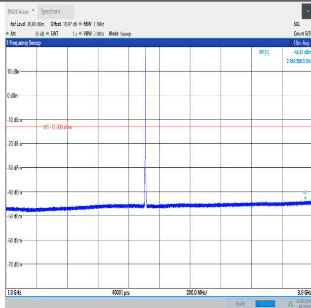
Band2_3MHz_16QAM_19185_1RB#14_1000~3000_1000~3000
