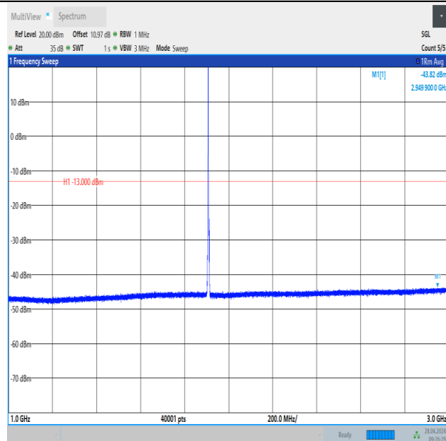
Band2_3MHz_16QAM_19185_1RB#0_1000~3000_1000~3000
