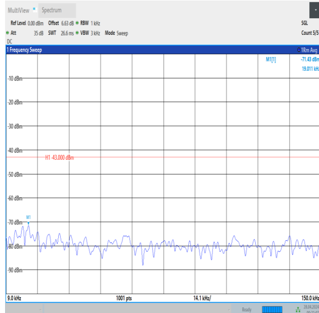
Band2_3MHz_16QAM_18900_1RB#0_0.009~0.15_0.009~0.15
