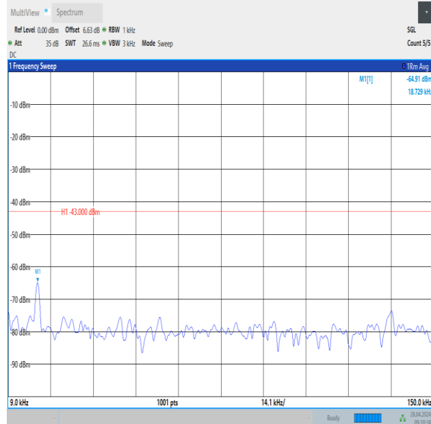
Band2_5MHz_QPSK_19175_1RB#0_0.009~0.15_0.009~0.15
