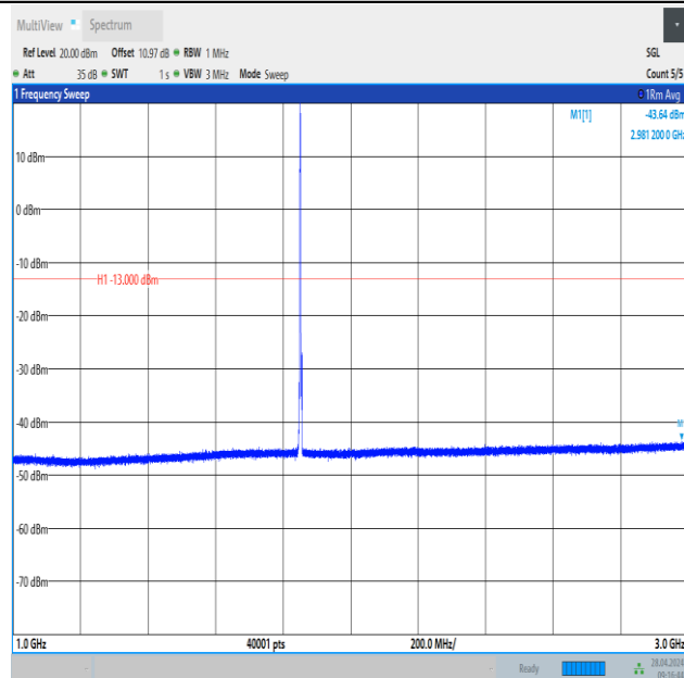
Band2_3MHz_16QAM_18615_1RB#0_1000~3000_1000~3000
