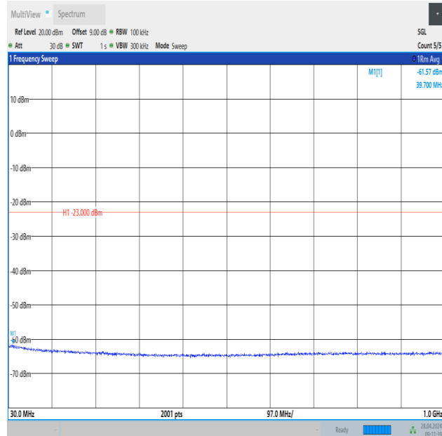
Band2_5MHz_16QAM_19175_1RB#0_30~1000_30~1000
