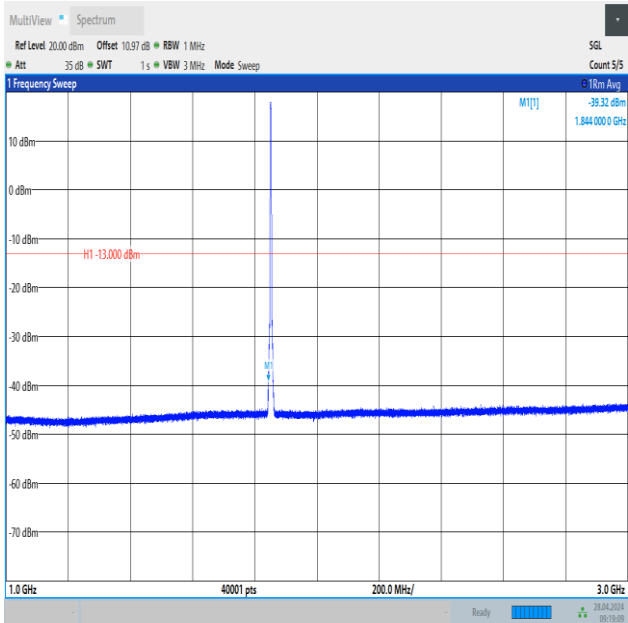
Band2_3MHz_QPSK_18615_15RB#0_1000~3000_1000~3000
