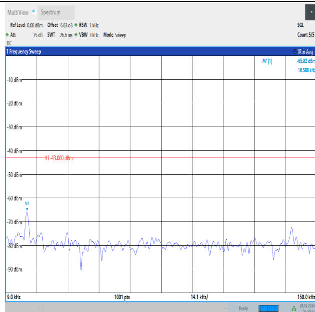
Band2_3MHz_16QAM_19185_15RB#0_0.009~0.15_0.009~0.15
