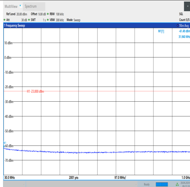
Band2_3MHz_QPSK_18900_1RB#14_30~1000_30~1000
