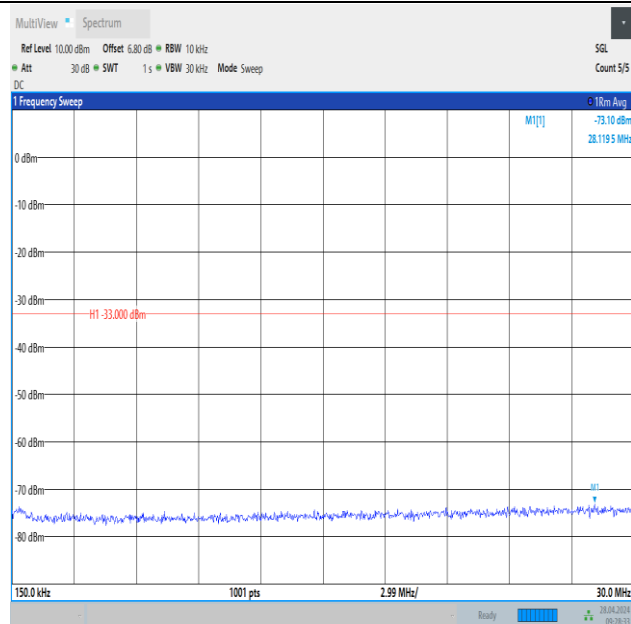
Band2_3MHz_QPSK_19185_15RB#0_0.15~30_0.15~30
