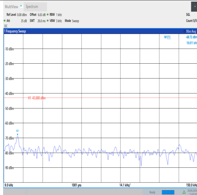
Band25_10MHz_QPSK_26365_1RB#0_0.009~0.15_0.009~0.15
