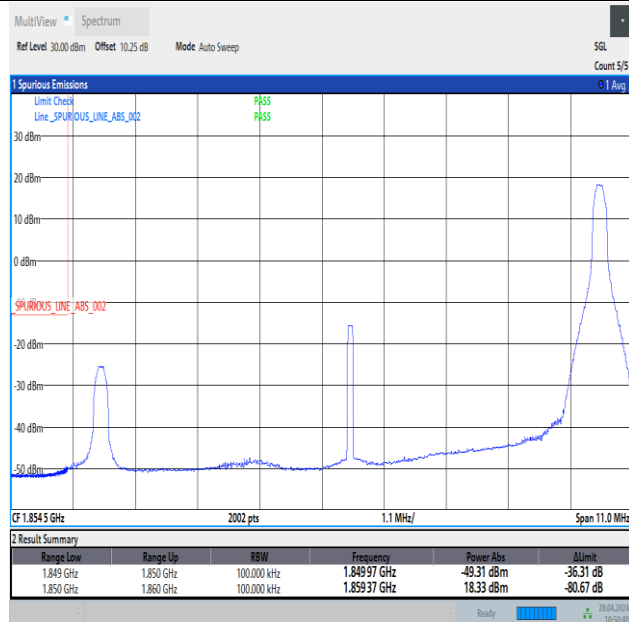
Band25_10MHz_16QAM_26090_1RB#49
