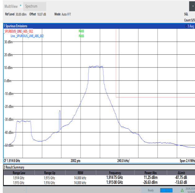
Band25_1.4MHz_QPSK_26683_1RB#5
