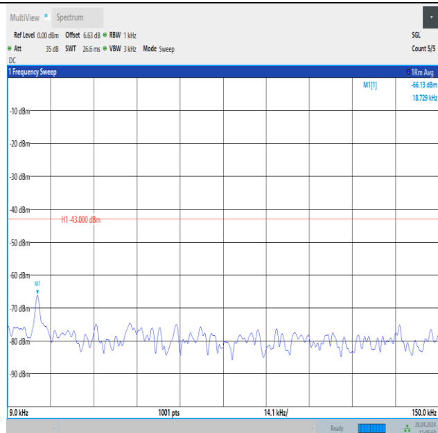
Band25_10MHz_16QAM_26090_1RB#49_0.009~0.15_0.009~0.15
