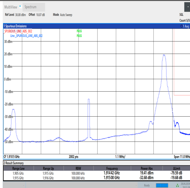
Band25_10MHz_QPSK_26640_1RB#49
