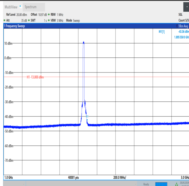
Band25_15MHz_QPSK_26115_75RB#0_1000~3000_1000~3000
