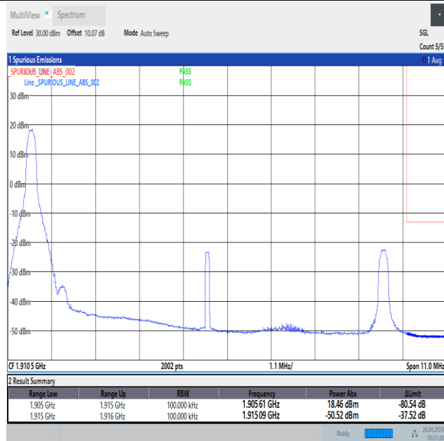
Band25_10MHz_16QAM_26640_1RB#0
