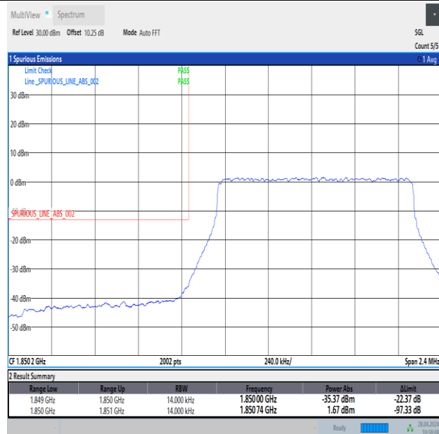
Band25_1.4MHz_16QAM_26047_6RB#0
