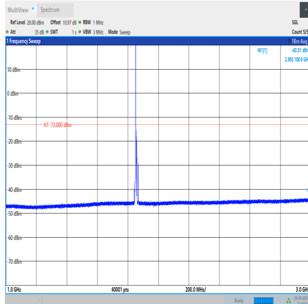
Band25_10MHz_QPSK_26090_1RB#0_1000~3000_1000~3000
