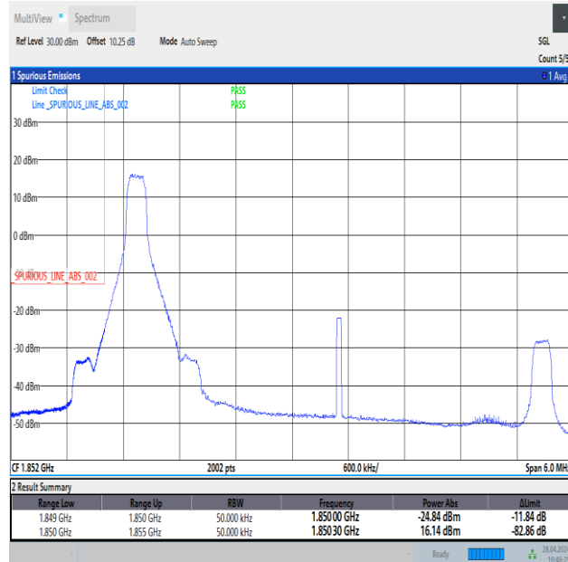
Band25_5MHz_QPSK_26065_1RB#0
