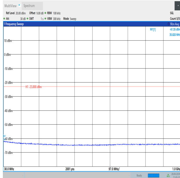
Band25_10MHz_16QAM_26090_1RB#0_30~1000_30~1000
