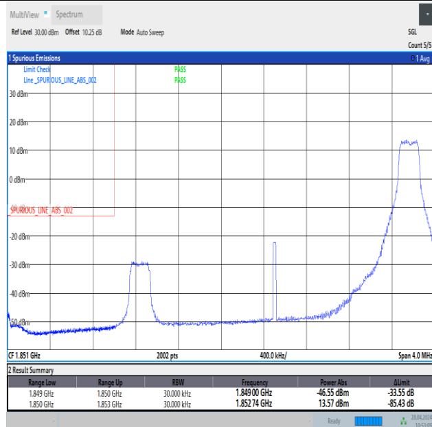
Band25_3MHz_16QAM_26055_1RB#14
