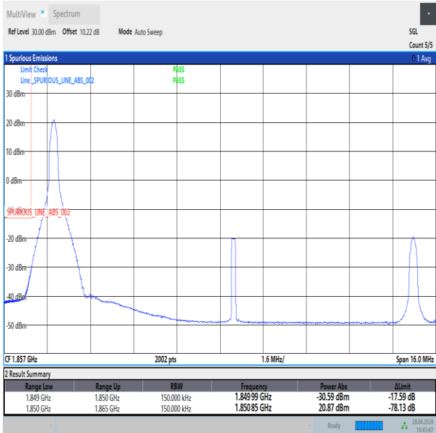
Band25_15MHz_QPSK_26115_1RB#0
