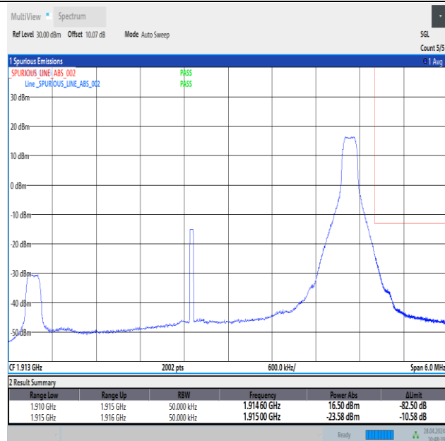
Band25_5MHz_QPSK_26665_1RB#24
