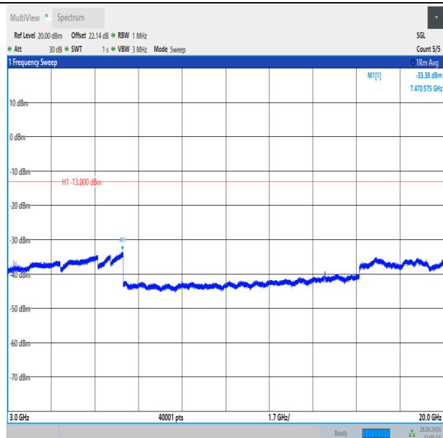
Band25_10MHz_16QAM_26090_1RB#0_3000~20000_3000~20000
