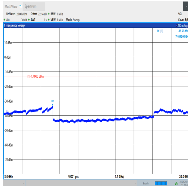
Band25_10MHz_QPSK_26090_1RB#0_3000~20000_3000~20000
