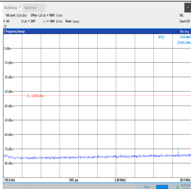
Band25_10MHz_QPSK_26090_1RB#49_0.15~30_0.15~30
