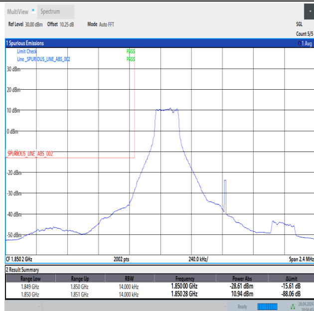
Band25_1.4MHz_QPSK_26047_1RB#0
