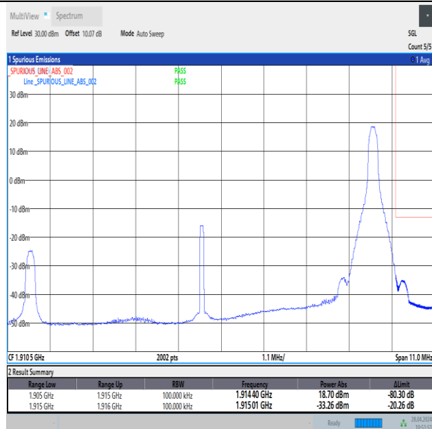
Band25_10MHz_16QAM_26640_1RB#49
