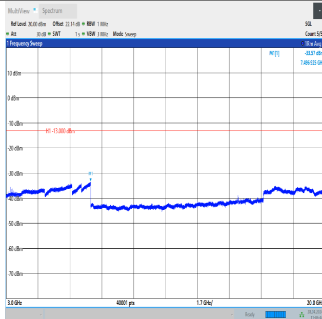
Band25_10MHz_QPSK_26090_1RB#49_3000~20000_3000~20000
