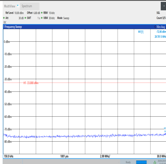
Band25_10MHz_QPSK_26365_1RB#0_0.15~30_0.15~30
