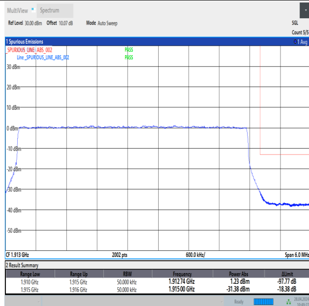
Band25_5MHz_16QAM_26665_25RB#0
