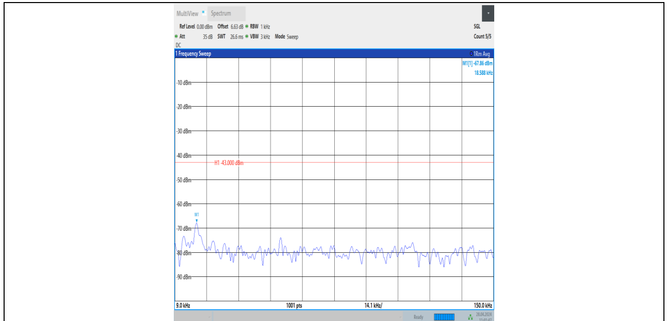
Band25_15MHz_QPSK_26115_75RB#0_0.009~0.15_0.009~0.15
