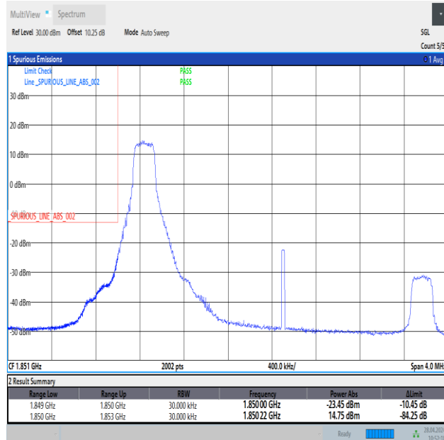
Band25_3MHz_QPSK_26055_1RB#0
