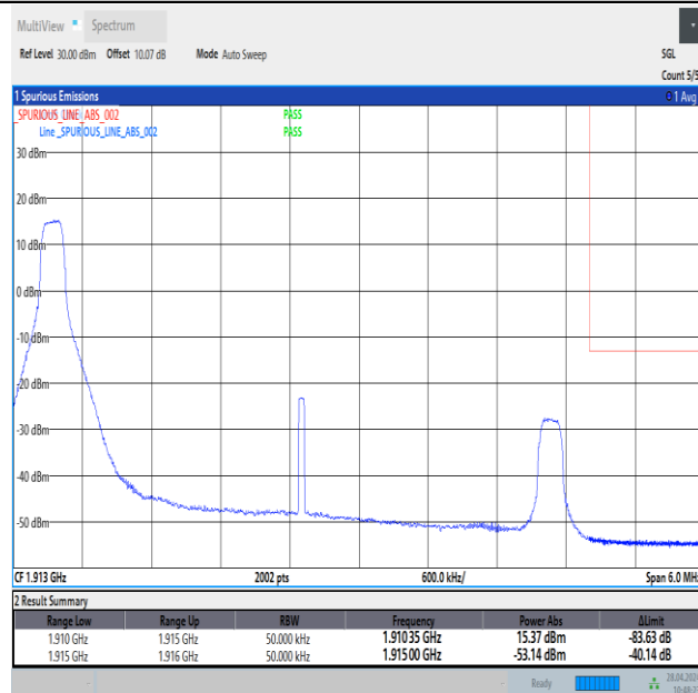
Band25_5MHz_16QAM_26665_1RB#0
