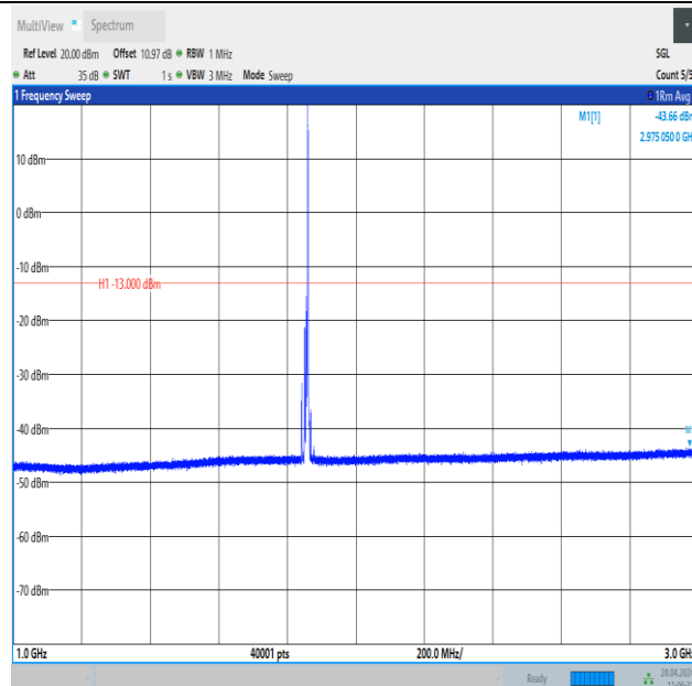
Band25_10MHz_QPSK_26090_1RB#49_1000~3000_1000~3000
