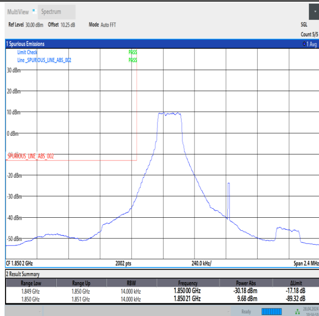
Band25_1.4MHz_16QAM_26047_1RB#0
