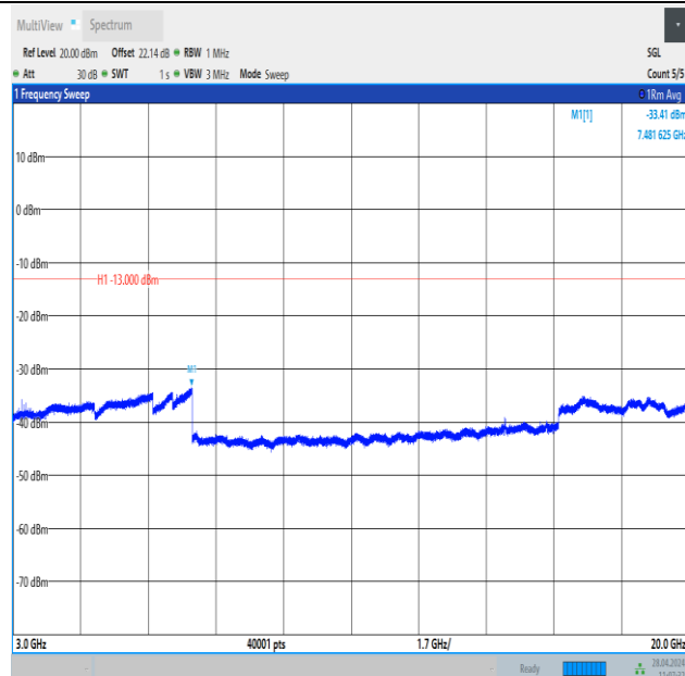
Band25_10MHz_16QAM_26090_1RB#49_3000~20000_3000~20000
