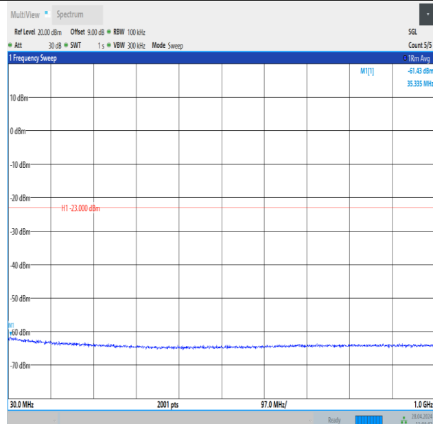
Band25_10MHz_QPSK_26090_1RB#0_30~1000_30~1000
