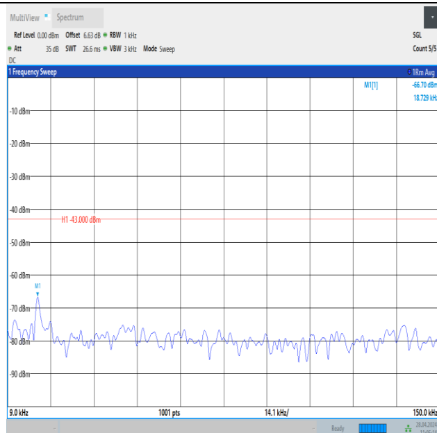
Band25_10MHz_16QAM_26090_1RB#0_0.009~0.15_0.009~0.15
