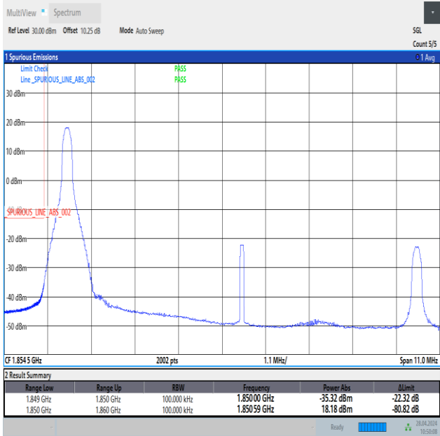
Band25_10MHz_16QAM_26090_1RB#0
