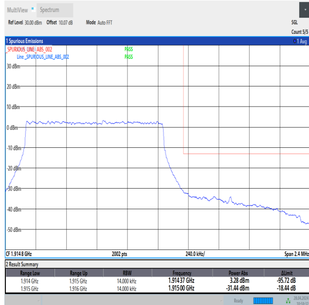
Band25_1.4MHz_QPSK_26683_6RB#0
