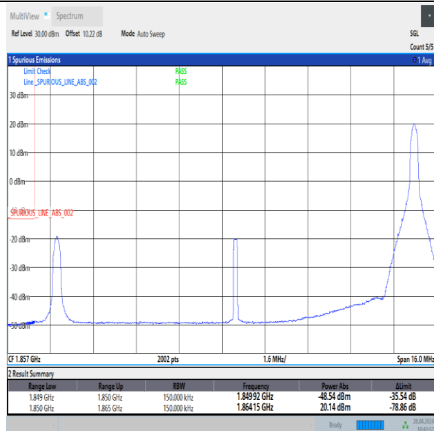
Band25_15MHz_16QAM_26115_1RB#74
