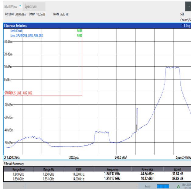
Band25_1.4MHz_16QAM_26047_1RB#5
