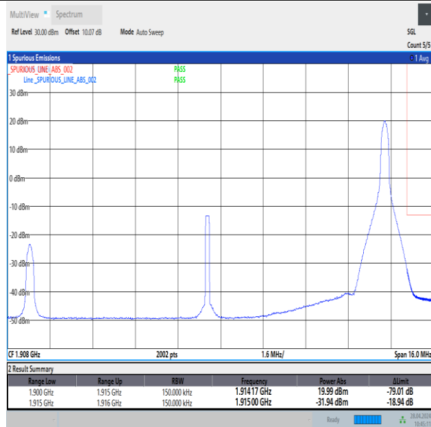
Band25_15MHz_16QAM_26615_1RB#74
