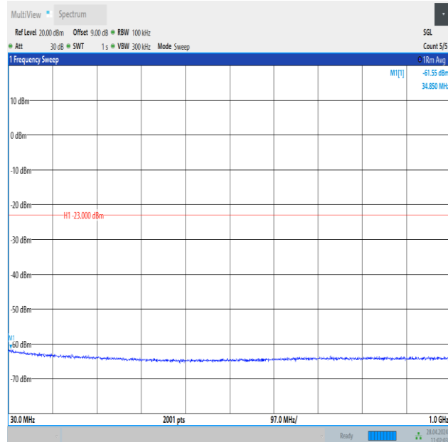
Band25_15MHz_QPSK_26115_75RB#0_30~1000_30~1000
