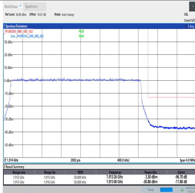
Band25_3MHz_16QAM_26675_15RB#0
