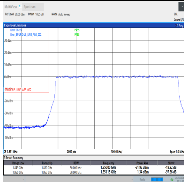
Band25_3MHz_16QAM_26055_15RB#0
