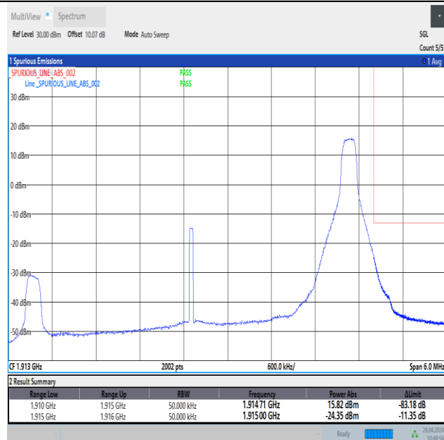
Band25_5MHz_16QAM_26665_1RB#24
