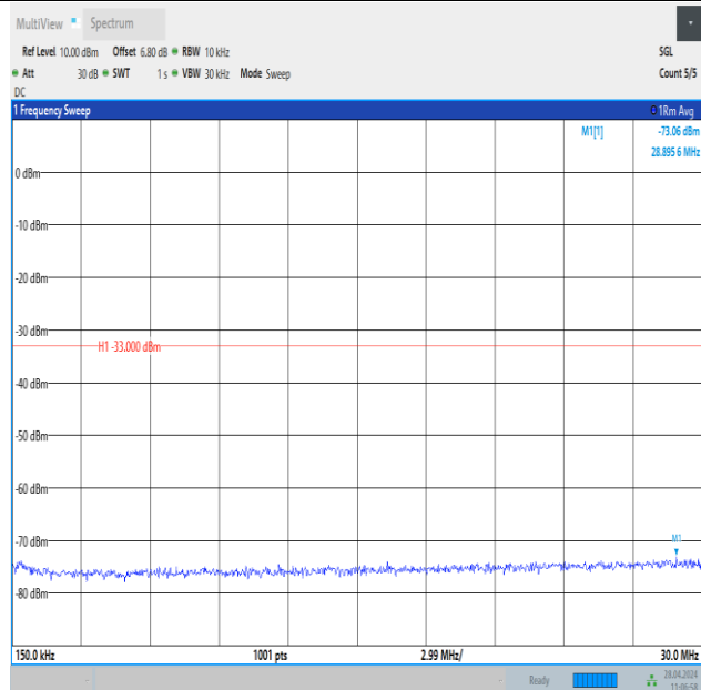
Band25_10MHz_16QAM_26090_1RB#49_0.15~30_0.15~30
