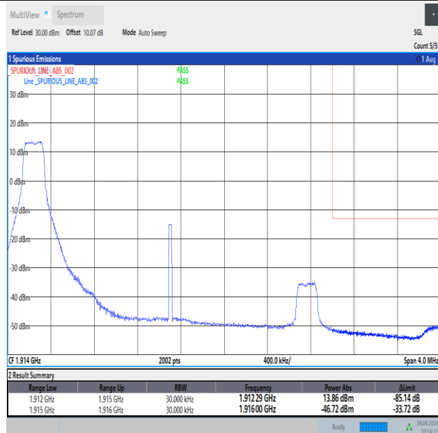
Band25_3MHz_16QAM_26675_1RB#0
