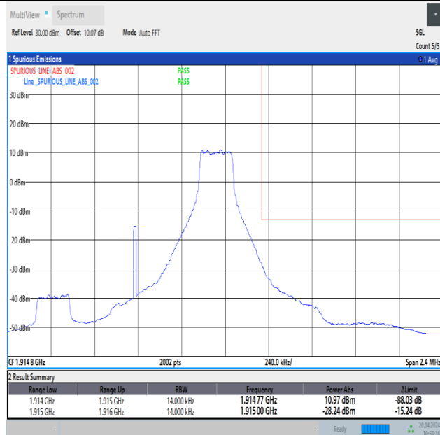
Band25_1.4MHz_16QAM_26683_1RB#5
