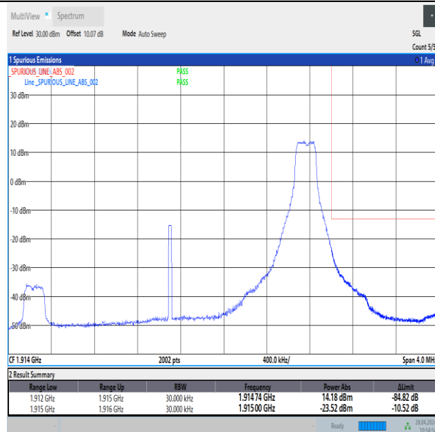
Band25_3MHz_16QAM_26675_1RB#14
