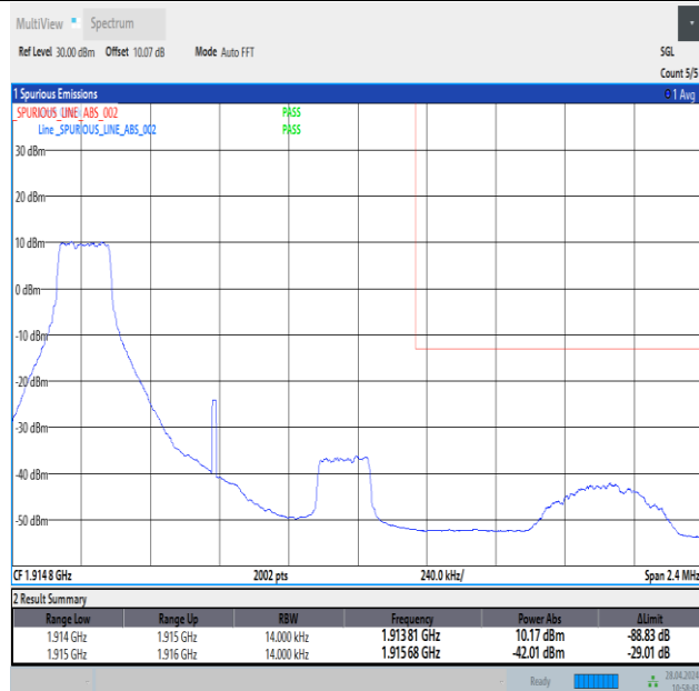
Band25_1.4MHz_16QAM_26683_1RB#0
