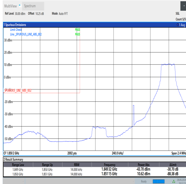
Band25_1.4MHz_QPSK_26047_1RB#5
