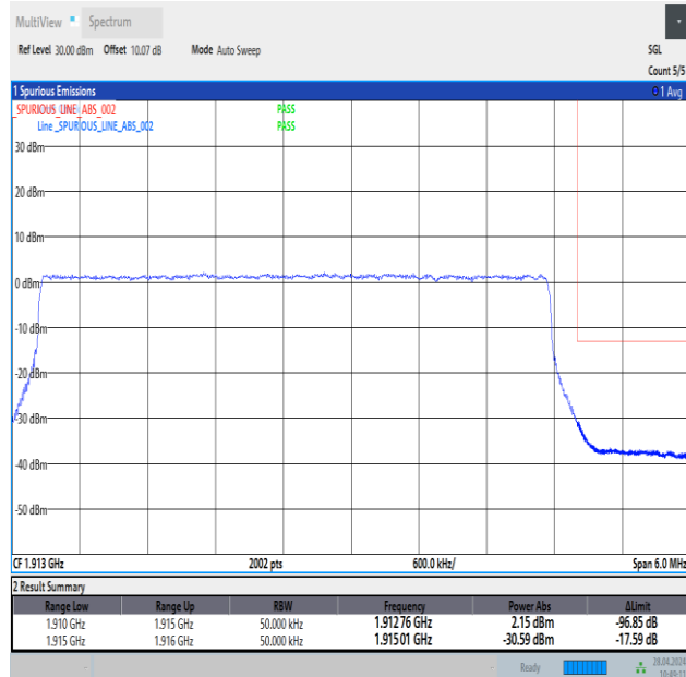
Band25_5MHz_QPSK_26665_25RB#0
