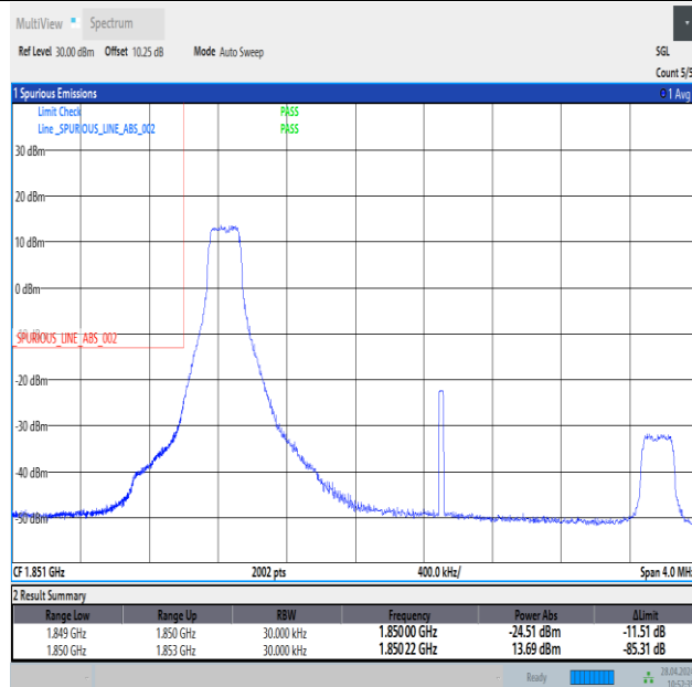
Band25_3MHz_16QAM_26055_1RB#0
