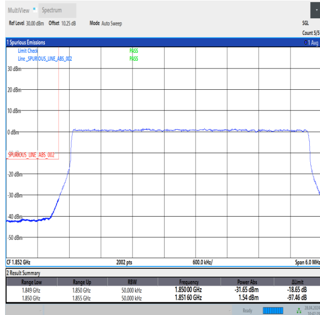
Band25_5MHz_QPSK_26065_25RB#0
