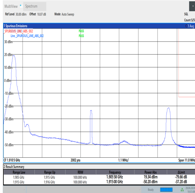
Band25_10MHz_QPSK_26640_1RB#0
