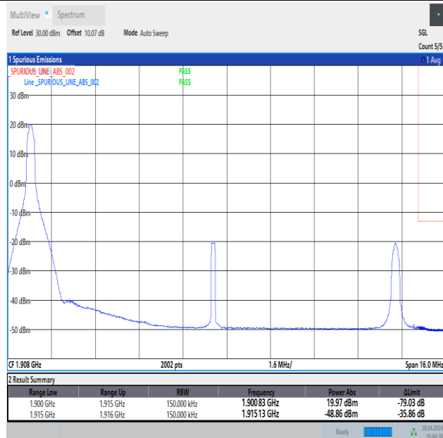
Band25_15MHz_16QAM_26615_1RB#0
