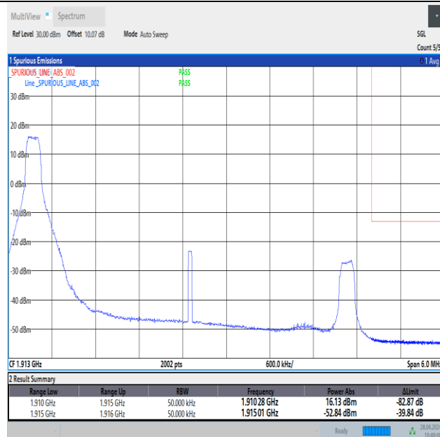
Band25_5MHz_QPSK_26665_1RB#0
