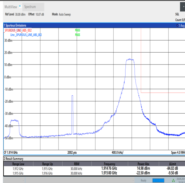
Band25_3MHz_QPSK_26675_1RB#14
