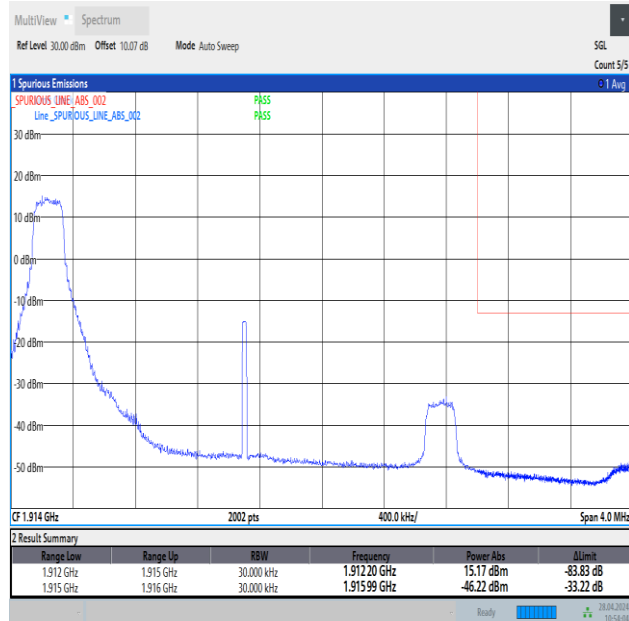
Band25_3MHz_QPSK_26675_1RB#0
