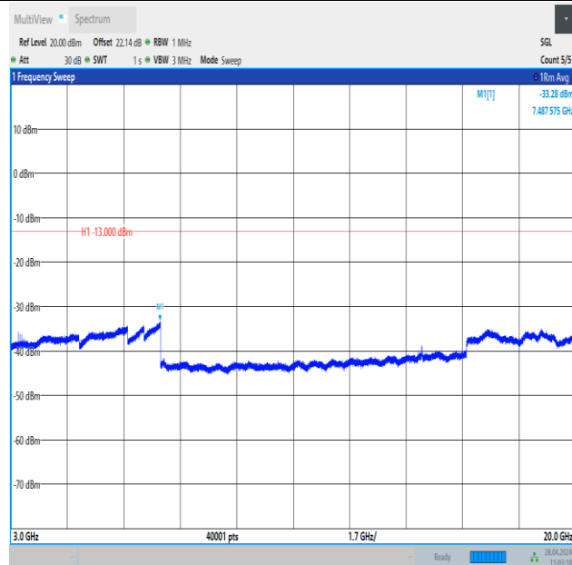
Band25_15MHz_QPSK_26365_75RB#0_3000~20000_3000~20000
