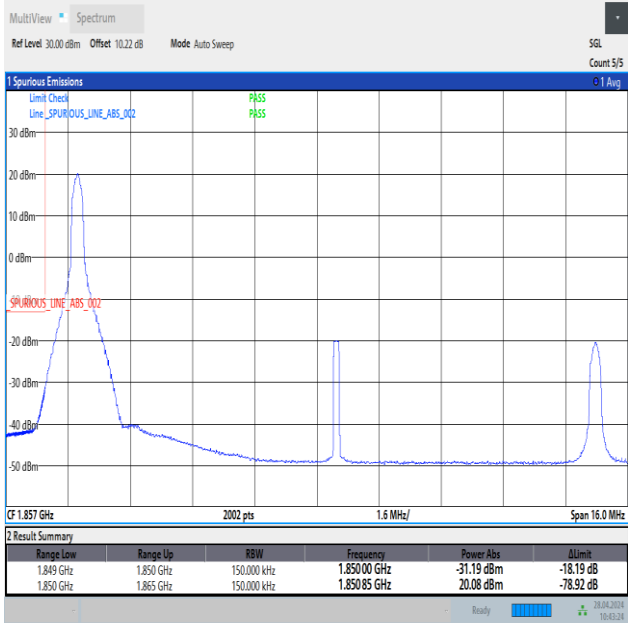
Band25_15MHz_16QAM_26115_1RB#0
