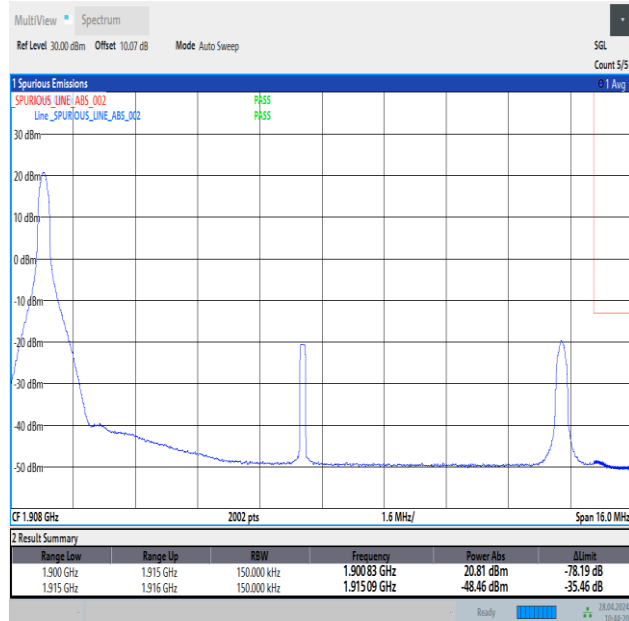
Band25_15MHz_QPSK_26615_1RB#0
