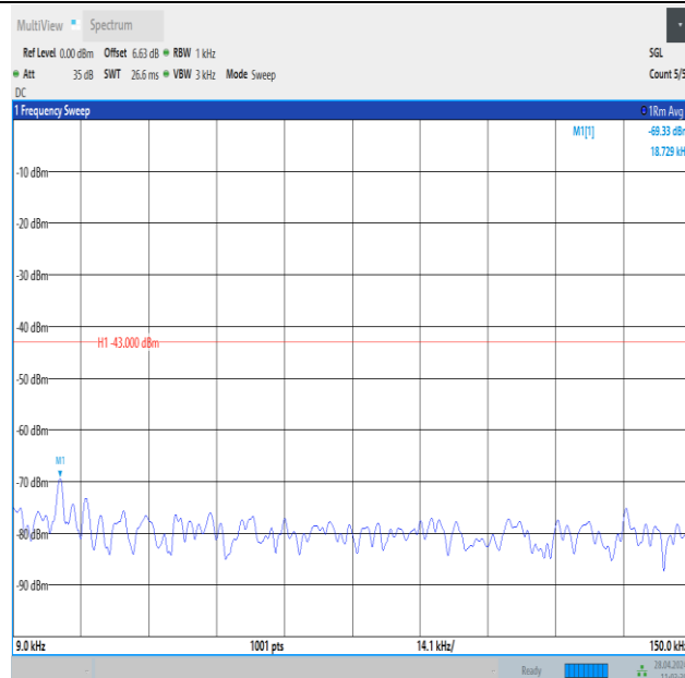
Band25_15MHz_QPSK_26615_75RB#0_0.009~0.15_0.009~0.15
