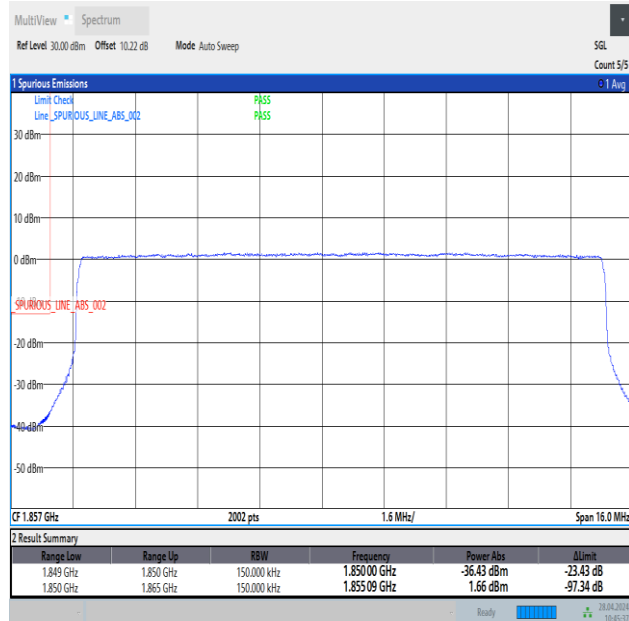
Band25_15MHz_QPSK_26115_75RB#0
