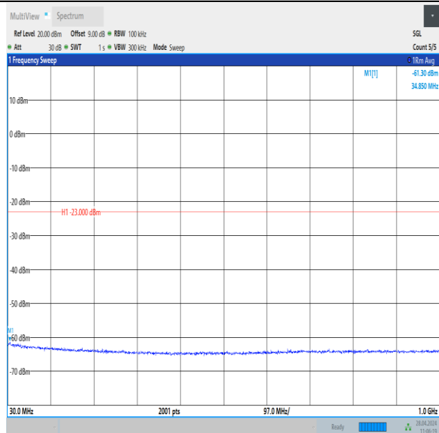
Band25_10MHz_QPSK_26090_1RB#49_30~1000_30~1000
