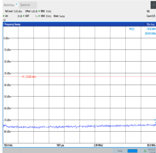
Band25_15MHz_QPSK_26365_75RB#0_0.15~30_0.15~30
