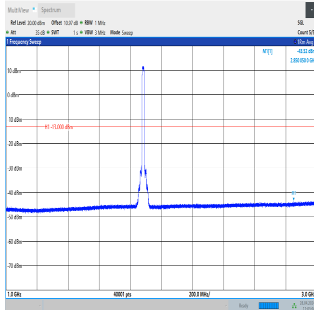
Band25_15MHz_QPSK_26365_75RB#0_1000~3000_1000~3000
