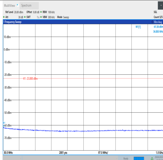
Band25_10MHz_QPSK_26365_1RB#0_30~1000_30~1000
