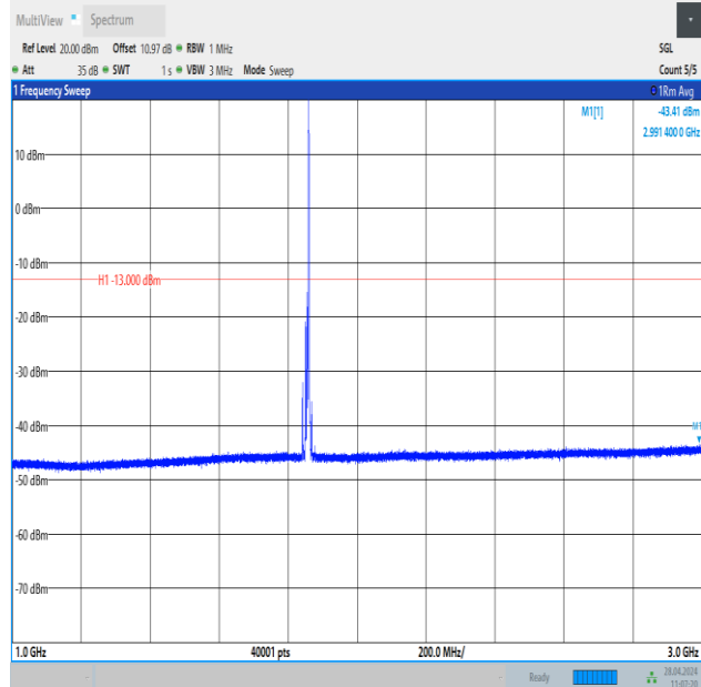
Band25_10MHz_16QAM_26090_1RB#49_1000~3000_1000~3000
