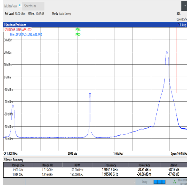
Band25_15MHz_QPSK_26615_1RB#74
