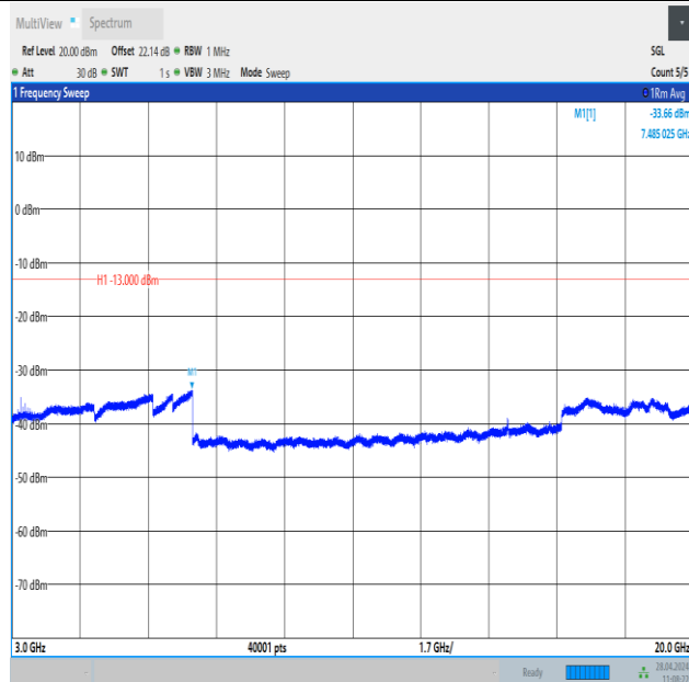
Band25_10MHz_QPSK_26365_1RB#0_3000~20000_3000~20000
