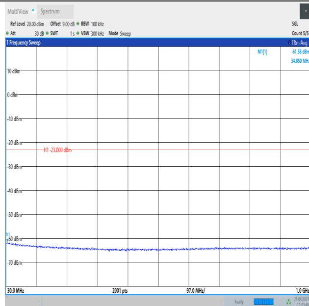
Band25_15MHz_QPSK_26615_75RB#0_30~1000_30~1000
