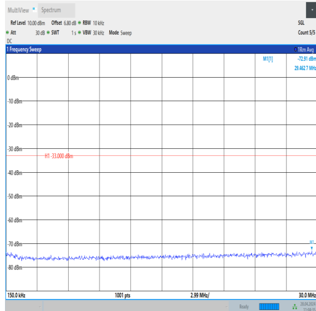
Band25_10MHz_QPSK_26090_1RB#0_0.15~30_0.15~30
