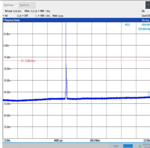
Band25_10MHz_16QAM_26090_1RB#0_1000~3000_1000~3000
