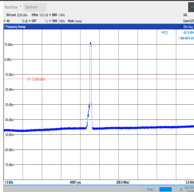
Band25_15MHz_QPSK_26615_75RB#0_1000~3000_1000~3000
