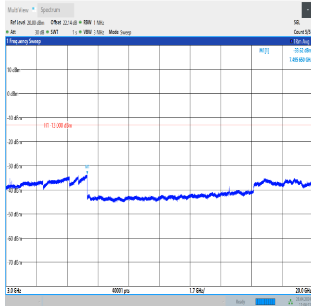
Band25_15MHz_QPSK_26615_75RB#0_3000~20000_3000~20000
