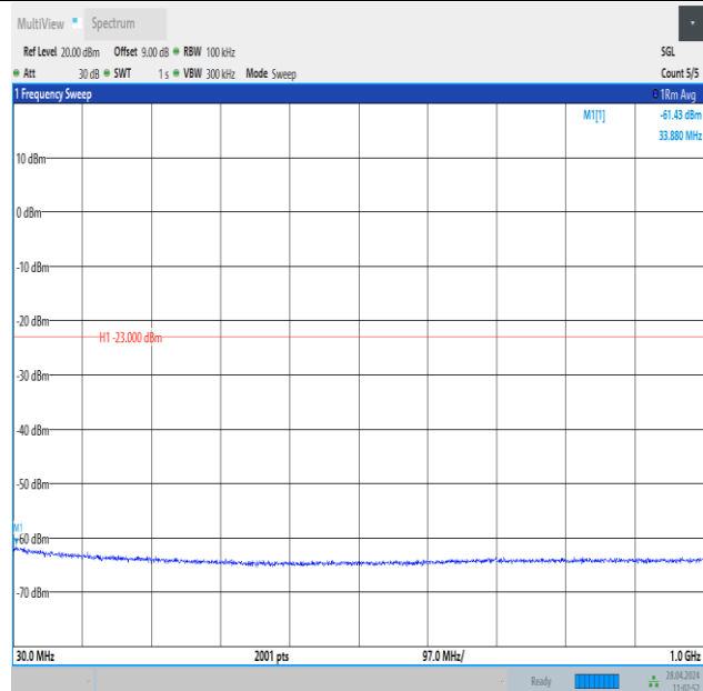
Band25_15MHz_QPSK_26365_75RB#0_30~1000_30~1000
