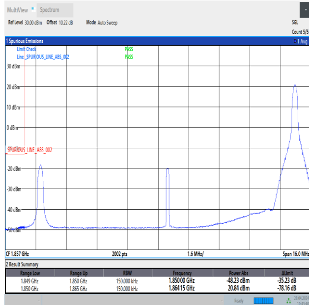
Band25_15MHz_QPSK_26115_1RB#74
