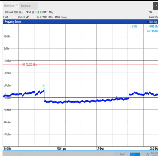
Band25_15MHz_QPSK_26115_75RB#0_3000~20000_3000~20000
