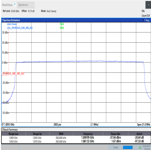
Band25_20MHz_QPSK_26140_100RB#0
