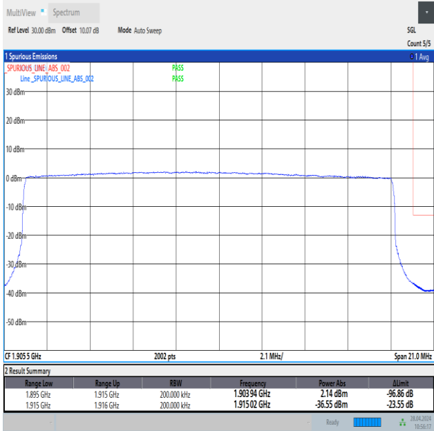
Band25_20MHz_QPSK_26590_100RB#0
