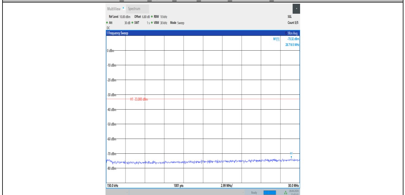
Band25_15MHz_QPSK_26115_75RB#0_0.15~30_0.15~30
