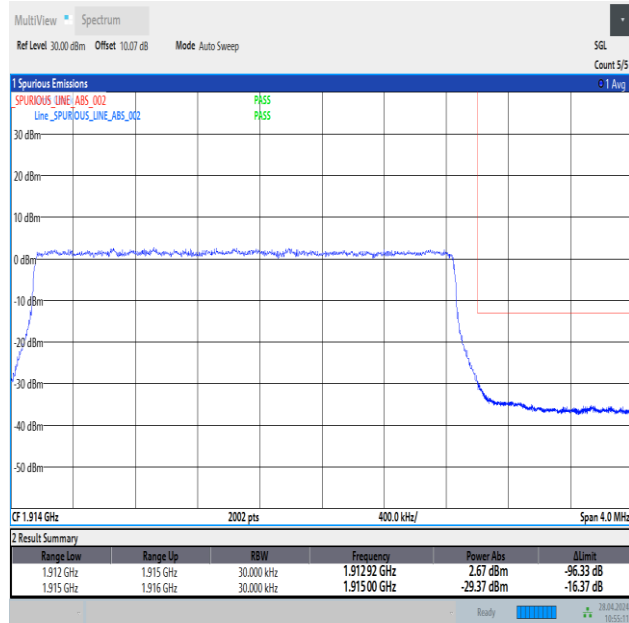
Band25_3MHz_QPSK_26675_15RB#0
