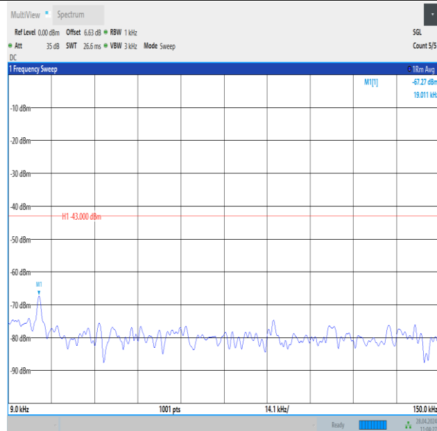
Band25_10MHz_QPSK_26090_1RB#0_0.009~0.15_0.009~0.15
