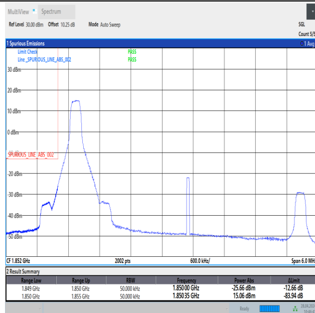
Band25_5MHz_16QAM_26065_1RB#0
