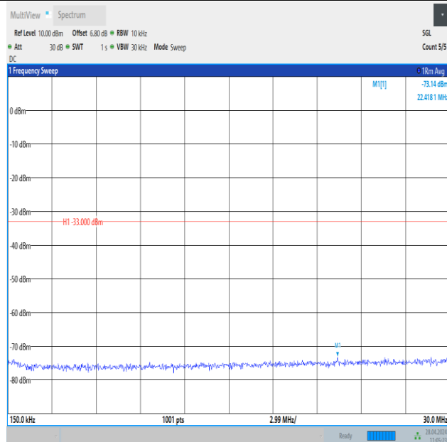
Band25_10MHz_16QAM_26090_1RB#0_0.15~30_0.15~30
