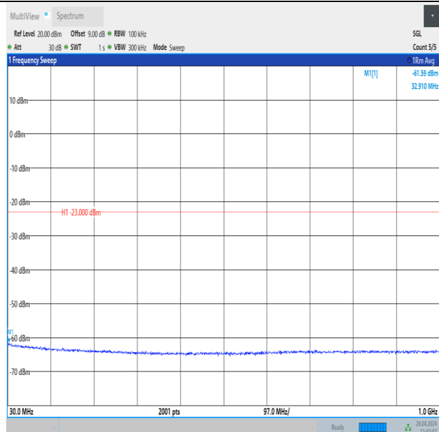
Band25_10MHz_16QAM_26090_1RB#49_30~1000_30~1000
