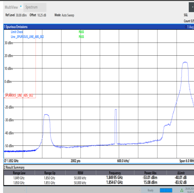
Band25_5MHz_16QAM_26065_1RB#24
