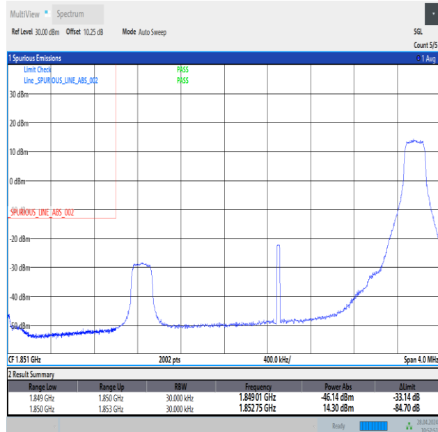
Band25_3MHz_QPSK_26055_1RB#14
