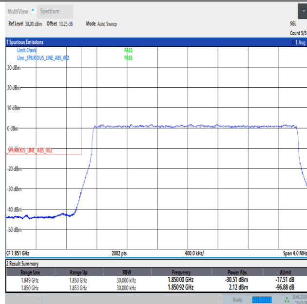
Band25_3MHz_QPSK_26055_15RB#0
