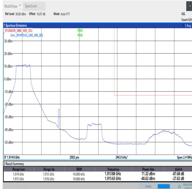
Band25_1.4MHz_QPSK_26683_1RB#0
