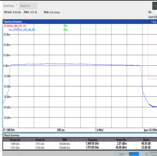
Band25_15MHz_QPSK_26615_75RB#0
