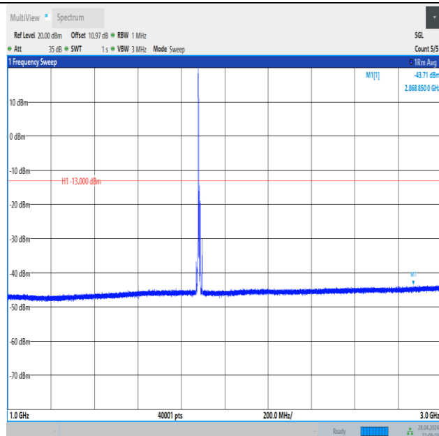
Band25_10MHz_QPSK_26365_1RB#0_1000~3000_1000~3000
