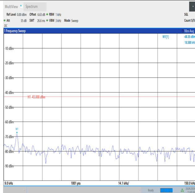
Band25_15MHz_QPSK_26365_75RB#0_0.009~0.15_0.009~0.15
