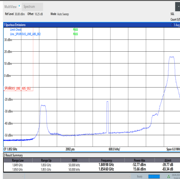
Band25_5MHz_QPSK_26065_1RB#24
