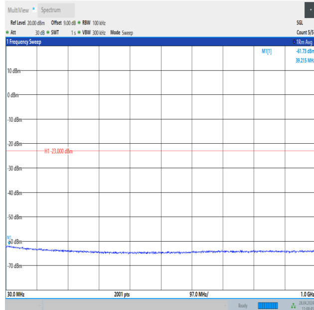
Band25_10MHz_16QAM_26365_1RB#0_30~1000_30~1000
