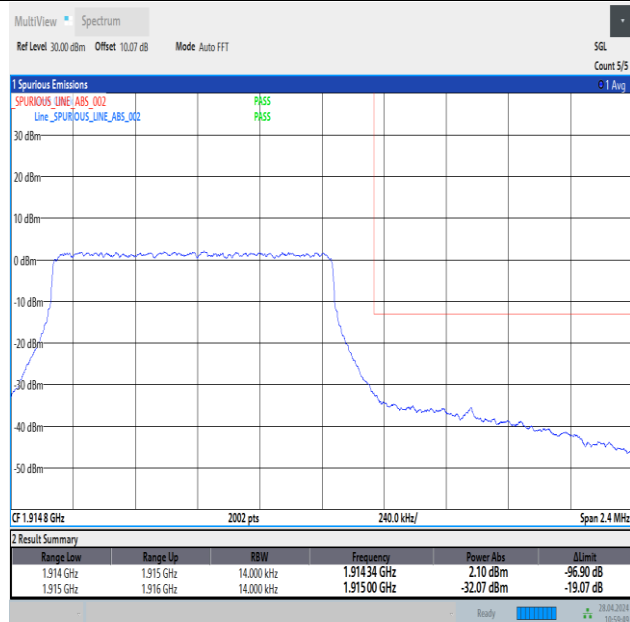
Band25_1.4MHz_16QAM_26683_6RB#0
