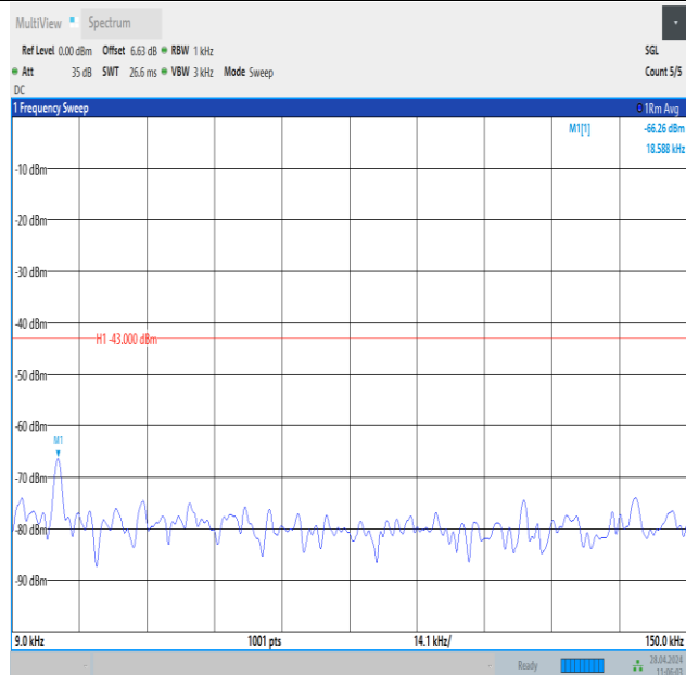
Band25_10MHz_QPSK_26090_1RB#49_0.009~0.15_0.009~0.15
