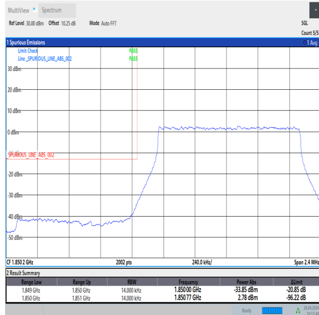
Band25_1.4MHz_QPSK_26047_6RB#0
