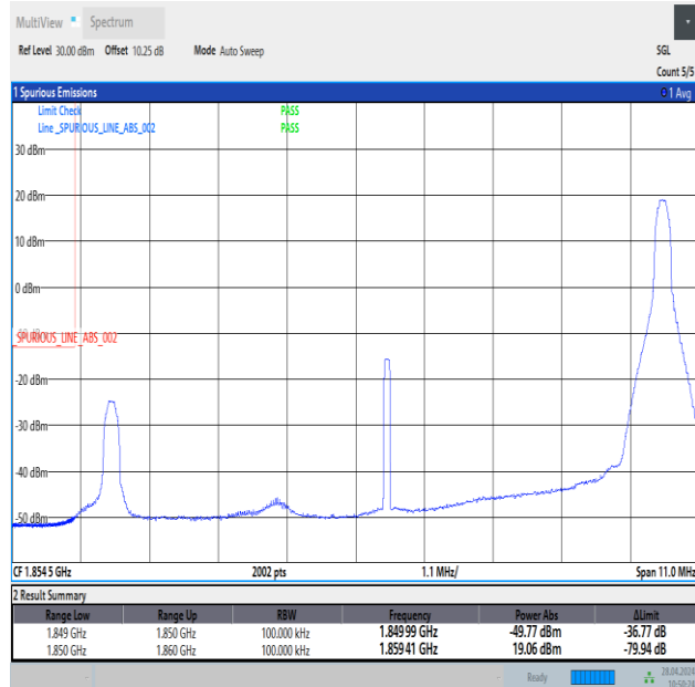
Band25_10MHz_QPSK_26090_1RB#49
