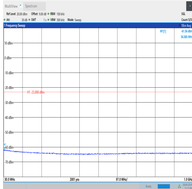
Band25_10MHz_16QAM_26640_1RB#49_30~1000_30~1000
