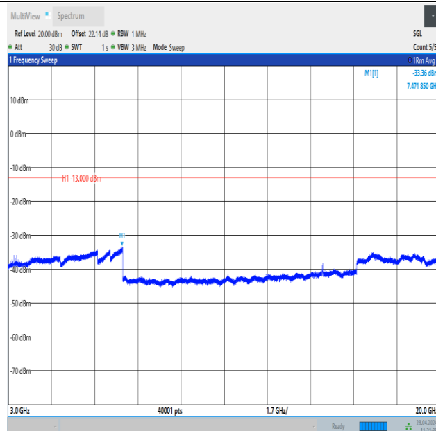
Band25_1.4MHz_16QAM_26047_1RB#5_3000~20000_3000~20000
