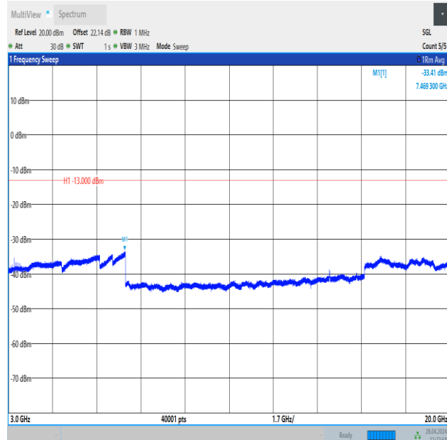
Band25_1.4MHz_16QAM_26365_6RB#0_3000~20000_3000~20000
