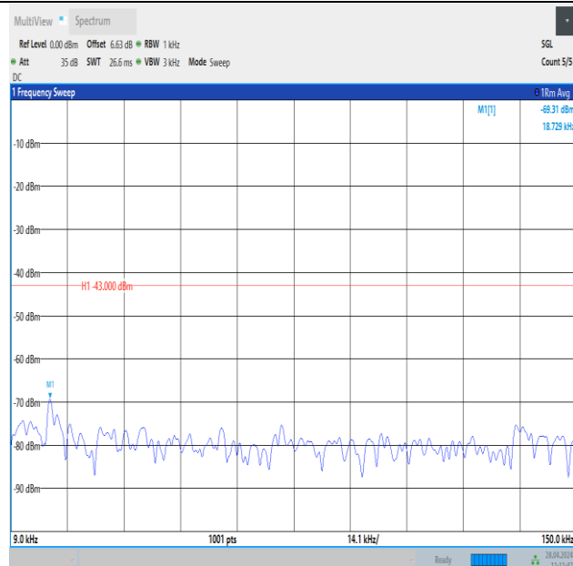
Band25_10MHz_16QAM_26640_1RB#0_0.009~0.15_0.009~0.15
