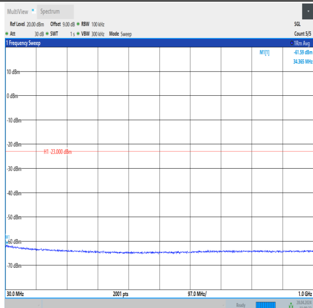
Band25_10MHz_QPSK_26365_1RB#49_30~1000_30~1000
