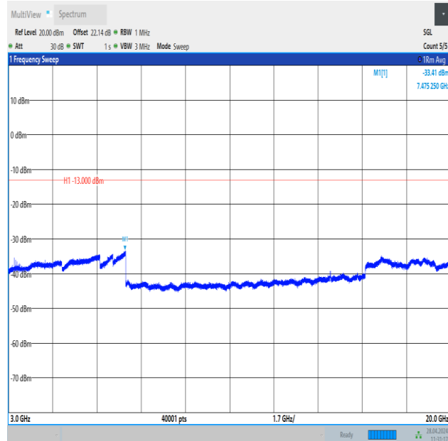
Band25_1.4MHz_16QAM_26683_1RB#5_3000~20000_3000~20000
