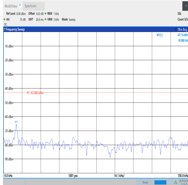
Band25_1.4MHz_16QAM_26047_1RB#0_0.009~0.15_0.009~0.15
