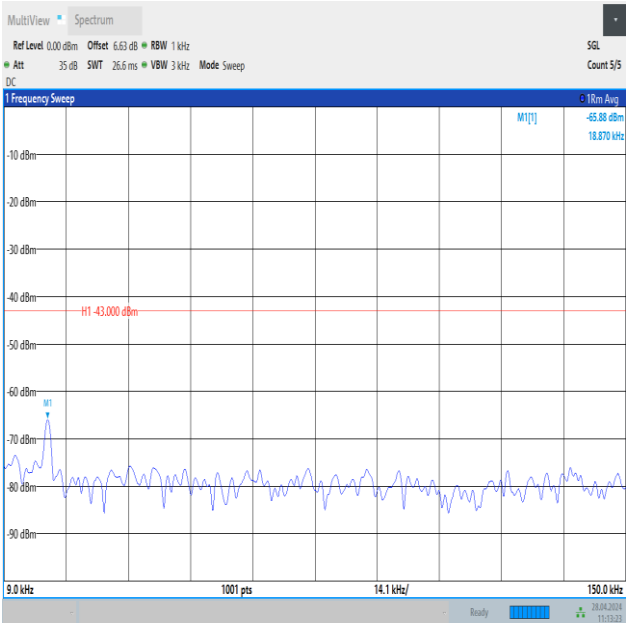
Band25_10MHz_16QAM_26640_1RB#49_0.009~0.15_0.009~0.15
