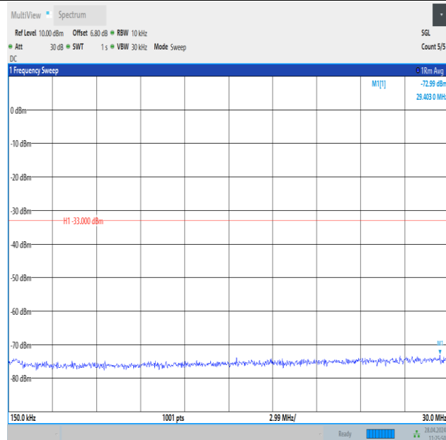
Band25_1.4MHz_16QAM_26365_1RB#5_0.15~30_0.15~30
