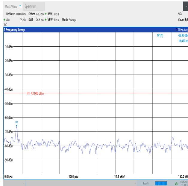
Band25_1.4MHz_QPSK_26365_1RB#5_0.009~0.15_0.009~0.15
