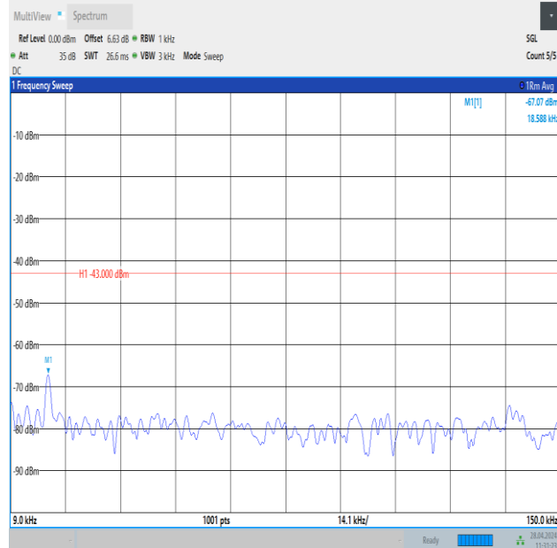
Band25_1.4MHz_QPSK_26683_6RB#0_0.009~0.15_0.009~0.15
