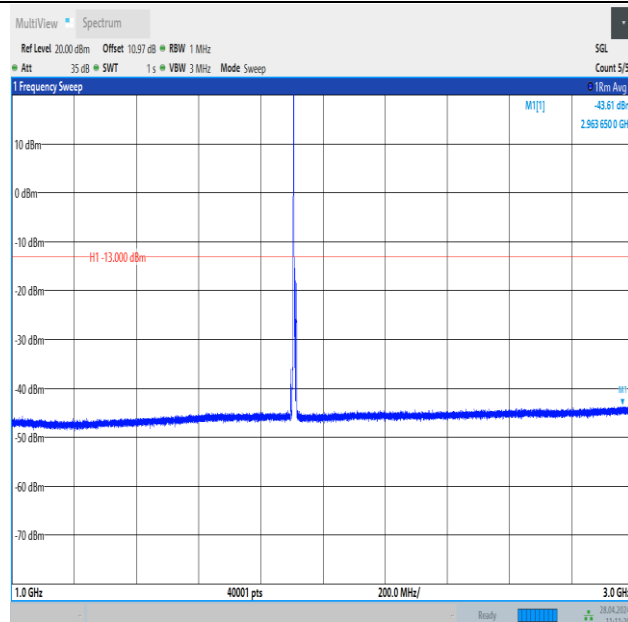
Band25_10MHz_QPSK_26640_1RB#0_1000~3000_1000~3000
