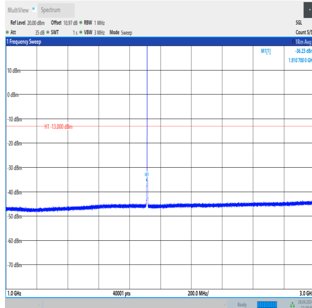
Band25_1.4MHz_QPSK_26683_1RB#0_1000~3000_1000~3000
