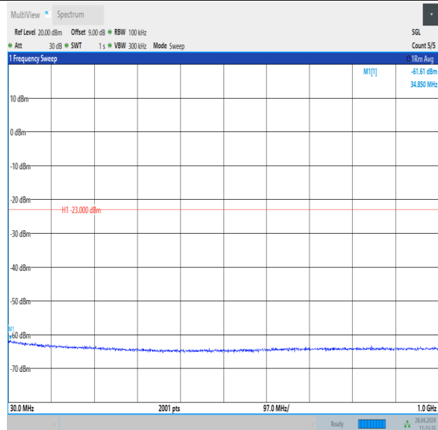
Band25_1.4MHz_QPSK_26365_1RB#0_30~1000_30~1000
