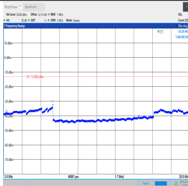
Band25_1.4MHz_QPSK_26683_6RB#0_3000~20000_3000~20000
