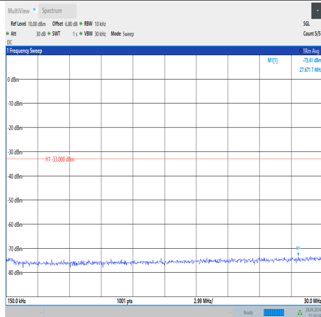
Band25_1.4MHz_16QAM_26365_1RB#0_0.15~30_0.15~30
