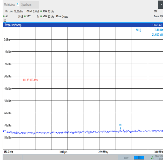
Band25_1.4MHz_16QAM_26683_1RB#5_0.15~30_0.15~30
