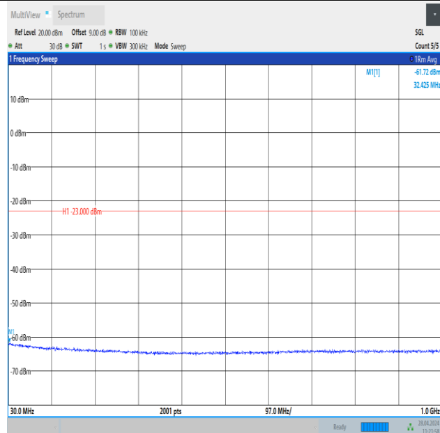
Band25_1.4MHz_QPSK_26047_6RB#0_30~1000_30~1000
