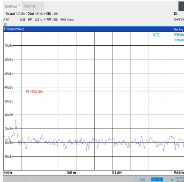
Band25_1.4MHz_QPSK_26365_6RB#0_0.009~0.15_0.009~0.15
