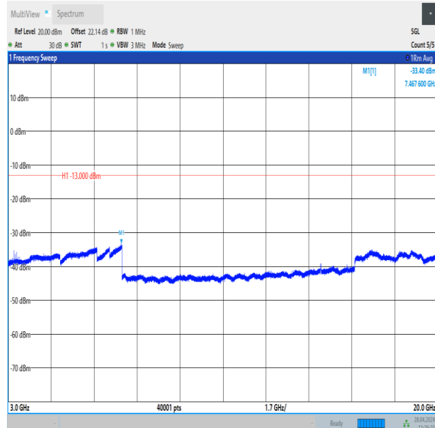
Band25_1.4MHz_16QAM_26365_1RB#5_3000~20000_3000~20000
