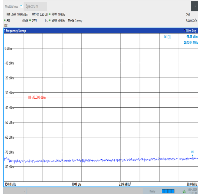
Band25_1.4MHz_QPSK_26365_1RB#0_0.15~30_0.15~30
