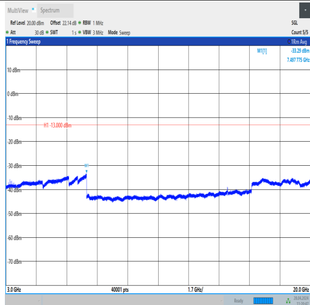
Band25_1.4MHz_QPSK_26047_1RB#5_3000~20000_3000~20000
