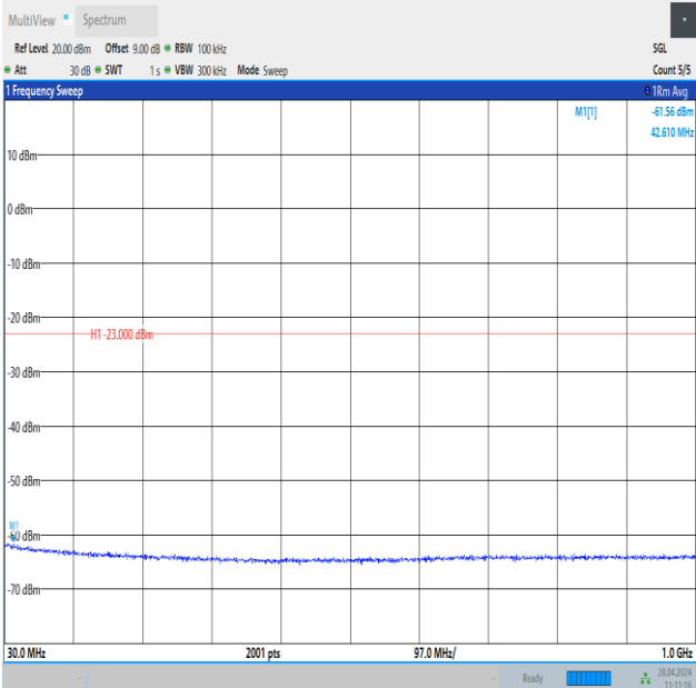
Band25_10MHz_QPSK_26640_1RB#0_30~1000_30~1000
