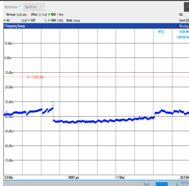
Band25_1.4MHz_QPSK_26683_1RB#0_3000~20000_3000~20000
