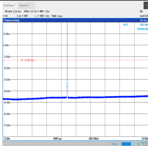
Band25_1.4MHz_16QAM_26365_1RB#0_1000~3000_1000~3000
