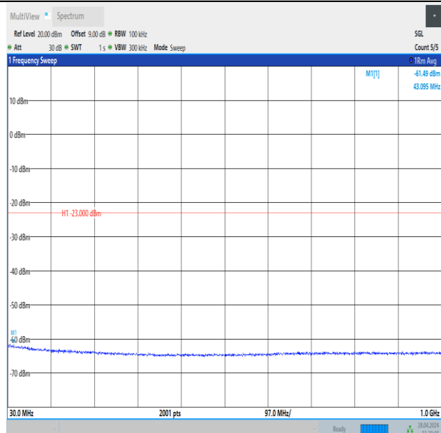
Band25_1.4MHz_QPSK_26683_1RB#5_30~1000_30~1000
