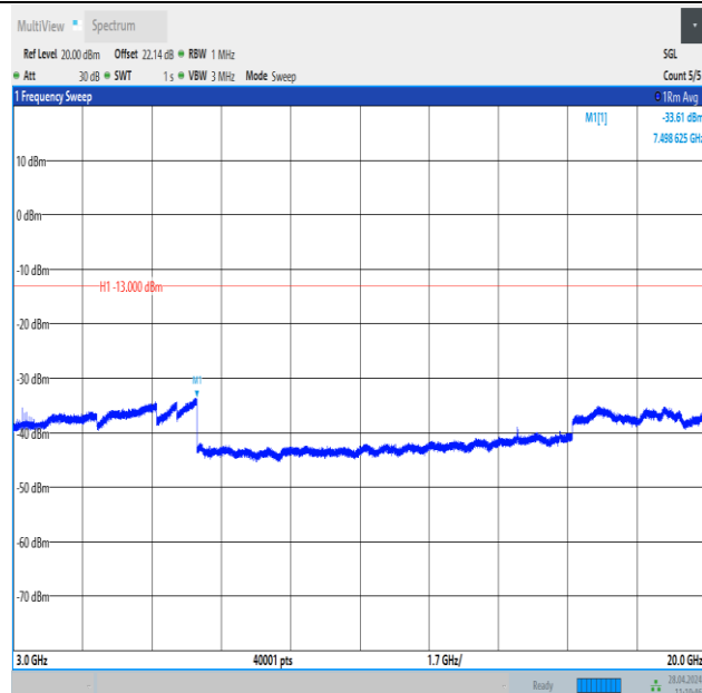
Band25_10MHz_16QAM_26365_1RB#49_3000~20000_3000~20000
