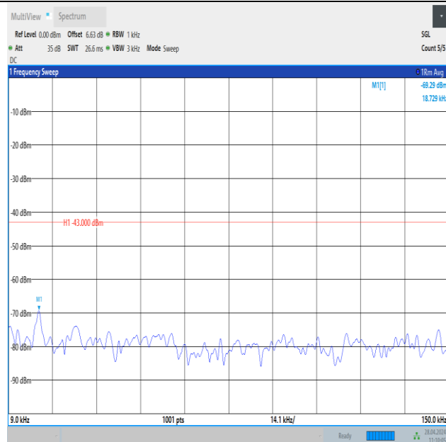
Band25_10MHz_16QAM_26365_1RB#49_0.009~0.15_0.009~0.15
