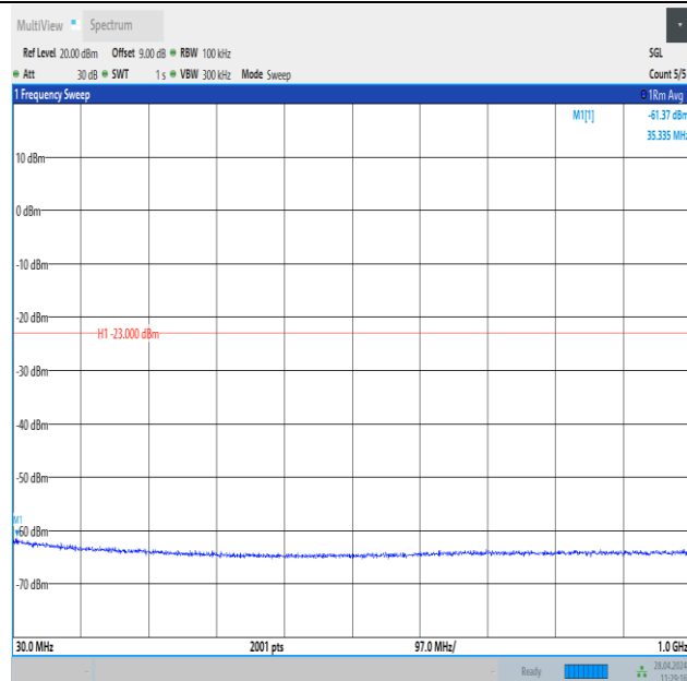
Band25_1.4MHz_16QAM_26683_1RB#0_30~1000_30~1000
