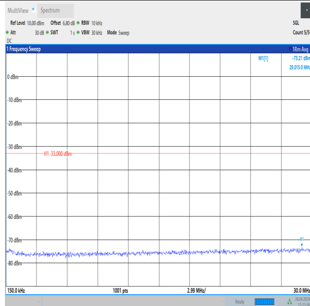
Band25_10MHz_16QAM_26640_1RB#0_0.15~30_0.15~30
