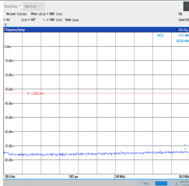
Band25_1.4MHz_16QAM_26683_6RB#0_0.15~30_0.15~30
