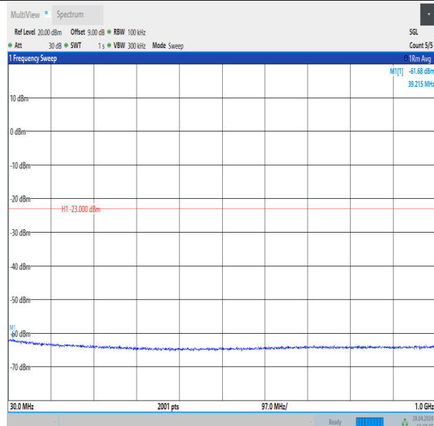
Band25_1.4MHz_QPSK_26047_1RB#0_30~1000_30~1000
