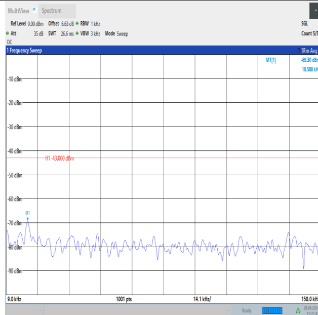
Band25_1.4MHz_QPSK_26047_6RB#0_0.009~0.15_0.009~0.15
