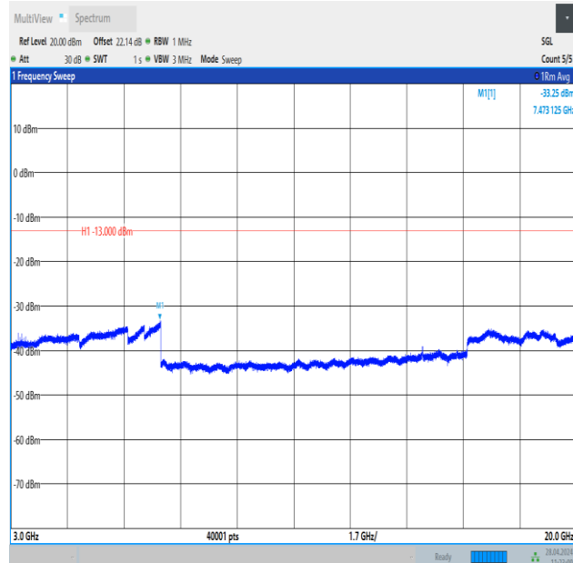
Band25_1.4MHz_16QAM_26047_6RB#0_3000~20000_3000~20000
