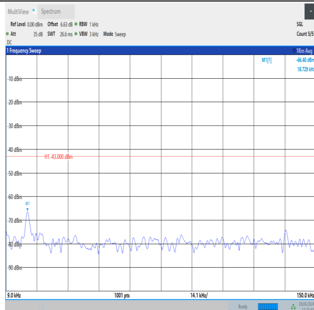
Band25_1.4MHz_16QAM_26365_1RB#5_0.009~0.15_0.009~0.15
