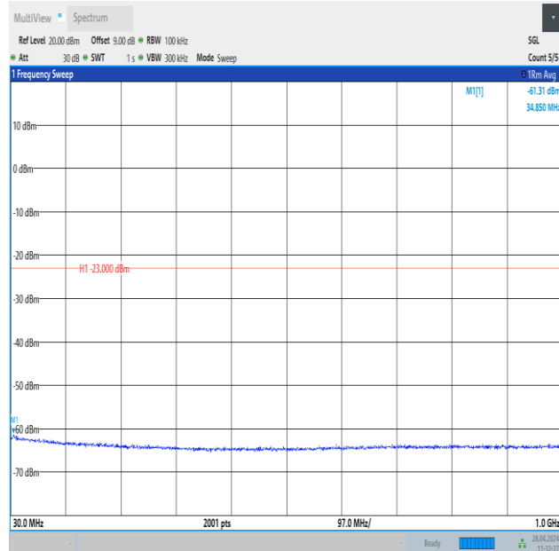
Band25_1.4MHz_16QAM_26683_6RB#0_30~1000_30~1000
