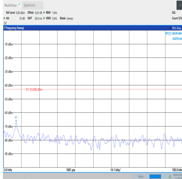
Band25_1.4MHz_QPSK_26047_1RB#0_0.009~0.15_0.009~0.15
