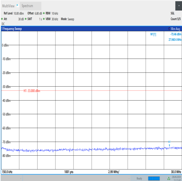
Band25_10MHz_QPSK_26640_1RB#0_0.15~30_0.15~30
