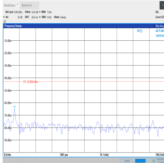
Band25_1.4MHz_16QAM_26047_1RB#5_0.009~0.15_0.009~0.15
