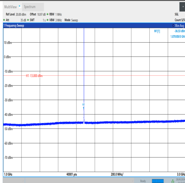
Band25_1.4MHz_QPSK_26365_1RB#0_1000~3000_1000~3000
