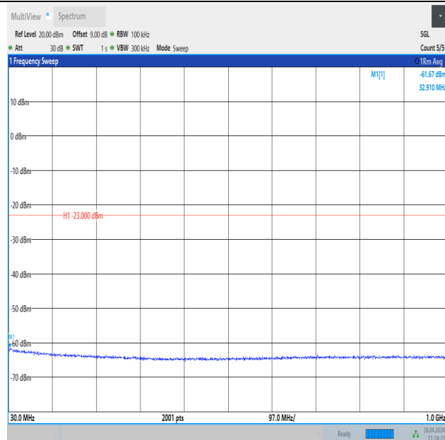
Band25_1.4MHz_16QAM_26365_1RB#0_30~1000_30~1000
