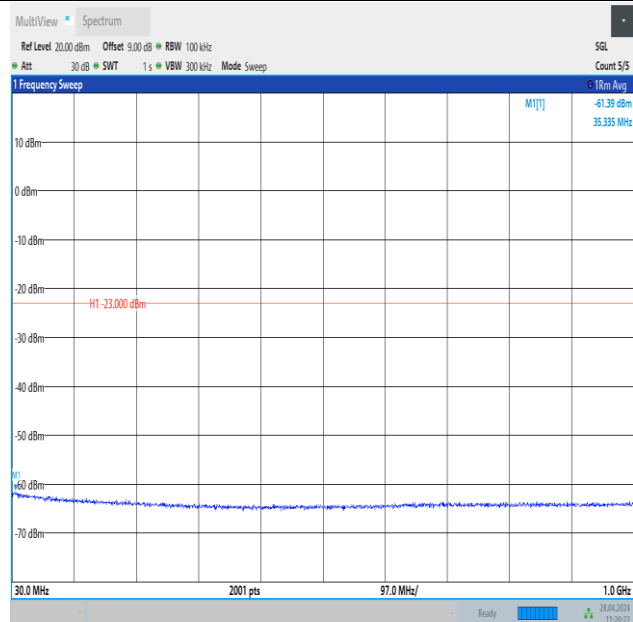
Band25_1.4MHz_QPSK_26047_1RB#5_30~1000_30~1000
