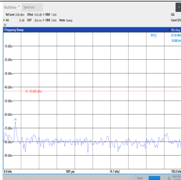
Band25_1.4MHz_16QAM_26683_1RB#0_0.009~0.15_0.009~0.15
