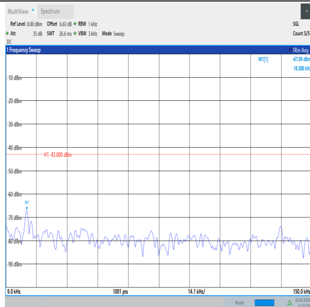
Band25_1.4MHz_16QAM_26683_6RB#0_0.009~0.15_0.009~0.15
