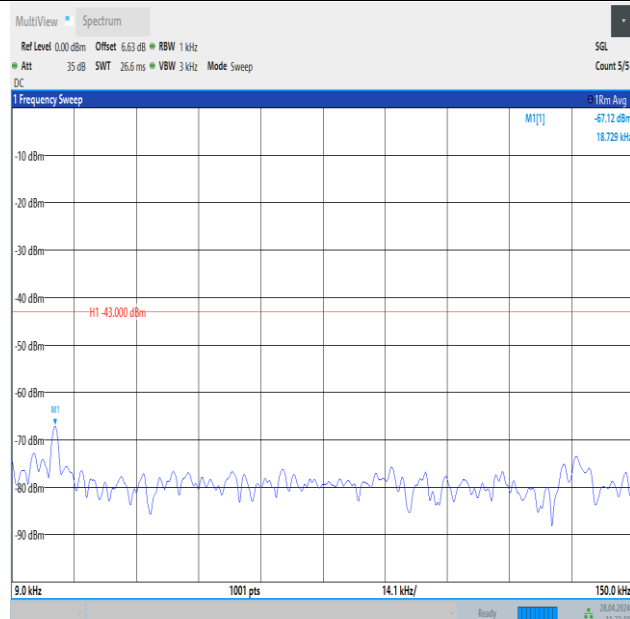
Band25_1.4MHz_QPSK_26365_1RB#0_0.009~0.15_0.009~0.15
