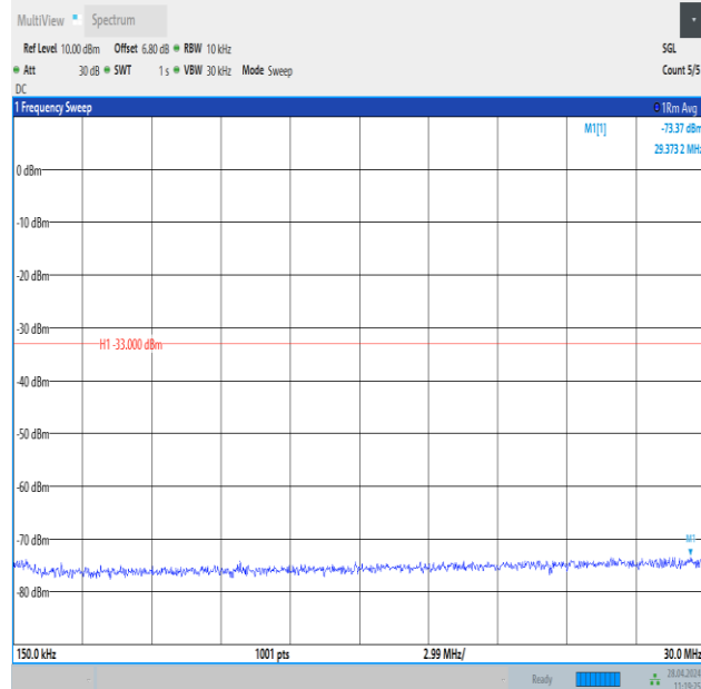
Band25_1.4MHz_16QAM_26047_1RB#0_0.15~30_0.15~30
