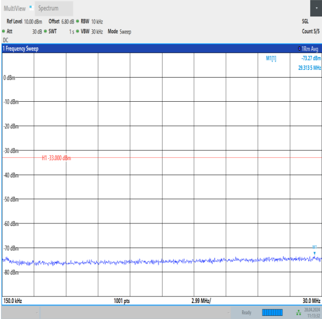
Band25_10MHz_16QAM_26640_1RB#49_0.15~30_0.15~30
