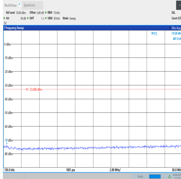
Band25_1.4MHz_16QAM_26047_1RB#5_0.15~30_0.15~30
