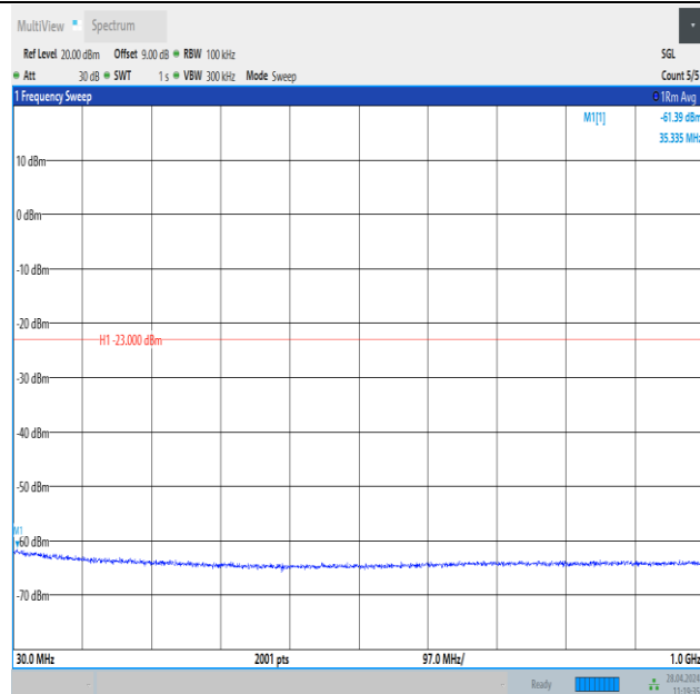
Band25_1.4MHz_16QAM_26047_1RB#0_30~1000_30~1000
