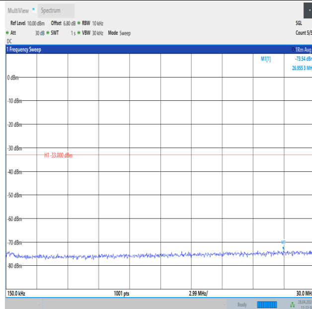
Band25_1.4MHz_16QAM_26047_6RB#0_0.15~30_0.15~30
