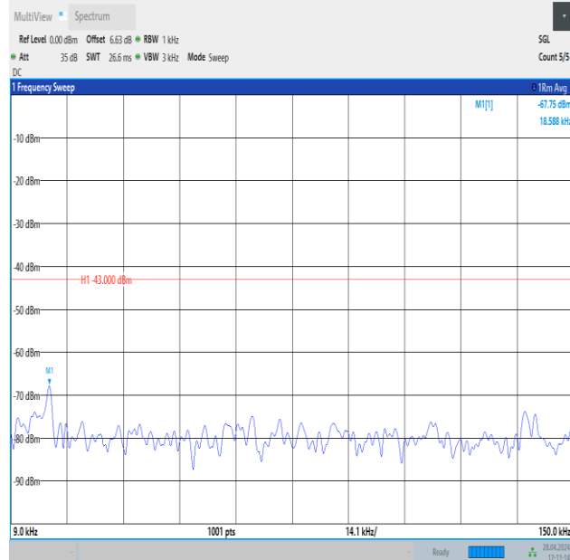
Band25_15MHz_16QAM_26115_1RB#0_0.009~0.15_0.009~0.15
