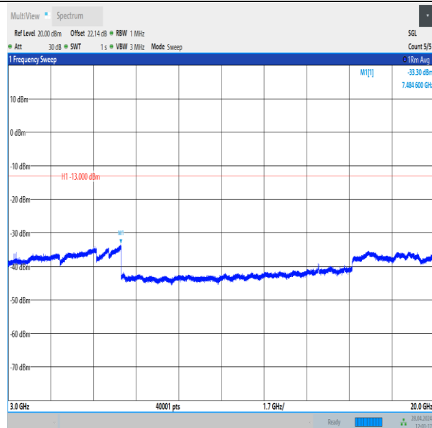
Band25_3MHz_QPSK_26365_15RB#0_3000~20000_3000~20000
