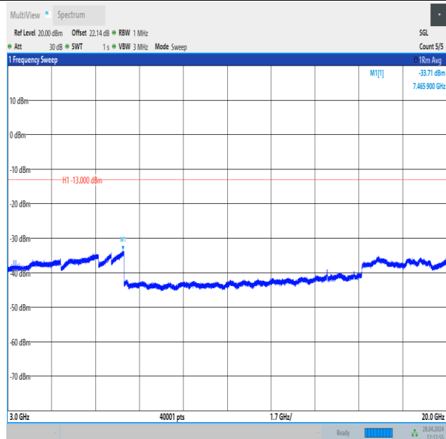
Band25_15MHz_16QAM_26115_1RB#0_3000~20000_3000~20000
