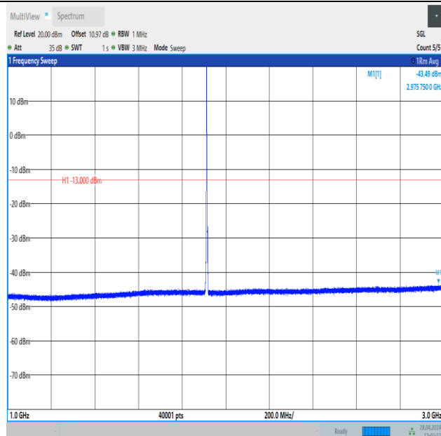
Band25_3MHz_16QAM_26675_1RB#0_1000~3000_1000~3000
