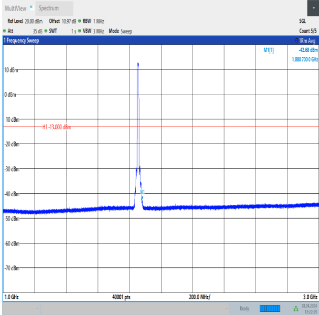
Band25_10MHz_QPSK_26090_50RB#0_1000~3000_1000~3000
