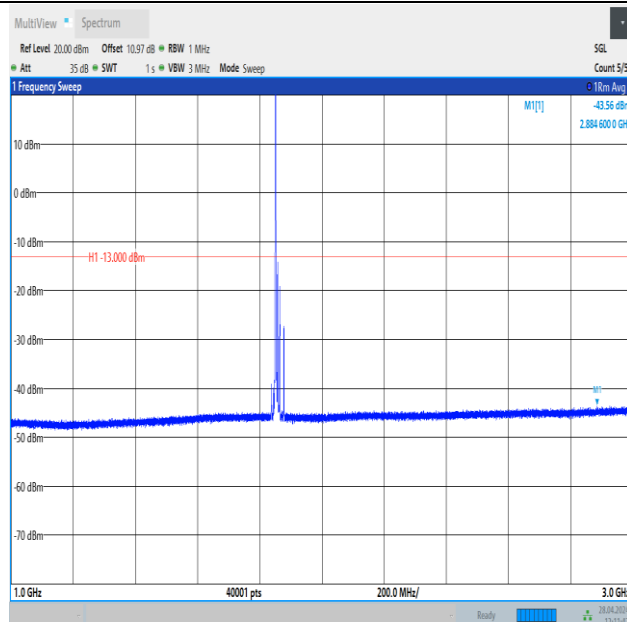
Band25_15MHz_16QAM_26115_1RB#0_1000~3000_1000~3000
