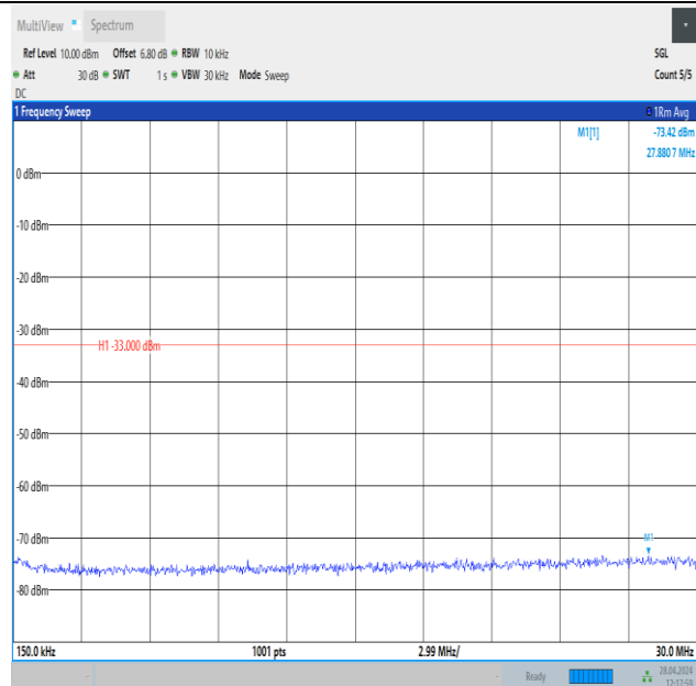
Band25_15MHz_16QAM_26615_1RB#0_0.15~30_0.15~30
