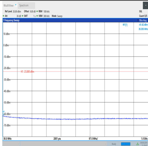
Band25_15MHz_16QAM_26615_1RB#0_30~1000_30~1000
