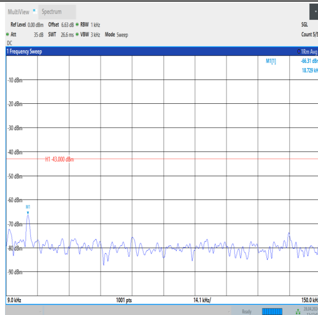
Band25_15MHz_QPSK_26615_1RB#0_0.009~0.15_0.009~0.15
