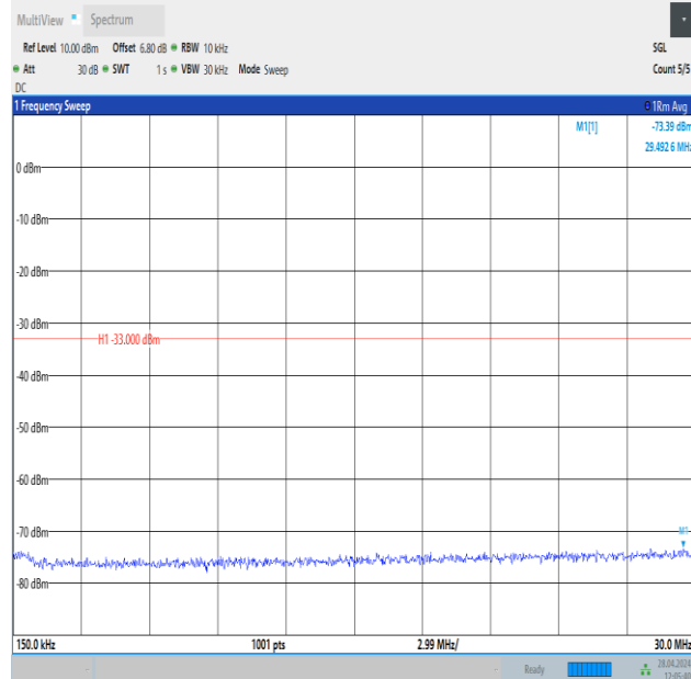
Band25_3MHz_QPSK_26675_15RB#0_0.15~30_0.15~30
