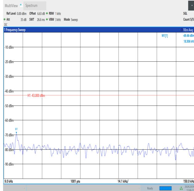
Band25_3MHz_16QAM_26675_15RB#0_0.009~0.15_0.009~0.15
