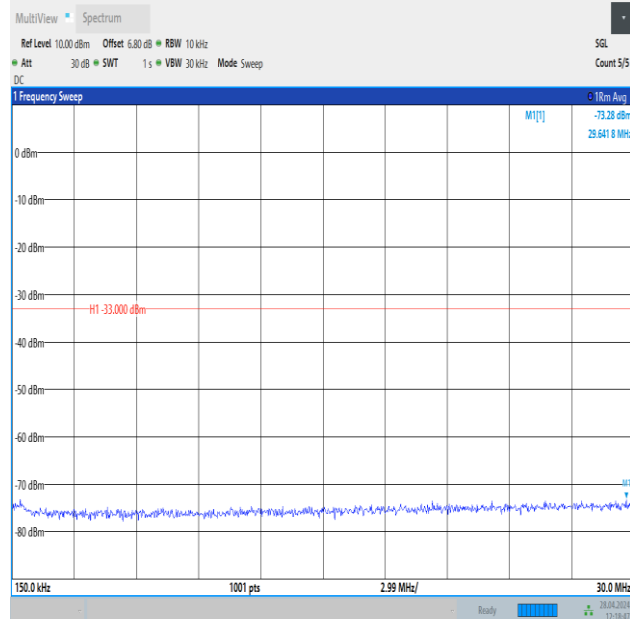
Band25_15MHz_QPSK_26615_1RB#74_0.15~30_0.15~30
