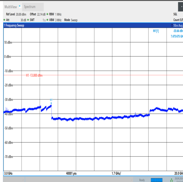
Band25_15MHz_QPSK_26615_1RB#0_3000~20000_3000~20000
