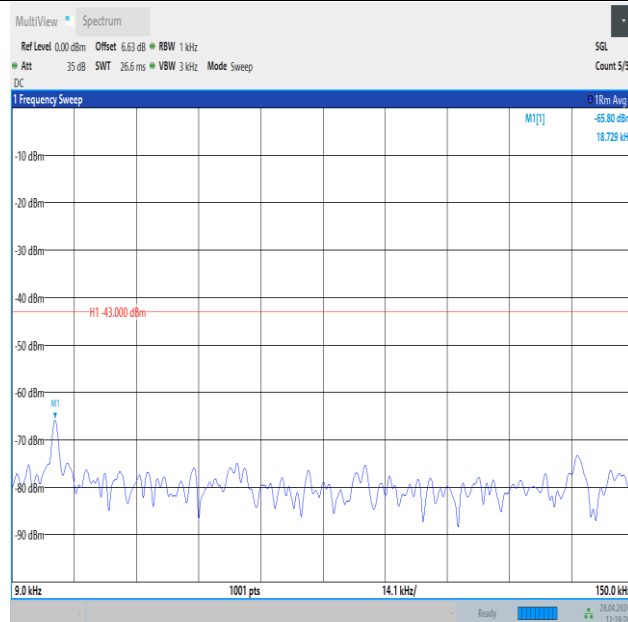
Band25_15MHz_16QAM_26615_1RB#74_0.009~0.15_0.009~0.15
