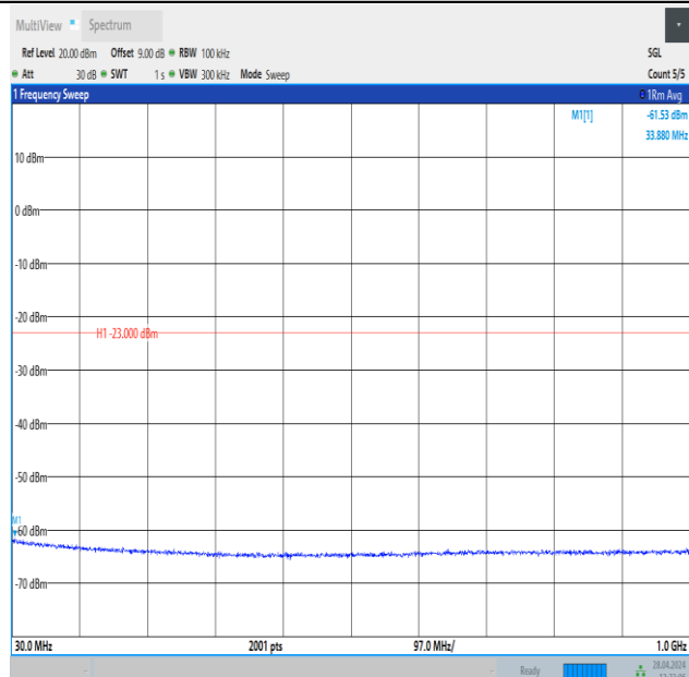
Band25_10MHz_QPSK_26365_50RB#0_30~1000_30~1000
