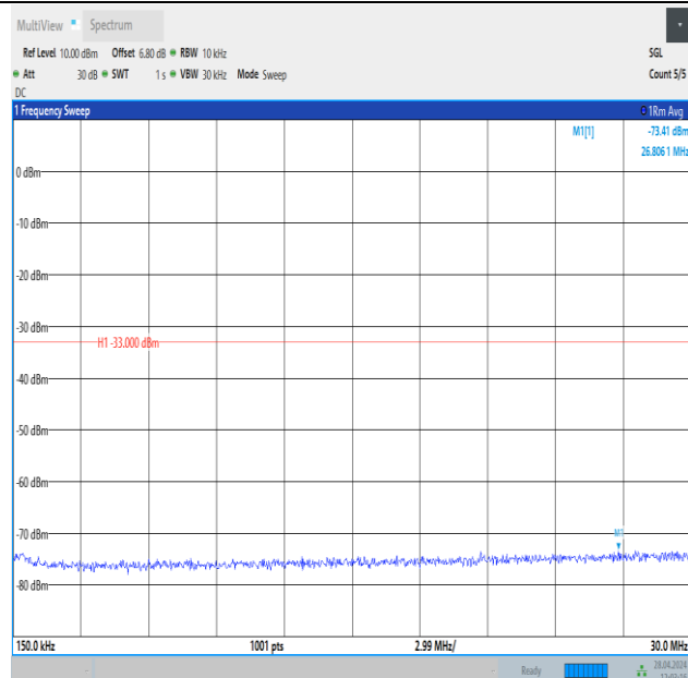
Band25_3MHz_16QAM_26675_1RB#0_0.15~30_0.15~30
