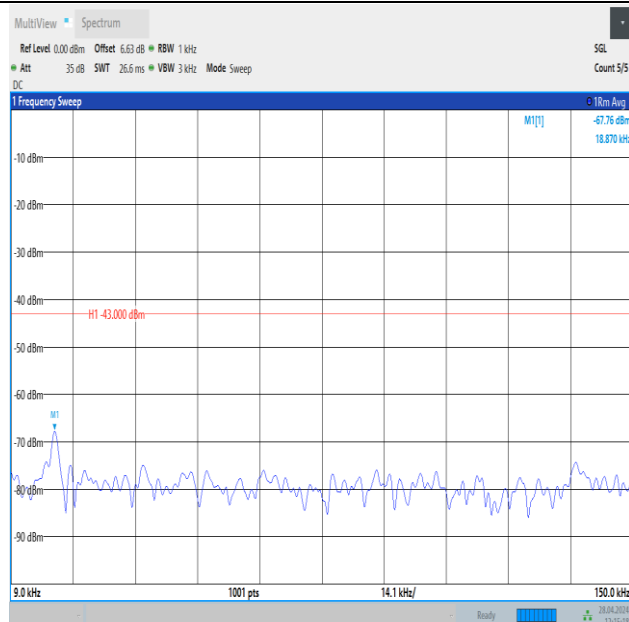
Band25_15MHz_QPSK_26365_1RB#74_0.009~0.15_0.009~0.15
