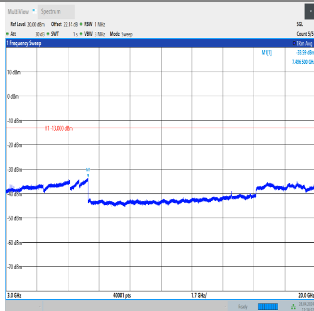
Band25_15MHz_QPSK_26365_1RB#0_3000~20000_3000~20000
