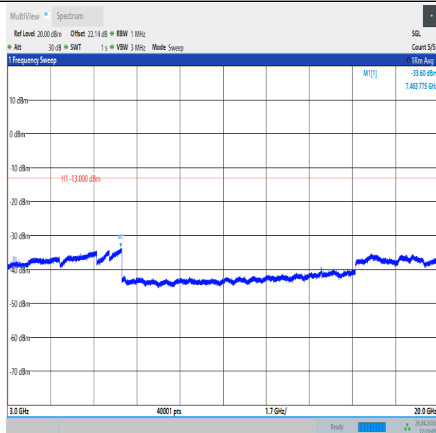
Band25_15MHz_16QAM_26615_1RB#74_3000~20000_3000~20000
