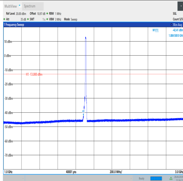
Band25_10MHz_QPSK_26640_50RB#0_1000~3000_1000~3000
