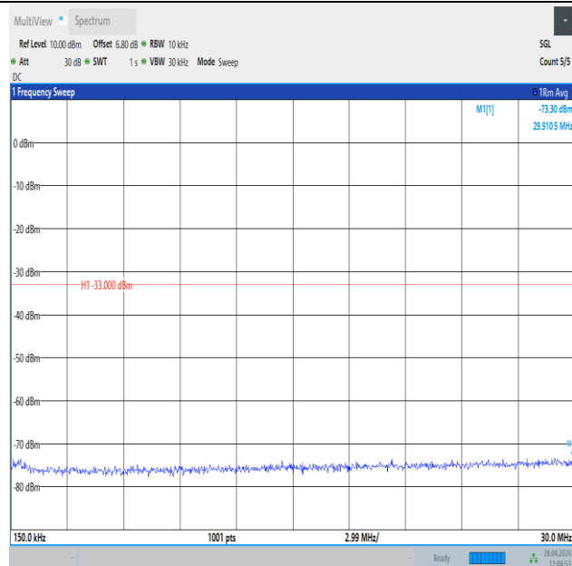
Band25_3MHz_16QAM_26675_1RB#14_0.15~30_0.15~30
