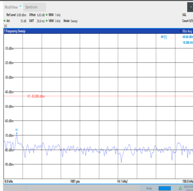
Band25_3MHz_QPSK_26675_15RB#0_0.009~0.15_0.009~0.15
