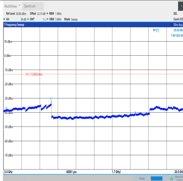
Band25_3MHz_16QAM_26675_1RB#14_3000~20000_3000~20000
