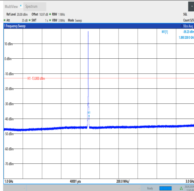
Band25_3MHz_QPSK_26365_15RB#0_1000~3000_1000~3000
