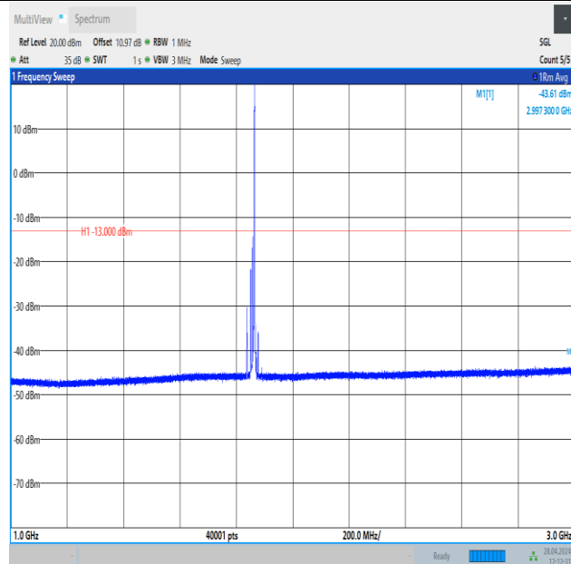
Band25_15MHz_QPSK_26115_1RB#74_1000~3000_1000~3000
