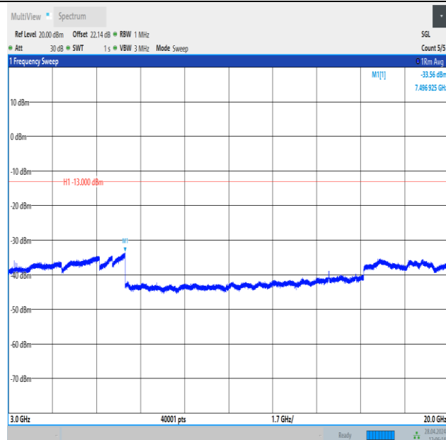
Band25_3MHz_QPSK_26675_15RB#0_3000~20000_3000~20000
