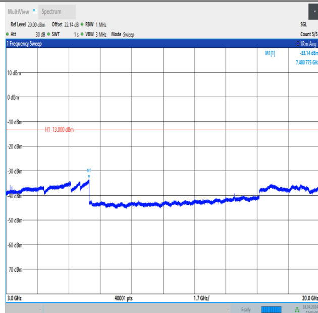
Band25_3MHz_QPSK_26675_1RB#0_3000~20000_3000~20000
