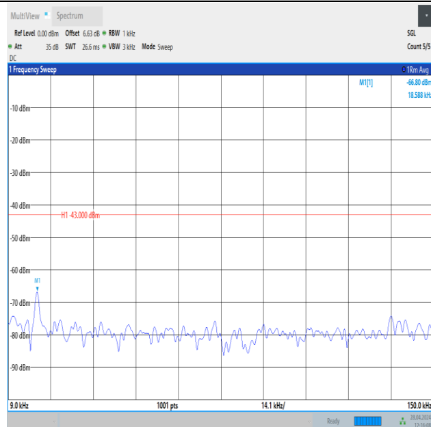
Band25_15MHz_16QAM_26365_1RB#74_0.009~0.15_0.009~0.15
