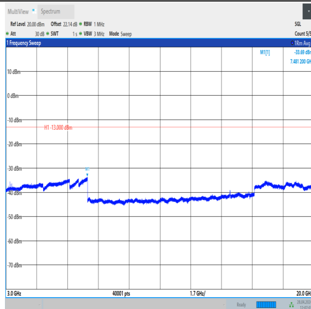
Band25_3MHz_16QAM_26675_15RB#0_3000~20000_3000~20000
