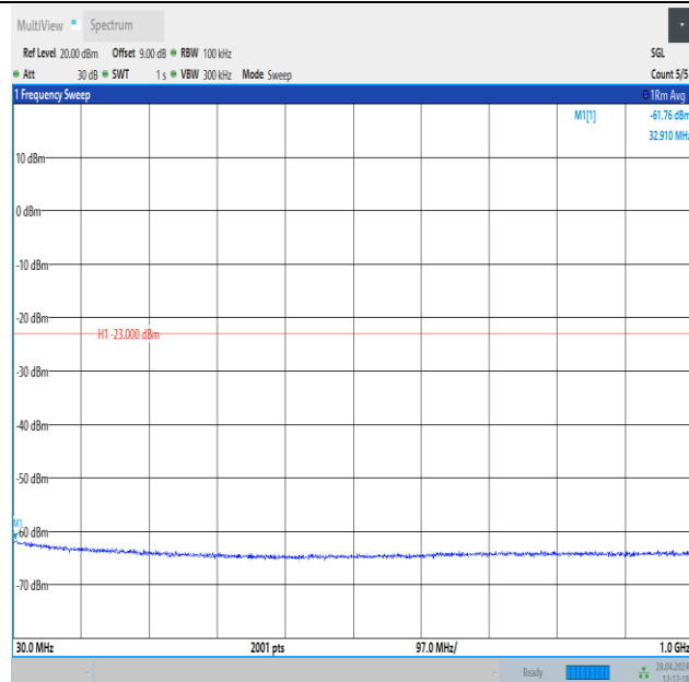
Band25_15MHz_QPSK_26615_1RB#0_30~1000_30~1000
