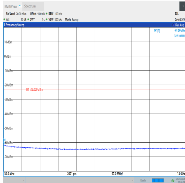
Band25_3MHz_16QAM_26365_1RB#14_30~1000_30~1000
