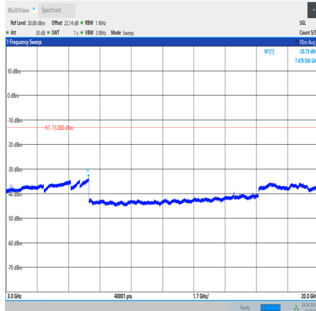
Band25_15MHz_QPSK_26615_1RB#74_3000~20000_3000~20000
