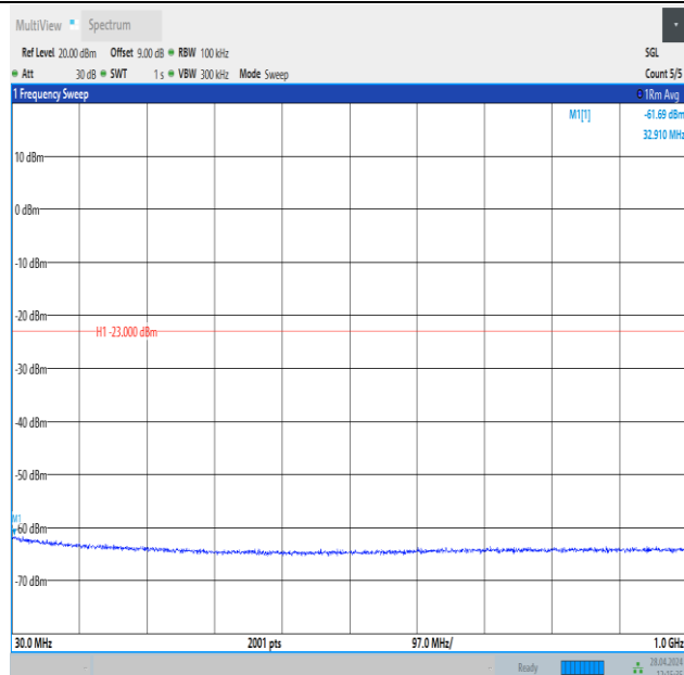
Band25_15MHz_QPSK_26365_1RB#74_30~1000_30~1000
