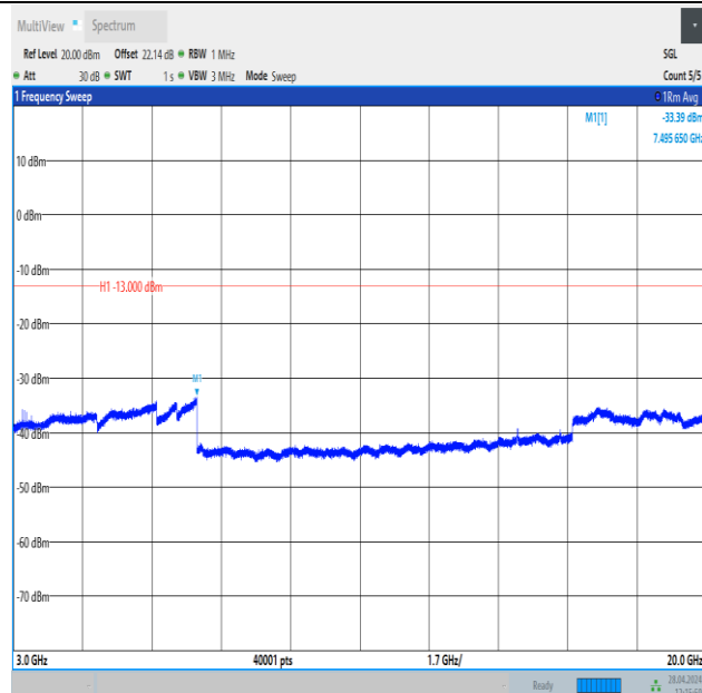
Band25_15MHz_QPSK_26365_1RB#74_3000~20000_3000~20000
