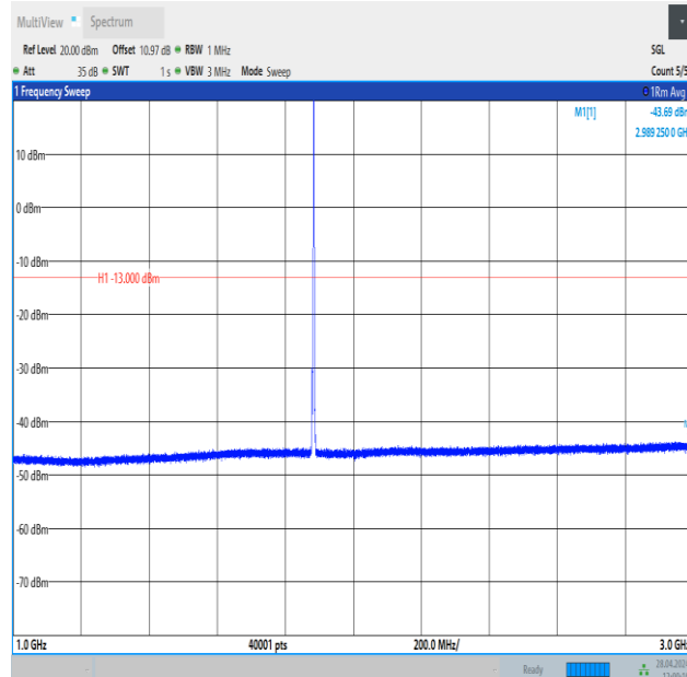
Band25_3MHz_16QAM_26365_1RB#14_1000~3000_1000~3000
