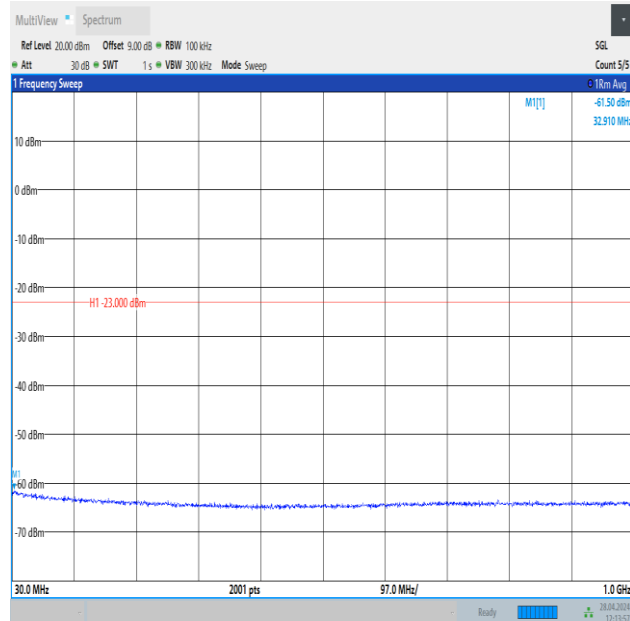
Band25_15MHz_QPSK_26365_1RB#0_30~1000_30~1000
