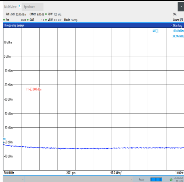
Band25_15MHz_16QAM_26365_1RB#74_30~1000_30~1000
