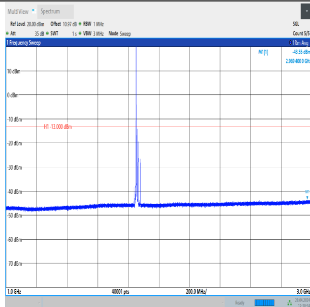
Band25_15MHz_QPSK_26115_1RB#0_1000~3000_1000~3000
