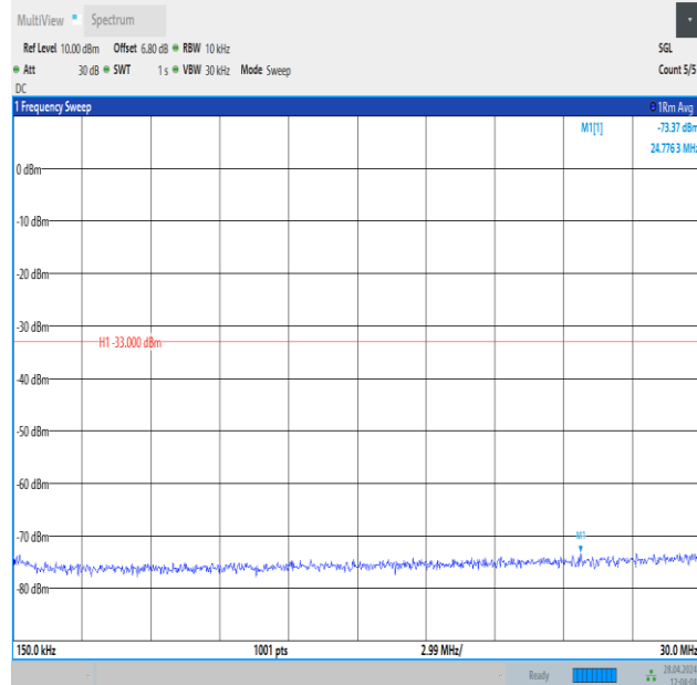
Band25_3MHz_QPSK_26675_1RB#14_0.15~30_0.15~30
