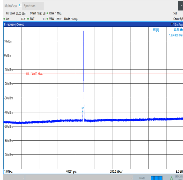
Band25_3MHz_16QAM_26365_15RB#0_1000~3000_1000~3000
