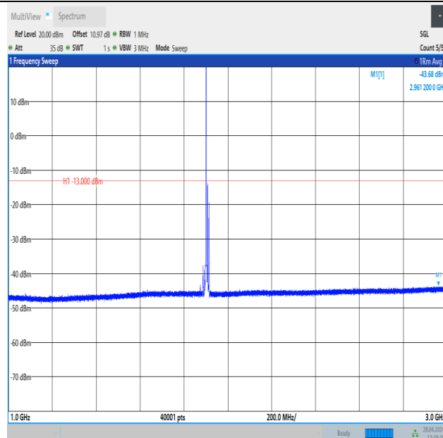
Band25_15MHz_16QAM_26615_1RB#0_1000~3000_1000~3000
