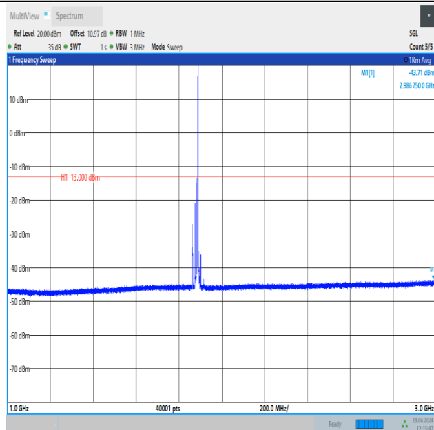
Band25_15MHz_QPSK_26365_1RB#74_1000~3000_1000~3000
