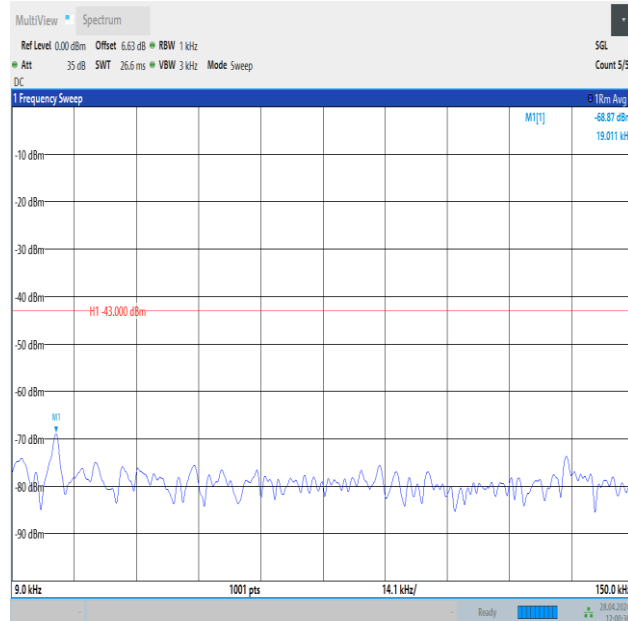
Band25_3MHz_QPSK_26365_15RB#0_0.009~0.15_0.009~0.15
