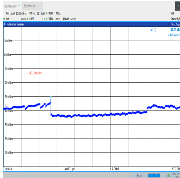
Band25_3MHz_16QAM_26365_15RB#0_3000~20000_3000~20000
