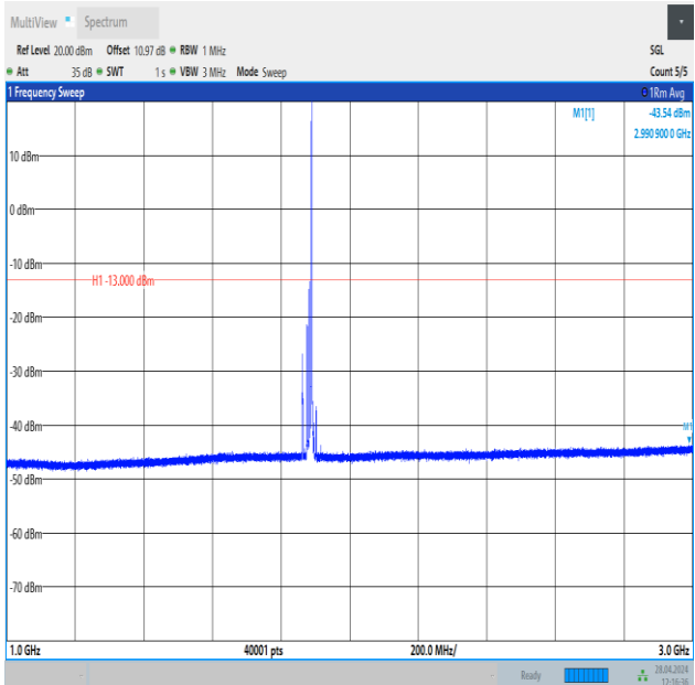
Band25_15MHz_16QAM_26365_1RB#74_1000~3000_1000~3000
