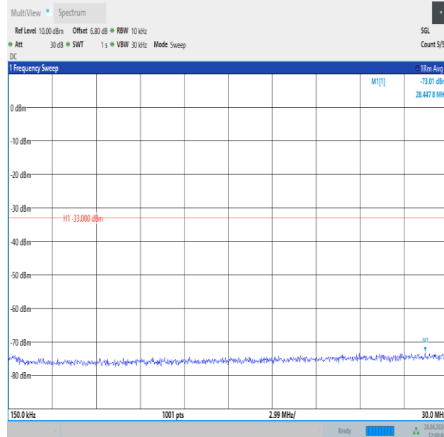
Band25_3MHz_QPSK_26365_15RB#0_0.15~30_0.15~30
