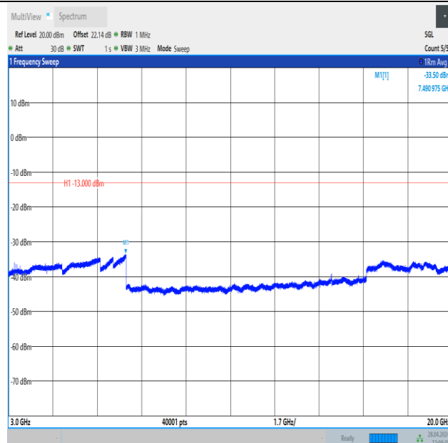
Band25_3MHz_QPSK_26675_1RB#14_3000~20000_3000~20000
