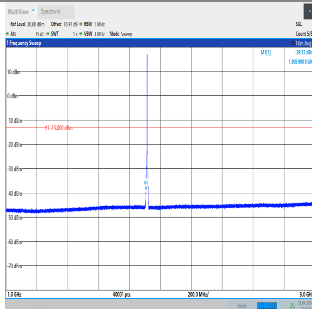
Band25_3MHz_16QAM_26675_15RB#0_1000~3000_1000~3000
