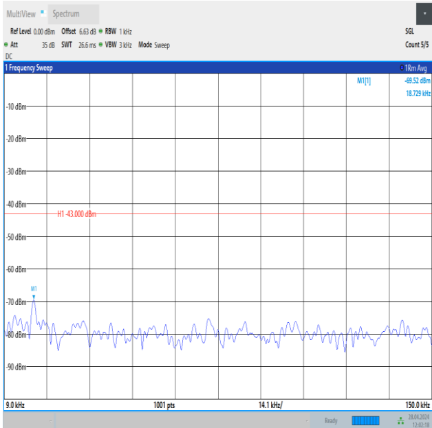
Band25_3MHz_QPSK_26675_1RB#0_0.009~0.15_0.009~0.15
