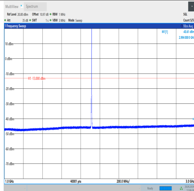
Band25_3MHz_QPSK_26675_1RB#14_1000~3000_1000~3000
