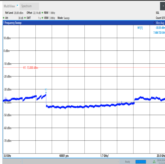
Band25_15MHz_16QAM_26115_1RB#74_3000~20000_3000~20000
