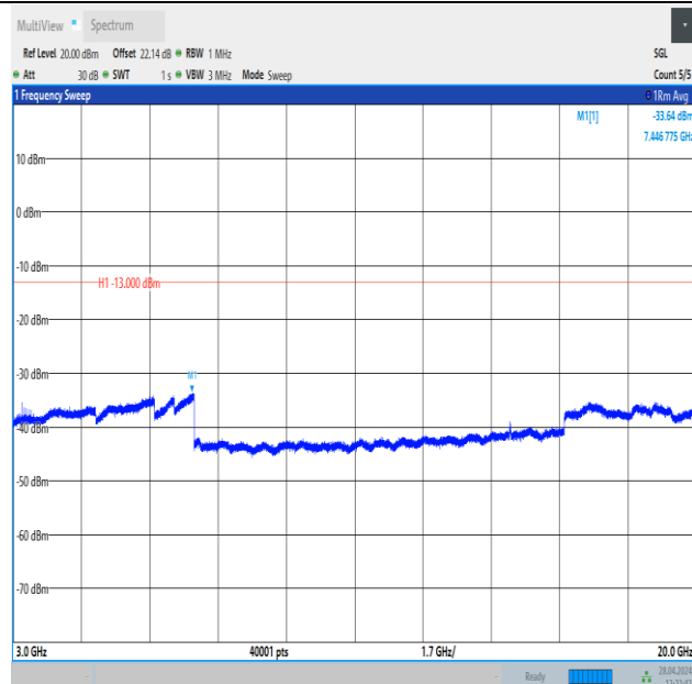
Band25_10MHz_QPSK_26090_50RB#0_3000~20000_3000~20000
