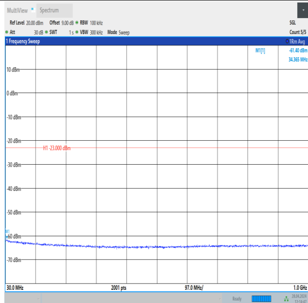
Band25_15MHz_16QAM_26365_1RB#0_30~1000_30~1000
