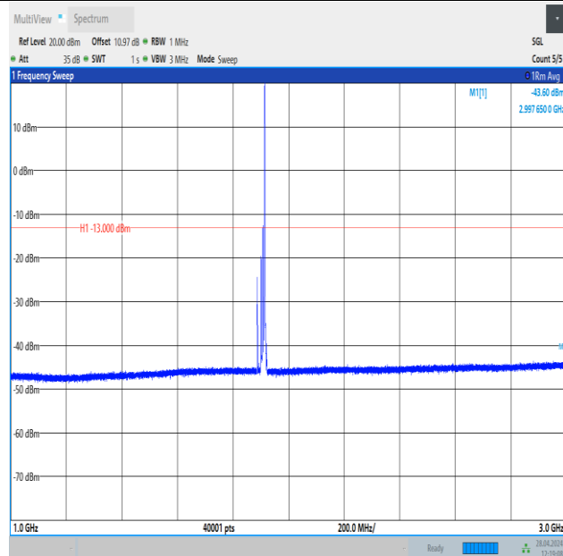
Band25_15MHz_QPSK_26615_1RB#74_1000~3000_1000~3000
