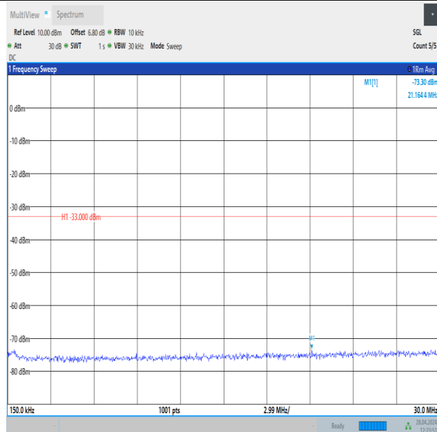
Band25_10MHz_QPSK_26640_50RB#0_0.15~30_0.15~30
