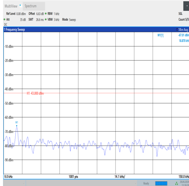
Band25_15MHz_QPSK_26615_1RB#74_0.009~0.15_0.009~0.15
