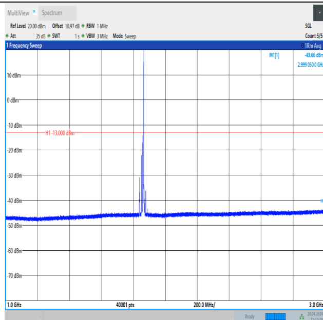
Band25_15MHz_16QAM_26115_1RB#74_1000~3000_1000~3000
