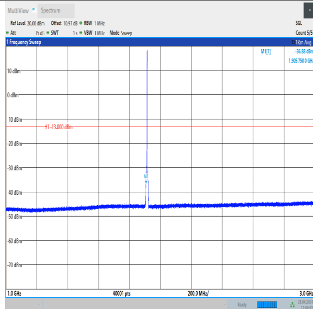
Band25_3MHz_QPSK_26675_15RB#0_1000~3000_1000~3000
