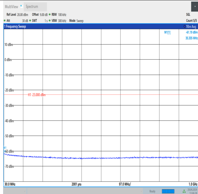
Band25_3MHz_16QAM_26675_15RB#0_30~1000_30~1000
