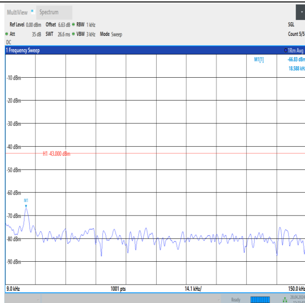
Band25_10MHz_QPSK_26640_50RB#0_0.009~0.15_0.009~0.15
