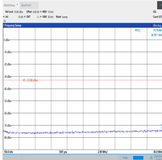
Band25_3MHz_16QAM_26365_1RB#14_0.15~30_0.15~30
