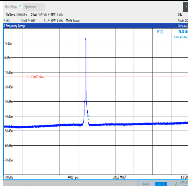
Band25_10MHz_QPSK_26365_50RB#0_1000~3000_1000~3000
