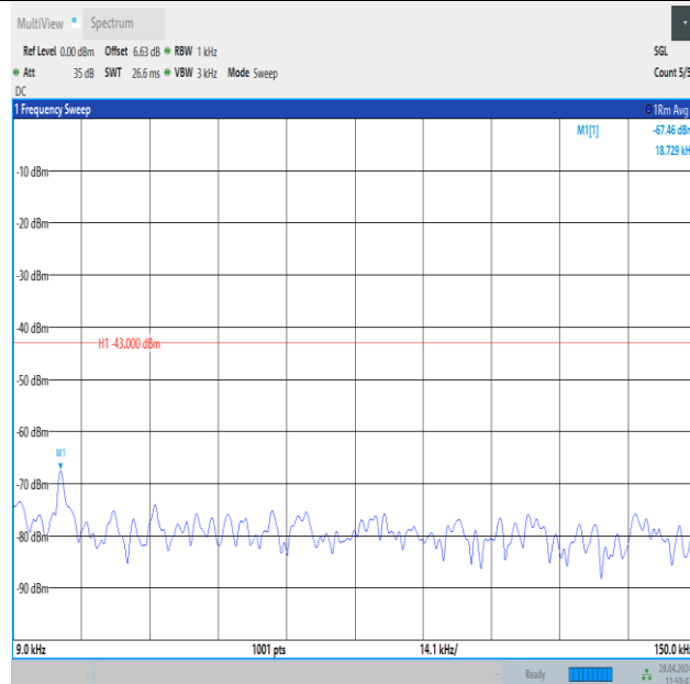
Band25_3MHz_16QAM_26365_1RB#14_0.009~0.15_0.009~0.15
