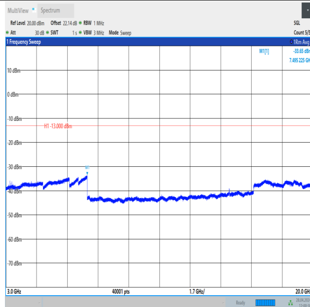
Band25_3MHz_16QAM_26365_1RB#14_3000~20000_3000~20000
