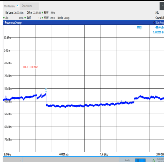
Band25_3MHz_QPSK_26365_1RB#14_3000~20000_3000~20000
