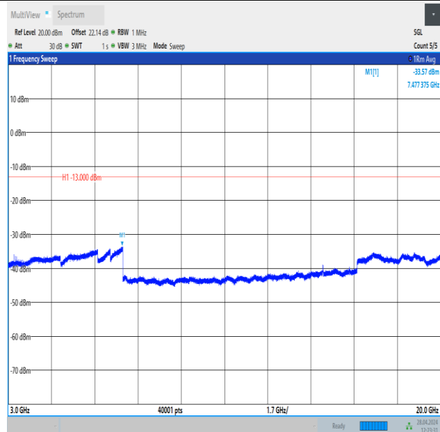
Band25_10MHz_QPSK_26365_50RB#0_3000~20000_3000~20000
