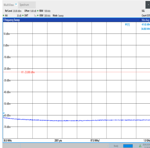
Band25_15MHz_QPSK_26615_1RB#74_30~1000_30~1000
