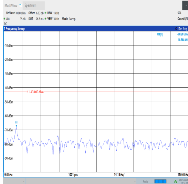
Band25_15MHz_16QAM_26365_1RB#0_0.009~0.15_0.009~0.15
