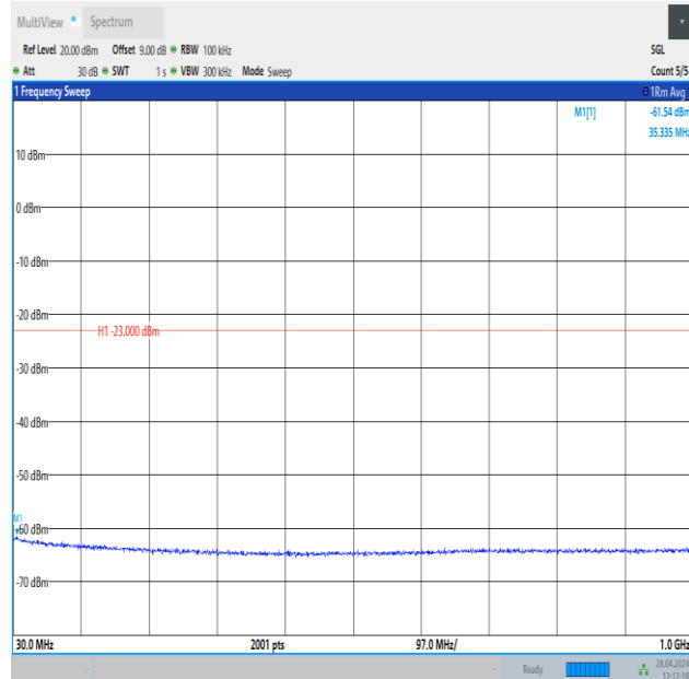
Band25_15MHz_QPSK_26115_1RB#74_30~1000_30~1000
