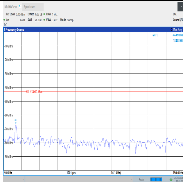
Band25_3MHz_QPSK_26675_1RB#14_0.009~0.15_0.009~0.15
