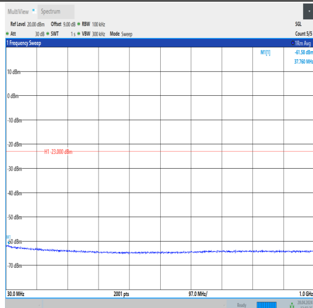
Band25_3MHz_16QAM_26675_1RB#0_30~1000_30~1000
