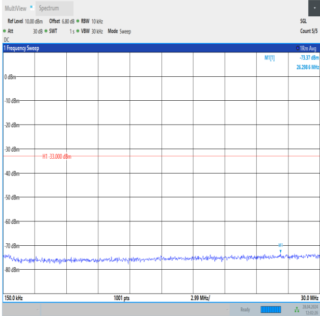
Band25_3MHz_QPSK_26675_1RB#0_0.15~30_0.15~30
