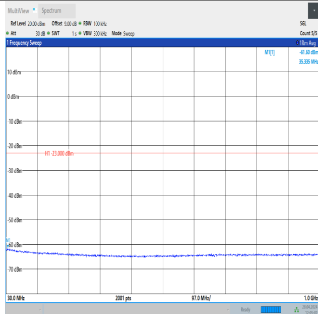
Band25_3MHz_16QAM_26675_1RB#14_30~1000_30~1000
