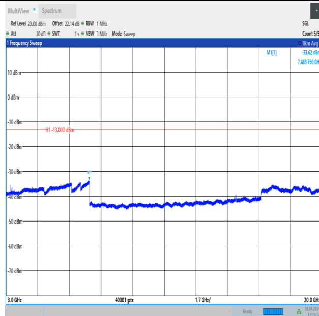
Band25_15MHz_16QAM_26365_1RB#0_3000~20000_3000~20000
