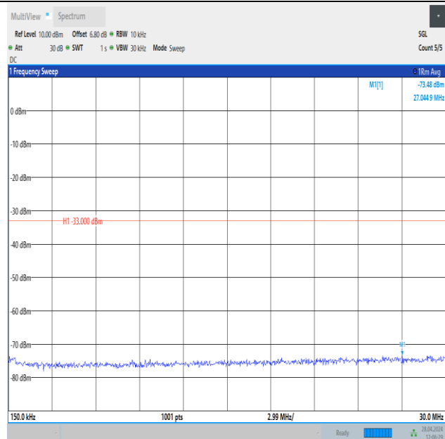
Band25_3MHz_16QAM_26675_15RB#0_0.15~30_0.15~30
