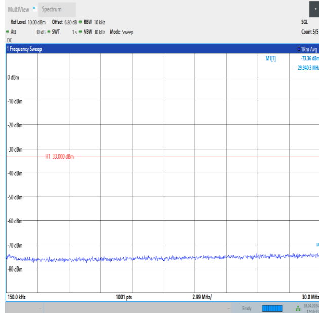
Band25_15MHz_QPSK_26115_1RB#0_0.15~30_0.15~30
