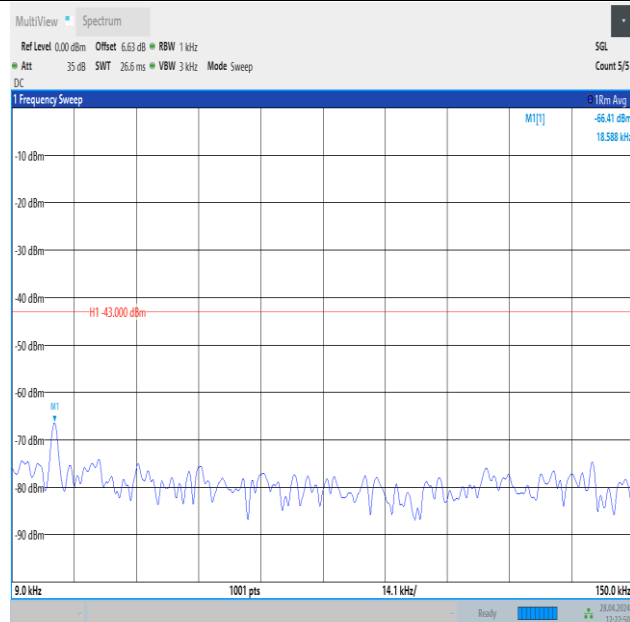
Band25_10MHz_QPSK_26365_50RB#0_0.009~0.15_0.009~0.15
