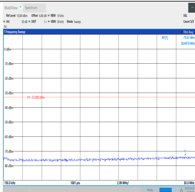
Band25_15MHz_16QAM_26365_1RB#74_0.15~30_0.15~30
