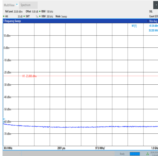
Band25_3MHz_QPSK_26675_15RB#0_30~1000_30~1000
