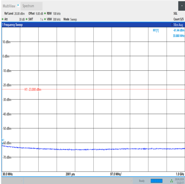
Band25_10MHz_QPSK_26090_50RB#0_30~1000_30~1000
