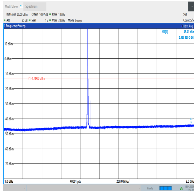
Band25_15MHz_QPSK_26365_1RB#0_1000~3000_1000~3000
