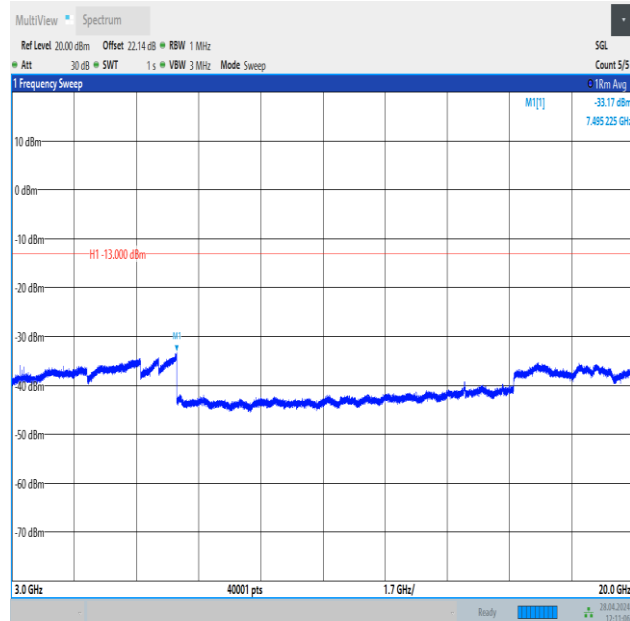
Band25_15MHz_QPSK_26115_1RB#0_3000~20000_3000~20000
