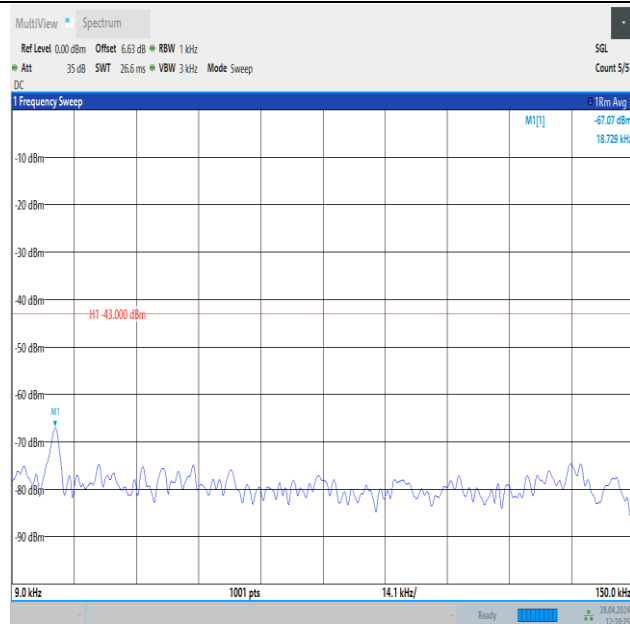
Band25_15MHz_QPSK_26115_1RB#0_0.009~0.15_0.009~0.15
