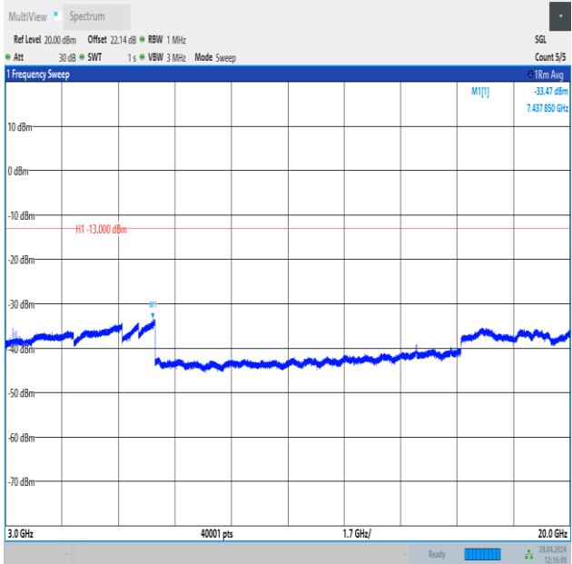
Band25_15MHz_16QAM_26365_1RB#74_3000~20000_3000~20000
