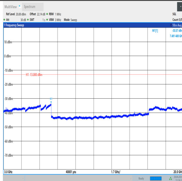
Band25_15MHz_16QAM_26615_1RB#0_3000~20000_3000~20000
