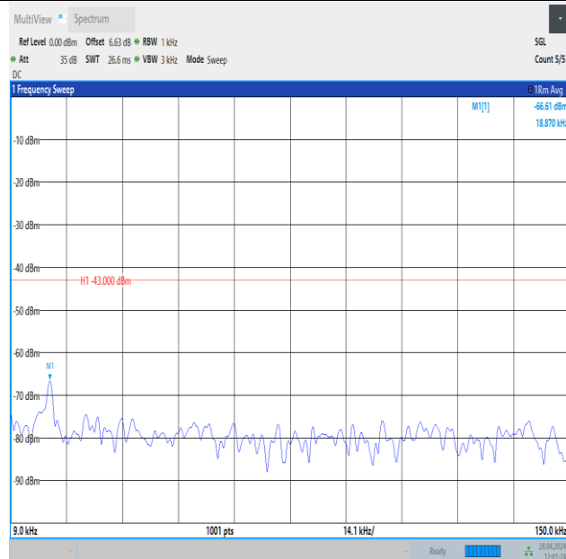
Band25_3MHz_16QAM_26365_15RB#0_0.009~0.15_0.009~0.15
