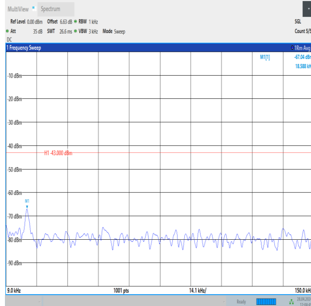
Band25_3MHz_16QAM_26675_1RB#14_0.009~0.15_0.009~0.15
