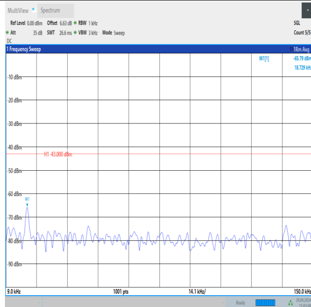
Band25_3MHz_16QAM_26675_1RB#0_0.009~0.15_0.009~0.15
