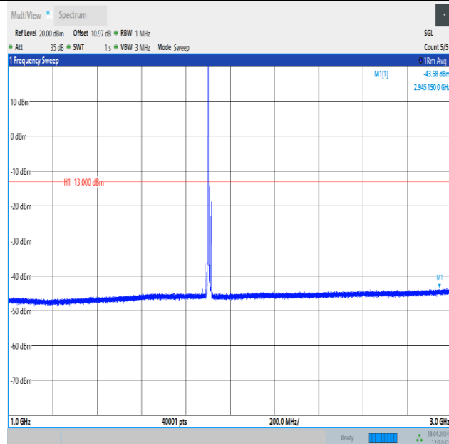
Band25_15MHz_QPSK_26615_1RB#0_1000~3000_1000~3000
