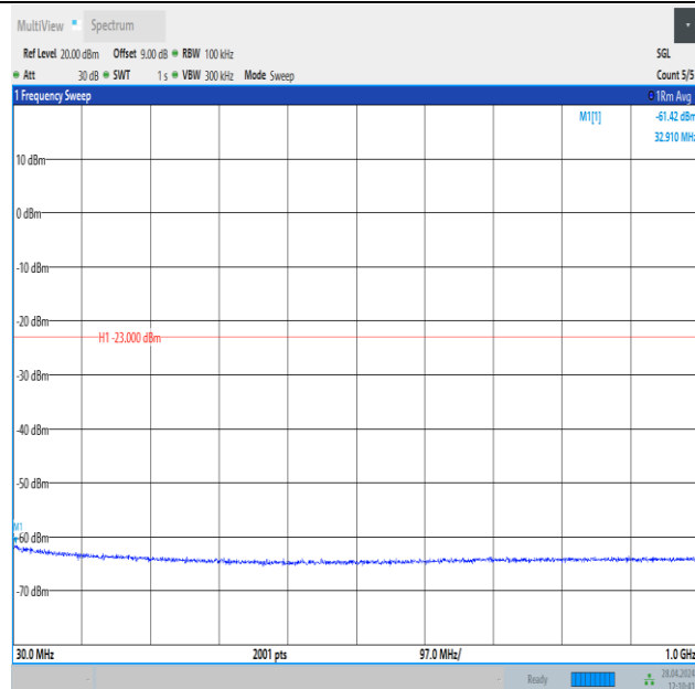
Band25_15MHz_QPSK_26115_1RB#0_30~1000_30~1000
