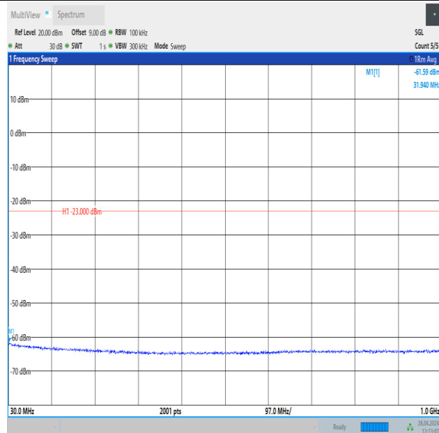
Band25_15MHz_16QAM_26115_1RB#74_30~1000_30~1000
