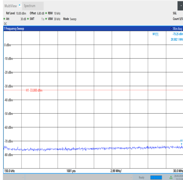
Band25_15MHz_16QAM_26115_1RB#74_0.15~30_0.15~30
