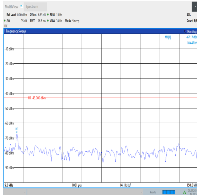
Band25_15MHz_16QAM_26115_1RB#74_0.009~0.15_0.009~0.15
