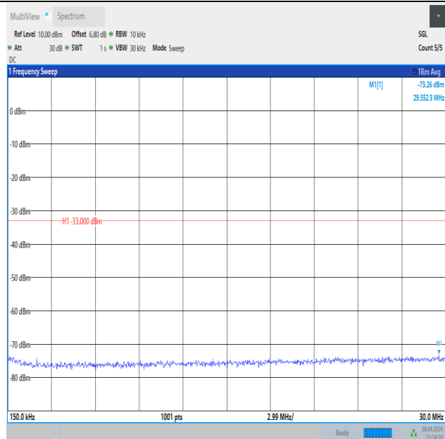
Band25_15MHz_16QAM_26365_1RB#0_0.15~30_0.15~30
