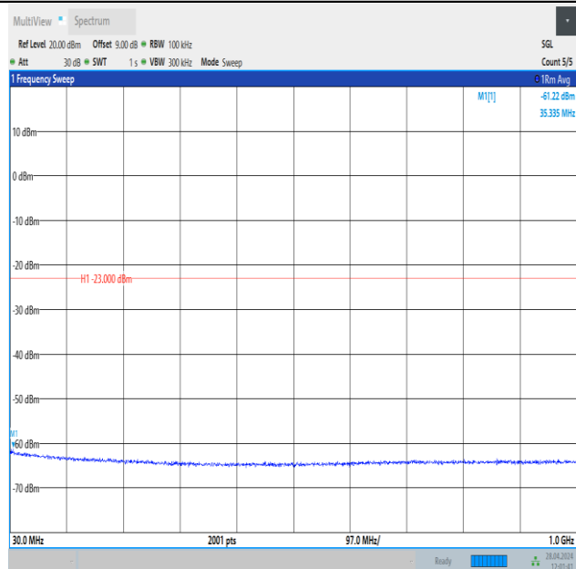
Band25_3MHz_16QAM_26365_15RB#0_30~1000_30~1000
