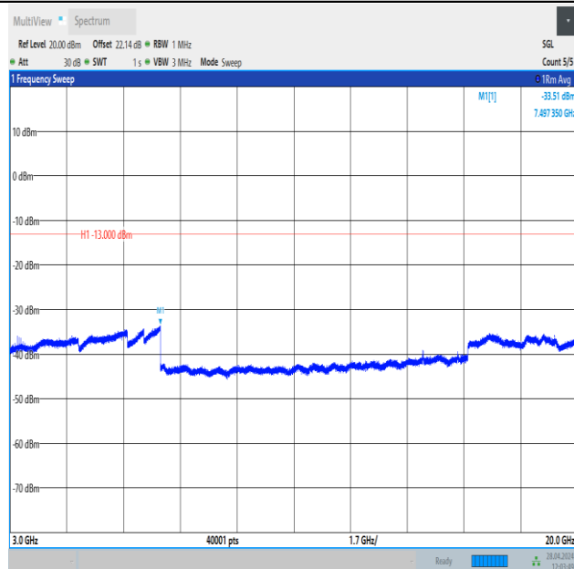
Band25_3MHz_16QAM_26675_1RB#0_3000~20000_3000~20000
