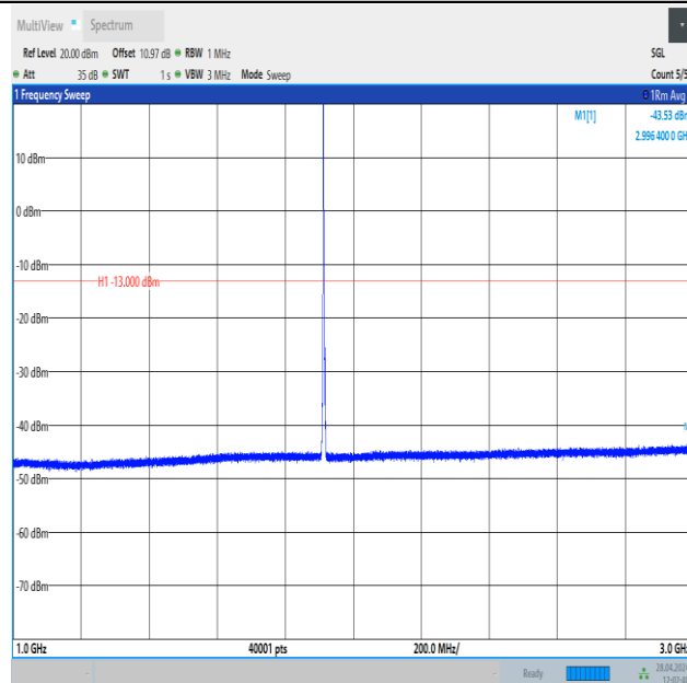
Band25_3MHz_QPSK_26675_1RB#0_1000~3000_1000~3000
