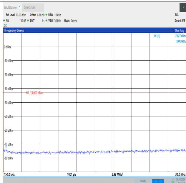
Band25_15MHz_16QAM_26615_1RB#74_0.15~30_0.15~30
