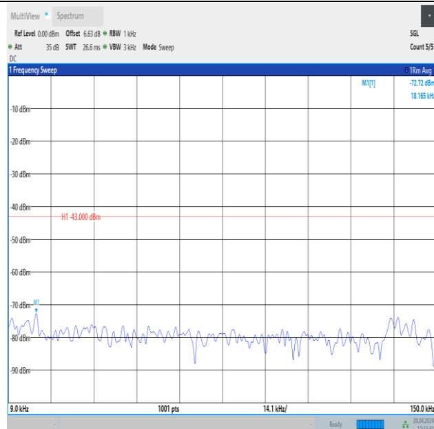
Band25_15MHz_QPSK_26365_1RB#0_0.009~0.15_0.009~0.15
