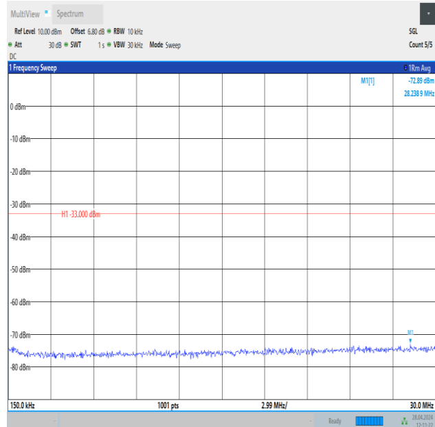
Band25_15MHz_16QAM_26115_1RB#0_0.15~30_0.15~30
