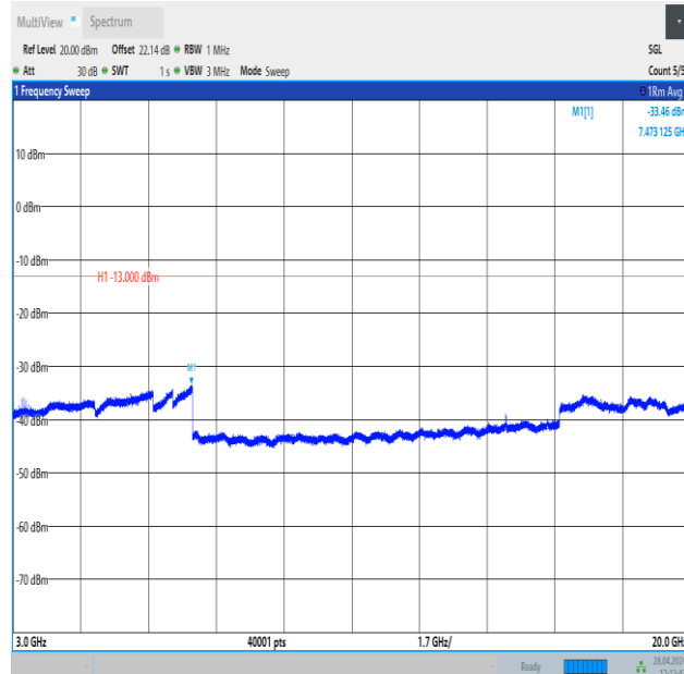
Band25_15MHz_QPSK_26115_1RB#74_3000~20000_3000~20000
