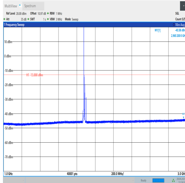
Band25_15MHz_16QAM_26365_1RB#0_1000~3000_1000~3000
