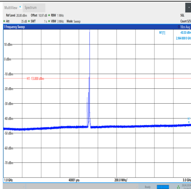
Band25_15MHz_16QAM_26615_1RB#74_1000~3000_1000~3000
