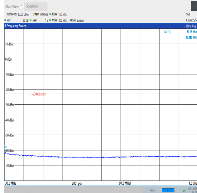
Band25_3MHz_QPSK_26675_1RB#14_30~1000_30~1000
