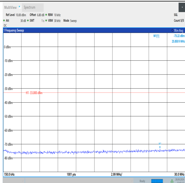
Band25_3MHz_16QAM_26365_15RB#0_0.15~30_0.15~30
