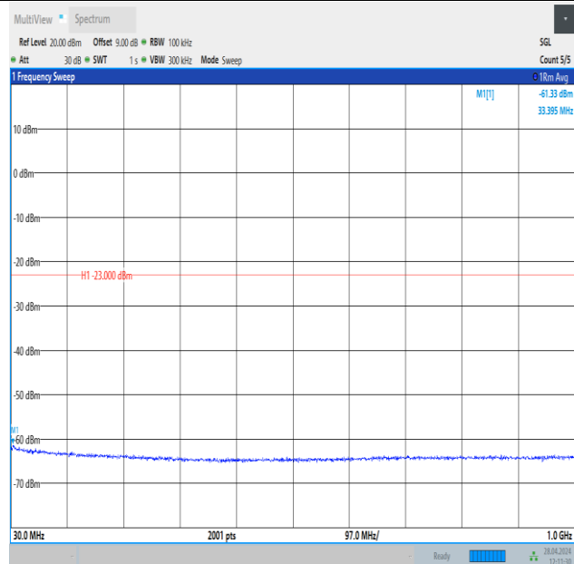
Band25_15MHz_16QAM_26115_1RB#0_30~1000_30~1000
