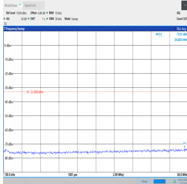
Band25_15MHz_QPSK_26365_1RB#0_0.15~30_0.15~30
