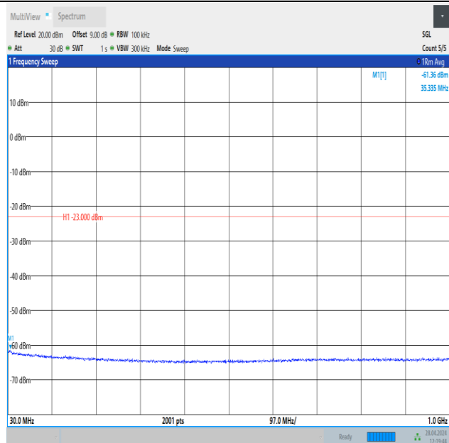
Band25_15MHz_16QAM_26615_1RB#74_30~1000_30~1000
