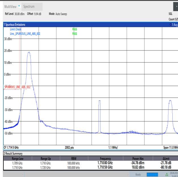
Band4_10MHz_16QAM_20000_1RB#0
