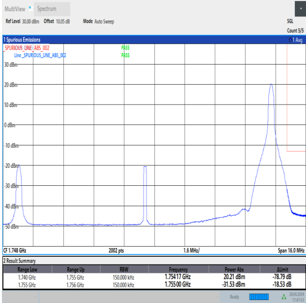
Band4_15MHz_16QAM_20325_1RB#74
