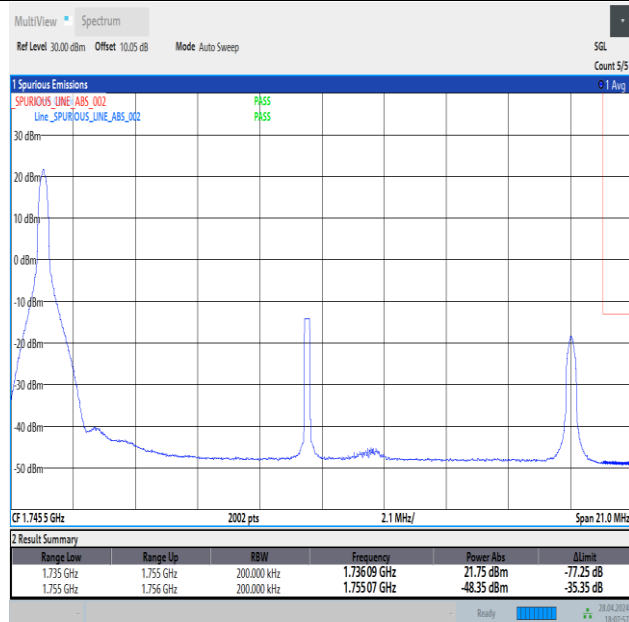
Band4_20MHz_16QAM_20300_1RB#0
