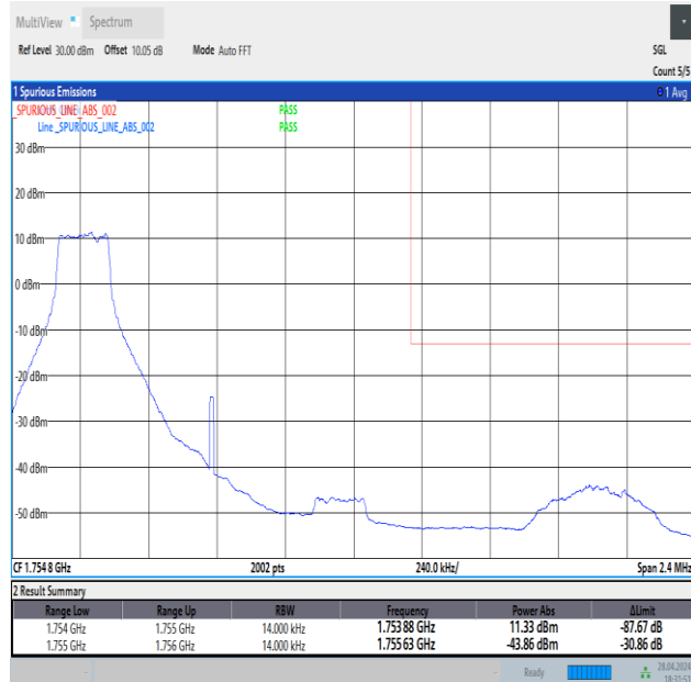
Band4_1.4MHz_QPSK_20393_1RB#0
