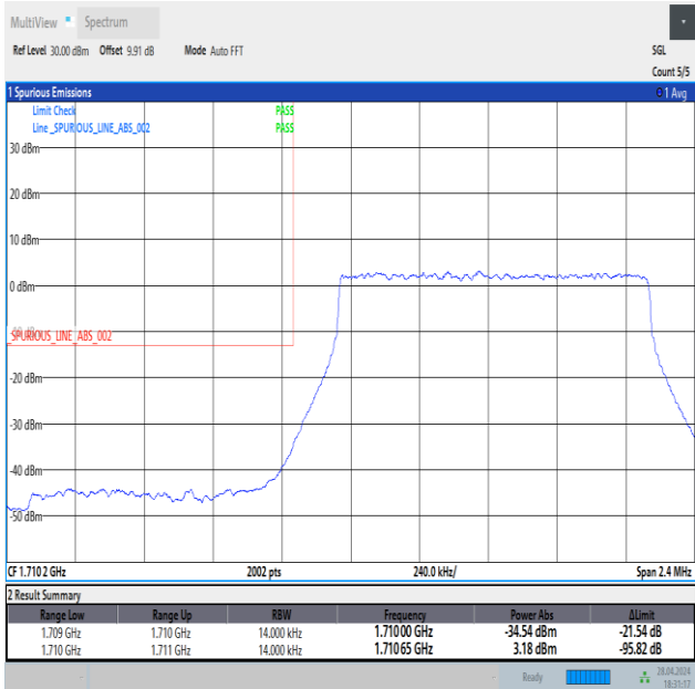
Band4_1.4MHz_QPSK_19957_6RB#0
