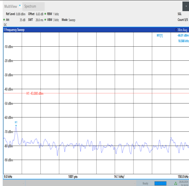
Band4_3MHz_16QAM_20175_1RB#0_0.009~0.15_0.009~0.15
