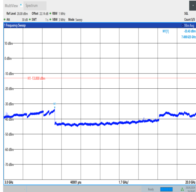
Band4_3MHz_16QAM_19965_1RB#0_3000~20000_3000~20000
