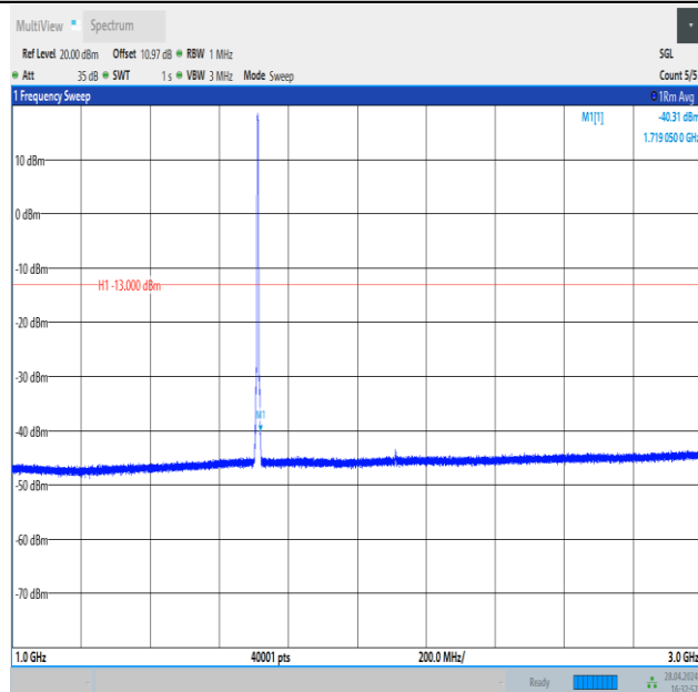
Band4_3MHz_QPSK_19965_15RB#0_1000~3000_1000~3000
