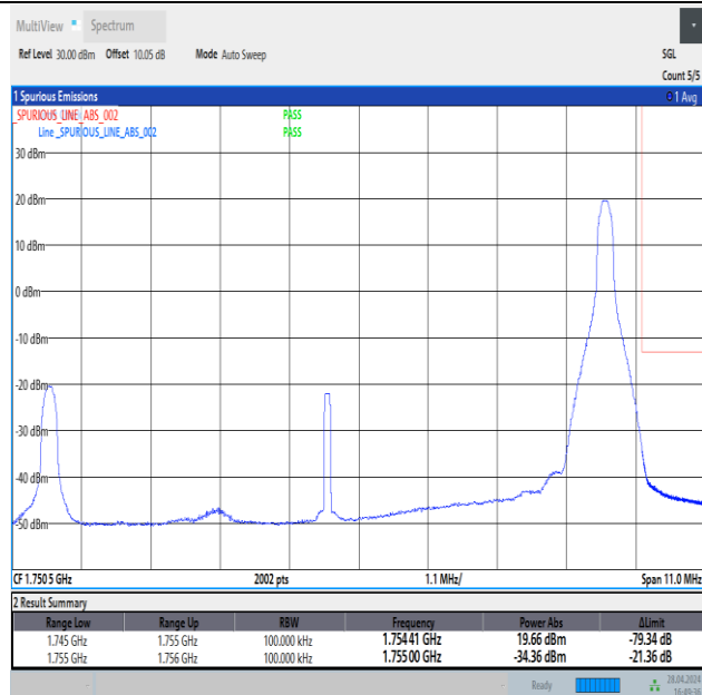
Band4_10MHz_QPSK_20350_1RB#49
