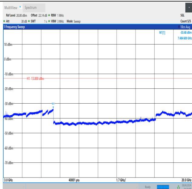
Band4_3MHz_QPSK_20175_1RB#0_3000~20000_3000~20000
