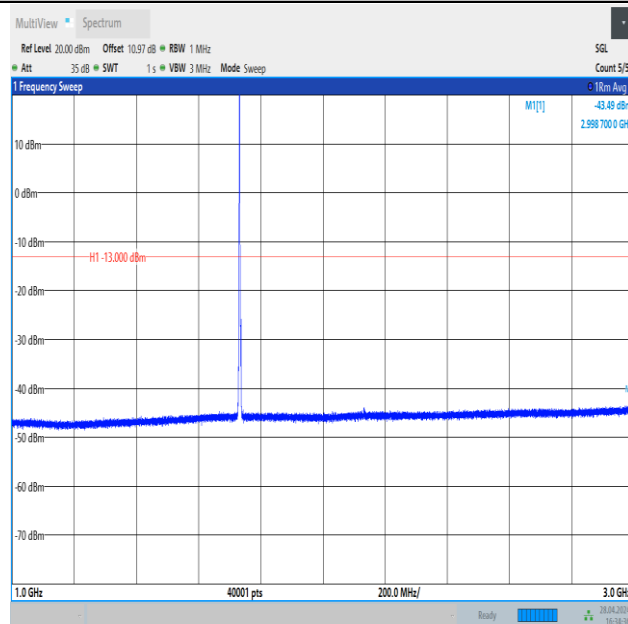
Band4_3MHz_QPSK_20175_1RB#0_1000~3000_1000~3000
