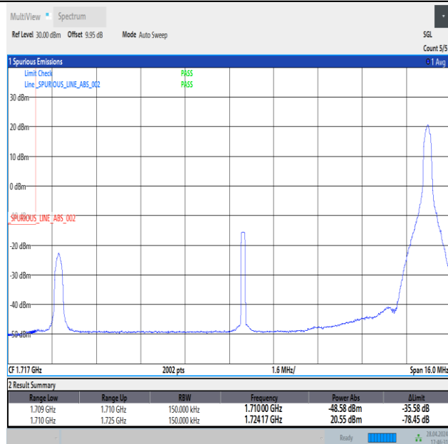
Band4_15MHz_16QAM_20025_1RB#74
