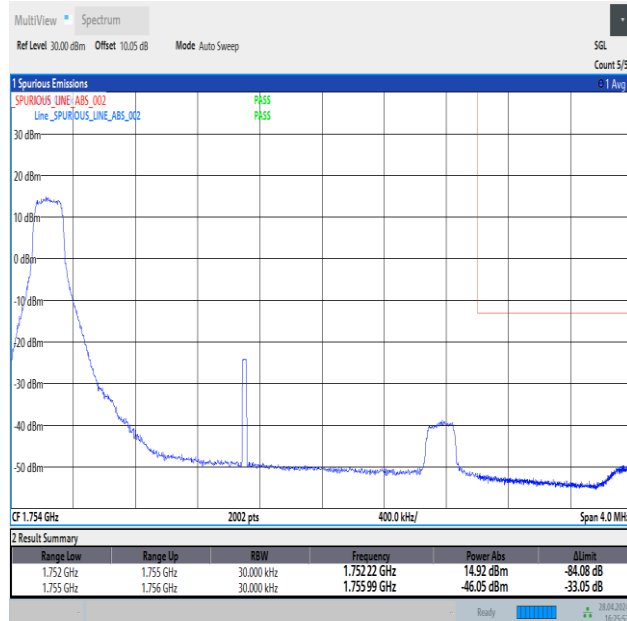
Band4_3MHz_QPSK_20385_1RB#0
