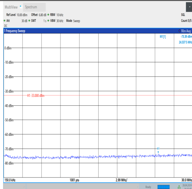
Band4_3MHz_16QAM_20175_1RB#0_0.15~30_0.15~30
