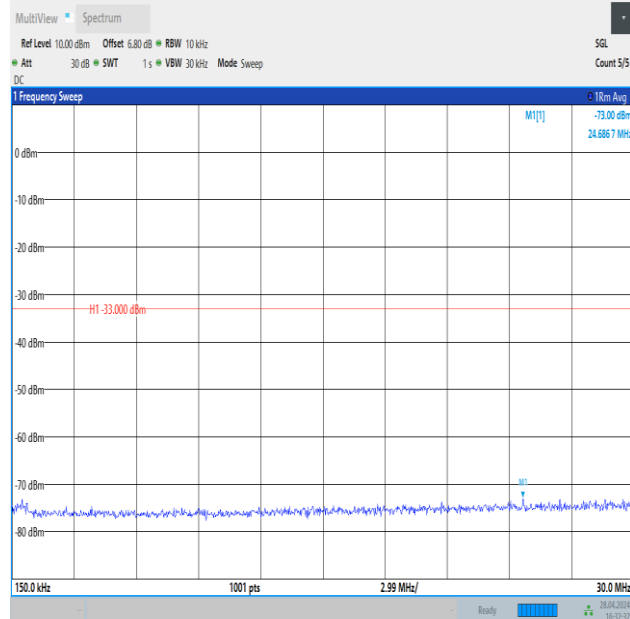
Band4_3MHz_QPSK_19965_15RB#0_0.15~30_0.15~30
