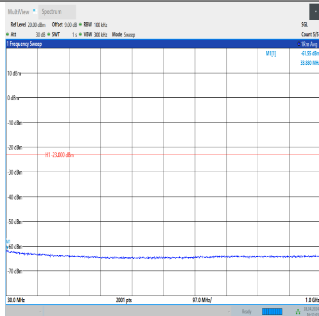
Band4_3MHz_QPSK_19965_1RB#14_30~1000_30~1000
