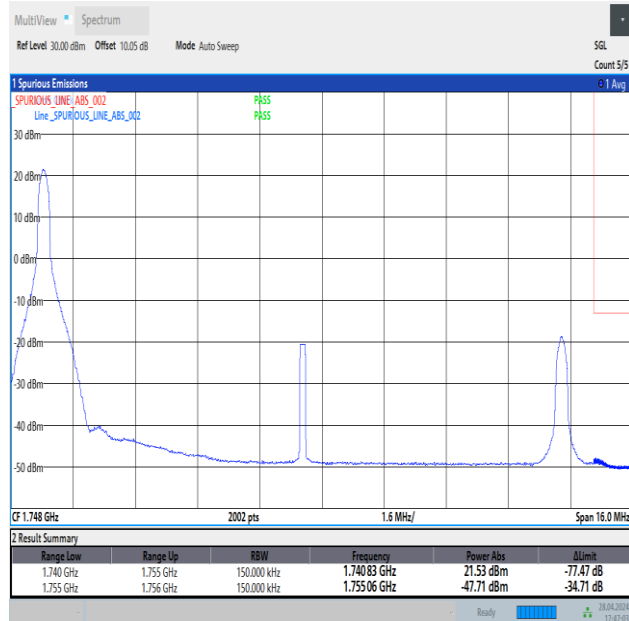
Band4_15MHz_QPSK_20325_1RB#0
