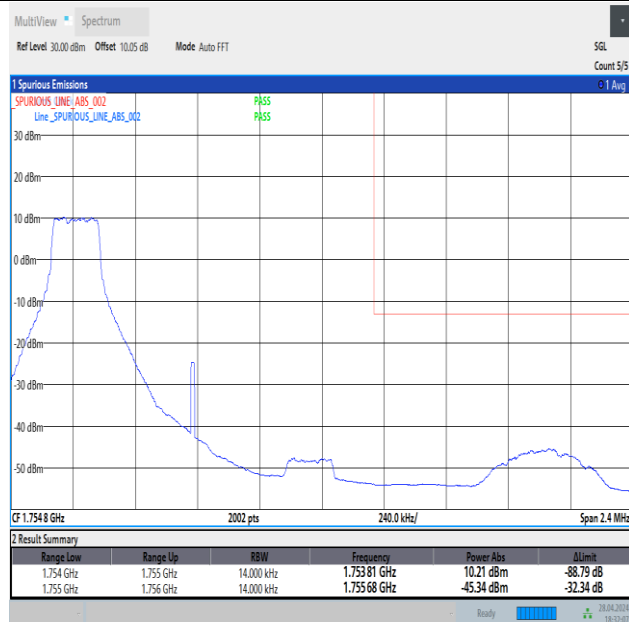
Band4_1.4MHz_16QAM_20393_1RB#0
