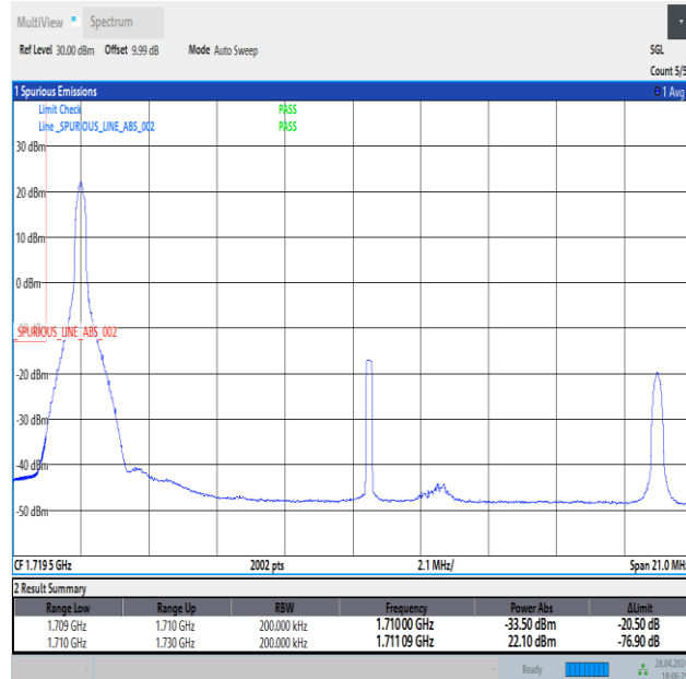
Band4_20MHz_QPSK_20050_1RB#0
