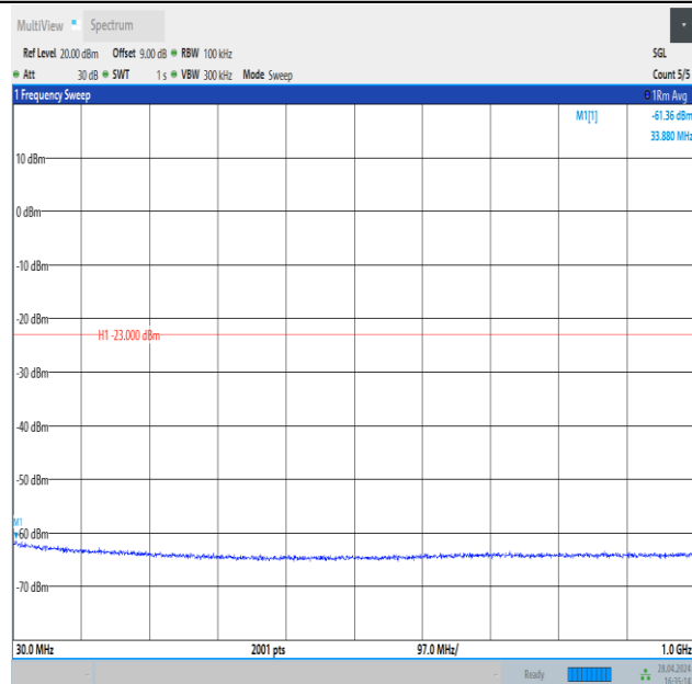
Band4_3MHz_16QAM_20175_1RB#0_30~1000_30~1000
