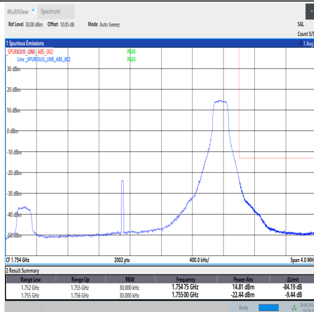
Band4_3MHz_QPSK_20385_1RB#14
