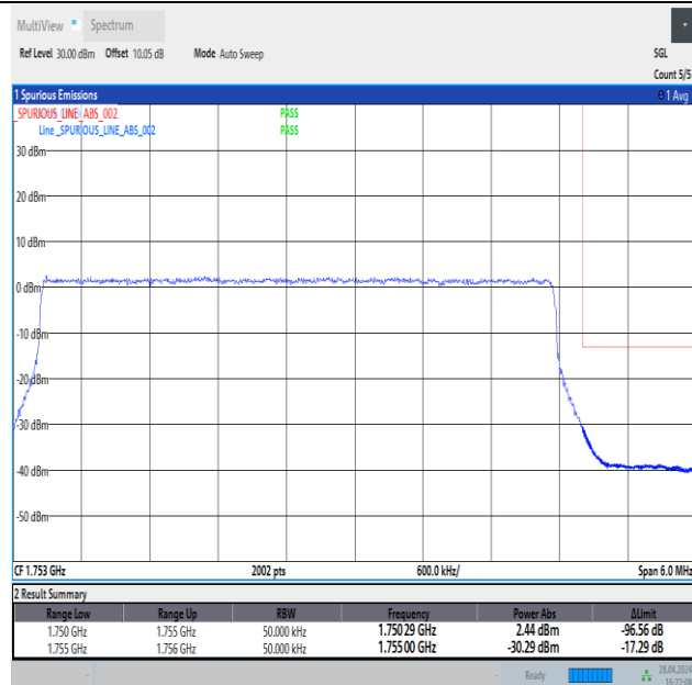
Band4_5MHz_QPSK_20375_25RB#0
