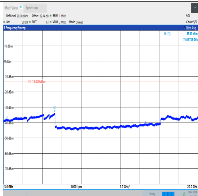
Band4_3MHz_QPSK_19965_15RB#0_3000~20000_3000~20000
