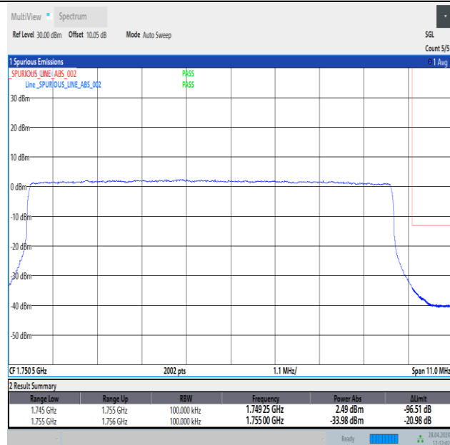
Band4_10MHz_QPSK_20350_50RB#0
