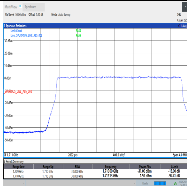
Band4_3MHz_16QAM_19965_15RB#0
