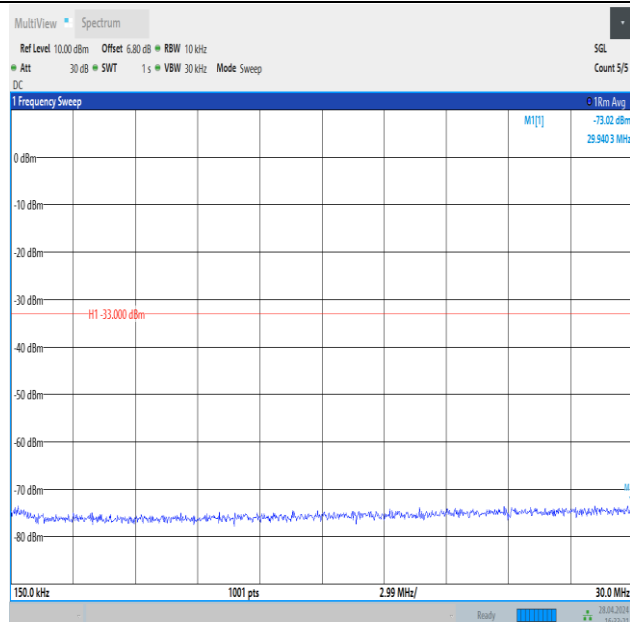
Band4_3MHz_16QAM_19965_15RB#0_0.15~30_0.15~30
