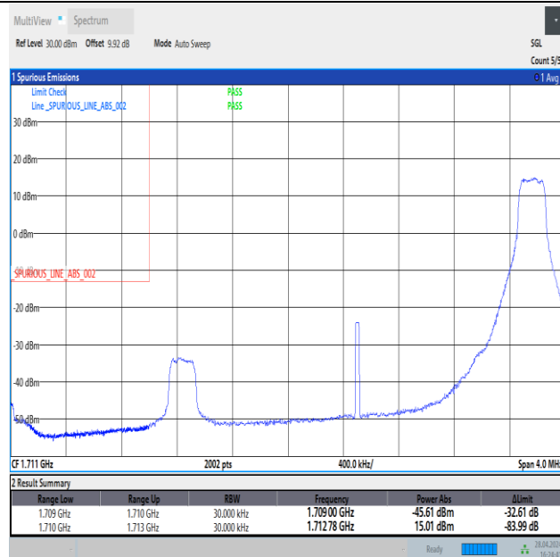
Band4_3MHz_QPSK_19965_1RB#14
