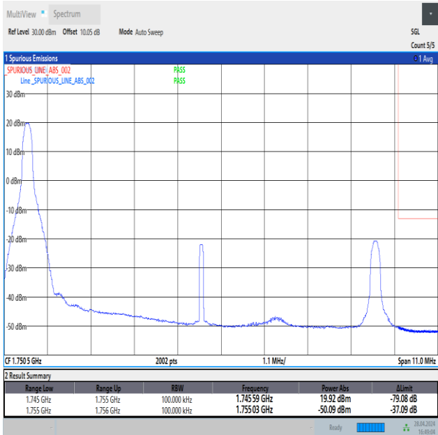
Band4_10MHz_QPSK_20350_1RB#0
