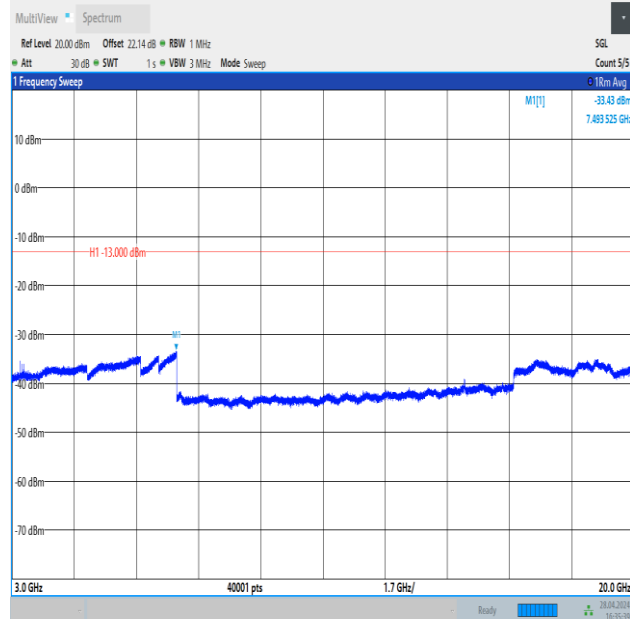
Band4_3MHz_16QAM_20175_1RB#0_3000~20000_3000~20000
