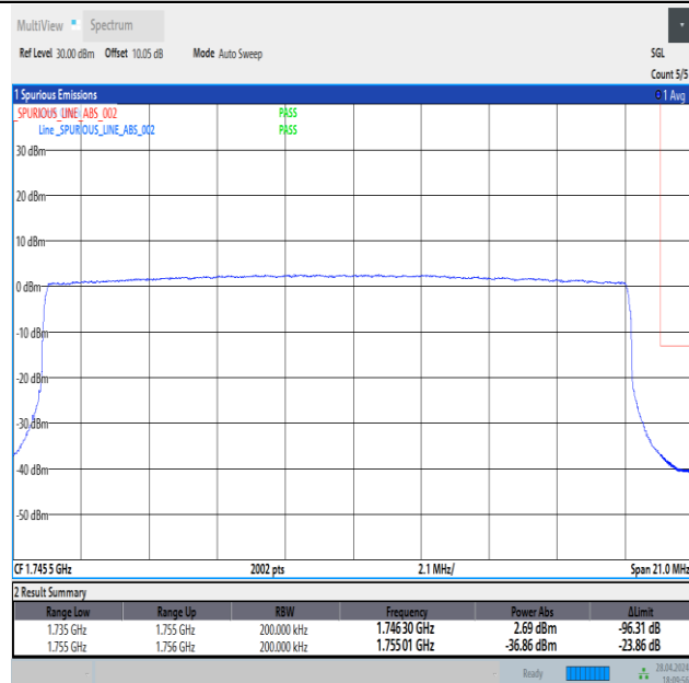
Band4_20MHz_QPSK_20300_100RB#0
