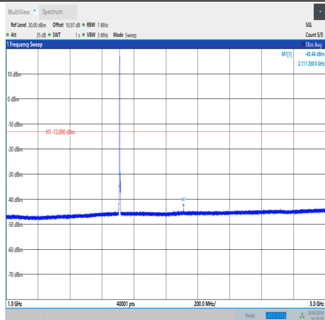
Band4_3MHz_QPSK_19965_1RB#0_1000~3000_1000~3000
