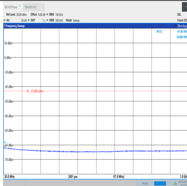
Band4_3MHz_QPSK_20175_1RB#14_30~1000_30~1000
