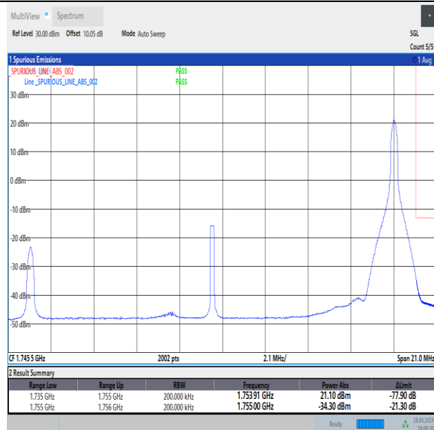
Band4_20MHz_16QAM_20300_1RB#99
