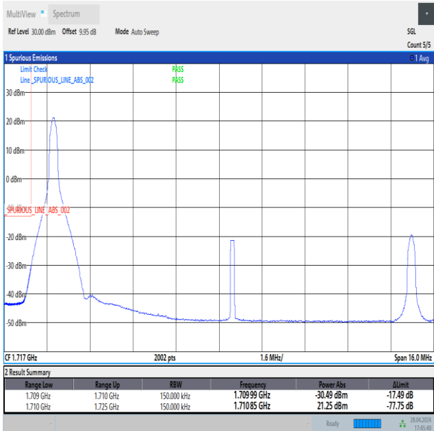
Band4_15MHz_QPSK_20025_1RB#0
