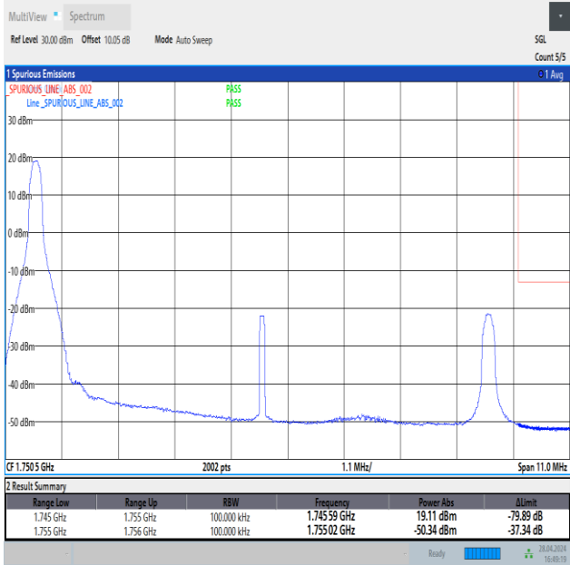
Band4_10MHz_16QAM_20350_1RB#0
