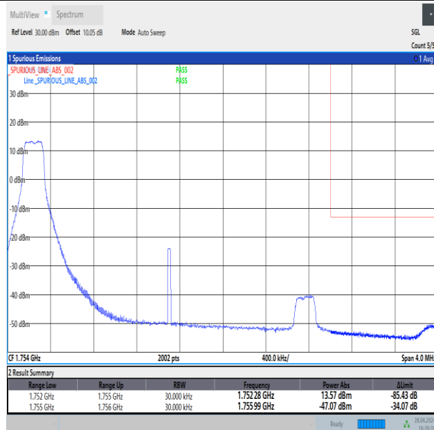
Band4_3MHz_16QAM_20385_1RB#0
