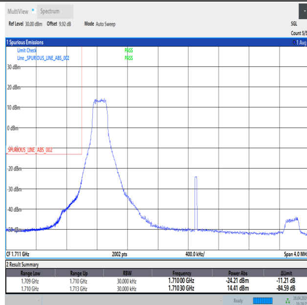
Band4_3MHz_16QAM_19965_1RB#0
