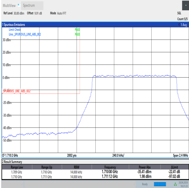
Band4_1.4MHz_16QAM_19957_6RB#0
