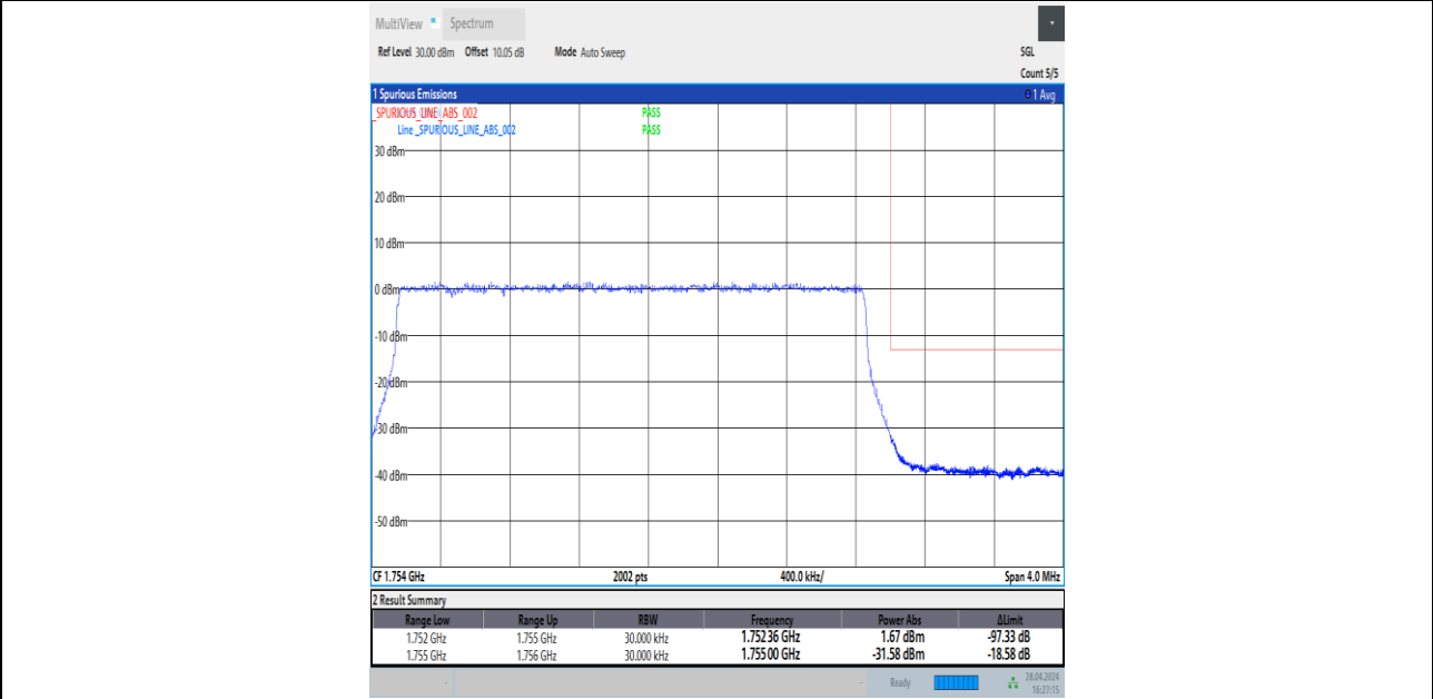
Band4_3MHz_16QAM_20385_15RB#0
