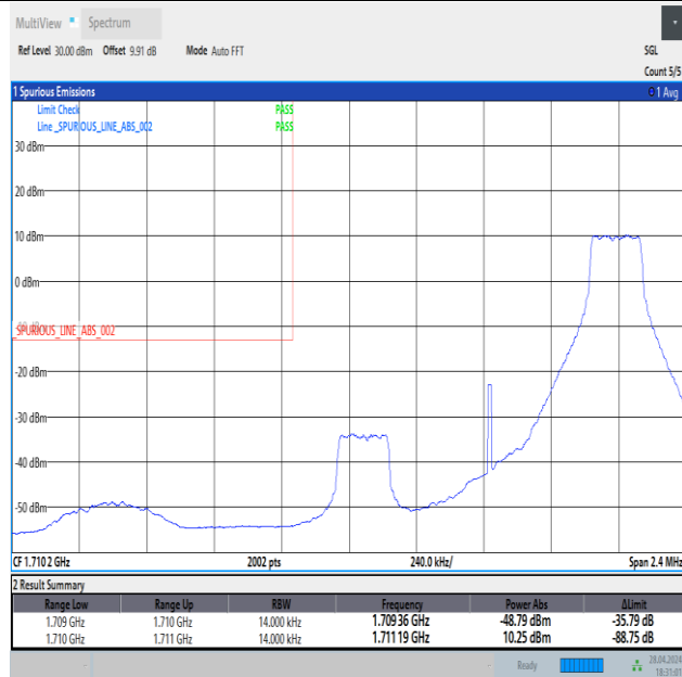
Band4_1.4MHz_16QAM_19957_1RB#5
