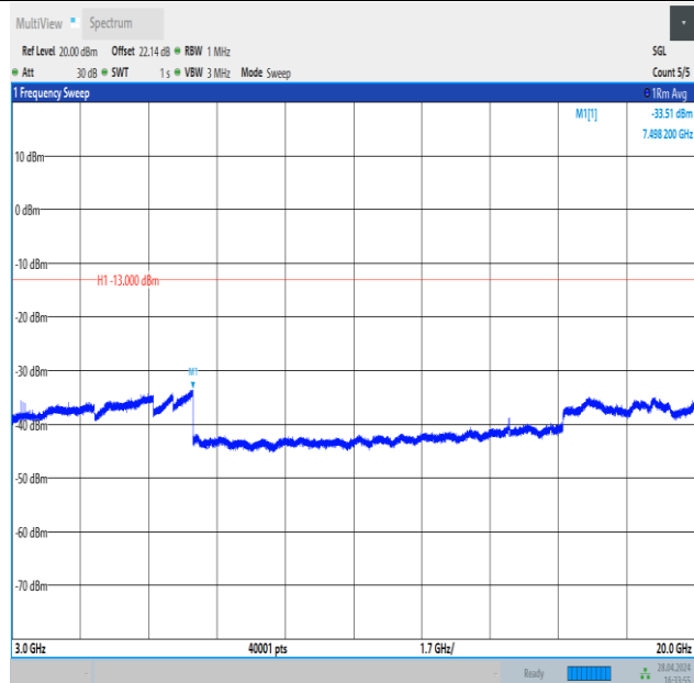
Band4_3MHz_16QAM_19965_15RB#0_3000~20000_3000~20000
