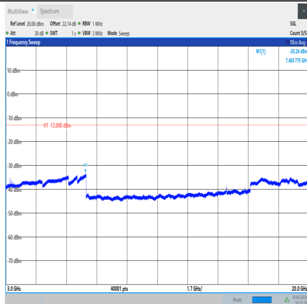
Band4_3MHz_16QAM_19965_1RB#14_3000~20000_3000~20000
