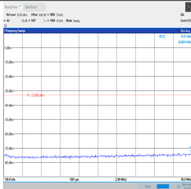
Band4_3MHz_16QAM_19965_1RB#0_0.15~30_0.15~30
