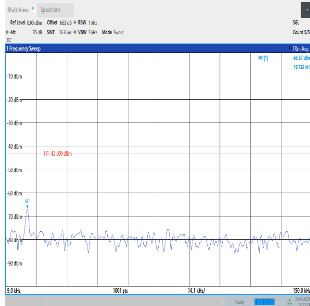
Band4_3MHz_QPSK_19965_15RB#0_0.009~0.15_0.009~0.15
