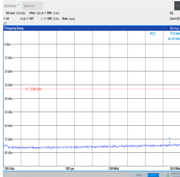
Band4_3MHz_16QAM_19965_1RB#14_0.15~30_0.15~30
