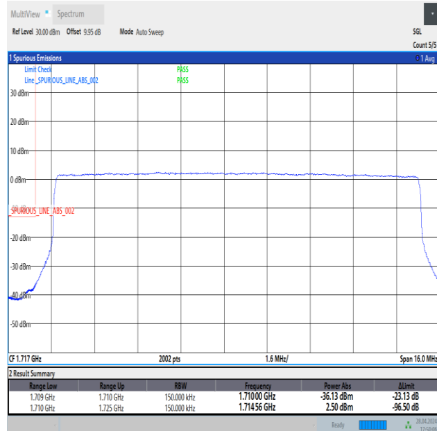
Band4_15MHz_QPSK_20025_75RB#0
