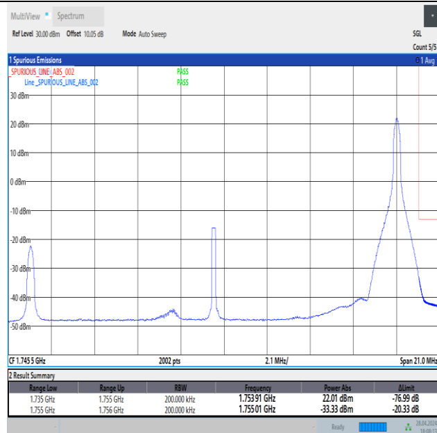
Band4_20MHz_QPSK_20300_1RB#99
