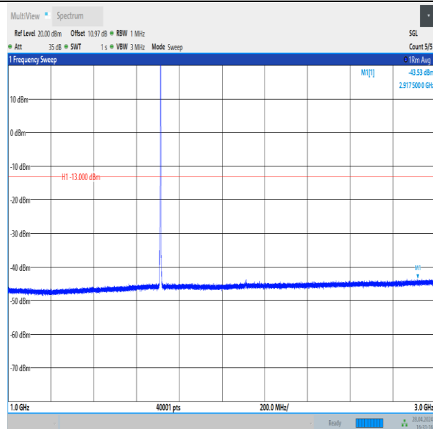
Band4_3MHz_QPSK_19965_1RB#14_1000~3000_1000~3000
