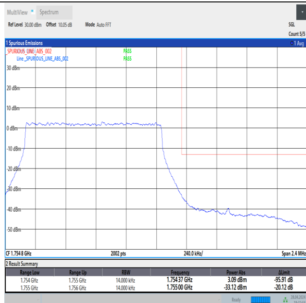
Band4_1.4MHz_QPSK_20393_6RB#0
