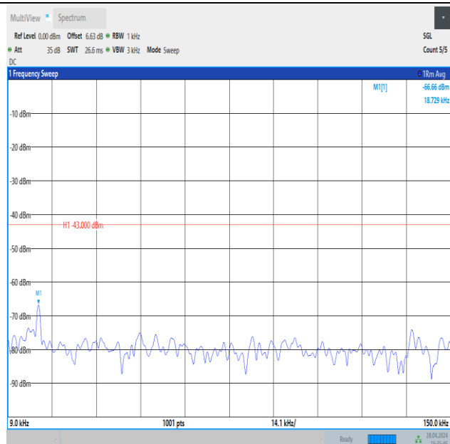
Band4_3MHz_QPSK_20175_1RB#14_0.009~0.15_0.009~0.15
