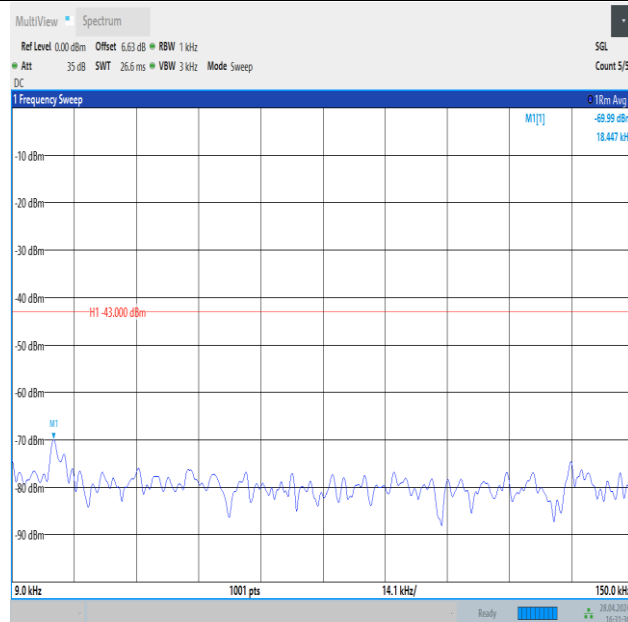
Band4_3MHz_16QAM_19965_1RB#14_0.009~0.15_0.009~0.15
