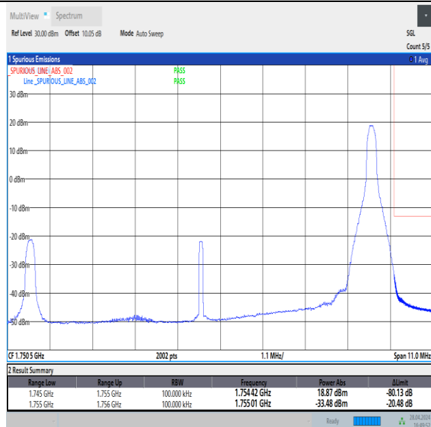
Band4_10MHz_16QAM_20350_1RB#49
