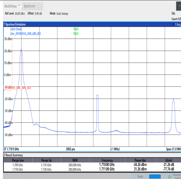
Band4_20MHz_16QAM_20050_1RB#0
