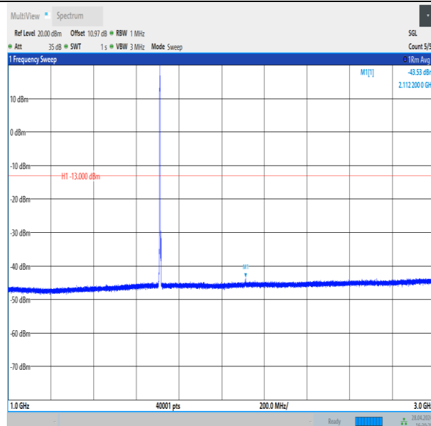
Band4_3MHz_16QAM_19965_1RB#0_1000~3000_1000~3000
