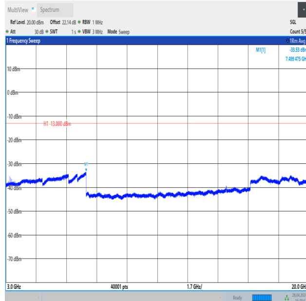
Band4_3MHz_QPSK_19965_1RB#0_3000~20000_3000~20000
