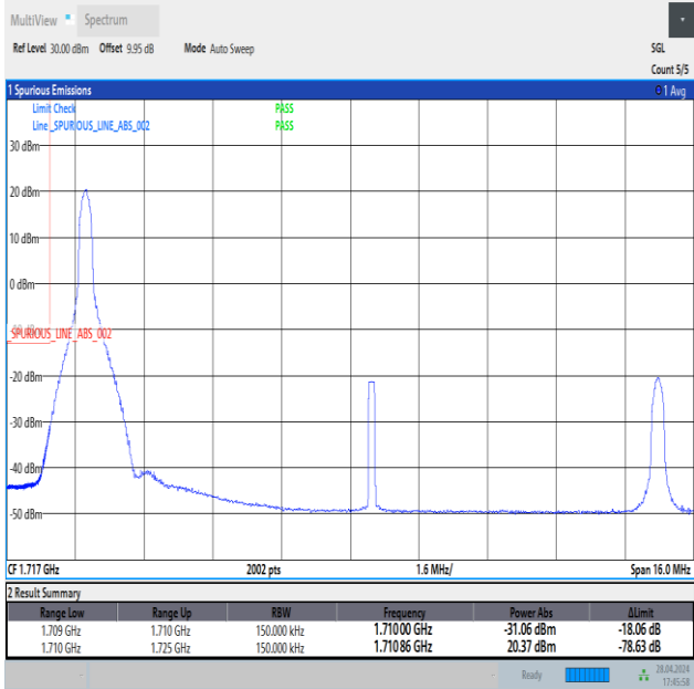
Band4_15MHz_16QAM_20025_1RB#0
