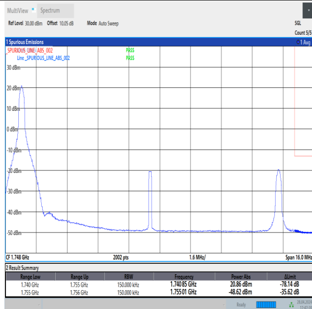
Band4_15MHz_16QAM_20325_1RB#0
