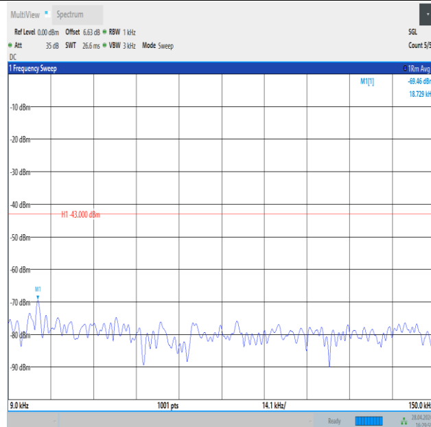
Band4_3MHz_16QAM_19965_1RB#0_0.009~0.15_0.009~0.15
