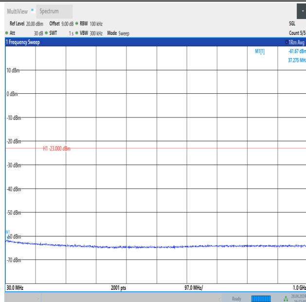
Band4_3MHz_QPSK_19965_15RB#0_30~1000_30~1000
