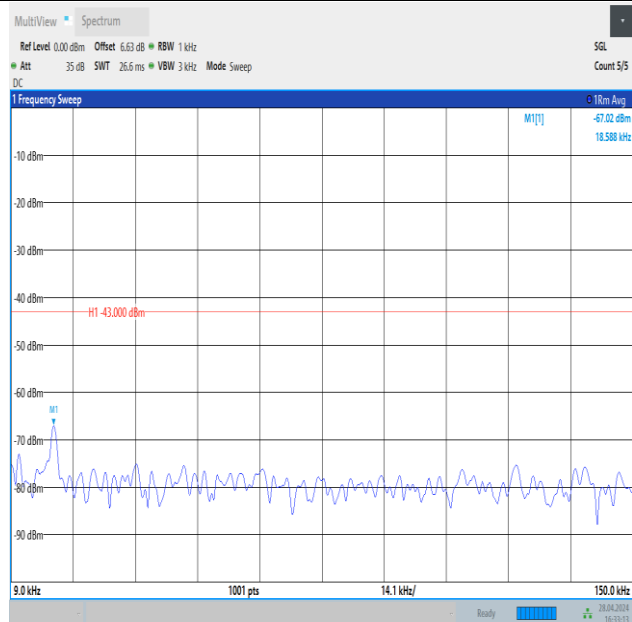
Band4_3MHz_16QAM_19965_15RB#0_0.009~0.15_0.009~0.15
