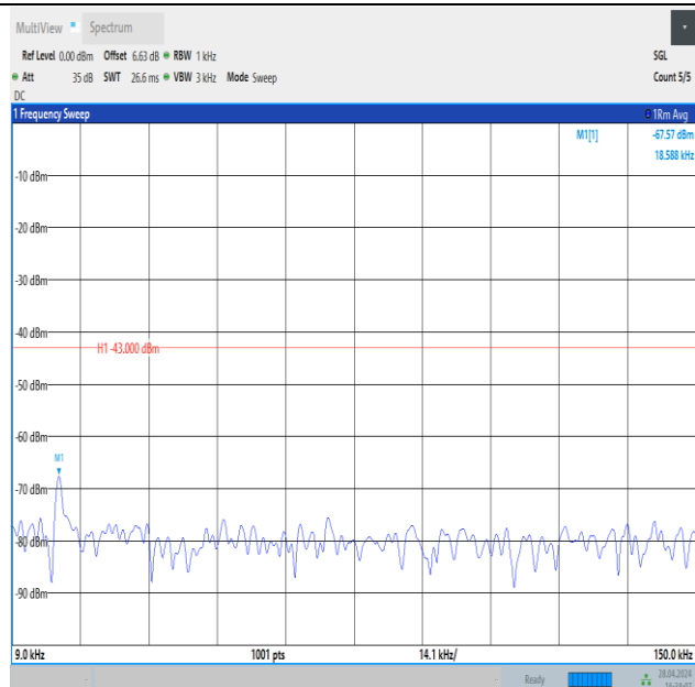
Band4_3MHz_QPSK_20175_1RB#0_0.009~0.15_0.009~0.15
