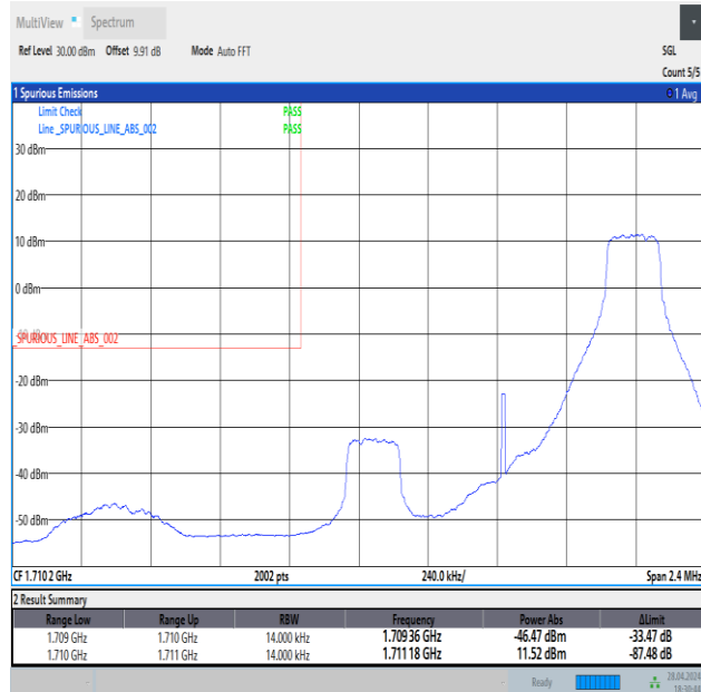
Band4_1.4MHz_QPSK_19957_1RB#5
