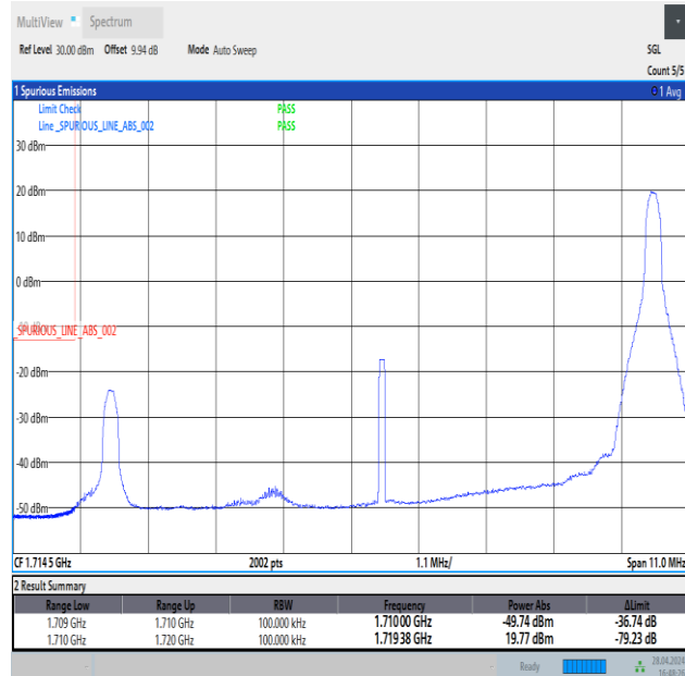
Band4_10MHz_QPSK_20000_1RB#49
