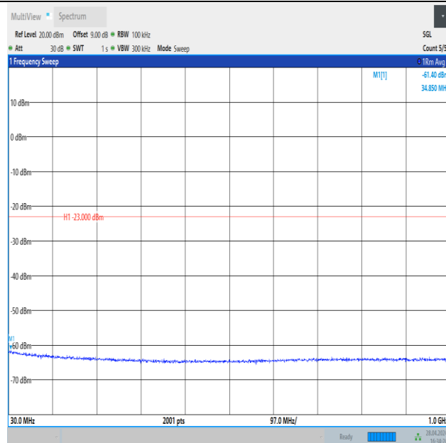
Band4_3MHz_QPSK_20175_1RB#0_30~1000_30~1000
