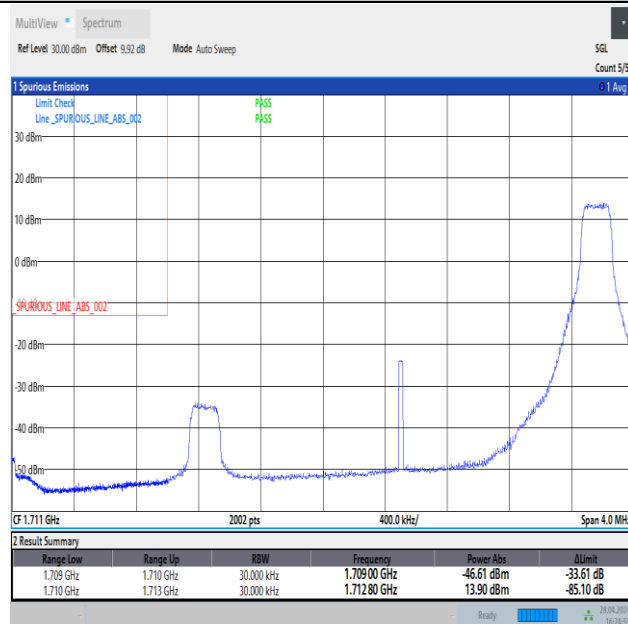
Band4_3MHz_16QAM_19965_1RB#14
