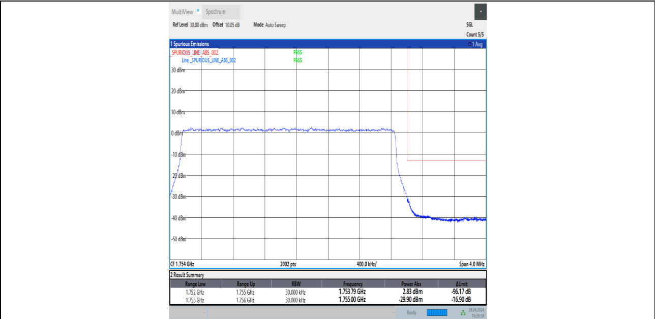
Band4_3MHz_QPSK_20385_15RB#0
