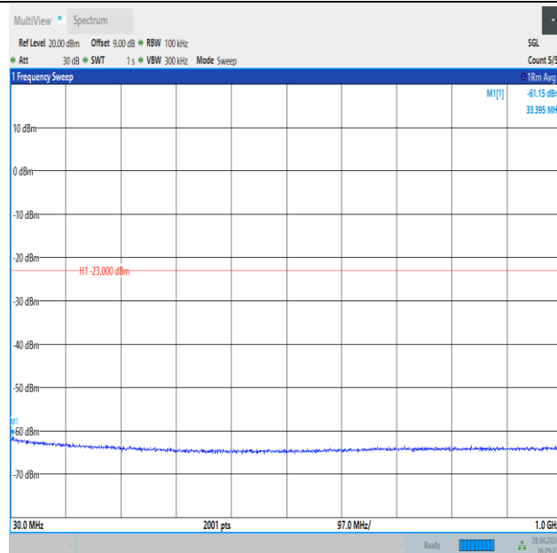
Band4_3MHz_QPSK_19965_1RB#0_30~1000_30~1000
