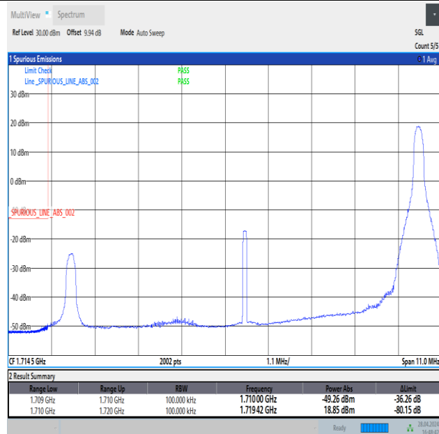
Band4_10MHz_16QAM_20000_1RB#49
