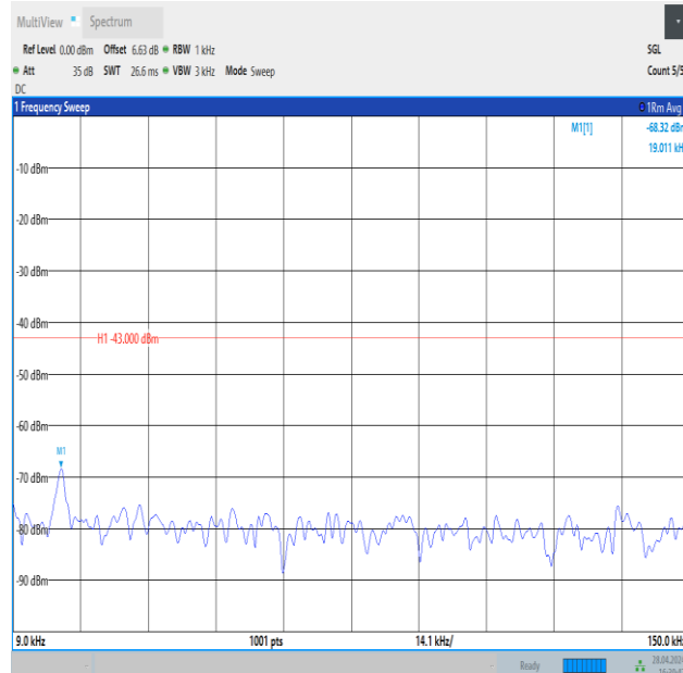
Band4_3MHz_QPSK_19965_1RB#14_0.009~0.15_0.009~0.15
